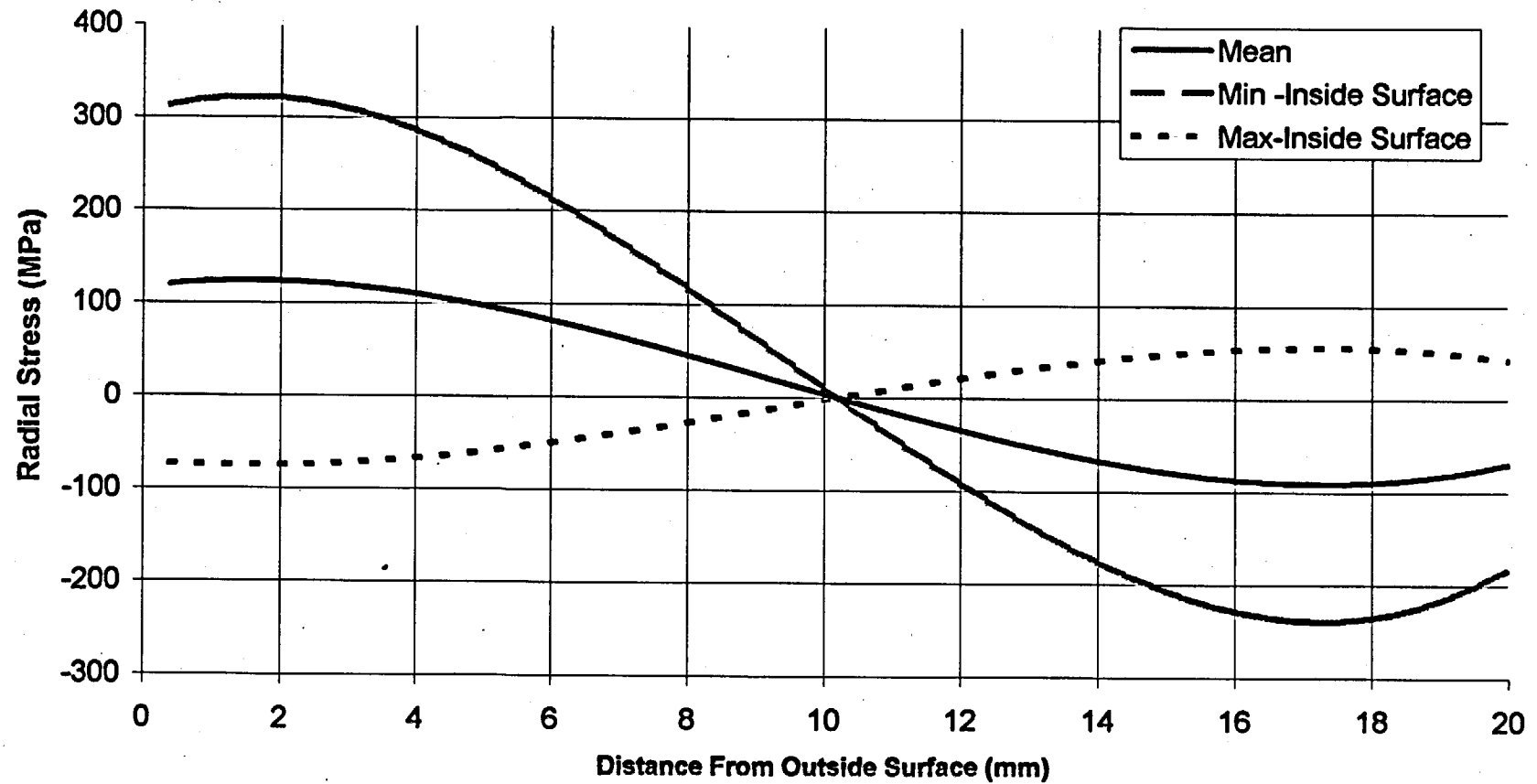
Unannealed, Outer Lid, Crack Originated From Outside Surface, Section 1-1, Sx, at 0 Deg
