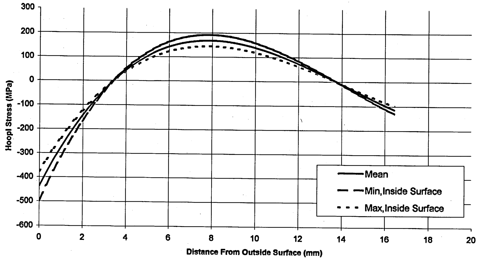
Peening, Middle Lid, Crack Originated From Outside Surface, Section 2-2, Sz, at 0 Deg
