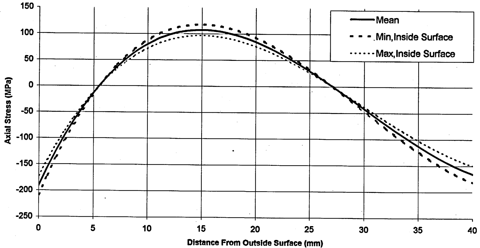
Peening, Middle Lid, Crack Originated From Outside Surface, Section 3-3, Sy at 0 Deg.
