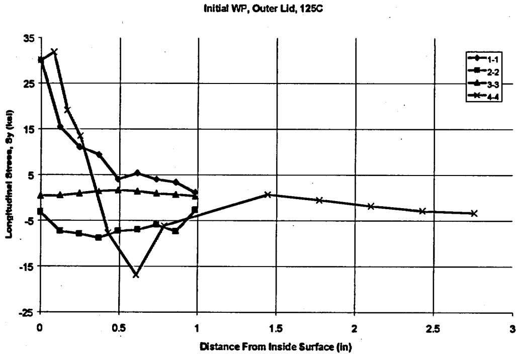
Figure 9. Longitudinal Stress, Outer Lid @ 125°C
