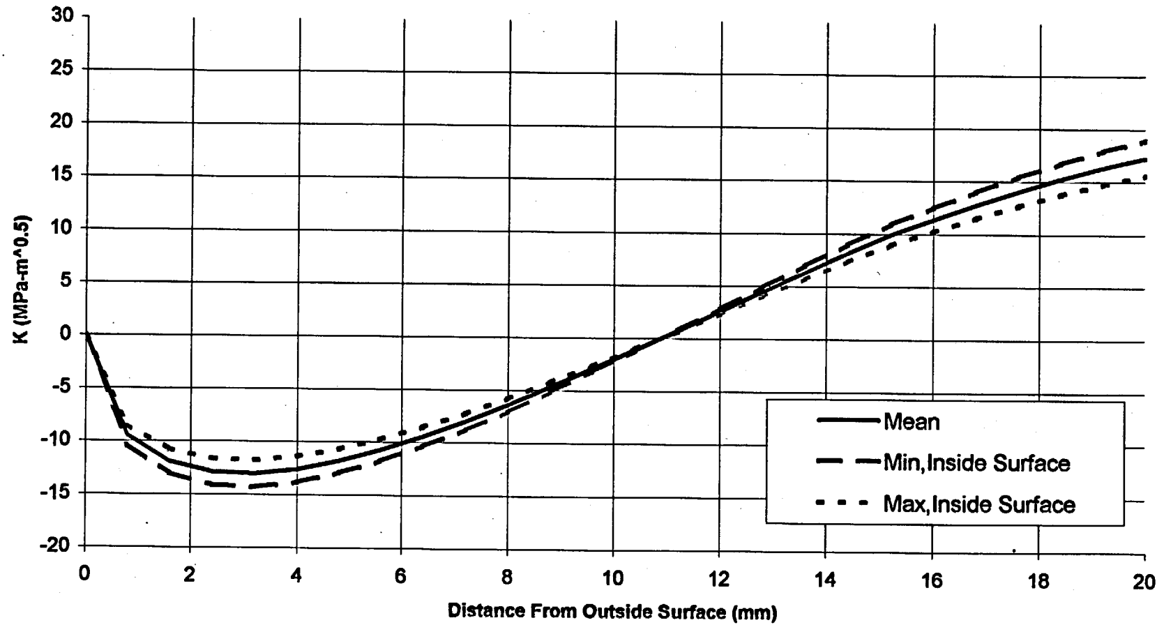
Peening, Middle Lid, Crack Originated From Outside Surface, Section 3-3, Sy, at 0 Deg
