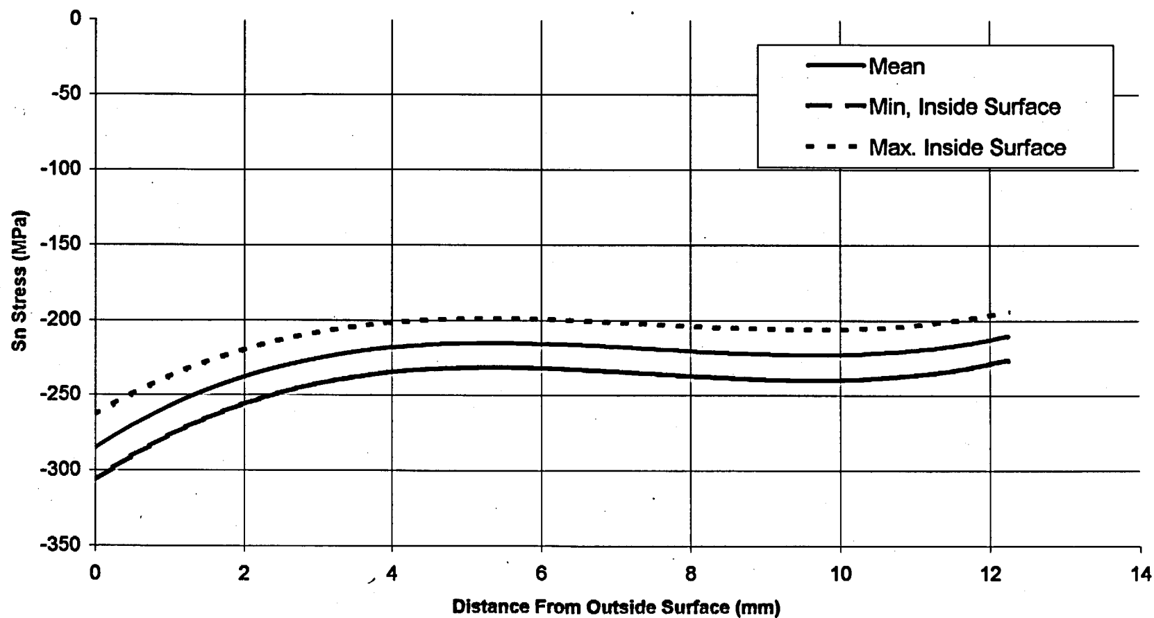
Peening, Middle Lid, Crack Originated From Outside Surface, Section 1-1, Sn, at 0 Deg
