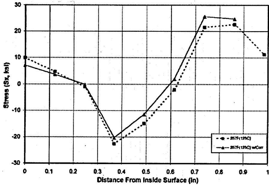
Figure 16. Effect of Corrosion on Radial Stress in Outer Lid
