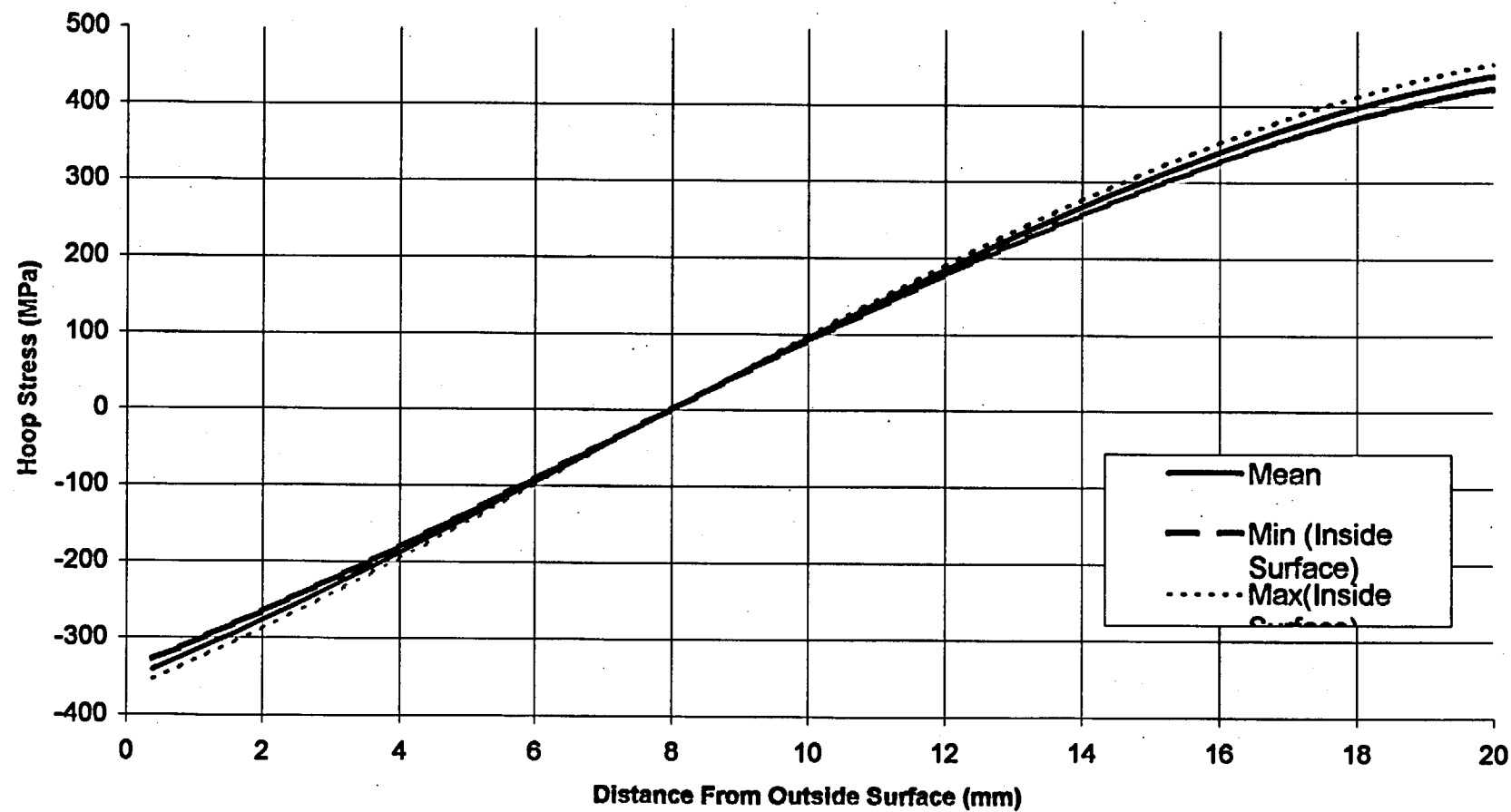
Annealed, Outer Lid, Crack Originated From Outside Surface, Sz, at 0 Deg
