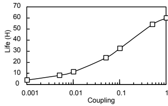
Figure 5: Touschek Lifetime
