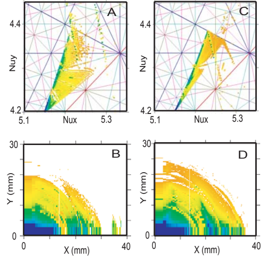
Figure 6: Frequency Map and Dynamic Aperture
