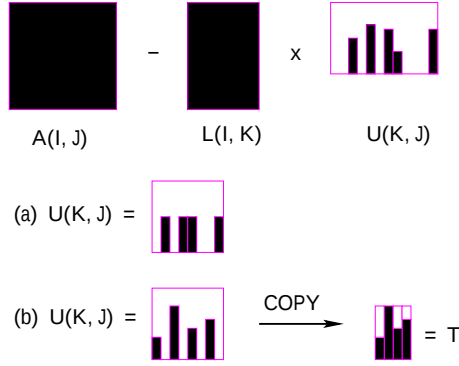
Figure 10: Illustration of the numerical kernels used in SuperLU_DIST .
