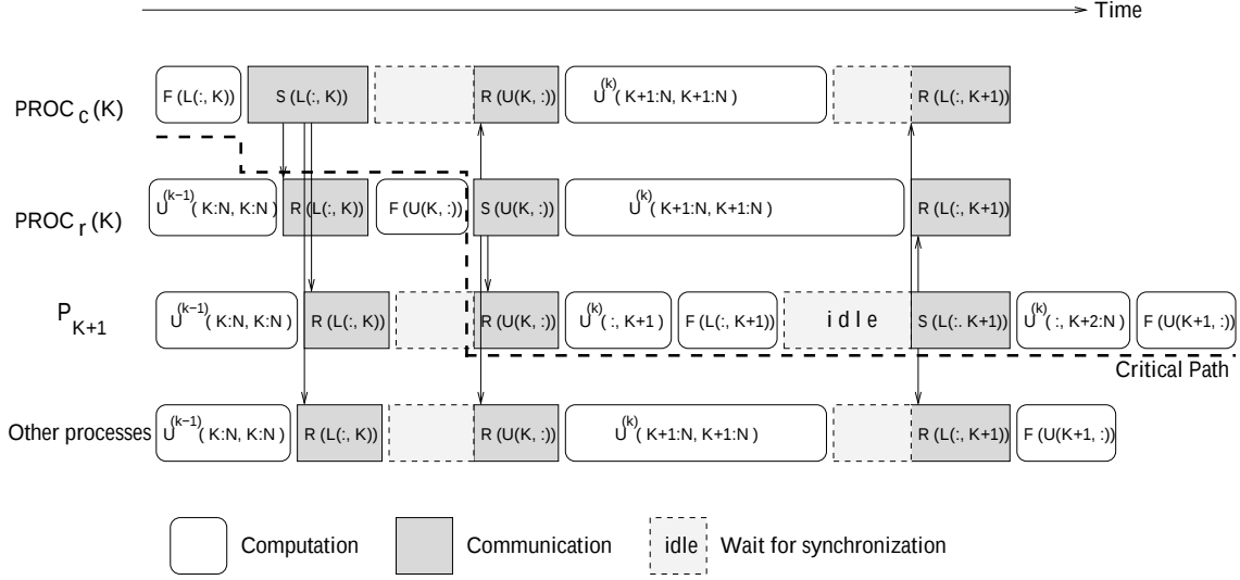
Figure 12: Illustration of the pipeline at Steps K and K + 1 during the SuperLU factorization.
