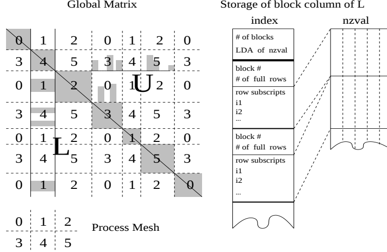
Figure 9: The 2D block-cyclic layout and the data structure to store a local block column of L .
