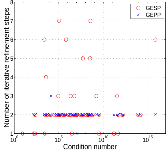
Figure 3: Iterative refinement steps.
