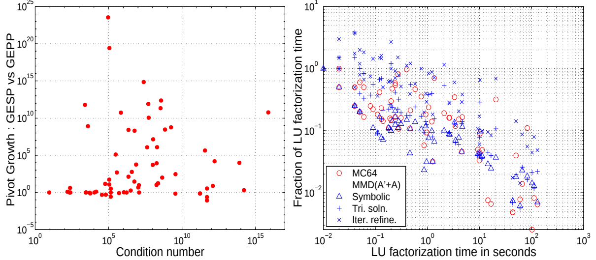
Figure 6: The ratio of pivot growth of GESP versus GEPP. Figure 7: The times for the other steps of GESP, as fraction of the factorization time.
