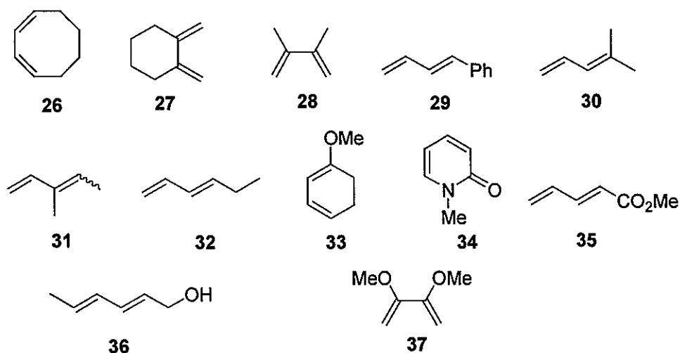
Figure 4. 1,3-Dienes investigated.
