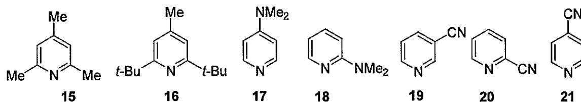
Figure 2. Pyridine bases.
