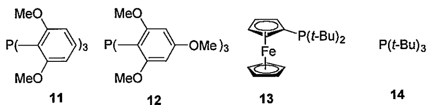
Figure 1. Phosphine ligands.
