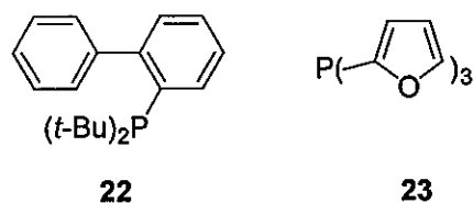
Figure 3. Phosphine ligands.
