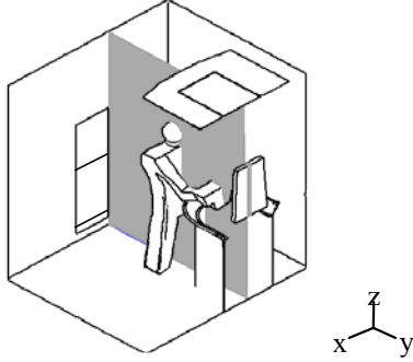
Figure 3: The Y-Z section used for displaying results. The plane passes through the middle of the figure showing the asymmetry of the downdraft table within the room. Center plane of downdraft table is 33"(0.84m) from the left wall and 56"(1.42m) from the right wall. This section illustrates the containment in front of the worker, and around the package.
