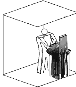
Figure 5. Particle tracks showing that all particles released are contained within the downdraft table for flow supplied through the back inlet at 1230 \text{ l/s} (2600 CFM) and the ceiling at 470 \text{ l/s} (1000 CFM).
