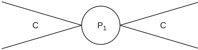
Figure 2: Moduli space for K = K' = 1 = N , \zeta \neq 0
