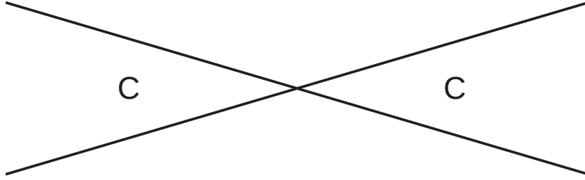
Figure 1: Moduli space for K = K' = 1 , \zeta = 0
