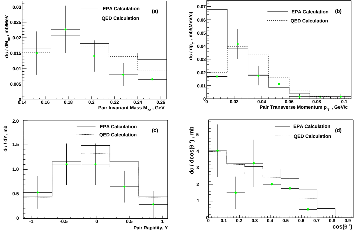
FIG. 2: (a) The pair mass distribution, (b) pair p_T , (c) pair rapidity and (d) pair \cos(\theta') distributions. The data (points) are compared with predictions from the EPA (solid histogram) and lowest-order QED (dashed histogram) calculations. The error bars include both statistical and systematic errors.
