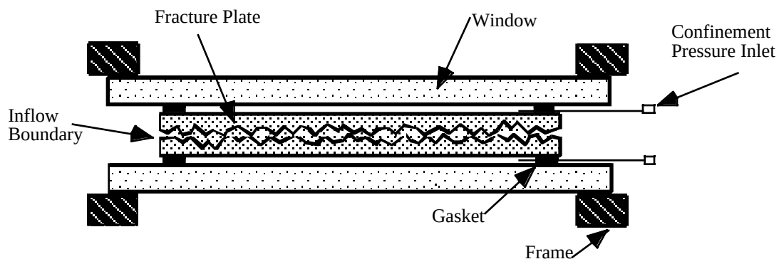
b) Micro-model/Fracture system, Cross-section
