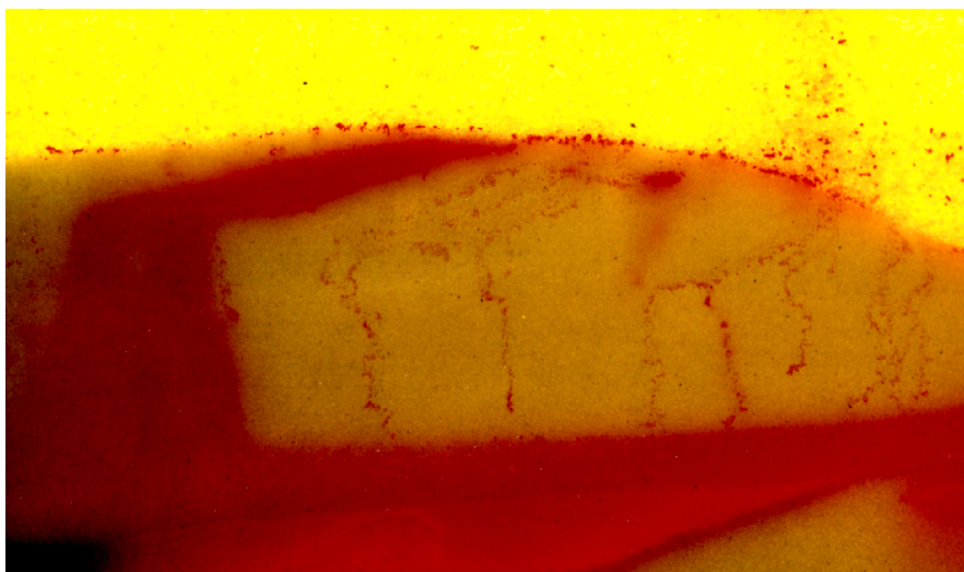
Figure 10. Enlarged photograph of mobilized TCE penetration into the fine sand aquitard during the MA surfactant flood. This photo shows the extreme lower left portion of the chamber and the pervasive penetration of the aquitard with mobilized TCE after 13.6 pore volumes of surfactant flooding. (Conrad et al., in review)
