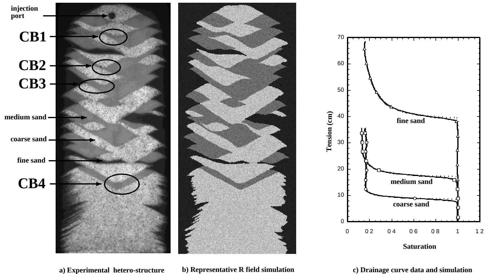
Figure 3. Digital image of the 60 cm tall macro- heterogeneous sand pack, simulation of R field and unit drainage curves: a) Digital image of the heterogeneous sand pack used in the invasion experiments. In this image the coarse sand transmits the most light and hence is the lightest; the medium sand appears gray; and the fine sand appears dark. The injection port and four major capillary barriers (labeled CB1 through CB4) are identified. These capillary barriers occur where medium sand separates coarse sand units. b) Representative R field simulation using unit locations and CDFs built from drainage curves measured on each unit. c) Comparison of measured and simulated drainage curves for each unit (solid lines designate data and dashed simulations). From Glass et al. (2000, 2001).
