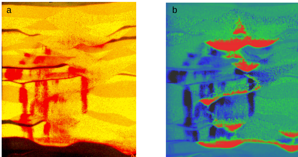
Figure 9. Extent of TCE mobilization after introduction of 2.6 pore volumes of MA surfactant solution (a) photograph showing red-dyed TCE, and (b) processed digital image where red denotes regions where TCE has been mobilized from and black and blue denotes regions where TCE has mobilized to. In the digital image, the red color shows the initial configuration of the TCE in a series of pools. Notice that all the pools have completely drained. Underexposure of the fine sand aquitard at the beneath the lowermost pool prevents us from seeing the extent of migration into the aquitard on these images. Chamber size is 60x60 cm. (Conrad et al., in review)
