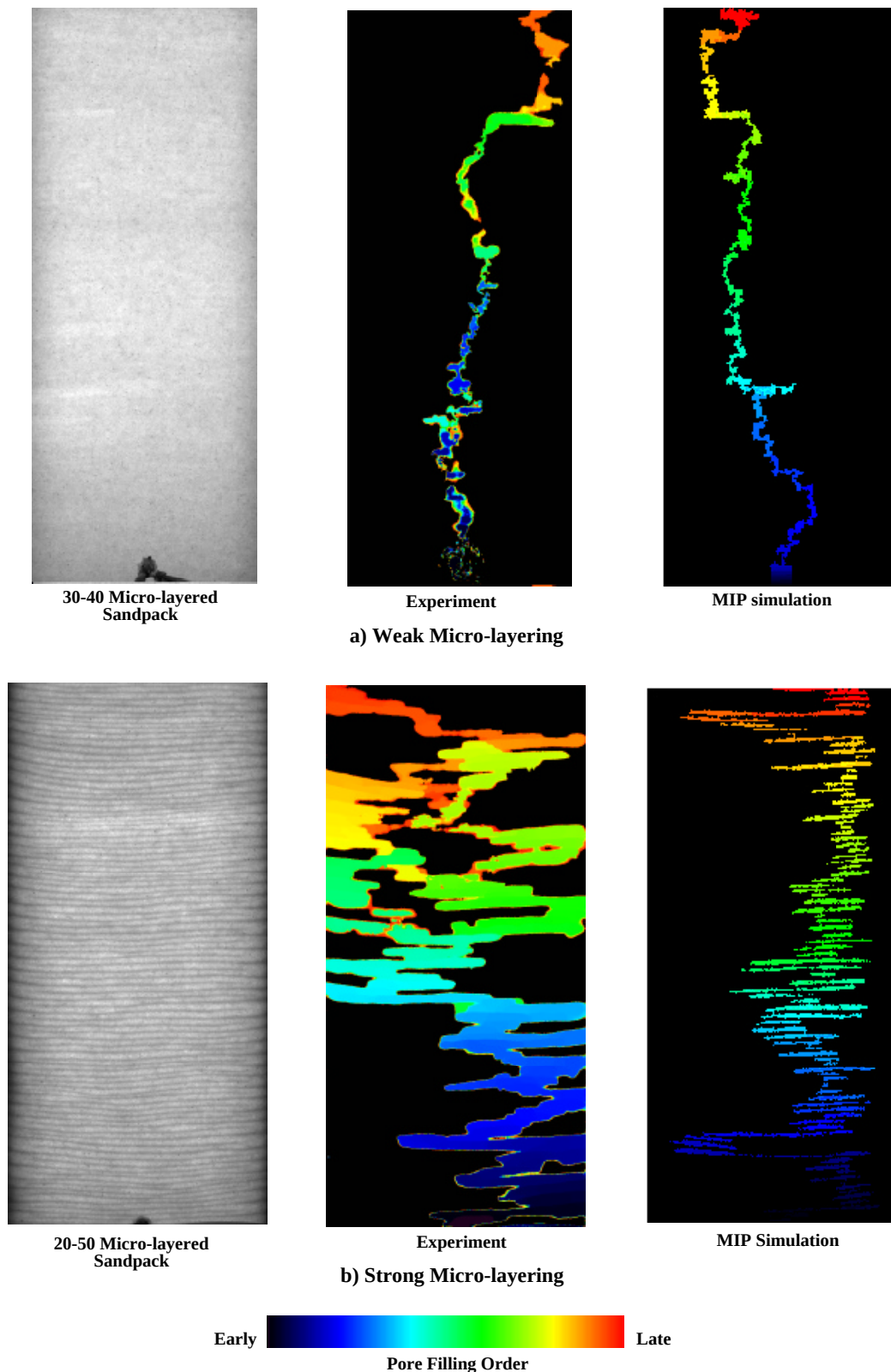
Figure 7. Influence of Micro-layering on nonwetting phase migration: Preliminary experiments and MIP simulations were conducted in microlayered sands 60 cm tall with a) weak and b) strong intensities. Colors represent first arrival filling order integrated across the thickness of the chamber or simulation network. Light refraction at the micro-layers and image reduction methods to yield first arrival blurr the experimental images somewhat. MIP images look closer to what one can see in the experiment and reflect the pore scale detail seen in the experiments extremely well. Also note that strong multiple pathways have formed in the strong micro-layer experiment due to gravity-capillary pulsation.
