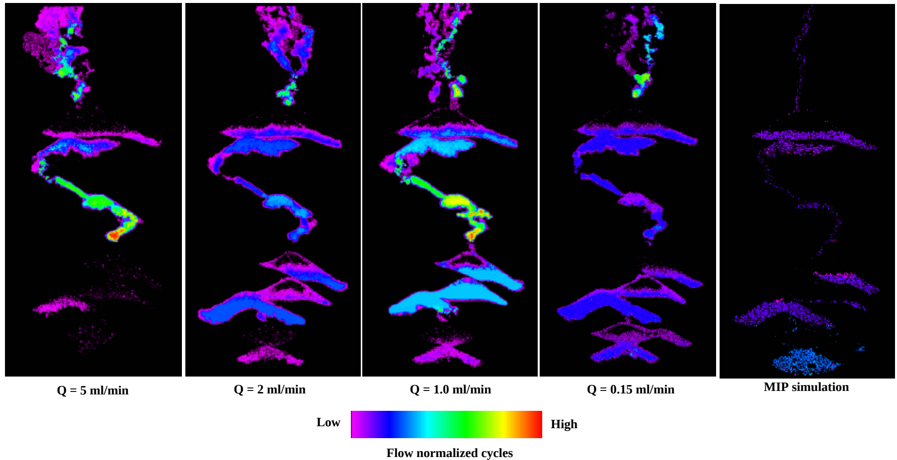
Figure 6. Capillary-gravity pulsation and suppression by viscous forces. The macro heterogeneous structure seen in figures 3 through 5 has been inverted and CO 2 injected from below. After system breakthrough, images were gathered in time and pulsation cycles were counted as a function of location within the system. Flow rate normalized cycles is seen to vary within the flow structure as a function of flow rate. At 5 ml/minute, pulsation has been largely suppressed in the lower 1/3 of the cell. A MIP simulation with simultaneous wetting and nonwetting invasion neglecting viscous forces is shown at the right to yield very similar behavior as we see experimentally at low flow. Note however, we see higher pulsation near the source than in the experiment and also, we do not find the generation of multiple pathways below the final capillary barrier in the model as we see in the experiment.
