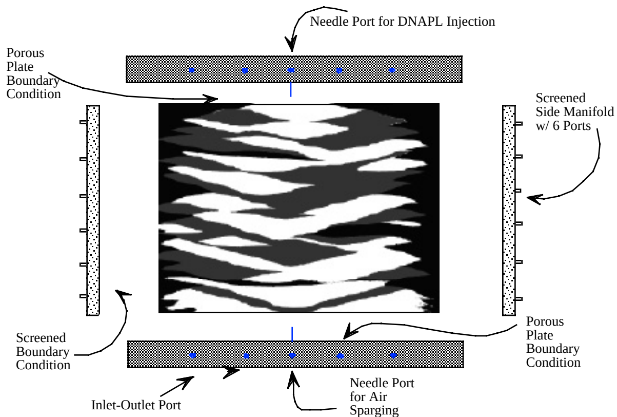
a) Heterogeneous Sand Pack System, Plan View
