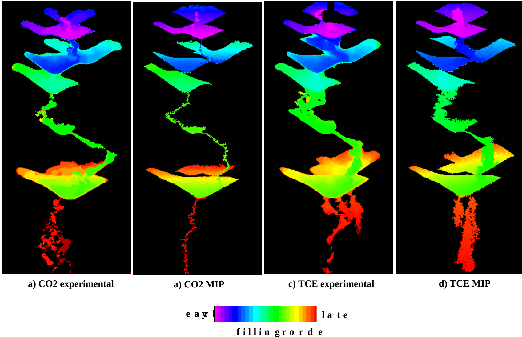
Figure 4. Invasion order images for experiments and MIP simulations: a) CO2 experiment, b) CO2 MIP simulation with no viscous forces, c) TCE experiment, d) TCE MIP simulation with viscous forces included. Colors represent first arrival filling order integrated across the thickness of the chamber or simulation network. CO2 experiments were conducted with chamber inverted (gas moving upward). Note that light refraction at the edges of the units and image reduction methods to yield first arrival blur the experimental images somewhat. MIP images look closer to what one can see in the experiment and reflect the pore scale detail very well. From Glass et al. (2000, 2001).
