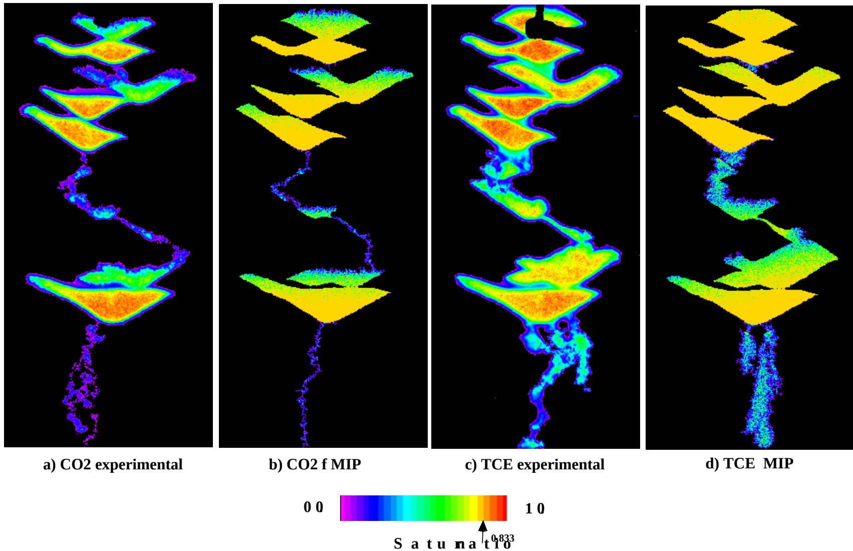
Figure 5. 2D saturation fields at system breakthrough: a) CO2 experiment, b) CO2 MIP simulation with no viscous forces, c) TCE experiment, d) TCE MIP simulation with viscous forces included. Colors represent non-wetting saturation averaged across the thickness of the chamber or simulation network, saturation of the non-wetting phase when the wetting phase is at residual (0.833) is noted on the color bar. Total volume of invaded fluid in MIP simulation matches experimental values for both CO2 and TCE of 51 and 73 ml, respectively. From Glass et al. (2000, 2001).
