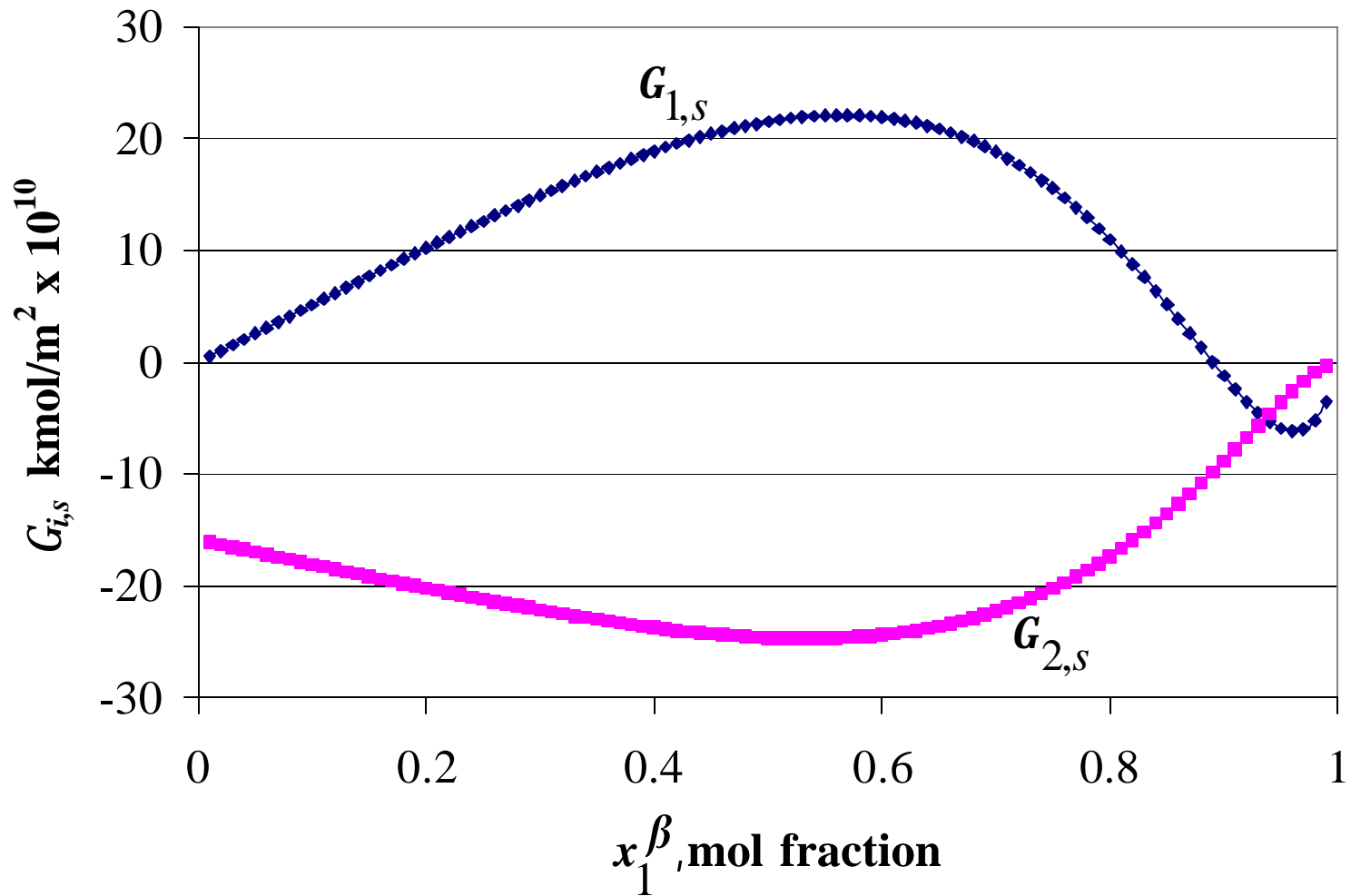
Fig. 4 – Adsorption at the Gas-Liquid Interface for Propane (1) and Normal Octane (2) Mixture vs. Mol Fraction of Propane in Liquid Phase: T = 369.8 K.
