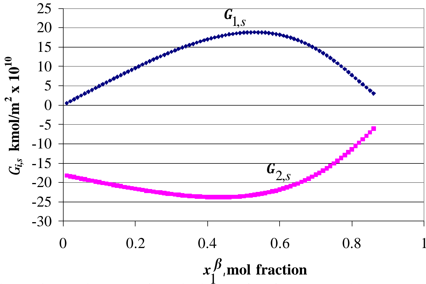
Fig. 5 – Adsorption at the Gas-Liquid Interface for Propane (1) and Normal Octane (2) Mixture vs. Mol Fraction of Propane in Liquid Phase: T = 400 K.
