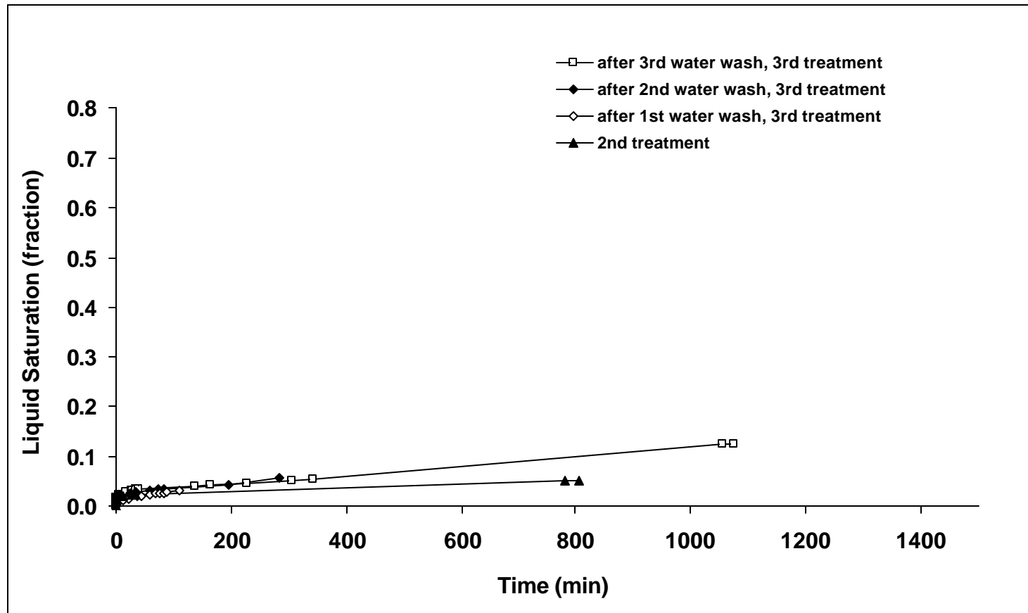
Fig. 13 - Spontaneous water imbibition at room temperature in MB19 treated with 1% and 2% EGC-1700 at room temperature.
