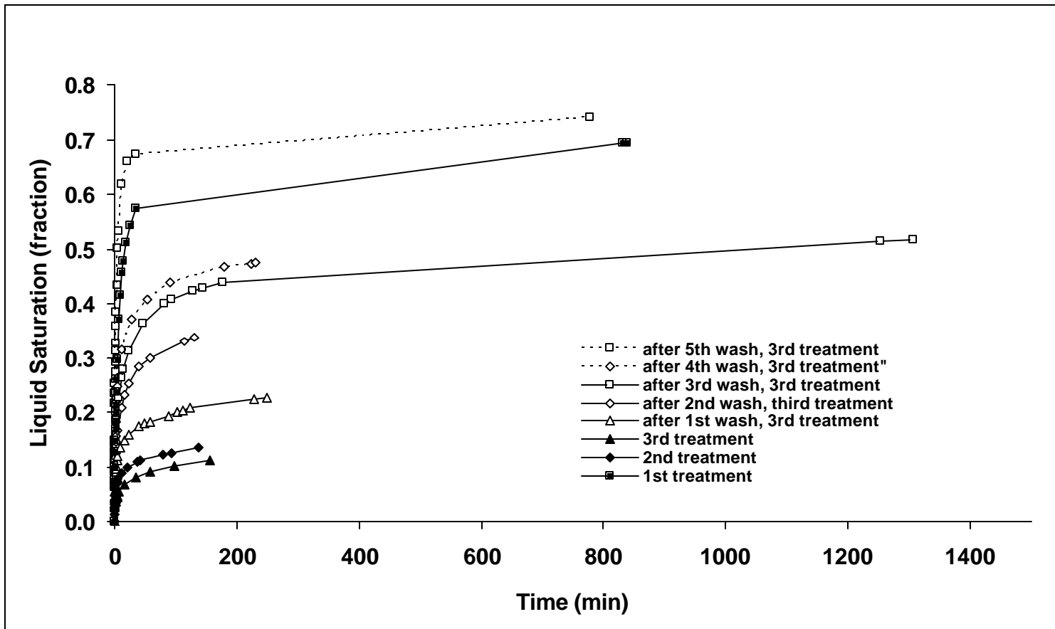
Fig. 22 - Spontaneous decane imbibition at room temperature in MB15 treated with 0.4% FC722 at room temperature.
