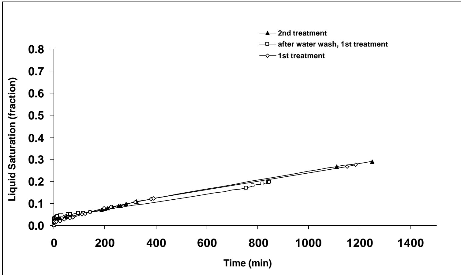
Fig. 8 - Spontaneous water imbibition at room temperature in MB21 treated with 8% L-chemical at 140°C.
