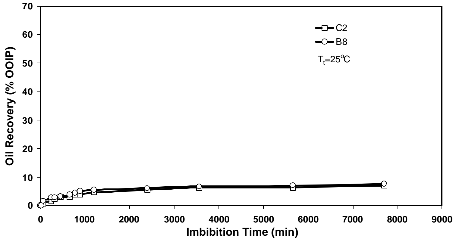
Fig.8b Oil Recovery by Spontaneous Water Imbibition for the Cores Treated with 8% FC-759
