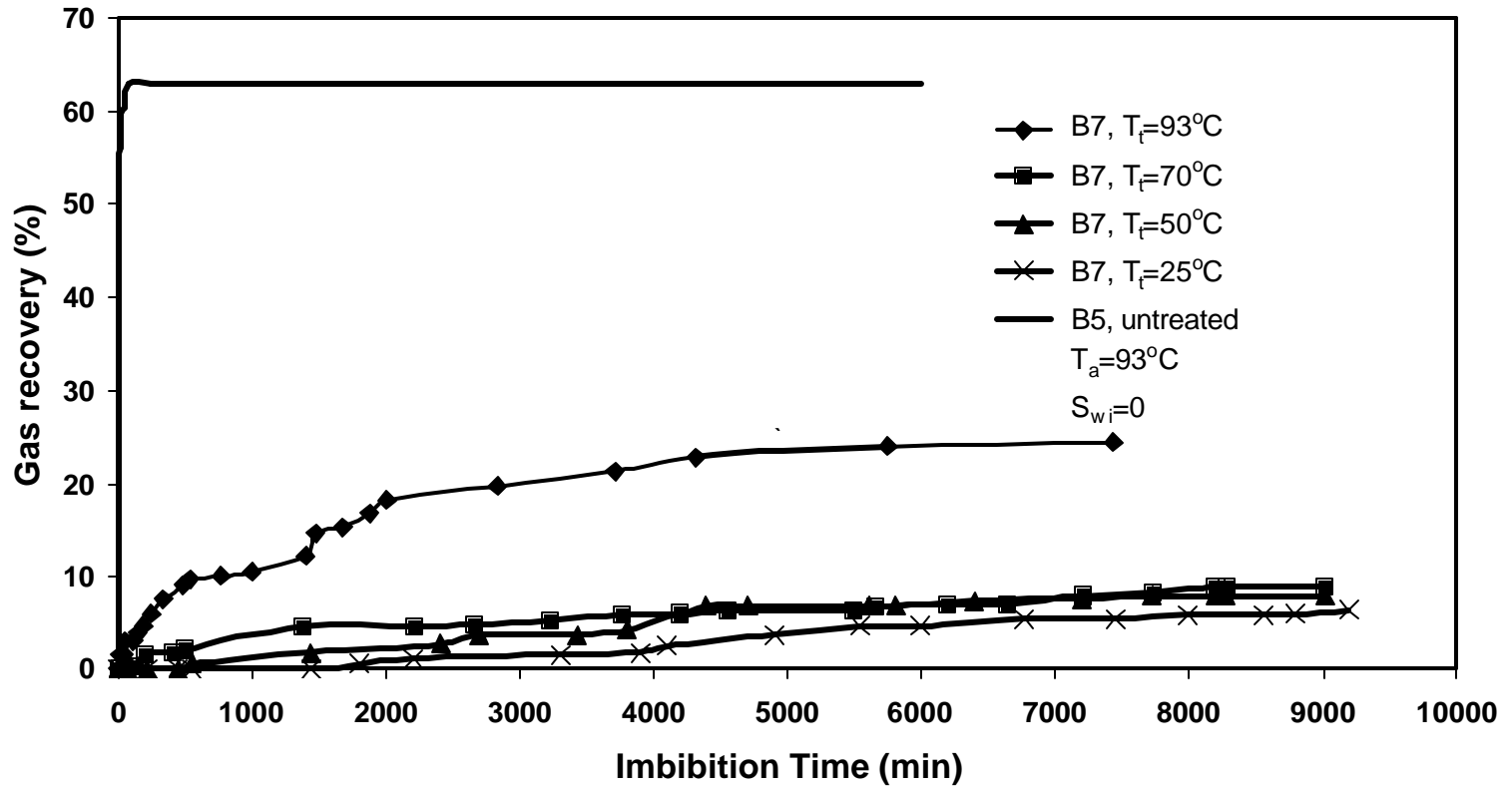
Fig.6d Effect of Temperature on Spontaneous Oil Imbibition for Berea Sample Treated With 10% FC-759
