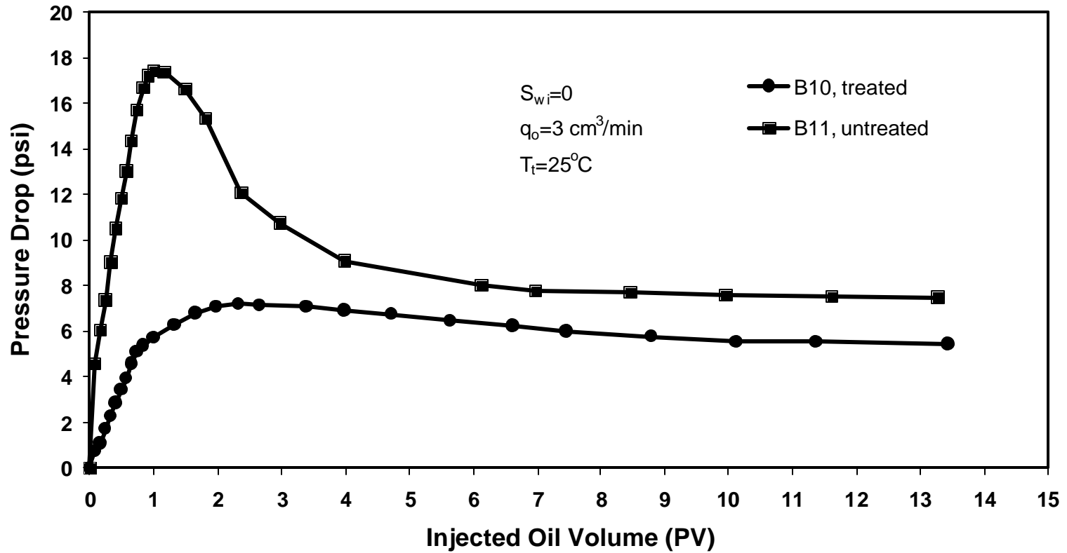
Fig. 9b. Effect of Wettability Alteration on Pressure Drop for Oil Injection in Gas Saturated Berea
