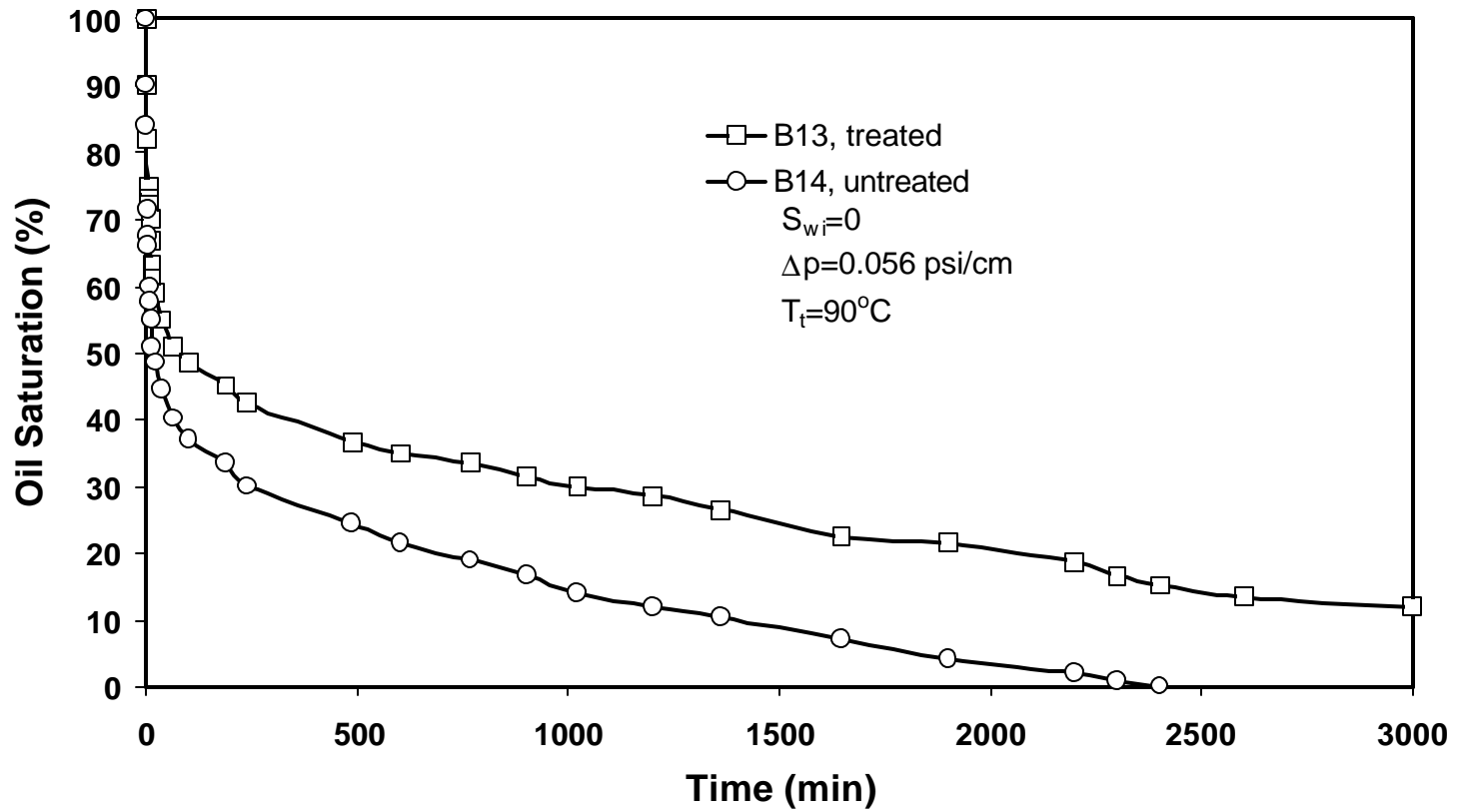
Fig.12b Effect of Wettability on Reduction of Oil Saturation by Dry Gas Injection at High Temperature
