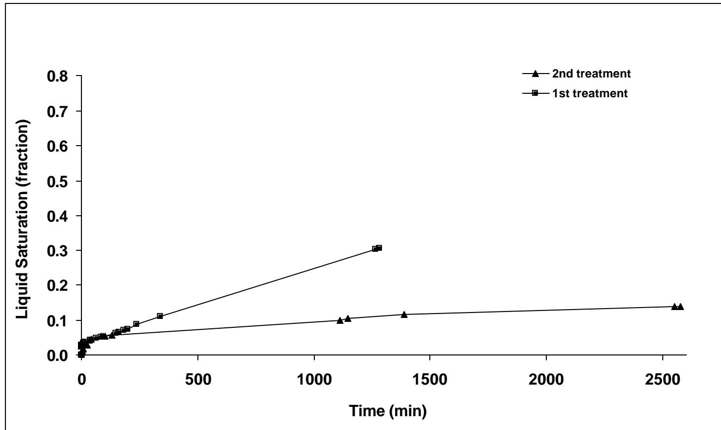
Fig. 9 - Spontaneous water imbibition at room temperature in MB23 treated with 1% EGC-1700 at 90°C.
