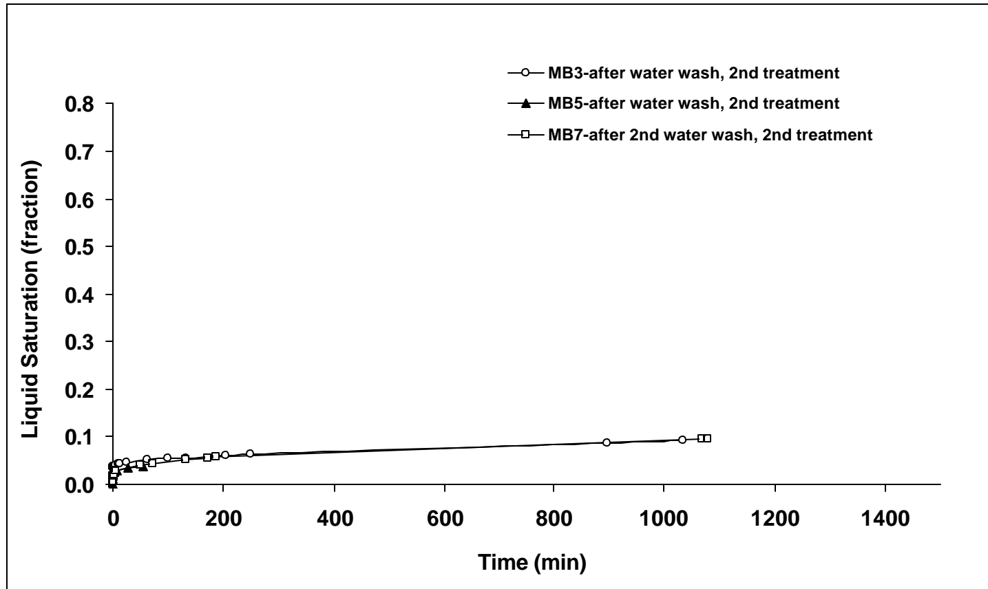
Fig. 11 - Spontaneous water imbibition at room temperature in MB3 and MB5 treated with 8% D- and B- chemicals and MB7 treated with 0.4% FC722 at room temperature.
