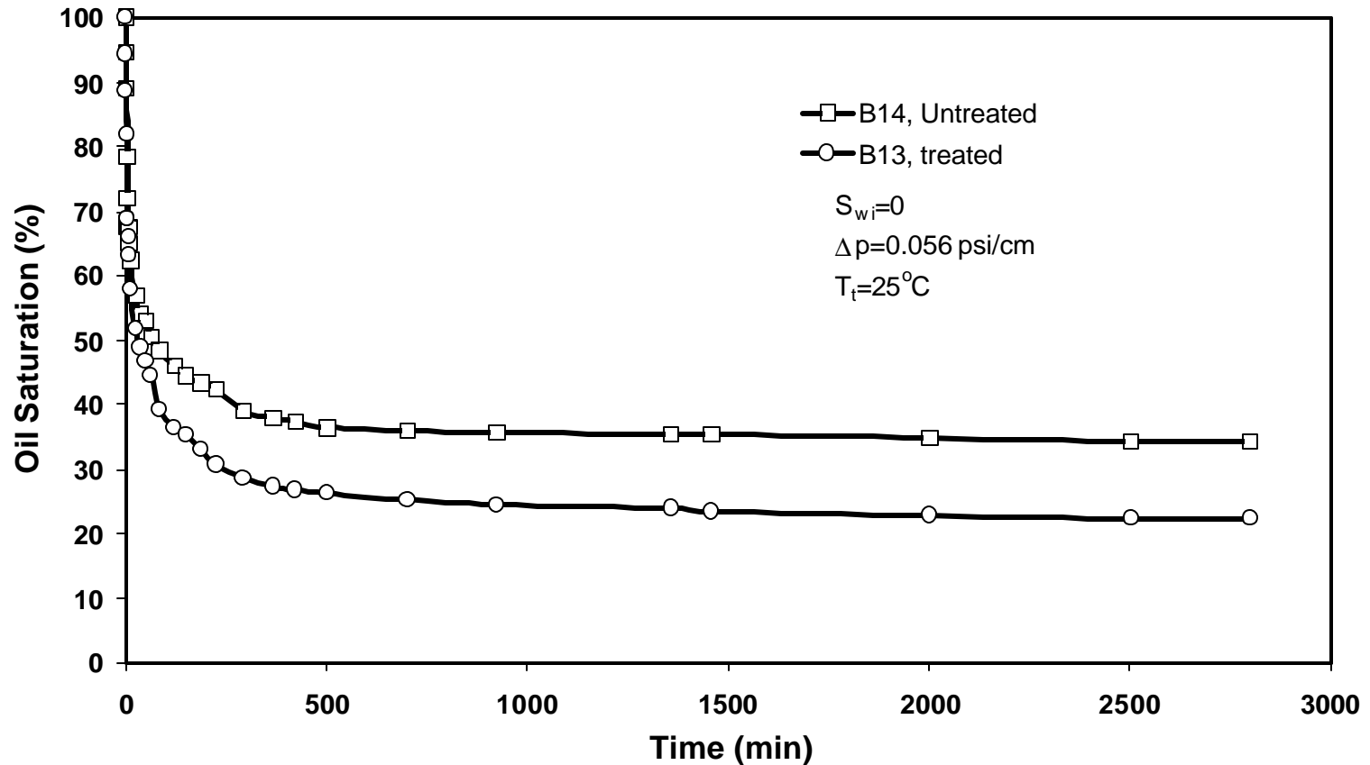
Fig.12a Effect of Wettability on Reduction of Oil Saturation by Dry Gas Injection at Room Temperature
