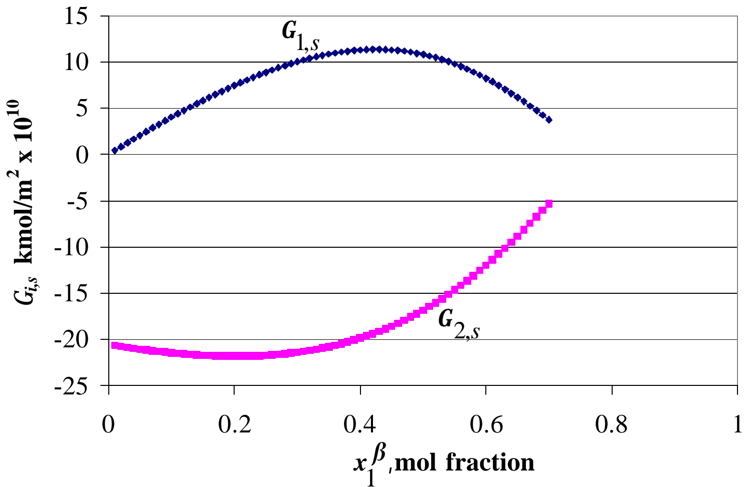
Fig. 6 – Adsorption at the Gas-Liquid Interface for Propane (1) and Normal Octane (2) Mixture vs. Mol Fraction of Propane in Liquid Phase: T = 450 K.
