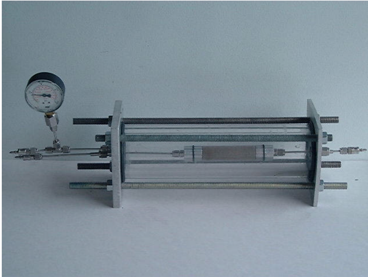
Fig. 2 - Visual core holder used for room temperature treatment, permeability measurements and fluid injection tests.
