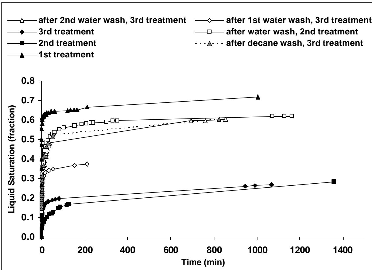
Fig. 15 - Spontaneous decane imbibition at room temperature in MB1 treated with 8% FC-759 at 140°C.
