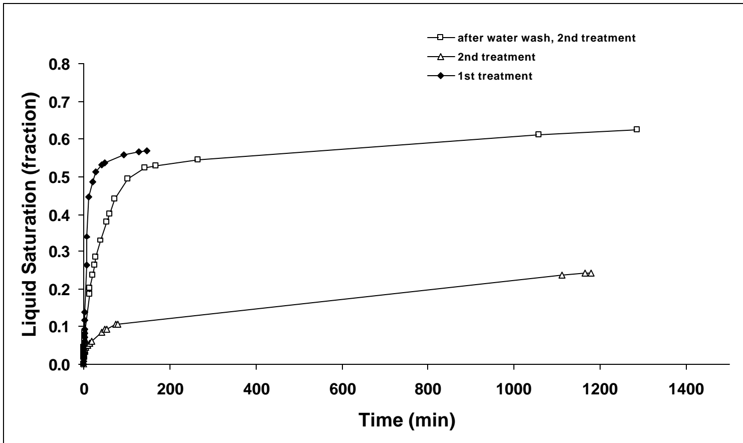
Fig. 23 - Spontaneous decane imbibition at room temperature in MB11 treated with 8% L-chemical at room temperature.
