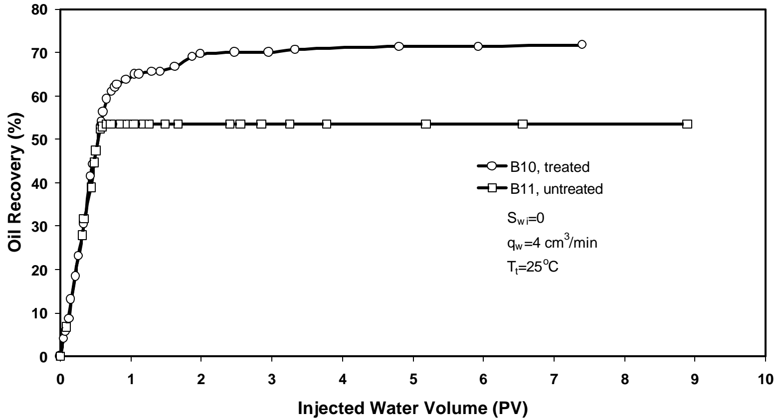
Fig.10a Effect of Wettability Alteration Oil Recovery by Water Injection
