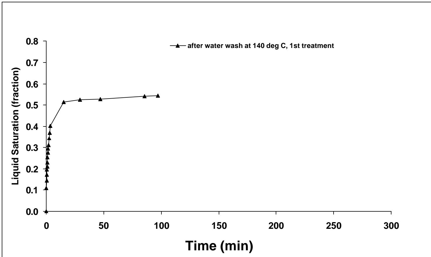
Fig. 19 - Spontaneous decane imbibition at room temperature in MB27 treated with 8% C-chemical at 140°C.
