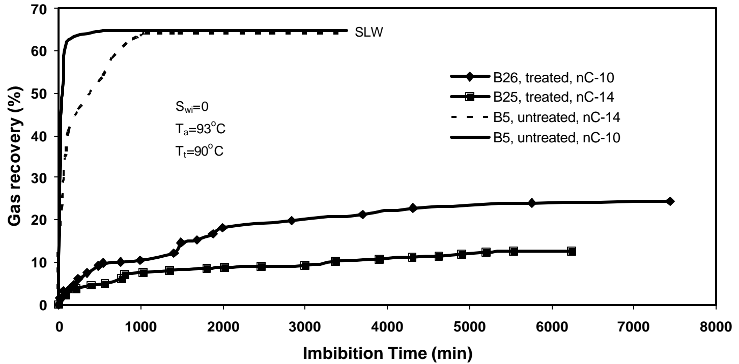
Fig.7 Spontaneous Imbibition of n\text{C}_{10} and n\text{C}_{14} for Bera Sample Treated with 10% FC-759
