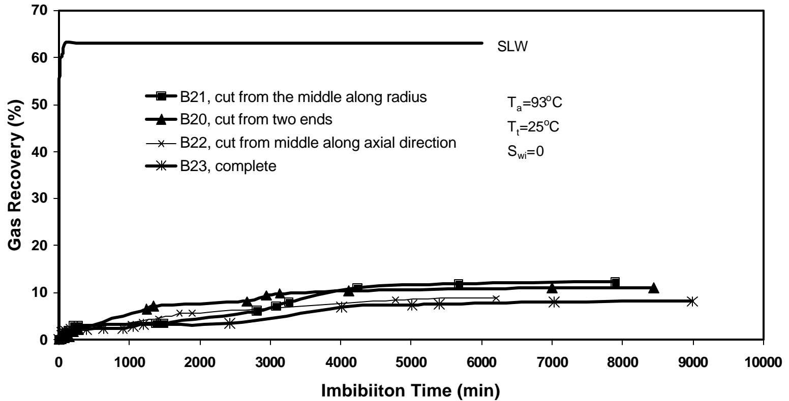
Fig. 3b Gas Recovery by Spontaneous Oil Imbibition for Cores Treated with 10% FC-759 before and after Cut
