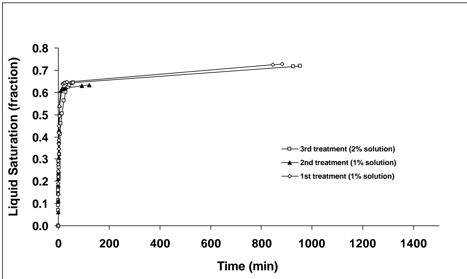
Fig. 24 - Spontaneous decane imbibition at room temperature in MB19 treated with 1% and 2% EGC-1700 at room temperature.
