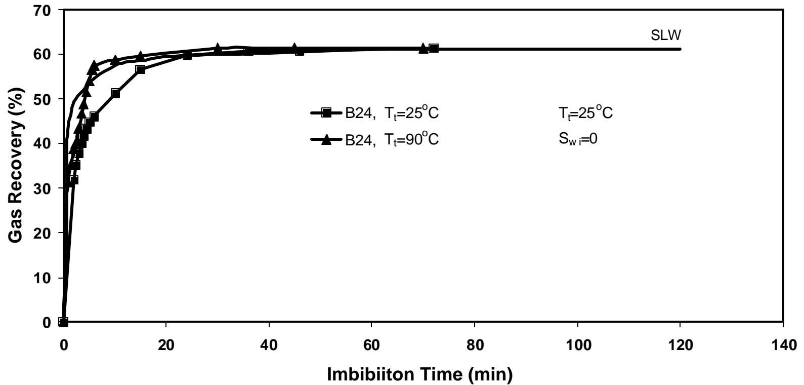
Fig. 6b Effect of Temperature on Spontaneous Oil Imbibition in Berea Treated with 1% Stearic Acid
