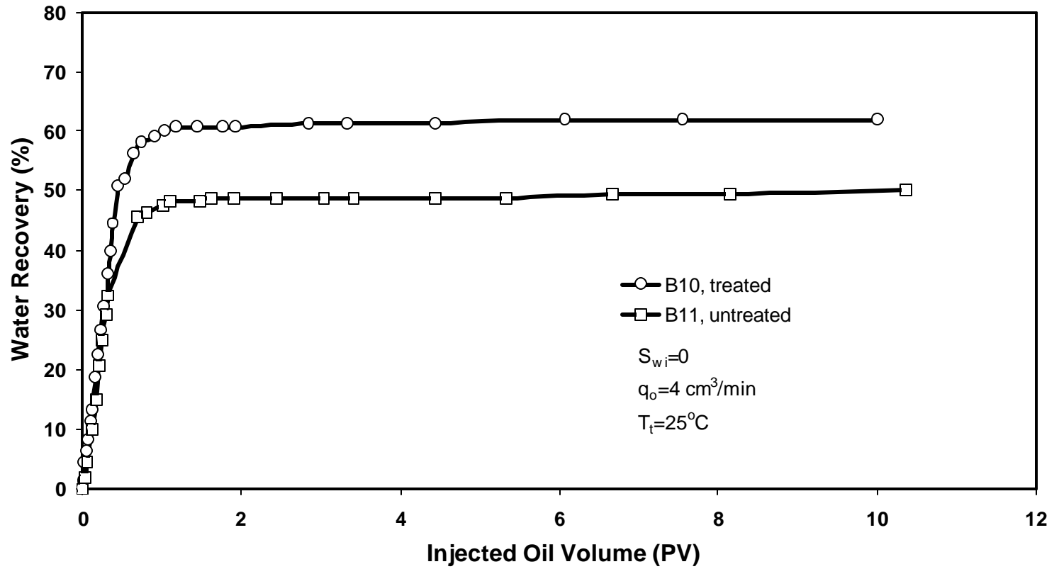
Fig.11a Effect of Wettability Alteration on Water Recovery by Oil Injection in Water Saturated Cores
