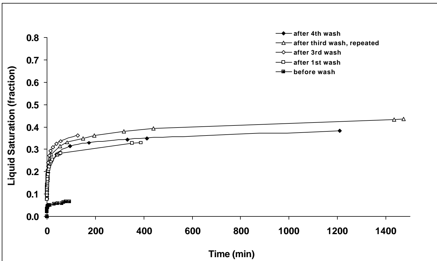
Fig. 21 - Spontaneous decane imbibition at room temperature in MB7 after the 2 nd treatment with 0.4% FC722 at room temperature.
