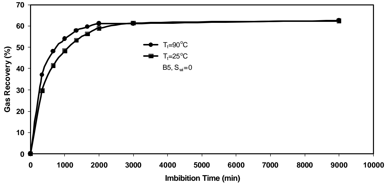
Fig.6a Effect of Temperature on Spontaneous Oil Imbibition for Untreated Berea
