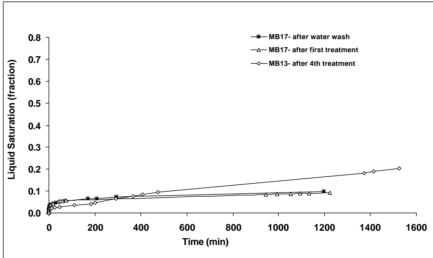
Fig. 7- Spontaneous water imbibition at room temperature in MB17 and MB13 treated with 0.4% FC722 at 140°C.
