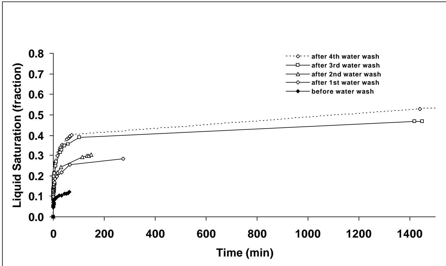
Fig. 20 - Spontaneous decane imbibition at room temperature in MB7 after the 1 st treatment with 0.4% FC-722 at room temperature.
