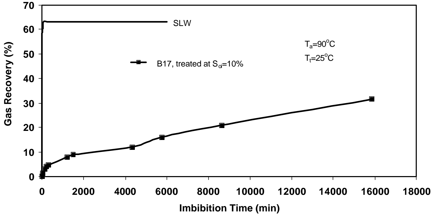
Fig.5b Effect of Initial Oil Saturation on Wettability Alteration by 10% FC-759
