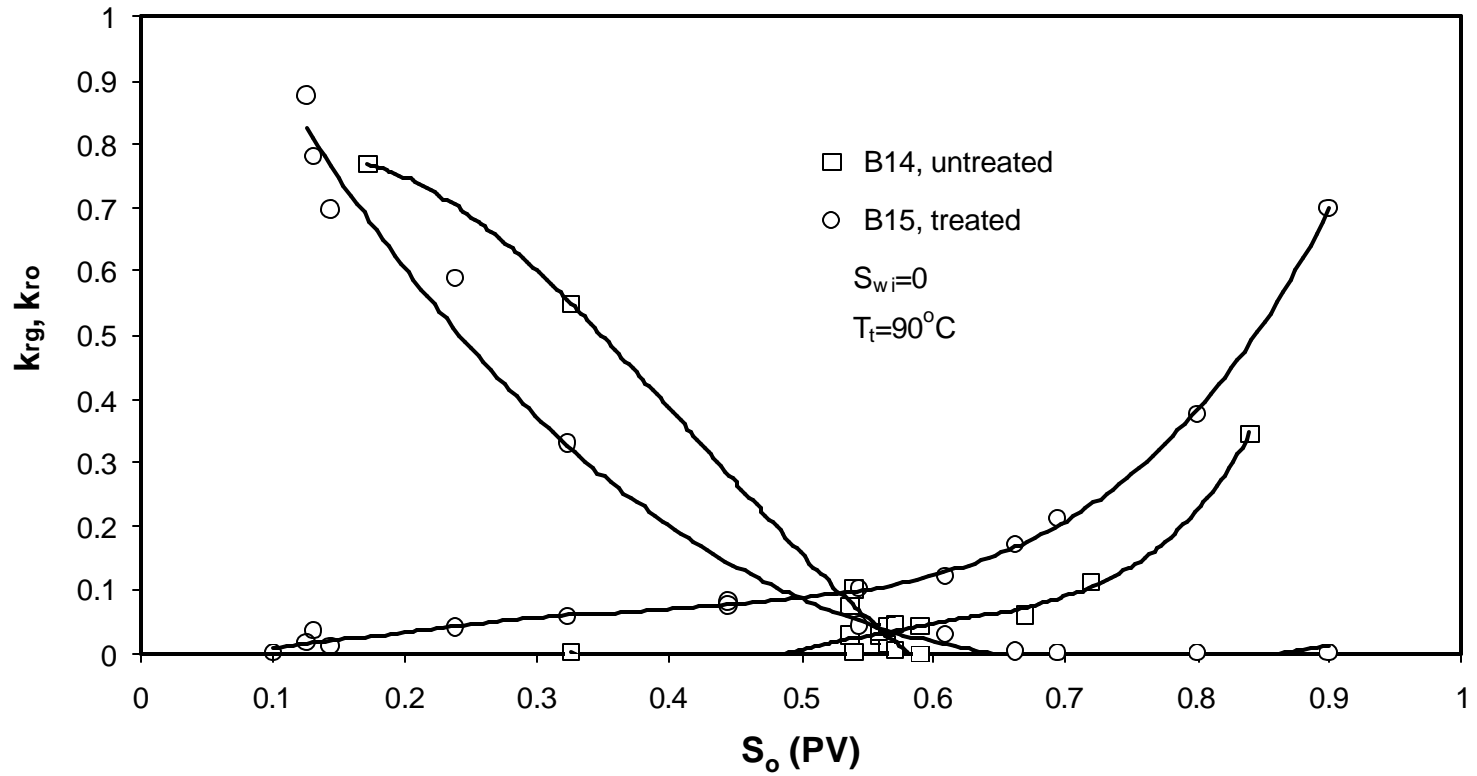
Fig.13a Gas and Oil Relative Permeabilities for Treated and Untreated Cores at T=90°C: nC-10
