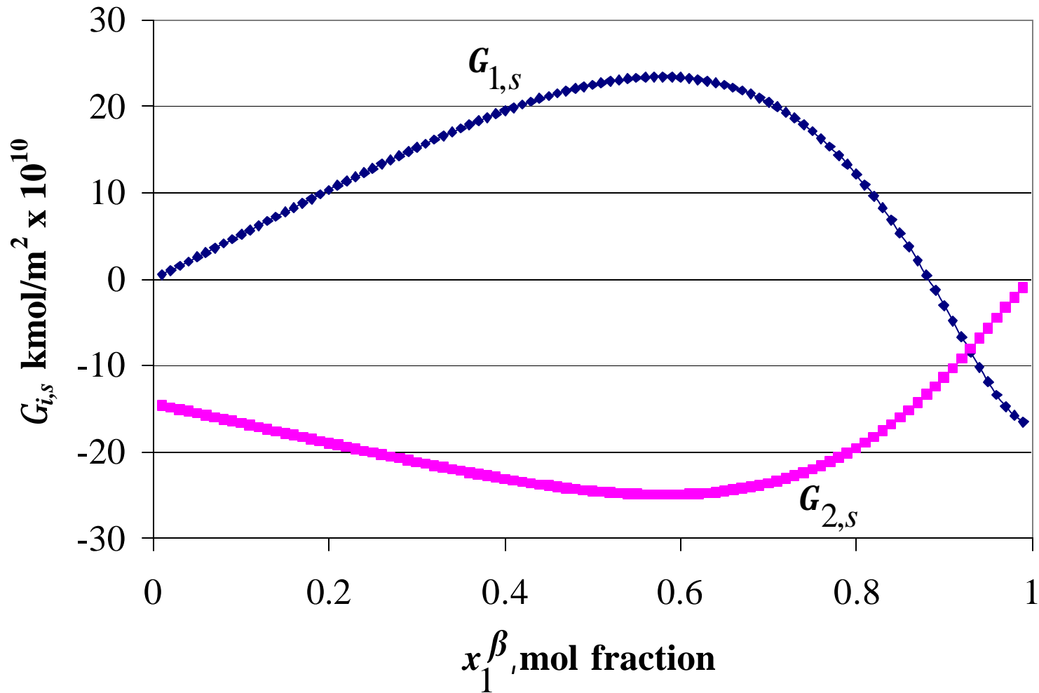
Fig. 3 – Adsorption at the Gas-Liquid Interface for Propane (1) and Normal Octane (2) Mixture vs. Mol Fraction of Propane in Liquid Phase: T = 350 K.
