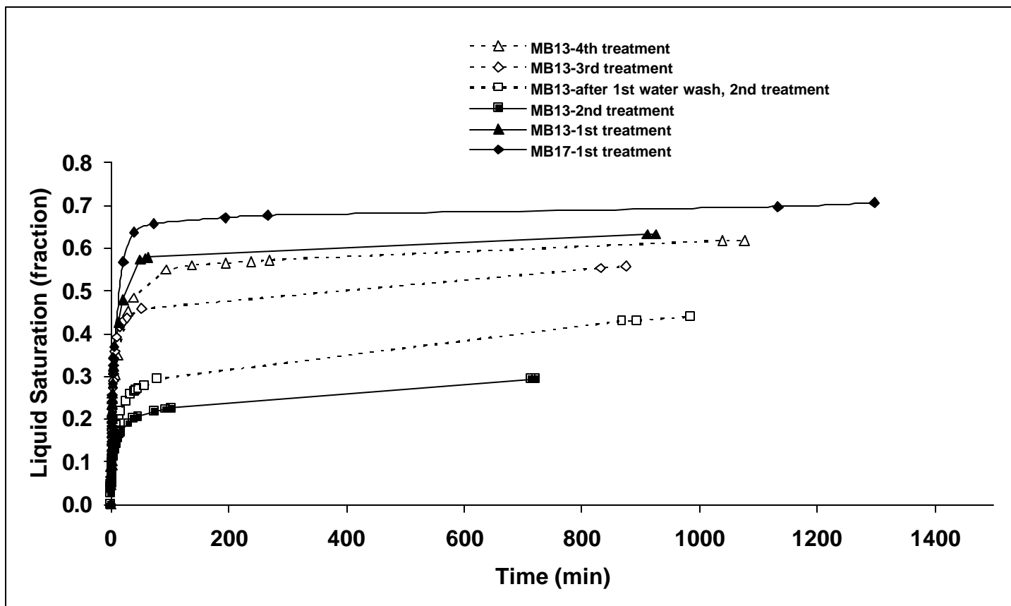
Fig. 18 - Spontaneous decane imbibition at room temperature in MB13 and MB17 treated with 0.4% FC-722 at 140°C.
