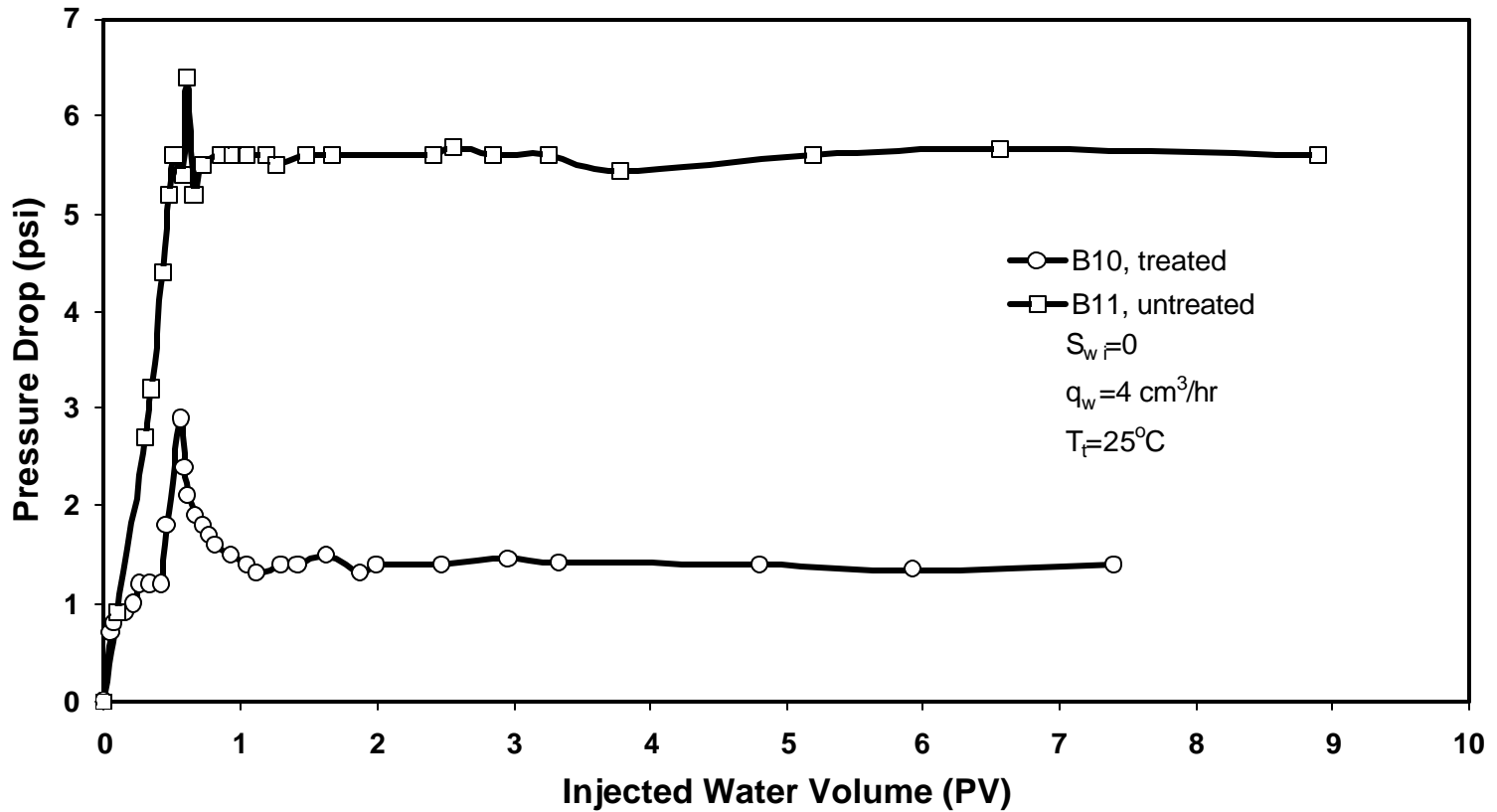
Fig.10b Effect of Wettability Alteration on Pressure Drop for Water Injection in Oil Saturated Cores
