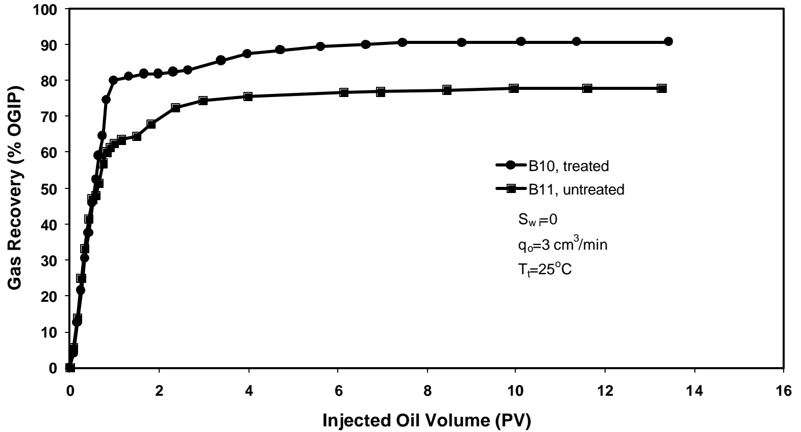
Fig.9a Effect of Wettability Alteration on Gas Recovery by Oil Injection.
