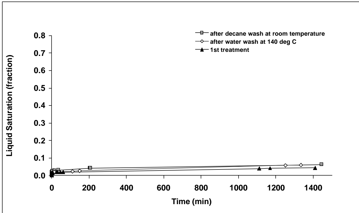
Fig. 10 - Spontaneous water imbibition at room temperature in MB27 treated once with 8% C-chemical at 140°C.
