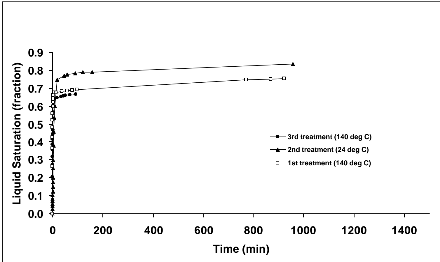
Fig. 16 - Spontaneous decane imbibition at room temperature in MB3 treated with 8% D-chemical at 140°C and at room temperature.
