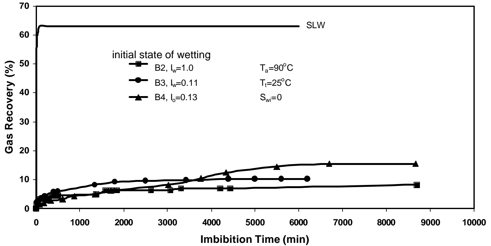
Fig.4 Effect of Initial Wettability on Wettability Alteration by 8% FC-759
