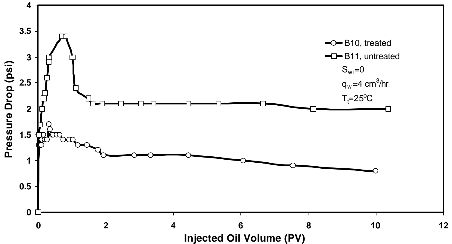
Fig.11b Effect of Wettability Alteration on Pressure Drop for Oil Injection in Water Saturated Cores
