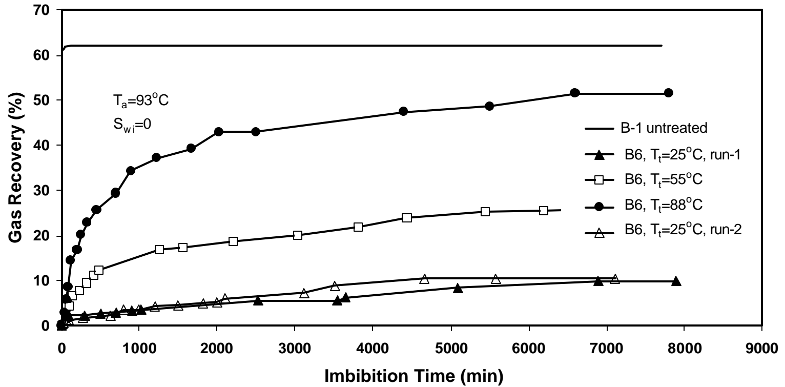
Fig.6c Effect of Temperature on Spontaneous Oil Imbibition for Berea Samples Treated with 2% FC-722.
