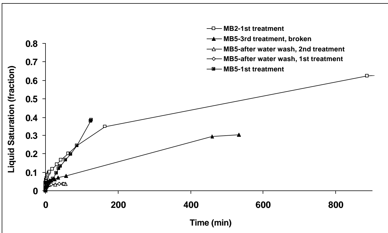
Fig. 6 - Spontaneous water imbibition at room temperature in MB2 and MB5 treated with 8% A-chemical and 8% B-chemical, respectively, at 140°C (2 nd treatment with B-chemical was at room temperature).
