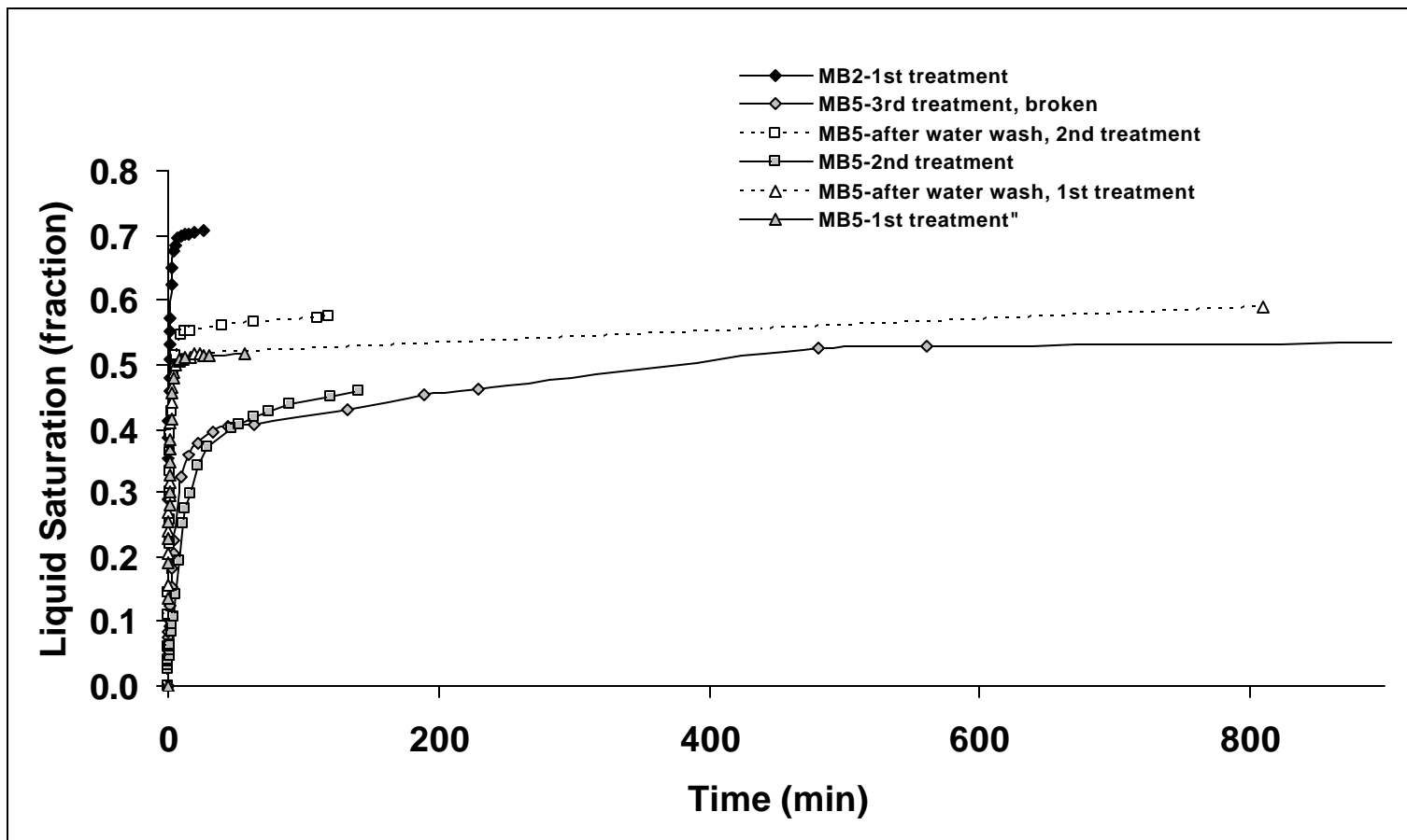
Fig. 17 - Spontaneous decane imbibition at room temperature in MB2 and MB5 treated with 8% A-chemical and 8% B-chemical, respectively, at 140°C (2 nd treatment with B-chemical was at room temperature)
