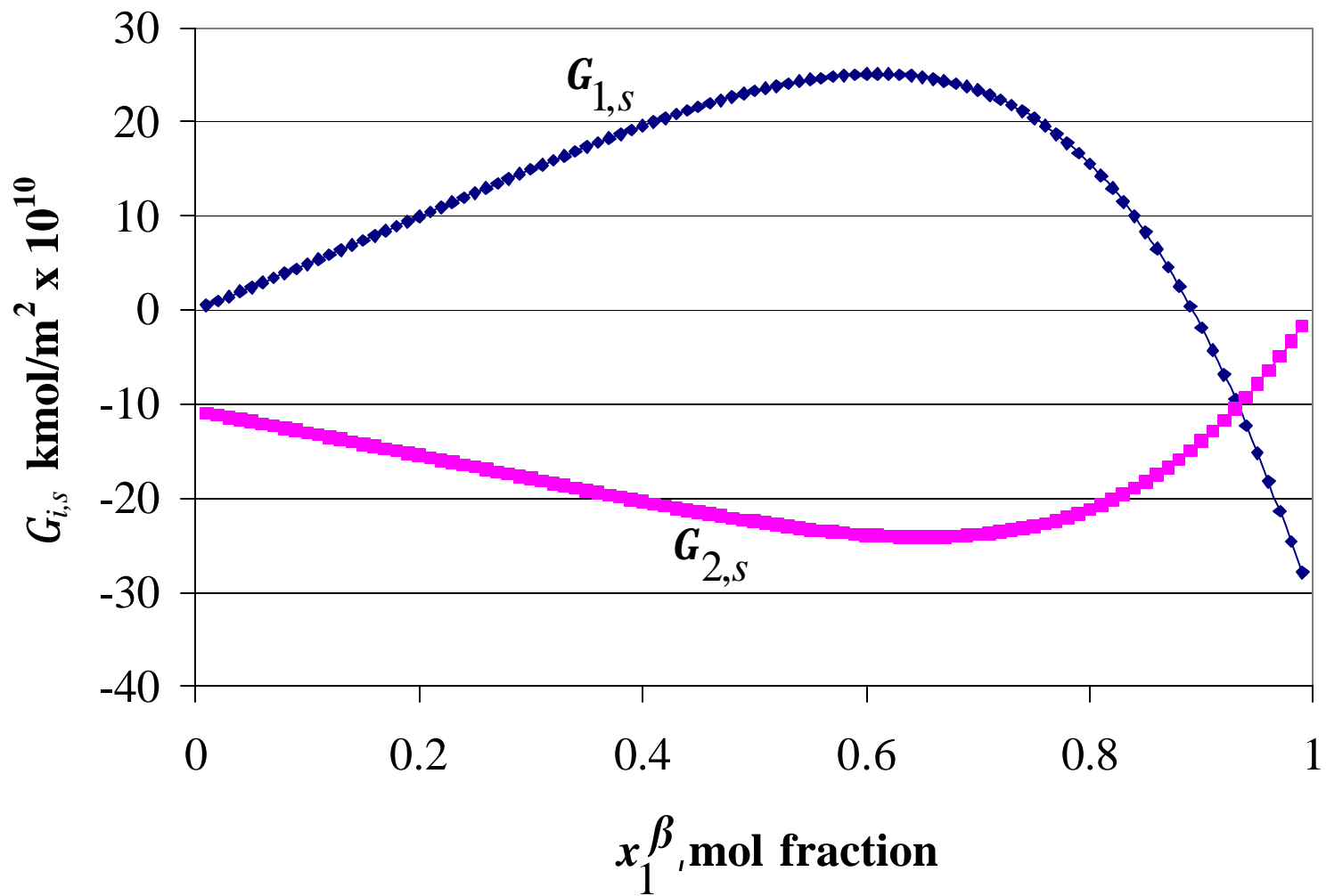
Fig. 2 – Adsorption at the Gas-Liquid Interface for Propane (1) and Normal Octane (2) Mixture vs. Mol Fraction of Propane in Liquid Phase: T = 300 K.
