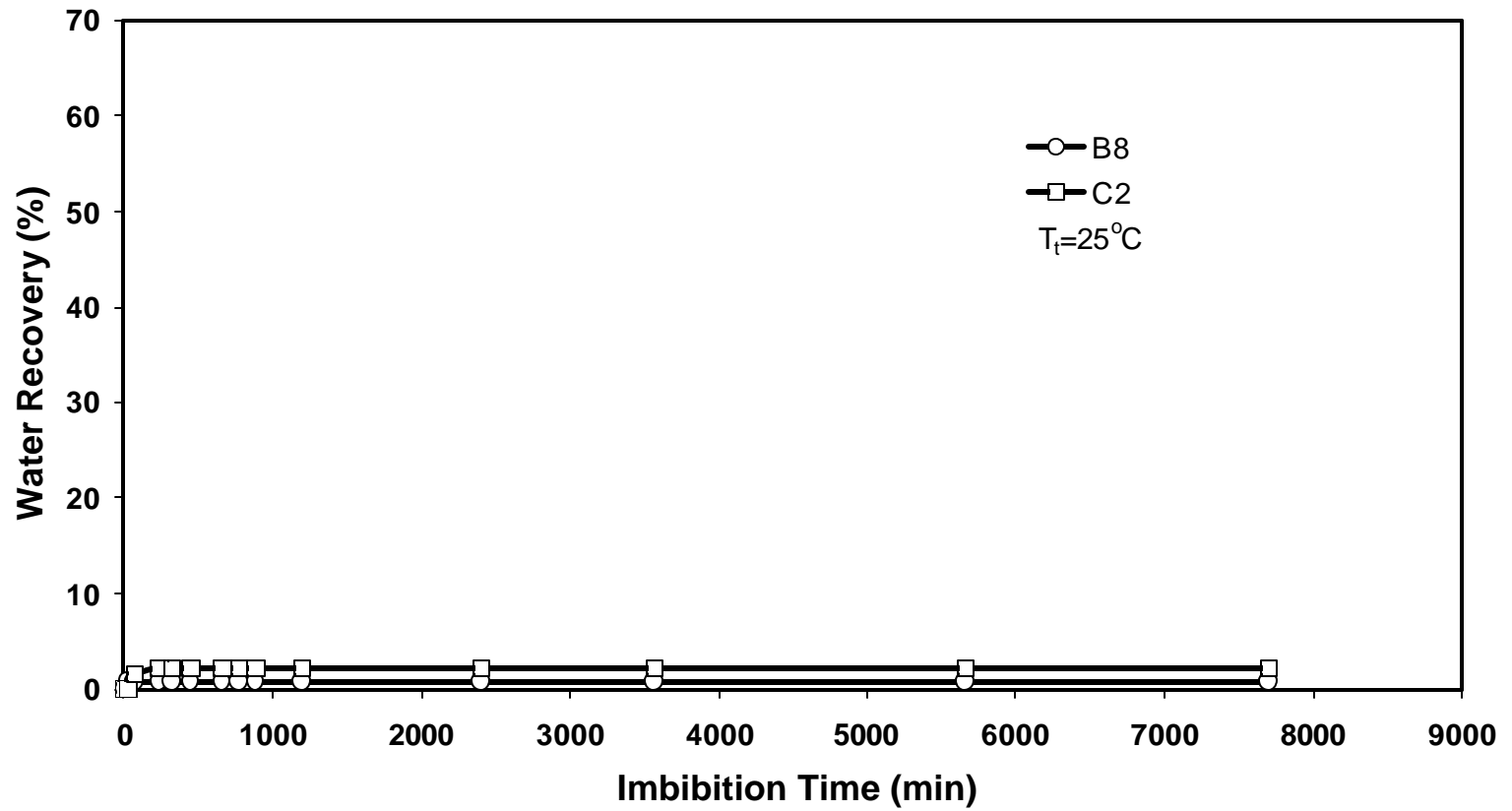
Fig.8a Water Recovery by Spontaneous Oil Imbibition for the Cores Treated with 8% FC-759
