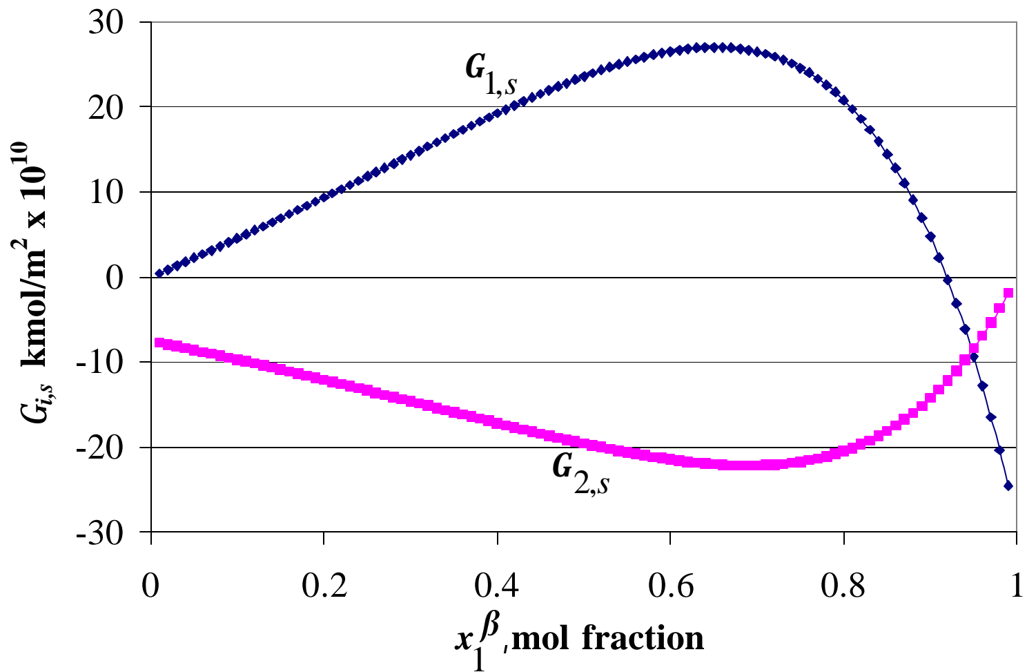
Fig. 1 – Adsorption at the Gas-Liquid Interface for Propane (1) and Normal Octane (2) Mixture vs. Mol Fraction of Propane in Liquid Phase: T = 250 K.
