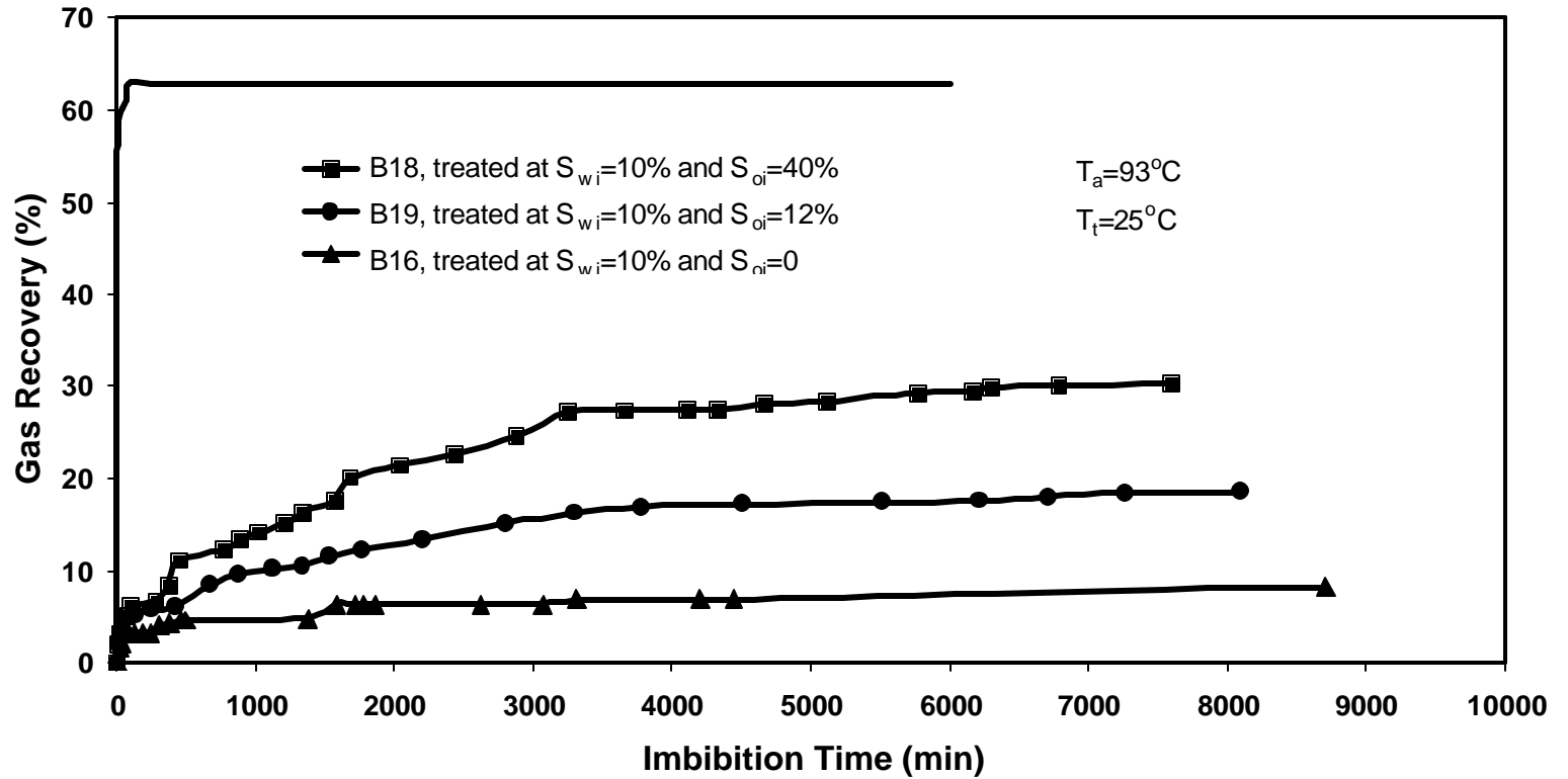
Fig.5c Effect of Initial Water and Oil Saturation on Wettability Alteration by 10% FC-759
