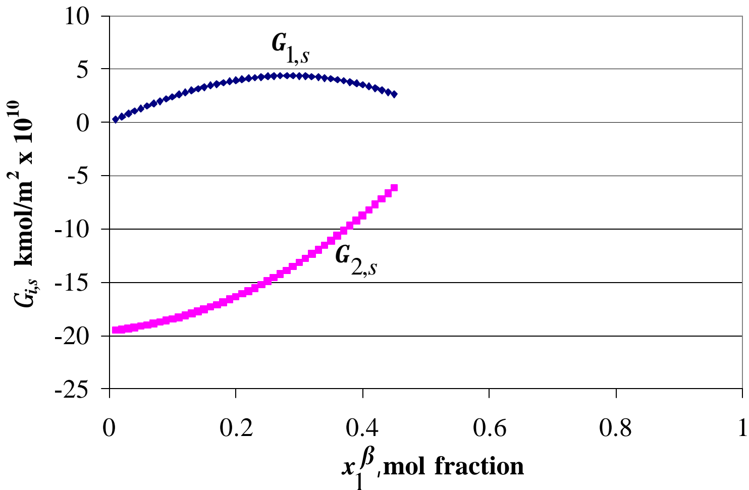
Fig. 7 – Adsorption at the Gas-Liquid Interface for Propane (1) and Normal Octane (2) Mixture vs. Mol Fraction of Propane in Liquid Phase: T = 500 K.
