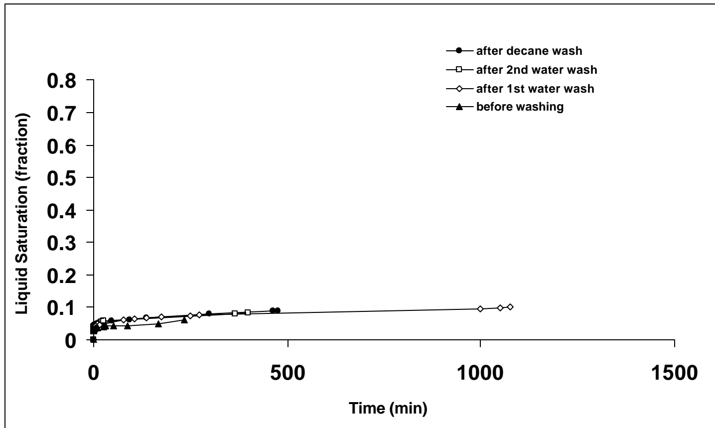
Fig. 4 - Spontaneous water imbibition at room temperature in MB1 treated with 8% FC-759 at 140°C (third treatment).
