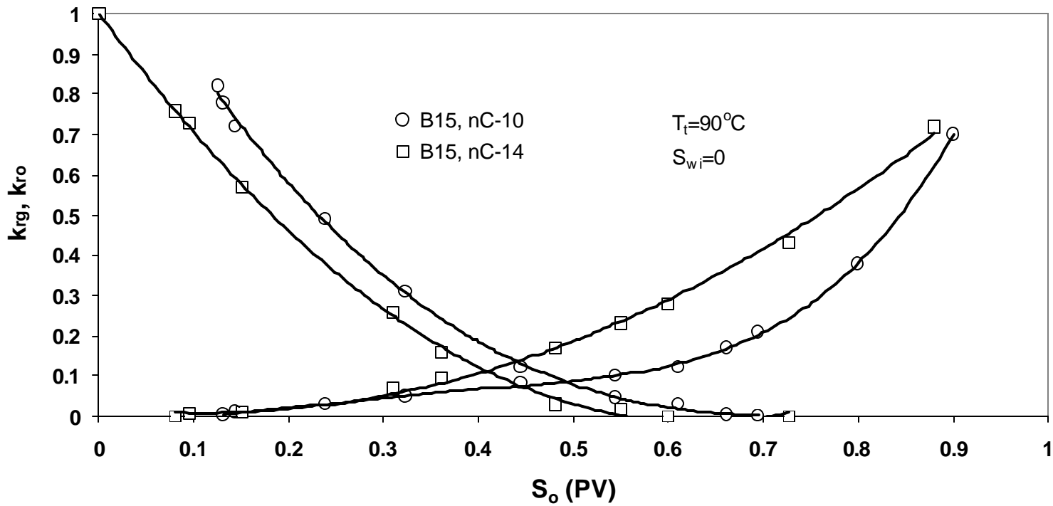
Fig.13b Gas and Oil Relative Permeabilities for Treated Berea at T=90°C for nC-10 and nC-14
