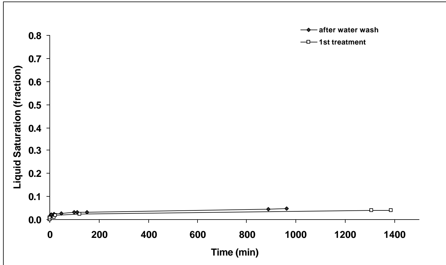
Fig. 14 - Spontaneous water imbibition at room temperature in MB25 treated with 8% C-chemical at room temperature.
