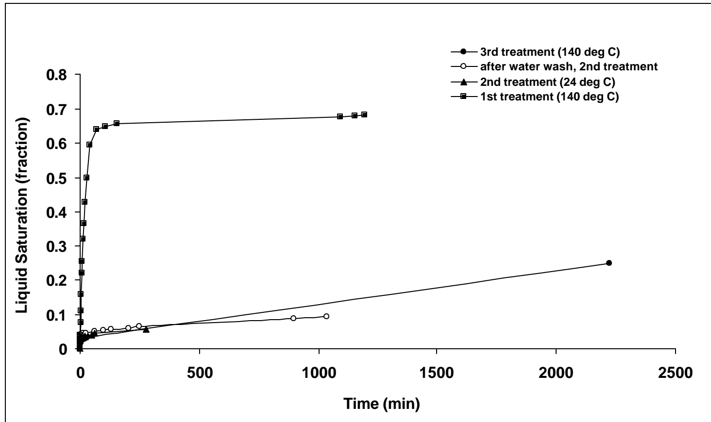
Fig. 5 - Spontaneous water imbibition at room temperature in MB3 treated with 8% D-chemical at 140°C and at room temperature.
