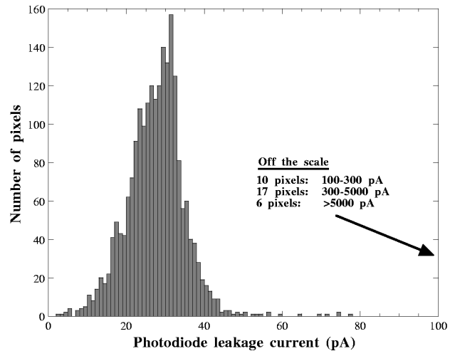
Fig. 3. Histogram of the leakage current values for pixels in 34 64-pixel arrays. Histogram bins are 1 pA wide. Photodiodes are 3 mm \times 3 mm in size and were in the dark at room temperature under a 50 V bias. The pixels with leakage current less than 100 pA (2143 out of 2176) demonstrate an average current of 28 \pm 7 pA.
