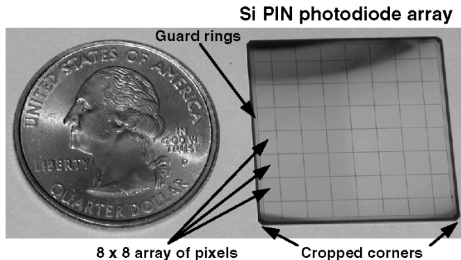
Fig. 2. Low-noise Si PIN photodiode array consisting of 64 3 mm \times 3 mm pixels, with a quarter (2.4 cm diameter) for scale. The side shown is the patterned p-layer, while the backside is the unpatterned, light-sensitive n-layer. A series of 4 guard rings encircle the array of pixels.
