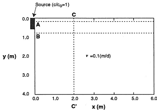
Figure 3. Schematic of the 2-D model domain for the two-dimensional radionuclide transport problem showing the velocity field and three cross sections for comparisons of the simulation results.
