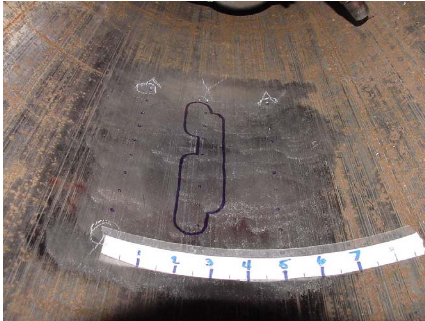
Figure 44 - Outline of Simulated Corrosion on Inside Diameter of Pipe Section
