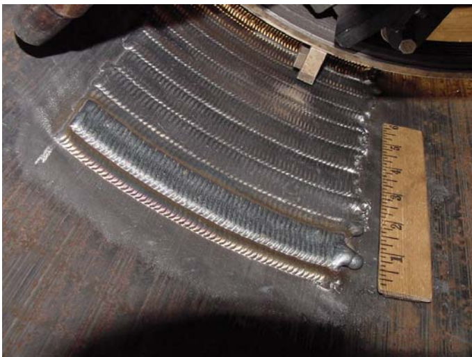
Figure 49 - First Pass of Second Layer of Deposited Weld Metal on Inside Pipe Diameter
