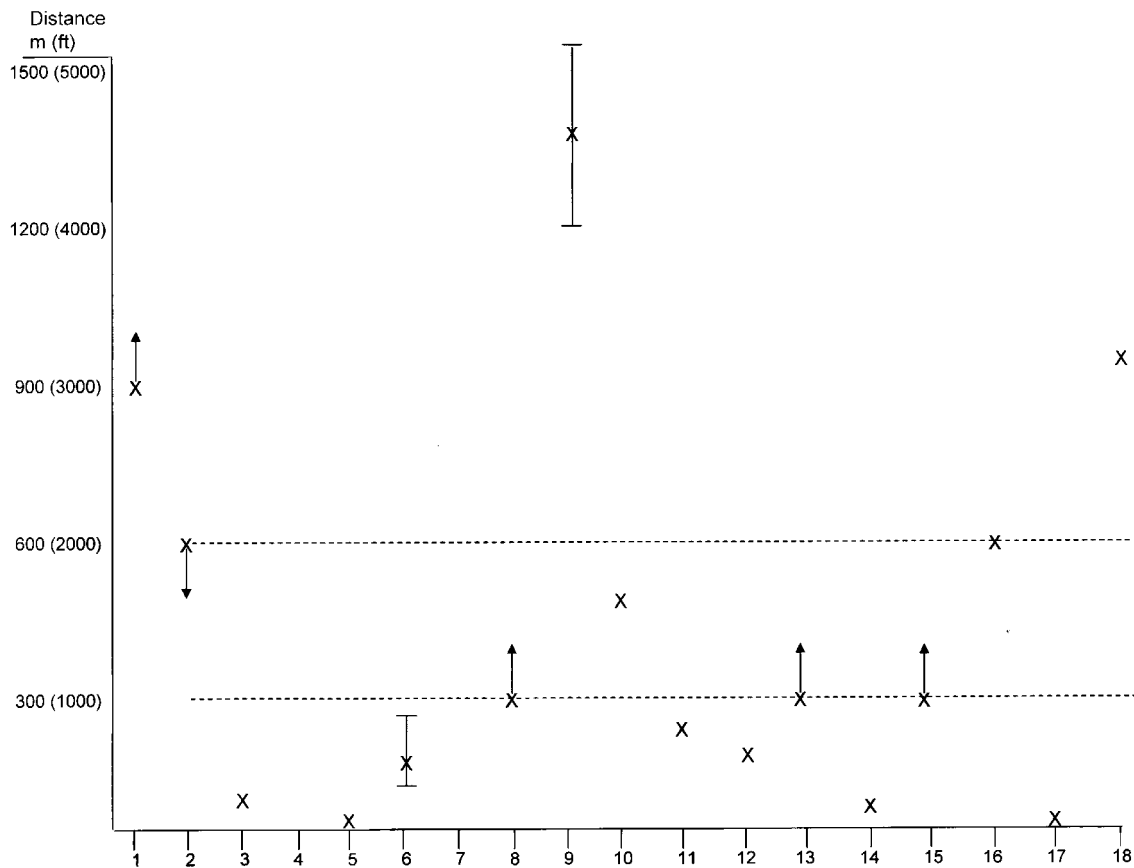
Figure 55 - Distance Repair System Required to Travel Down Pipe
