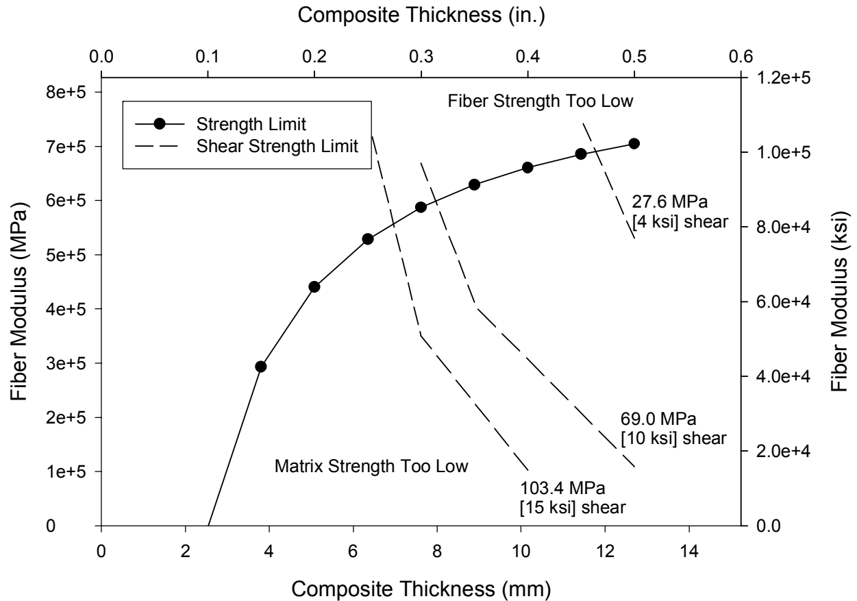
Figure 89 - Design Space for Composite Liner
