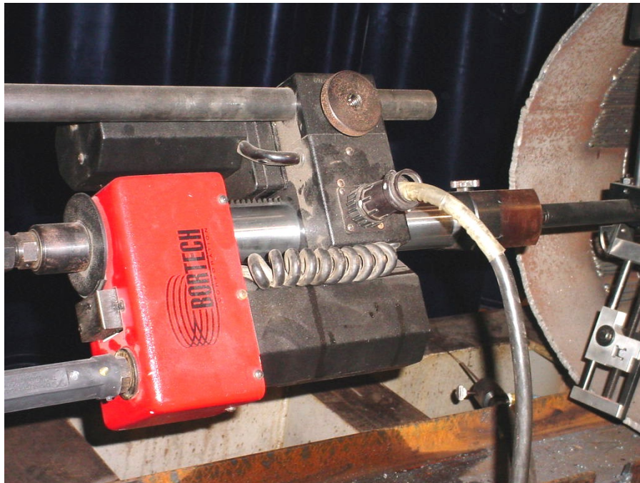
Figure 29 - Bortech Motion Mechanism for Continuous Spiral Deposition
