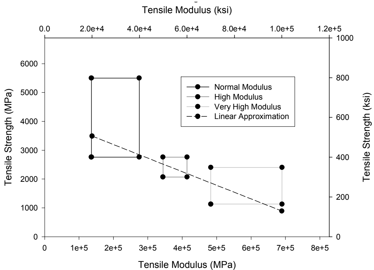
Figure 88 - Relationship Between Modulus and Strength for Carbon Fibers
