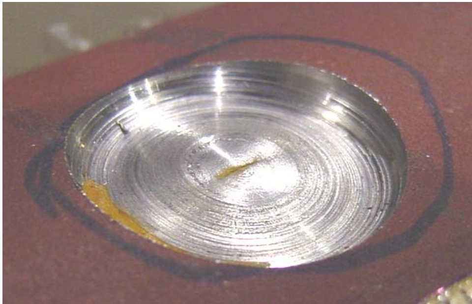
Figure 75 - Pipe Section with Short, Deep Simulated Corrosion Damage – Without Liner – Following Hydrostatic Pressure Test
