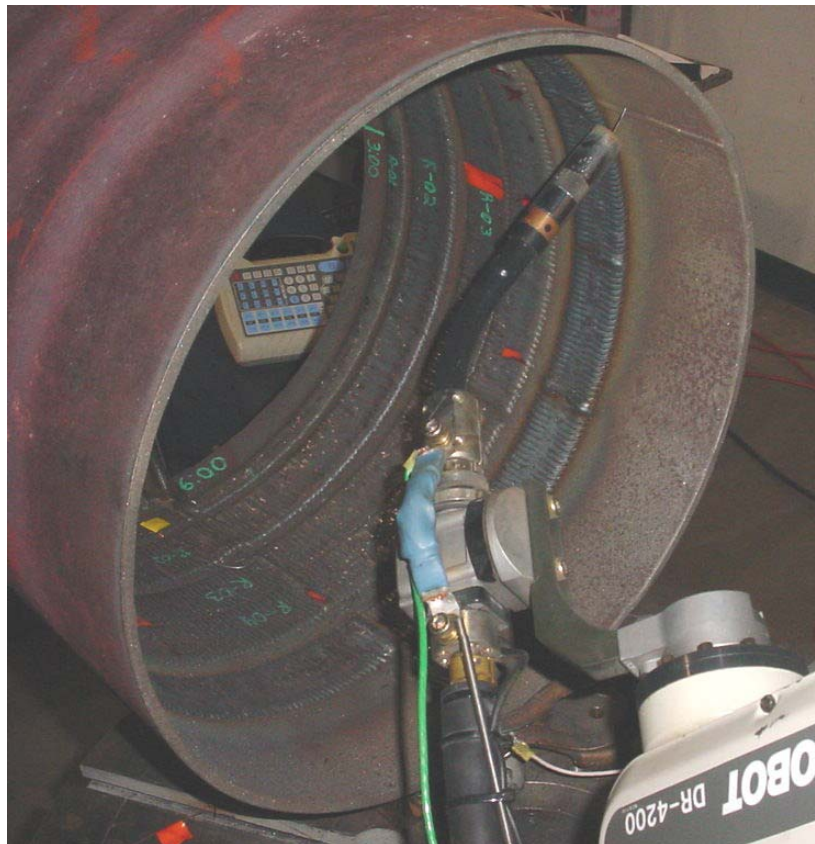
Figure 33 - OTC Robot Arm and Torch
