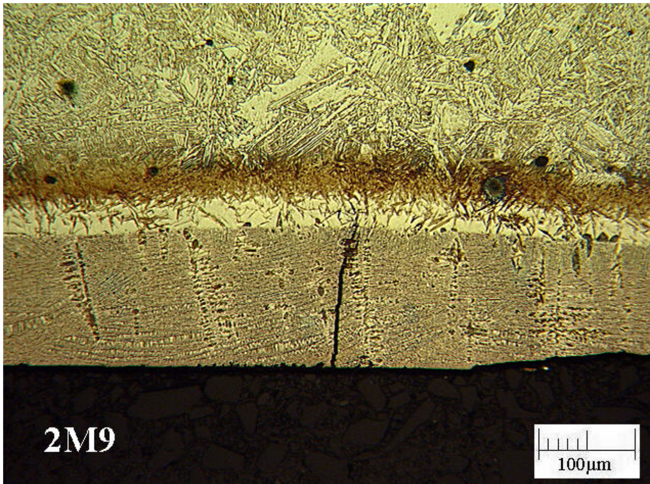
Figure 104 - Cracks in Eutectic Iron Layer of Metallographic Section Shown in Figure 103
