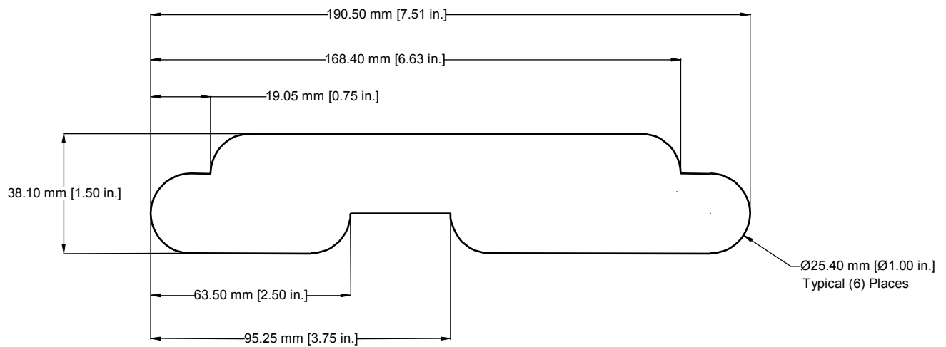
Figure 39 - Dimensions of Simulated Corrosion on 558.80 mm (22 in.) Pipe
