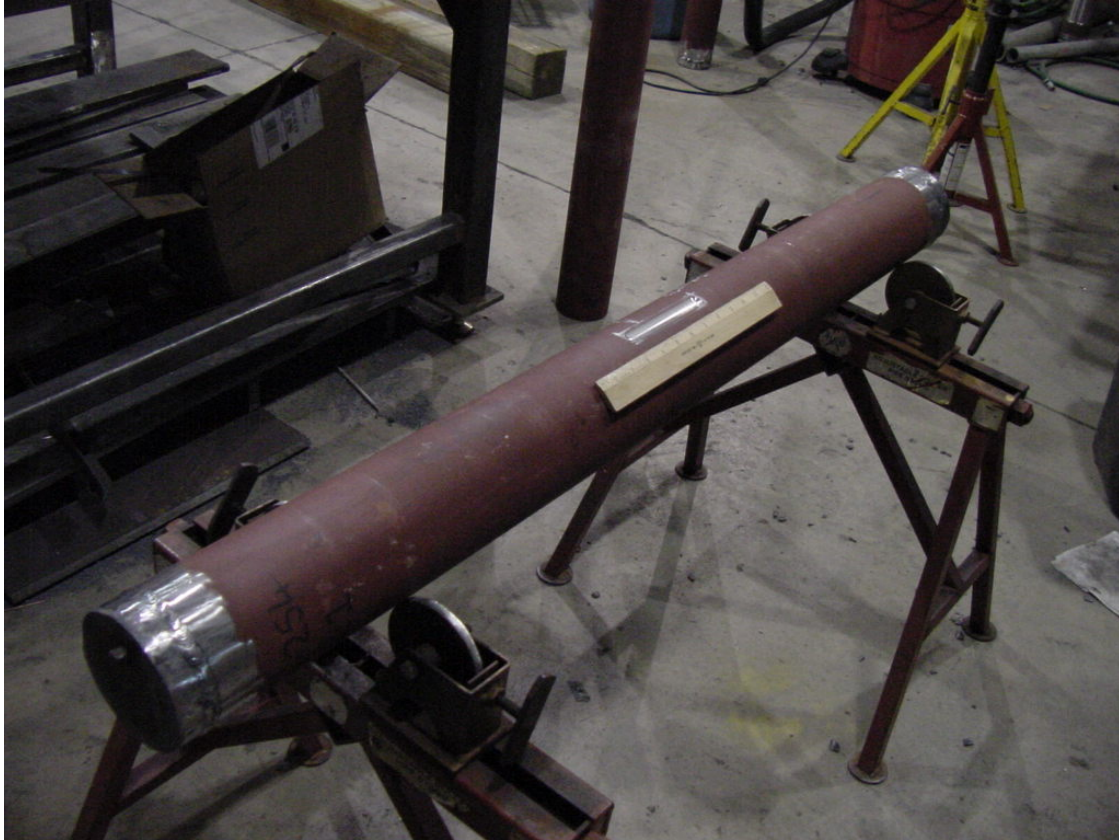
Figure 14 - 114.3 mm (4.5 in.) Diameter Pipe Section with End Caps Welded and Simulated Corrosion Damage
