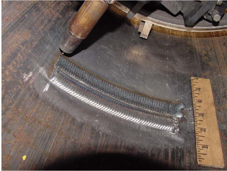
Figure 46 - Second Pass of First Layer of Deposited Weld Metal on Inside Pipe Diameter
