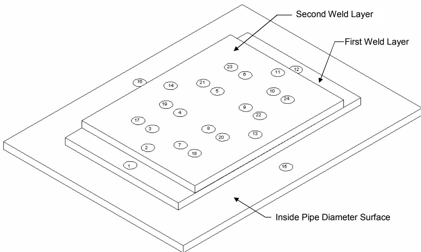
Figure 93 - Ultrasonic Thickness Measurement Locations on Weld Deposition Repair
