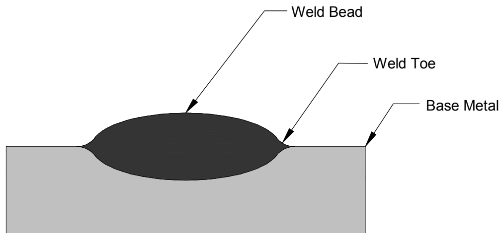
Figure 80 - Weld Bead Shape Diagram
