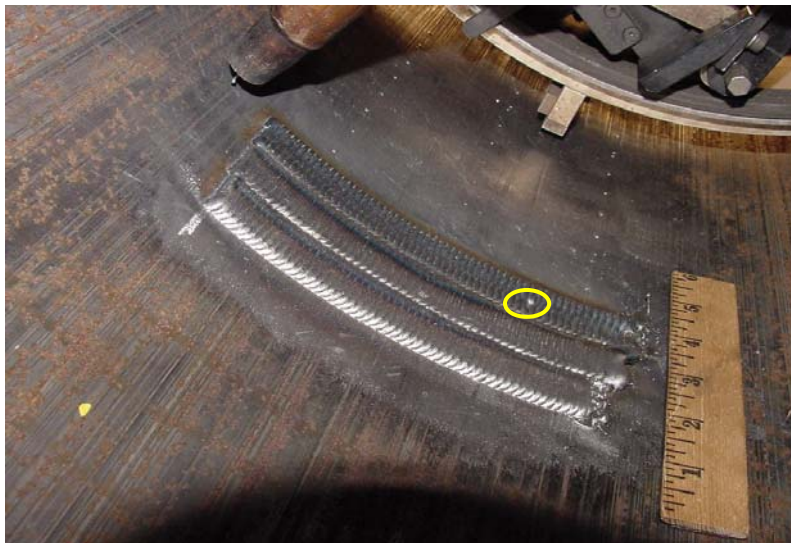
Figure 47 - Third Pass of First Layer of Deposited Weld Metal on Inside Pipe Diameter
