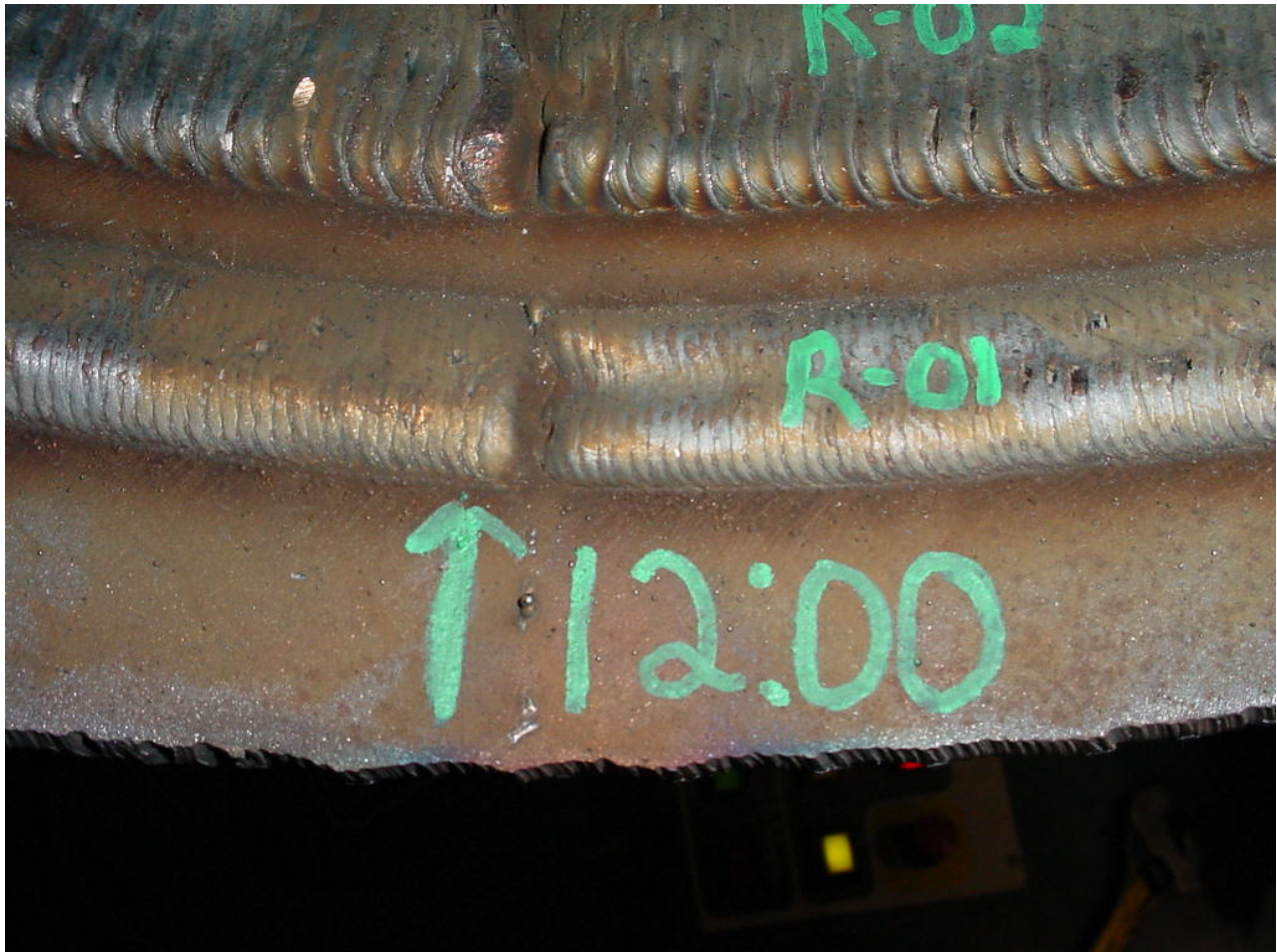
Figure 82 - Test R-01 at 12:00 Showing Poor Stop-Start Tie-In
