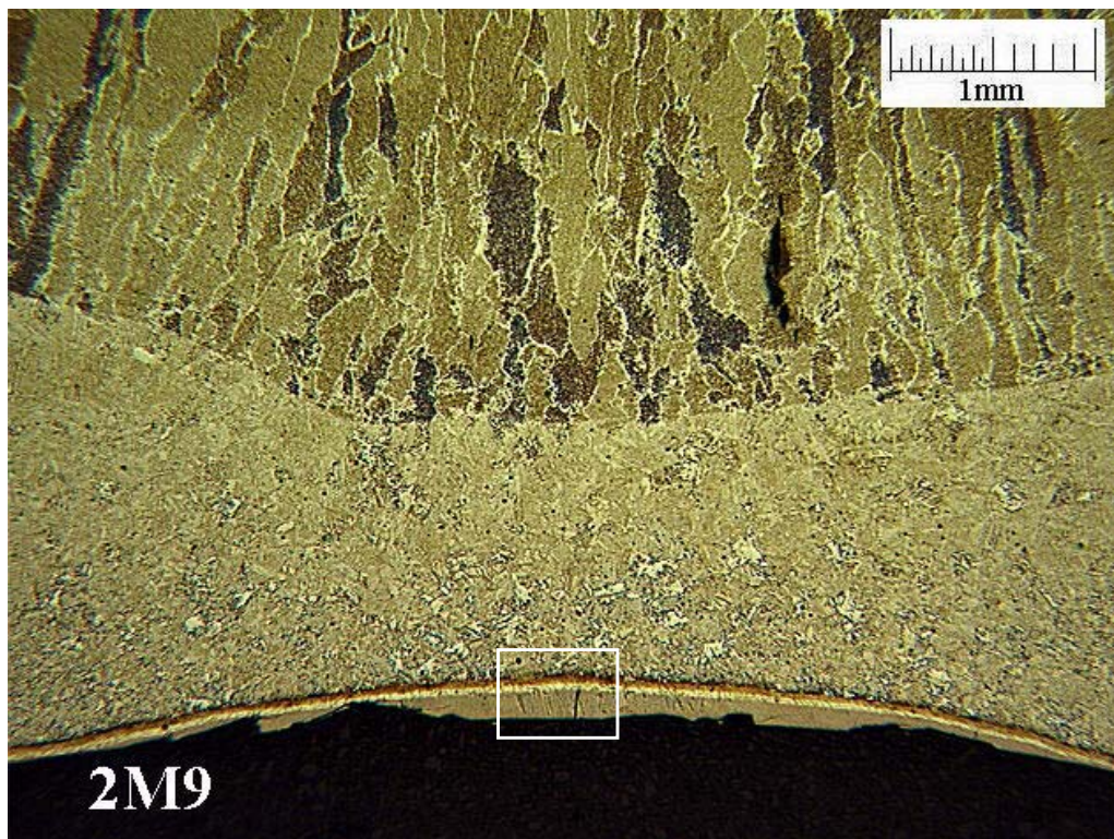
Figure 103 - Eutectic Iron Layer at Inside Surface of Metallographic Section through Weld 2M9
