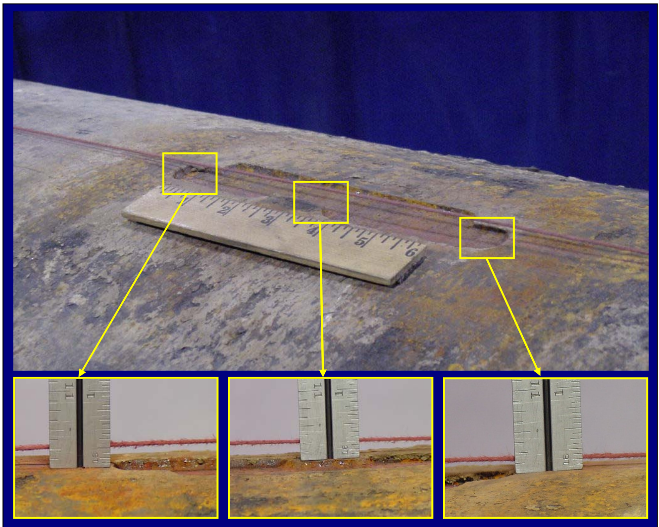
Figure 97 - Magnified Pictures of Dent at Ends and Middle of Simulated Damage
