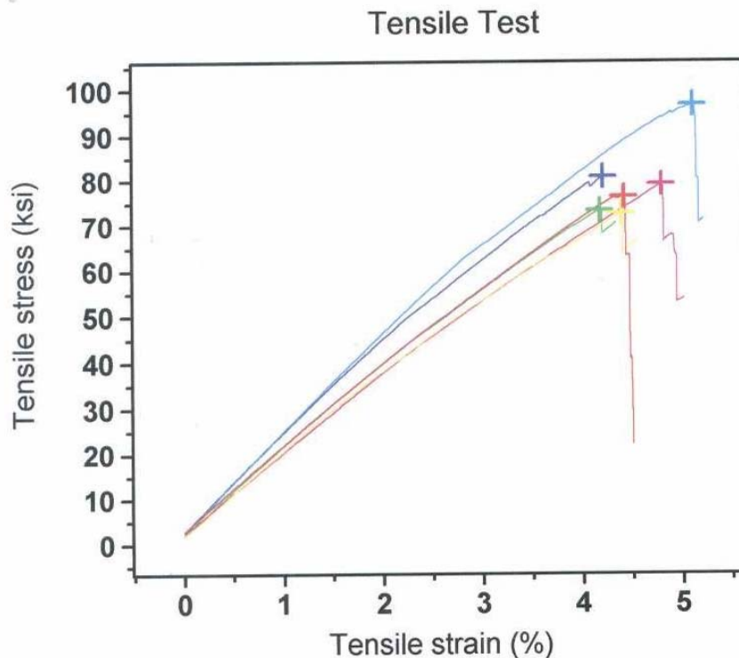
Figure 79 - Tensile Testing Results for Glass/Polypropylene Liner Material
