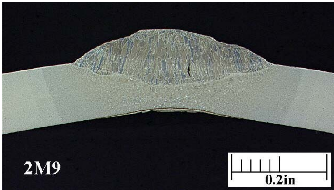
Figure 102 - Metallographic Section through Weld 2M9 (middle weld shown in Figure 100 and Figure 101)
