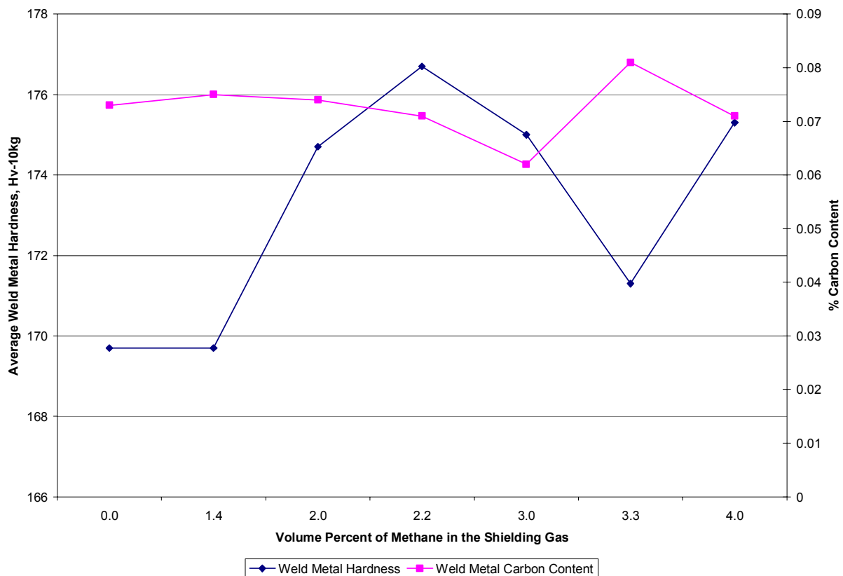
Figure 105 - Graphical Representation of Table 19 Hardness Values and Carbon Content
