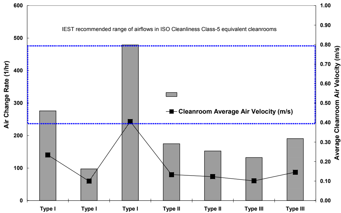
Figure 2. Actual recirculation air change rates and cleanroom air velocities vs. IEST recommended ranges [11]
