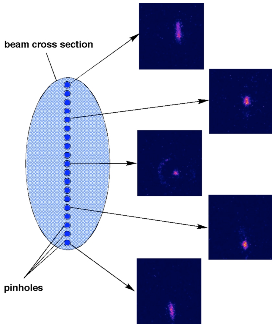
Figure 7. Beam imaging technique to measure the phase-space distribution f(x,y,x',y') .
