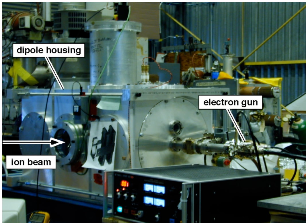
Figure 9. Photograph of the NTX non-intercepting beam diagnostic.
