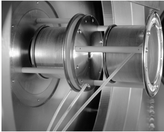
Figure 10. Photograph of the NTX beam scraper system.
