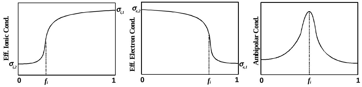
Figure 4. Diagram showing the relationship between effective ionic and electron conductivity, and the ambipolar conductivity as a function of composite volume fraction.
