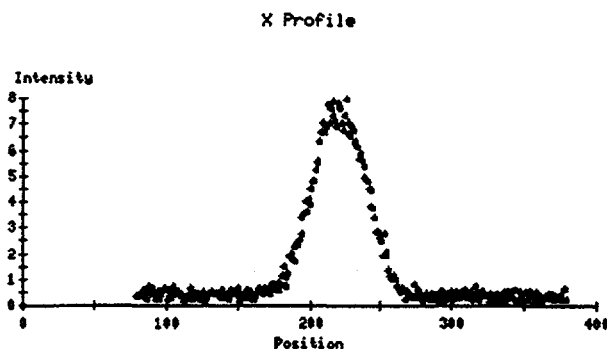
Figure 2: Video image profile of the PAR beam after damping using OSR. The total observed size was \Delta x=3.6 mm (FWHM) and \Delta y=0.6 mm (FWHM).
