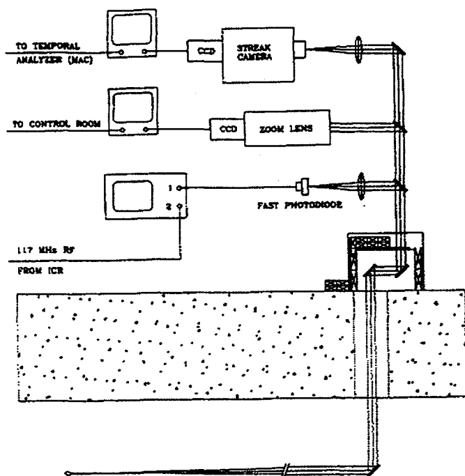
Figure 1: Schematic of OSR transport by mirrors out of the PAR and IS tunnels to detectors on an optics table.
