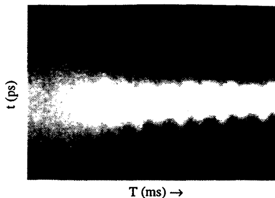
Figure 5: Dual-sweep streak image of the IS bunch length variation during the energy ramping cycle. These data cover from 35 to 130 ms in the ramp cycle on the horizontal axis and 1500 ps on the vertical axis. The bunch length is about 158 ps (FWHM) at the right-hand side.
