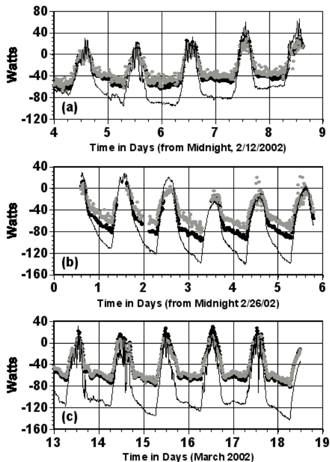
Figure 6. Performance of Prime/Storm Window Combinations. In each plot, the measured net heat flow through a prime/storm window combination (black dots) is compared with the simultaneously-measured net heat flow through the replacement window (gray dots). In addition, a continuous curve describes the calculated net heat flow through the prime window alone under the same instantaneous conditions. (a) Exterior low-e storm window tests. (b) Exterior uncoated storm window test. (c) Interior low-e storm window test.
