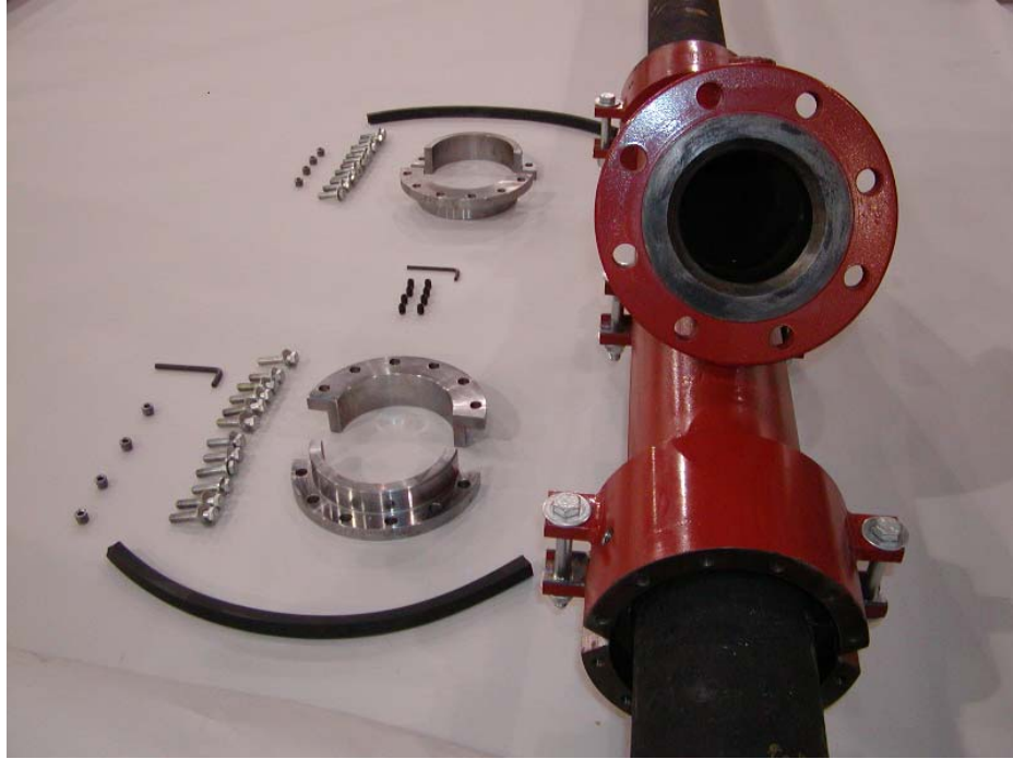
Figure 30. Cast Iron Entry Fitting (4-inch Prototype)
