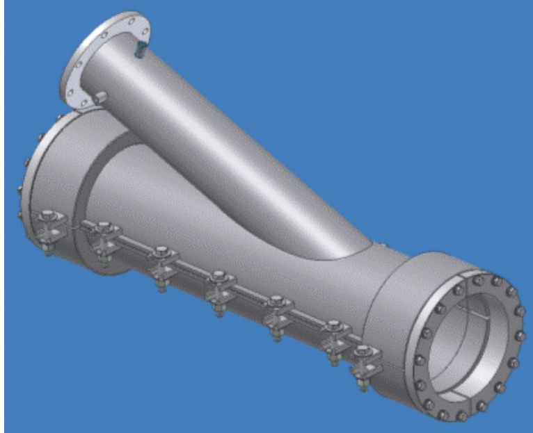
Figure 32. 12-Inch Entry Fitting
