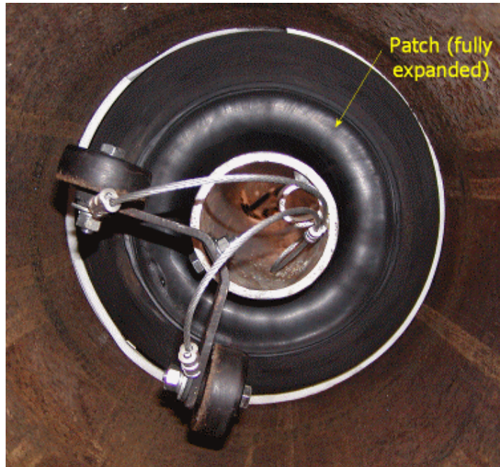
Figure 15. Patch Setting Test
