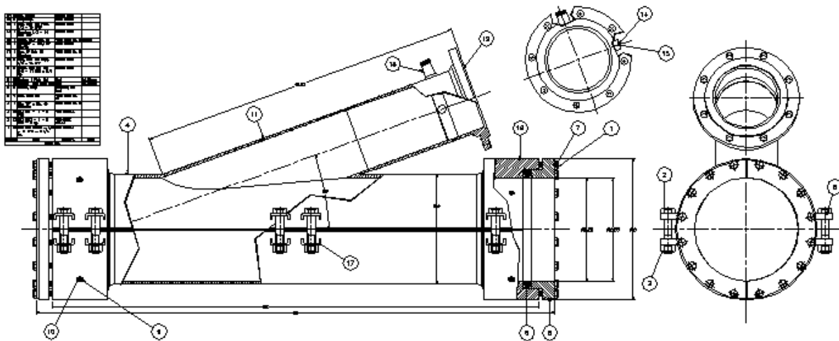
Figure 31. Entry Fitting for 12-inch Diameter Pipes
