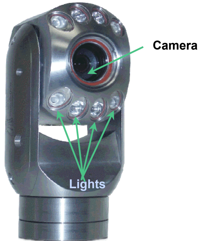
Figure 18. PZT Camera
