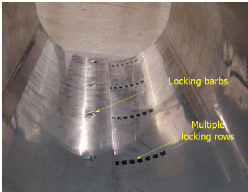
Figure 16. Locking Ratchets on Patch
