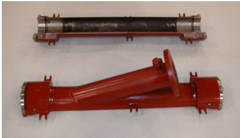
Figure 28. Cast Iron Entry Fitting (4-inch Prototype)
