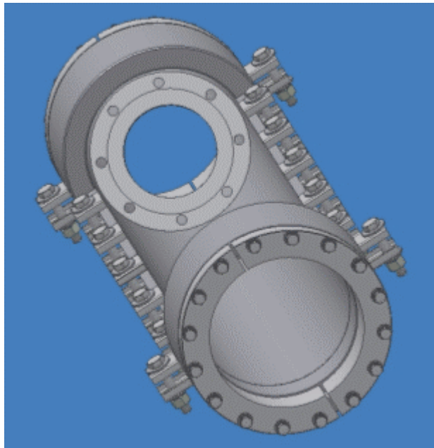
Figure 33. 12-Inch Entry Fitting Cutaway
