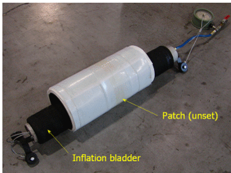
Figure 14. Patch-Setting Module
