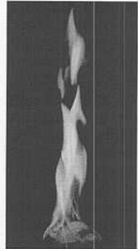
Figure 2. Methane Hydrate
