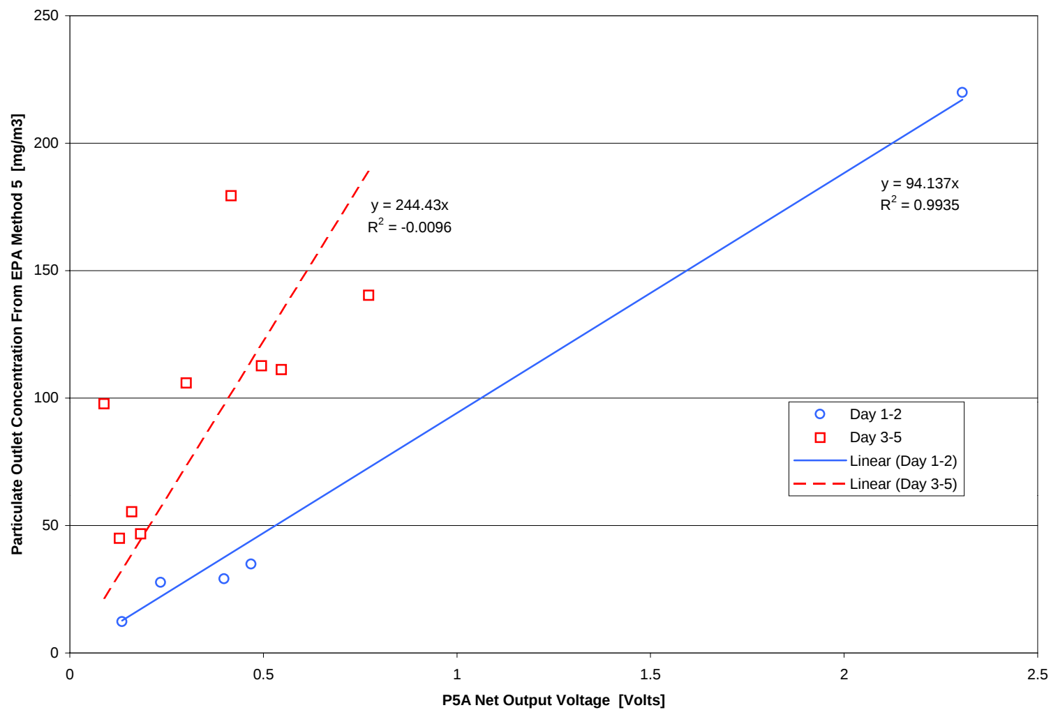
Figure 25: Correlation of P5A Output to EPA Method 5 Data
