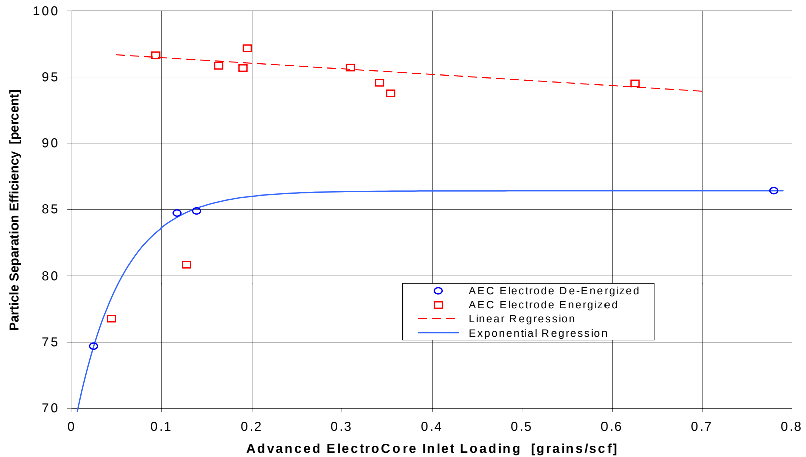
Figure 24: Efficiency of Advanced ElectroCore Field Prototype From P5A Analysis
