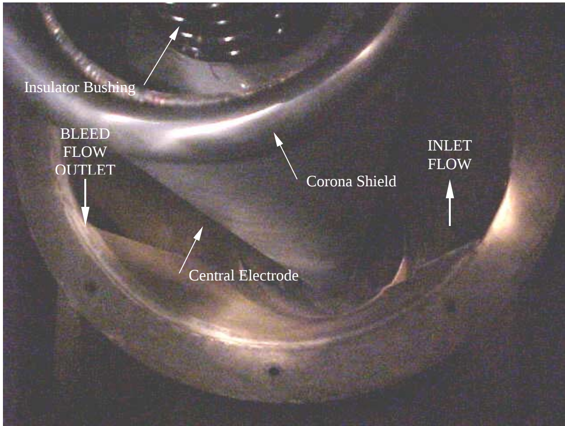
Figure 1: View Looking Down Into ElectroCore Separator Through Polycarbonate Top Cover
