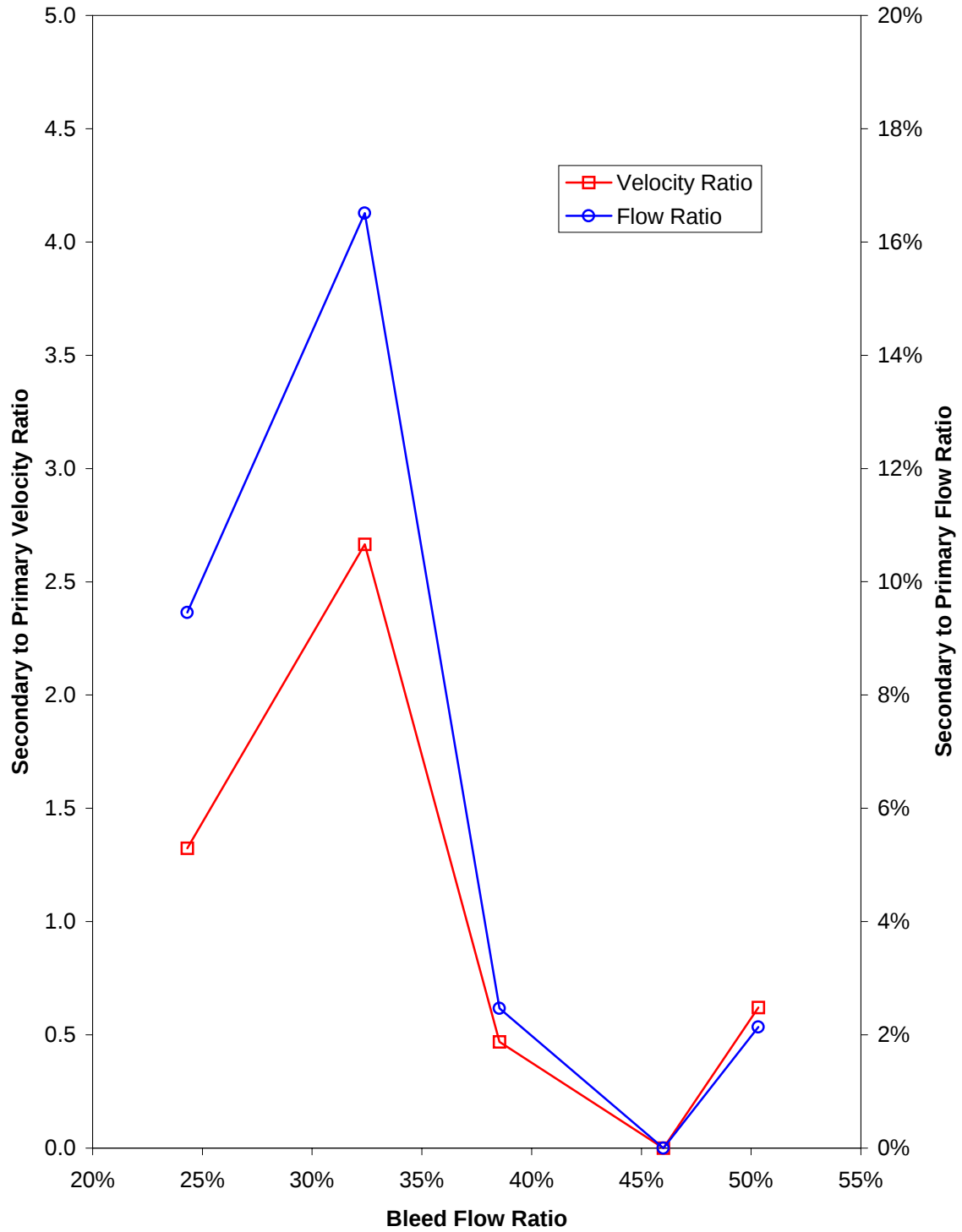
Figure 4: Secondary Bleed Flow Required to Stop Backflow
