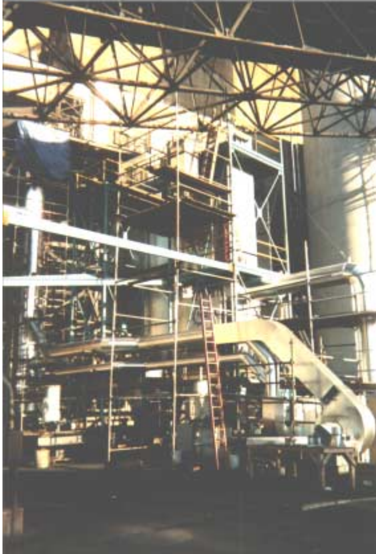
Figure 20: Complete System With Fans and Connecting Ductwork
