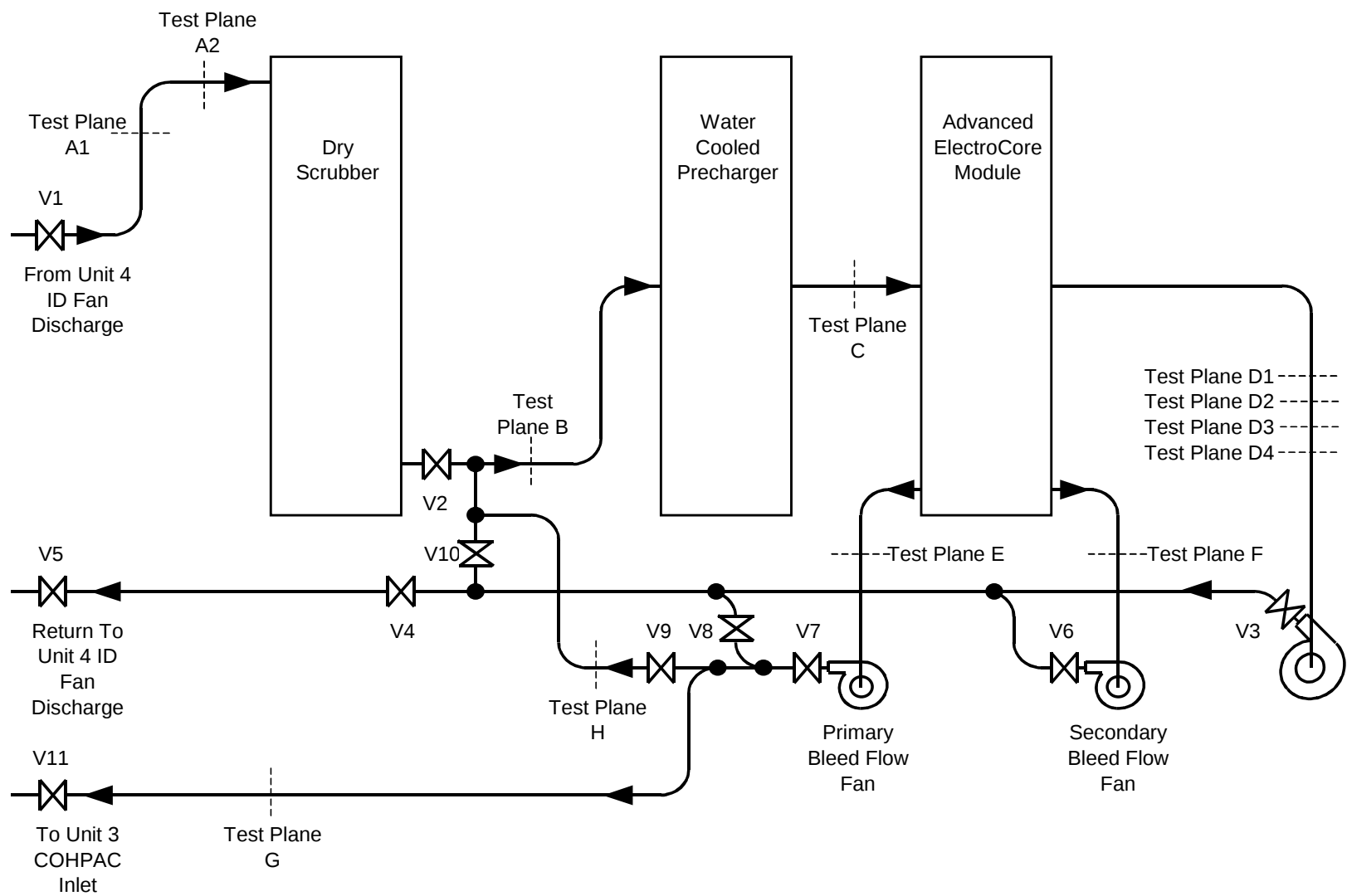
Figure 21: Advanced ElectroCore Field Prototype Flow Schematic
