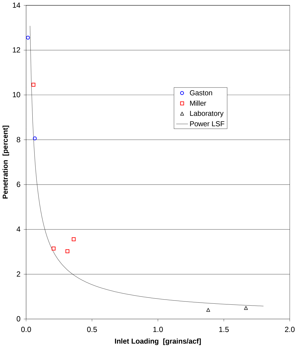
Figure 28: Effect of Inlet Loading on Particulate Penetration
