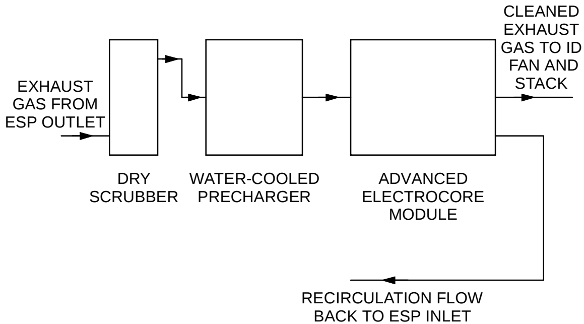
Figure 5: Schematic of Advanced ElectroCore Field Prototype
