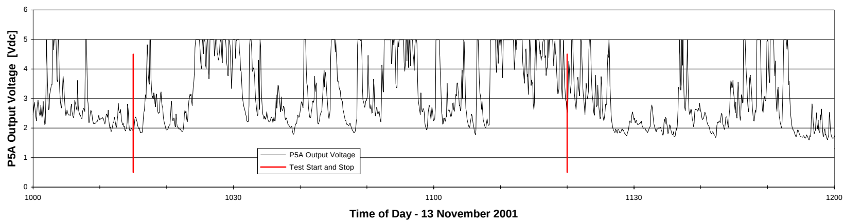
Figure 27: P5A Output Voltage For Test Number 4
