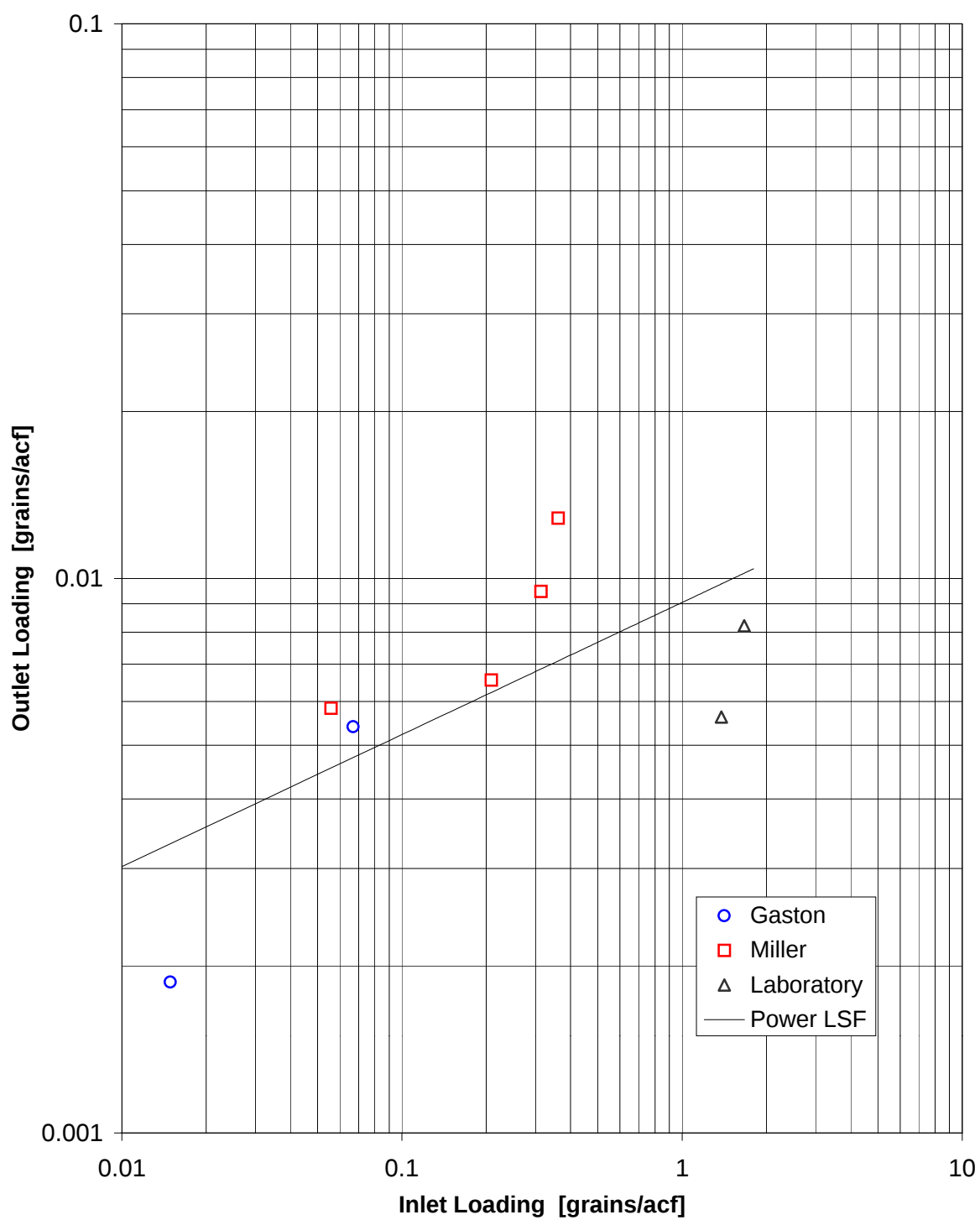
Figure 29: Effect of Inlet Loading on Particulate Outlet Loading
