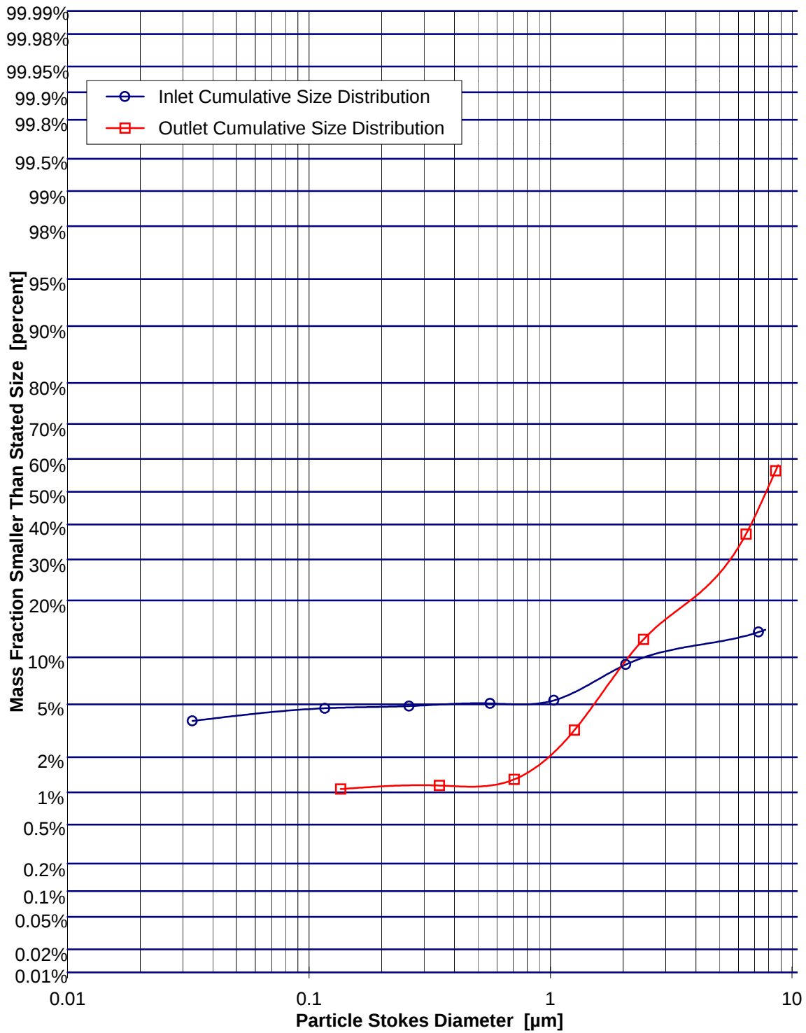
Figure 23: Inlet and Outlet Cumulative Particle Size Distribution
