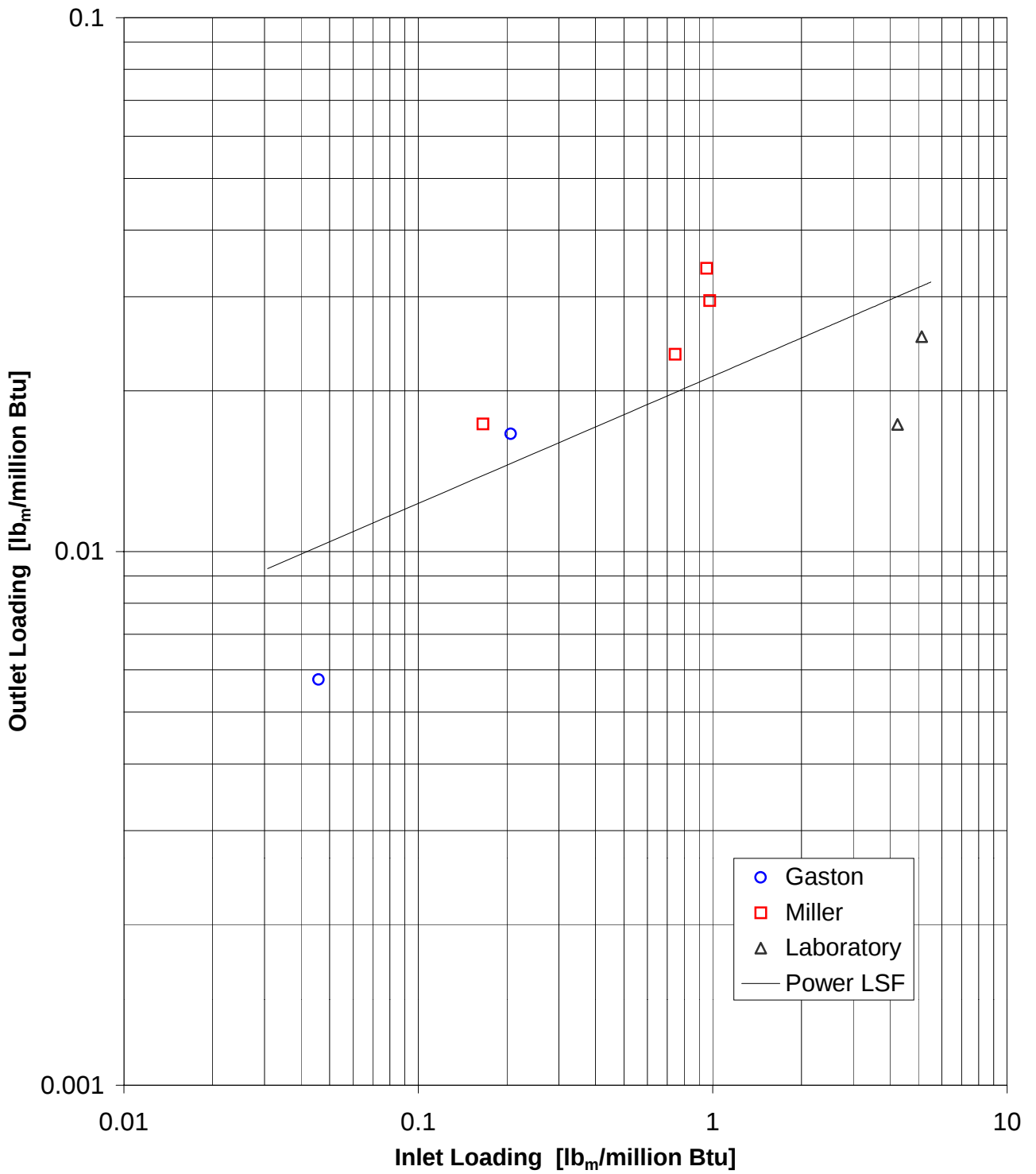
Figure 30: Effect of Inlet Loading on Particulate Outlet Loading Expressed in Pounds per Million Btu
