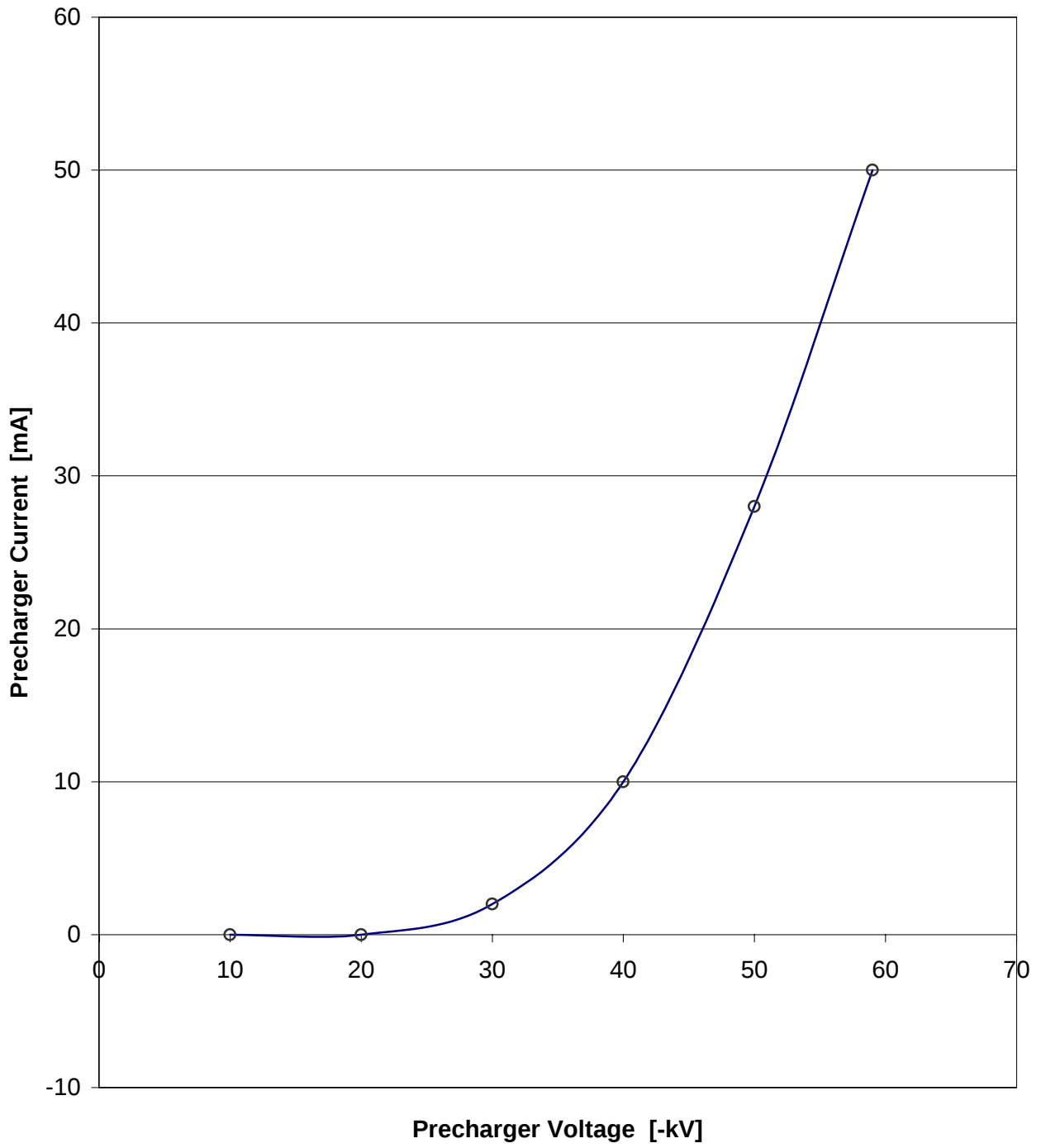
Figure 22: Precharger V-I Curve – As New
