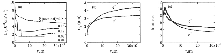
FIG. 1: Evolution of luminosity, vertical rms beam size and kurtosis ( \langle y^4 \rangle / 3 \langle y^2 \rangle ) obtained by the strong-strong simulation.
