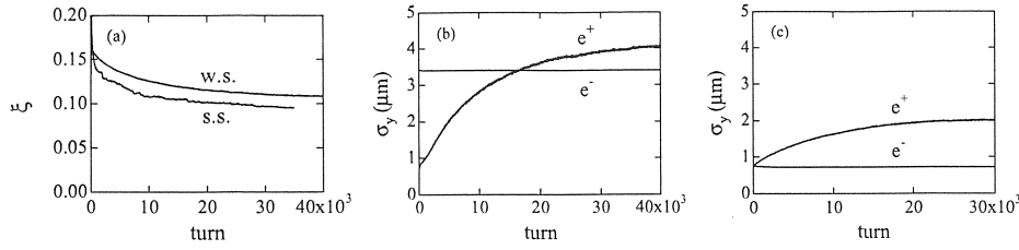
FIG. 4: Evolution of the beam-beam parameter and vertical size of electron and positron beams. Evolutions of \xi for the weak-strong and strong-strong simulation is depicted in (a), where the final distribution of the strong-strong simulation is used as a fixed distribution in the weak-strong simulation. Evolution of the beam size for the weak-strong simulation is depicted in (b). Evolution of the size of positron beam that interacts with fixed Gaussian electron beam is depicted in (c).
