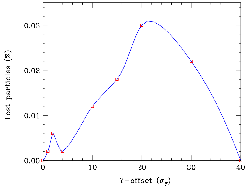
Figure 23: Particle loss in the extraction line vs. beam IP offset \Delta y (in undisrupted \sigma_y ) in option H with E_{cms} = 490 GeV.
