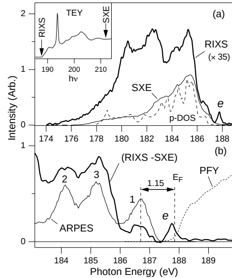
Fig. 3. (a) \text{CaB}_6 valence x-ray emission excited at-threshold (RIXS) and above-threshold (SXE) with comparison to calculated [12] boron p-DOS (dashed). (Inset) TEY absorption spectrum indicating excitation energies. (b) k-resolved RIXS difference spectrum (RIXS-SXE) with comparison to ARPES X-point spectrum showing alignment of valence band peaks and alignment of the ARPES Fermi level to the PFY absorption threshold.
