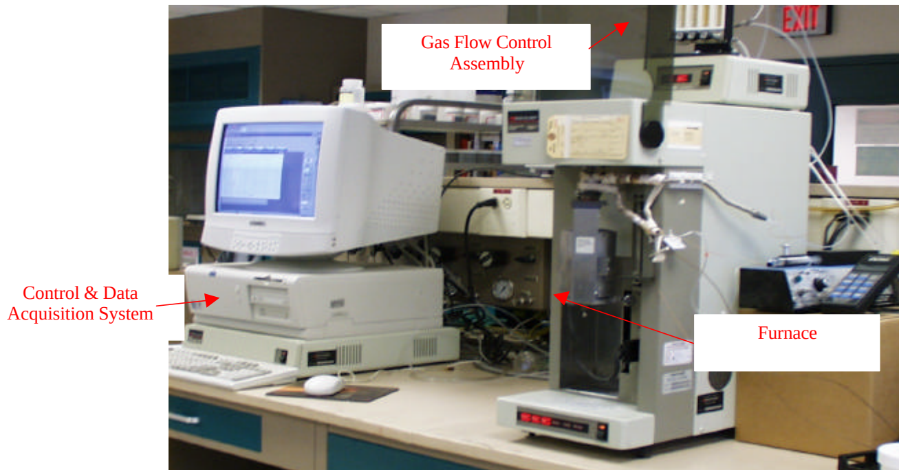
Figure 2.2. 1: Thermo-Gavimetric Analyzer (TGA)
