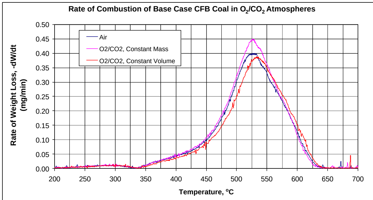
Figure 3.2.5: Rate of Weight Loss of Base Case CFB Coal in air and O_2/CO_2 Mixtures as a Function of Temperature
