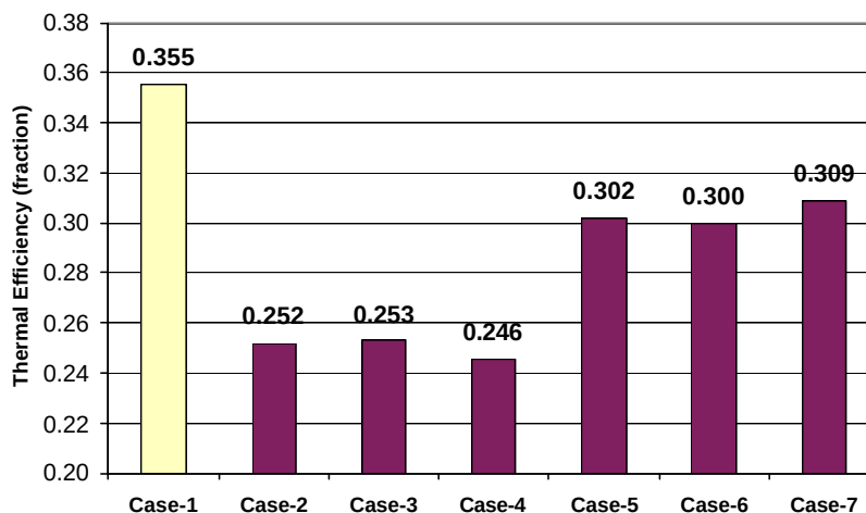
Figure 5.1. 7: Combustion Cases Plant Thermal Efficiency Comparison
