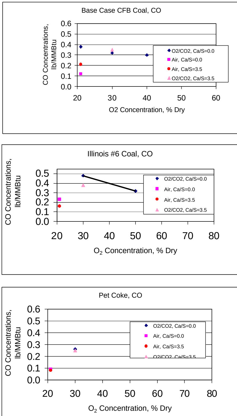
Figure 3.3.11: Variation of CO Emissions from Test Fuels as a Function of O 2 Concentration in Combustion Gas
