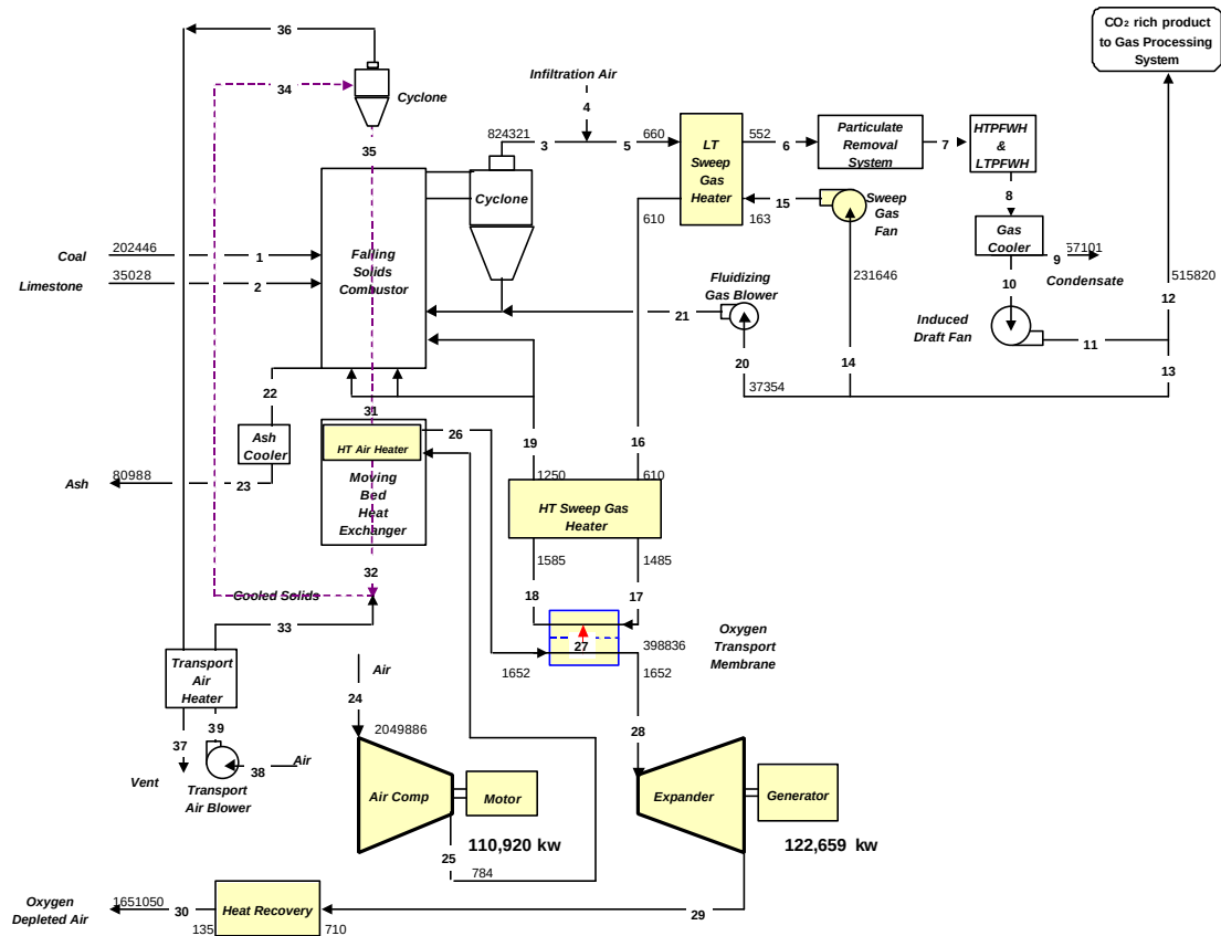
Figure 2.6. 1: Case-6 Simplified Boiler Island Gas Side Process Flow Diagram
