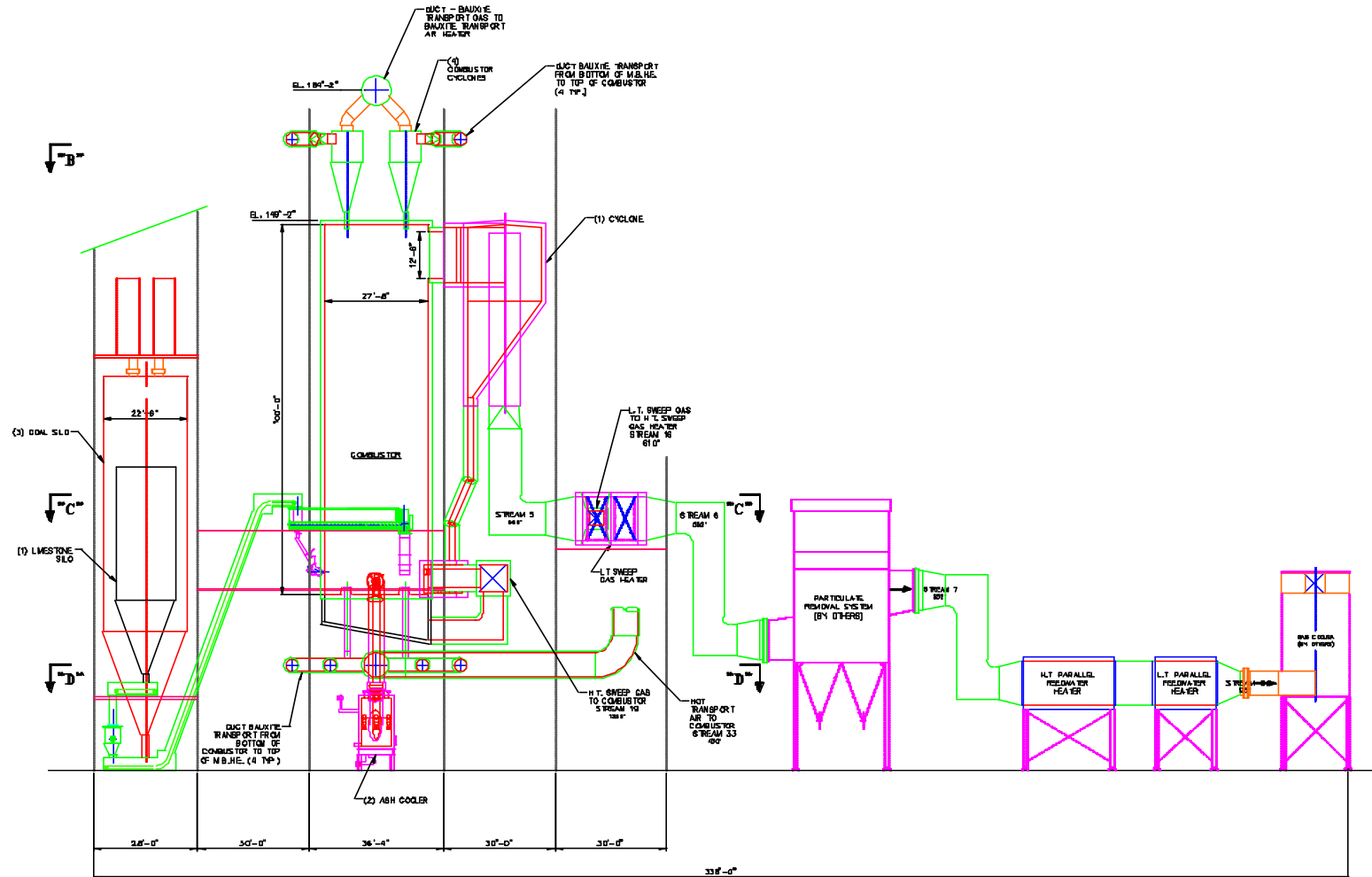
Figure 2.6. 2: Case-6 Boiler Island General Arrangement Drawing – Side Elevation
