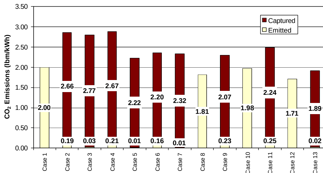
Figure 5.3. 3: CO 2 Emissions Comparison between Combustion and Gasification Cases
