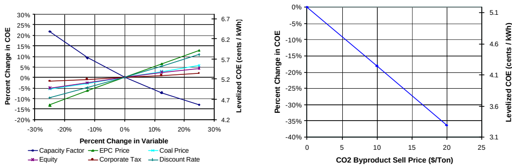
Figure 4.3.3: Case 13 – ALSTOM Advanced Chemical Looping with CO 2 Capture Economic Sensitivity Results
