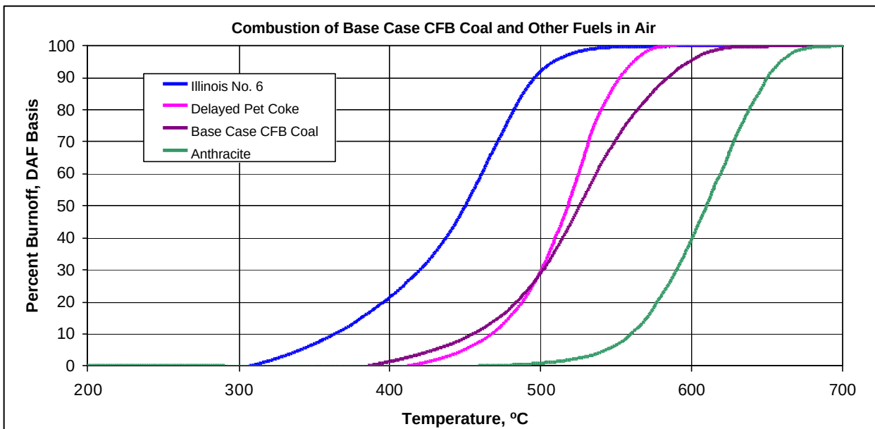
Figure 3.2.2: Burn-Off Shown as Weight Loss of Various Fuels in Air as a Function of Temperature
