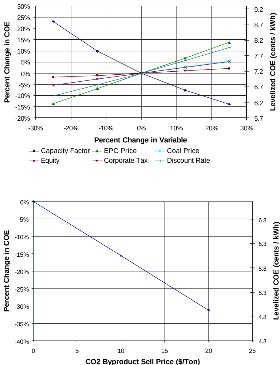
Figure 9.4.11: Case 11 - Texaco Commercially Offered IGCC with CO 2 Capture Economic Sensitivity Results
