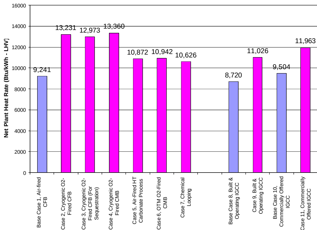
Figure 5.4. 1: Net Plant Heat Rates (LHV basis) from This Work
