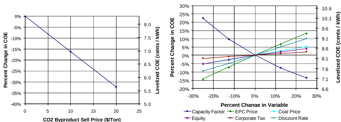
Figure 4.3. 1: Case 2 - Oxygen-Fired CFB with ASU and CO 2 Capture Economic Sensitivity Results
