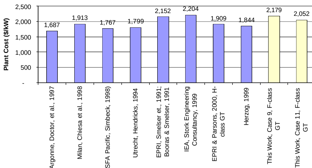
Figure 5.4. 6: IGCC's with CO 2 Capture - Comparison with Other Work
