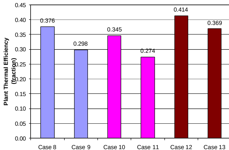
Figure 5.2. 4: Gasification Plants Thermal Efficiency Comparison
