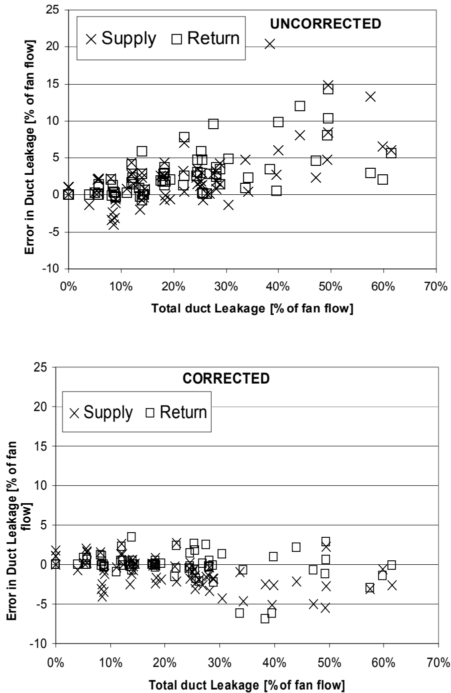
Figure 8. DeltaQ Error Variability with Total Leakage (sum of Supply and Return).
