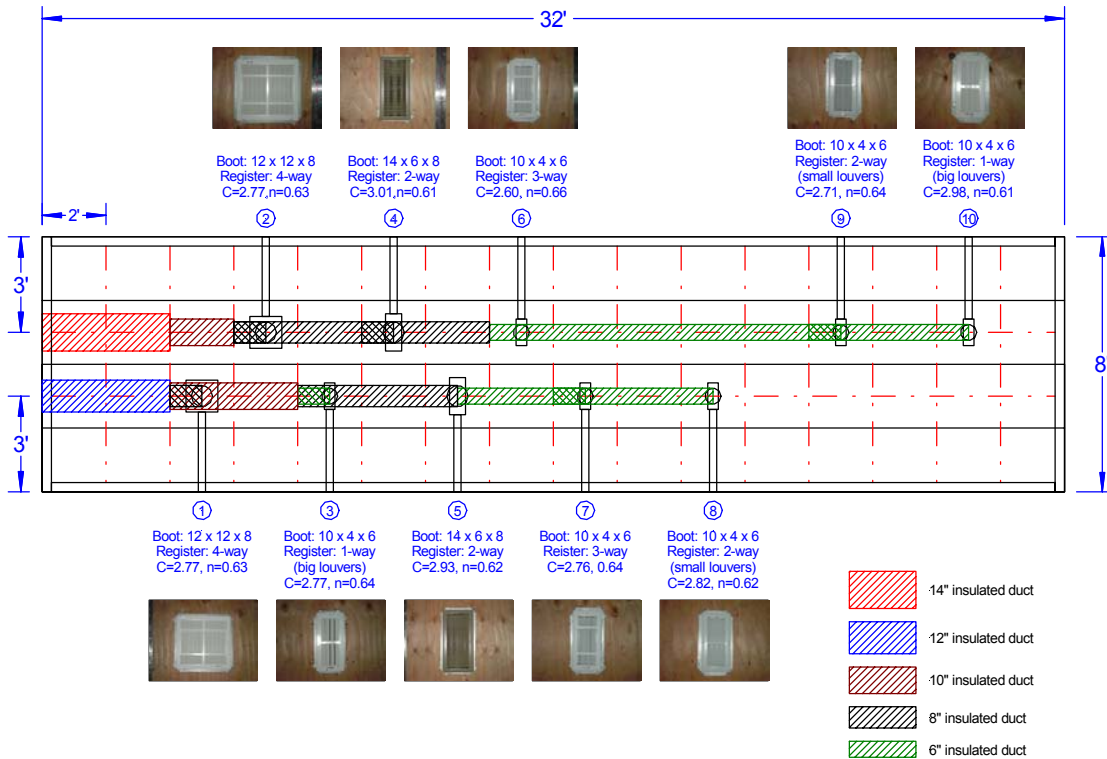
Figure 4. Floor plan of test chamber showing duct system layout, register location and added boot leakage locations numbered 1-10.
