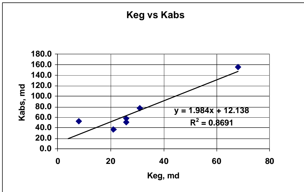
Figure 15: Correlation between Effective Gas and Absolute Permeability
