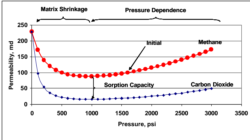
Figure 17: Permeability Changes with Pressure and Concentration
