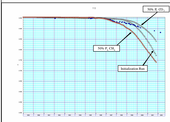
Figure 29: Actual versus Simulated Results, Langmuir Pressure for Methane and Carbon Dioxide at 50% of Original Value.
