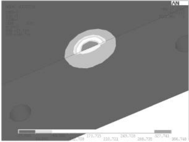
Figure 6. Temperature distribution at the target for the beam spot size calculated using the IGUN. The surface temperature of the titanium in this case is 366 °C.
