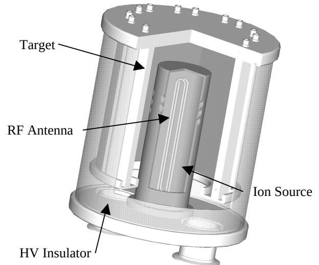
Figure 2. Co-axial neutron generator. RF-antenna inside the plasma chamber, surrounded by the target pieces. The outer pyrex cylinder is the HV insulator
