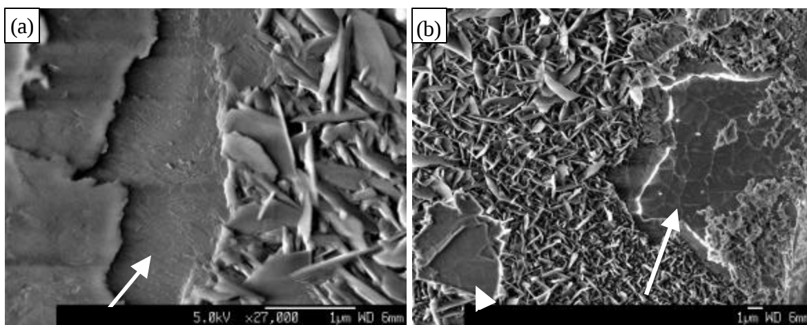
Figure 2: SEM micrographs of typical scale morphology on NiAl showing (a) initial transition alumina and smooth alloy surface after 5hr at 1000°C and (b) \alpha -Al 2 O 3 that had nucleated at the scale/alloy interface and the imprinted alloy surface after 65 hr.
