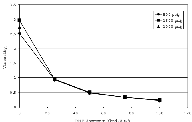
Figure 1. Blend response of viscosity to DME addition at various pressures [4].
