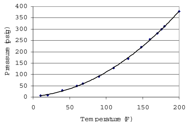
Figure 5. Vapor pressure of DME as a function of temperature [50].
