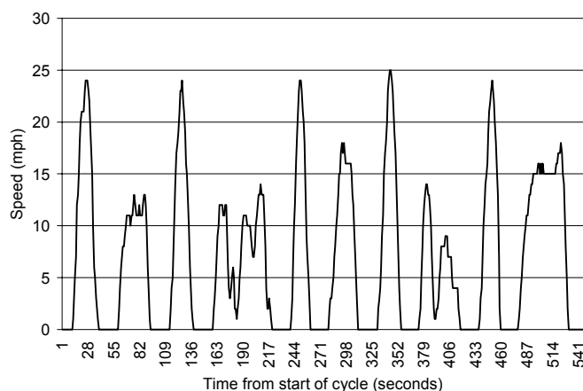
Figure 8. Manhattan Cycle – Driving Cycle to Represent Transit Bus Operation in Manhattan, NY.
