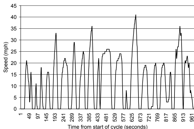
Figure 6. Part One of the Orange County Cycle – Driving Cycle to Represent Transit Bus Operation in Orange County, CA.
