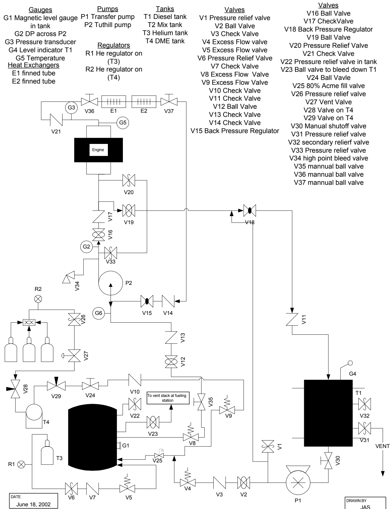
Figure 2. Schematic Diagram of the DME-Diesel Fueling System
