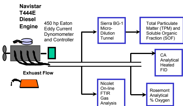
Figure 1. Multicylinder Test Cell, Navistar T444E Turbodiesel
