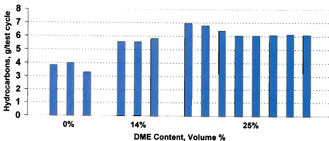
Figure 21. Hydrocarbon Emissions During the Manhattan Cycle (cumulative mass emissions per test cycle) for 0, 14 and 25 vol.% DME in Diesel Fuel.
