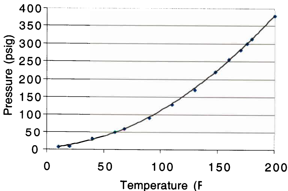
Figure 15. Vapor pressure of DME as a function of temperature [6].
