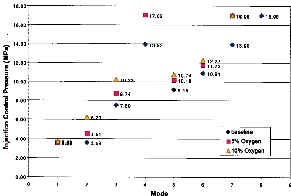
Figure 4. Engine Injection Pressure
