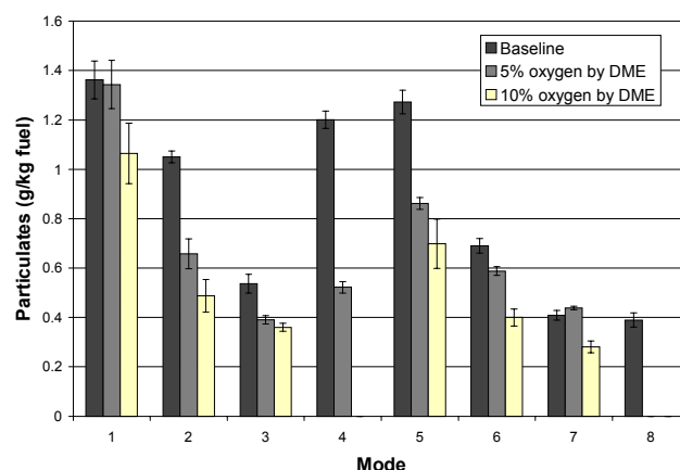
Figure 3. Particulate Matter Results per unit fuel consumed, g/kg fuel
