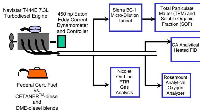
Figure 1. Multicylinder Engine Test Cell Navistar T444E 7.3L Turbodiesel
