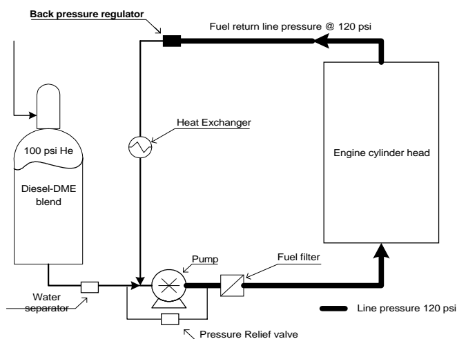
Figure 2. Pressurized Fuel System Diagram for the Navistar T444E Turbodiesel Engine.
