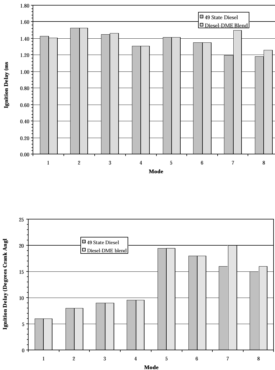
Figure 4-6: Ignition Delay Comparison
