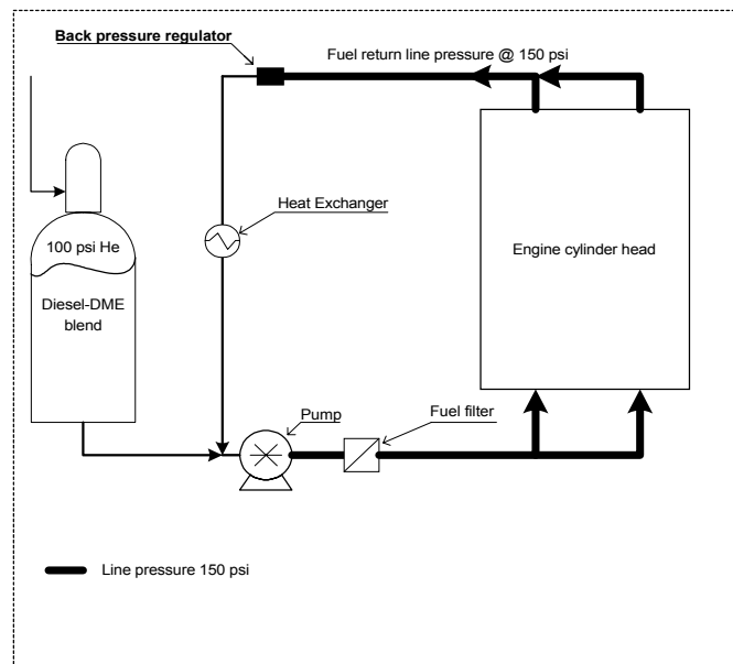
Figure 2. Diagram of the pressurized fuel system [5].
