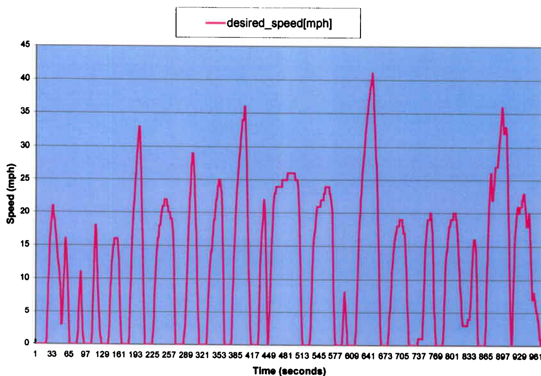
Figure 17. Part One of the Orange County Cycle – Driving Cycle to Represent Transit Bus Operation in Orange County, CA.
