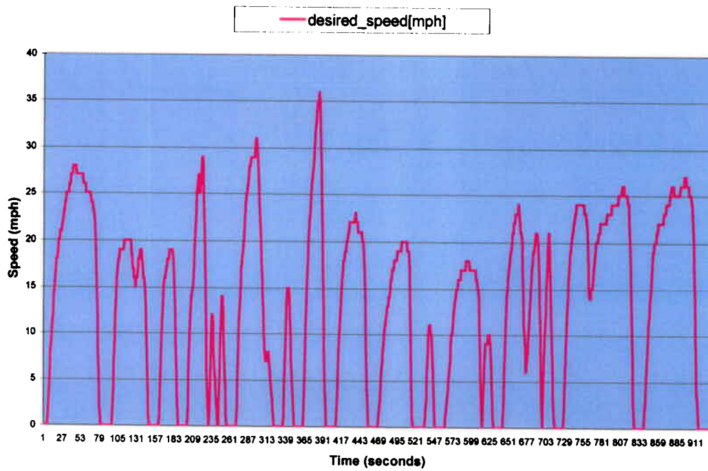
Figure 18. Part Two of the Orange County Cycle.
