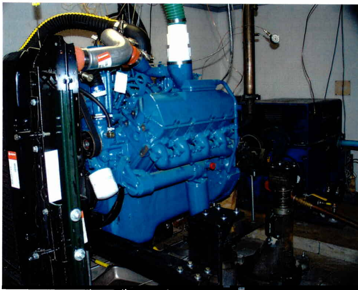
Figure 1. Photo of the Navistar T444E Turbodiesel Engine in the 450 hp Engine Test Cell Prior to Conversion to DME-Diesel Blends
