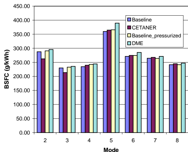
Figure 9. Fuel Consumption, Brake Specific Basis.
