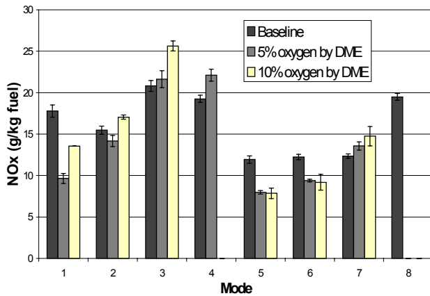
Figure 4. NOx Emission Results per unit fuel consumed, g/kg fuel
