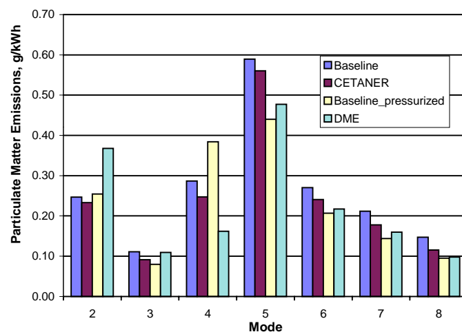
Figure 3. Particulate Matter Emissions, Brake Specific Basis.
