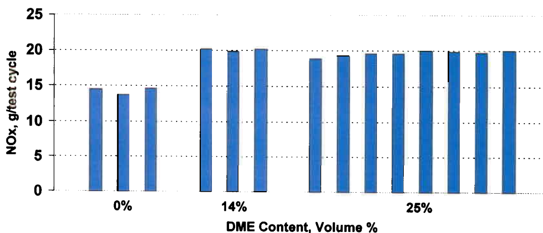
Figure 22. NOx Emissions During the Manhattan Cycle (cumulative mass emissions per test cycle) for 0, 14 and 25 vol.% DME in Diesel Fuel.
