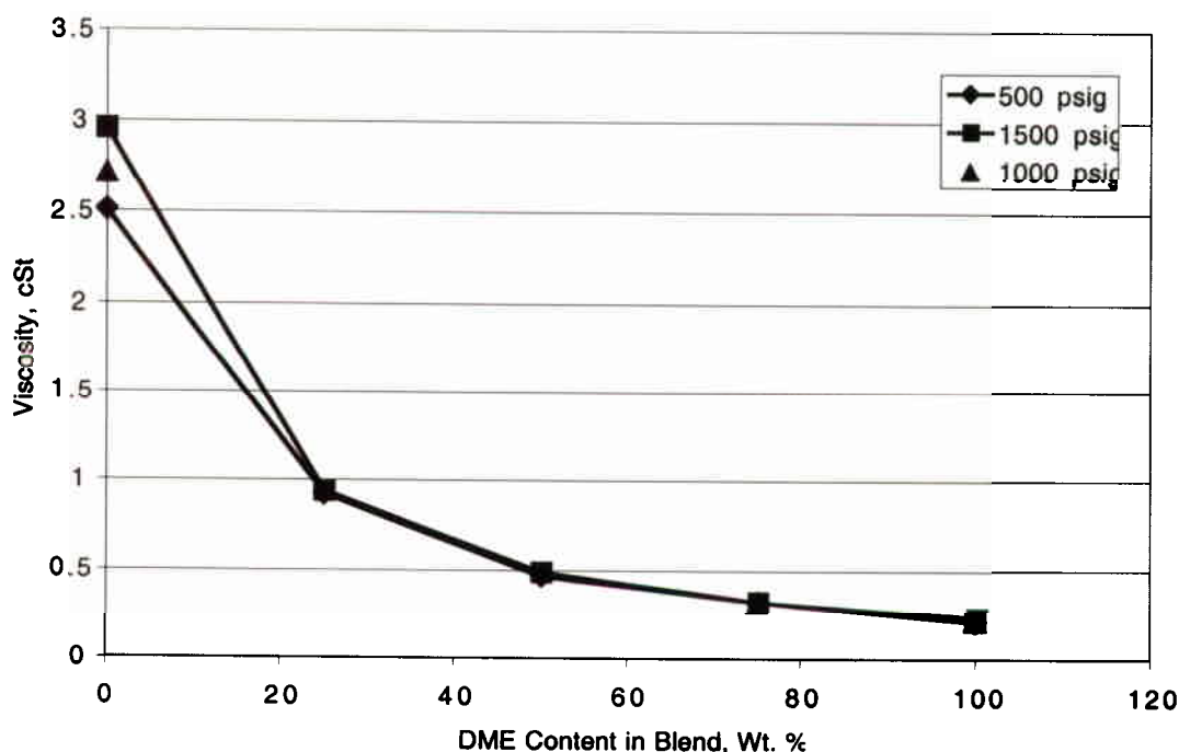
Figure 9. Viscosity – DME Content Relationship at Different Pressures @100 F
