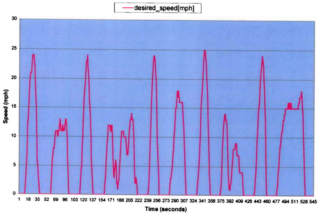
Figure 19. Manhattan Cycle – Driving Cycle to Represent Transit Bus Operation in Manhattan, NY.
