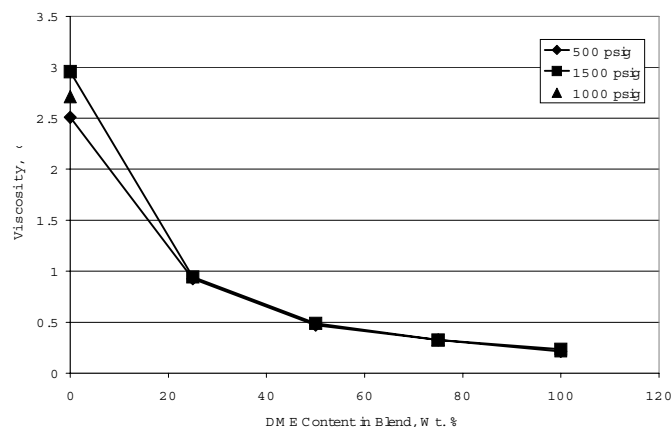
Figure 4. Blend response of viscosity to DME addition at various pressures.
