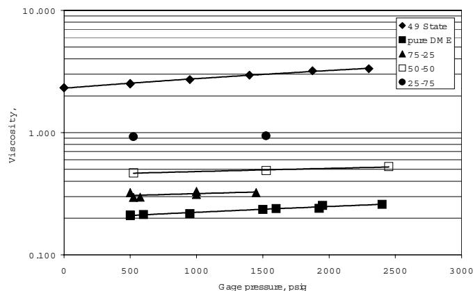
Figure 3. Viscosity of DME-diesel blends at pressures from 500 to 2500 psi.
