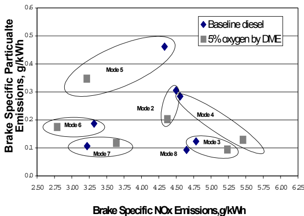
Figure 5. Brake-Specific Particulate Emission vs. NOx Emission Tradeoff
