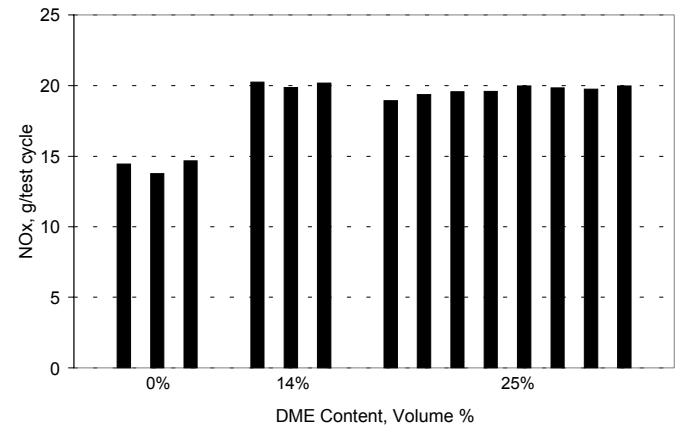
Figure 11. NO x Emissions During the Manhattan Cycle (cumulative mass emissions per test cycle) for 0, 14 and 25 vol.% DME in Diesel Fuel.
