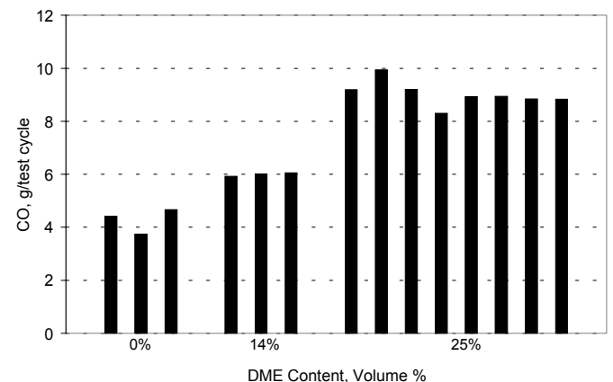
Figure 12. Carbon Monoxide Emissions During the Manhattan Cycle (cumulative mass emissions per test cycle) for 0, 14 and 25 vol.% DME in Diesel Fuel.
