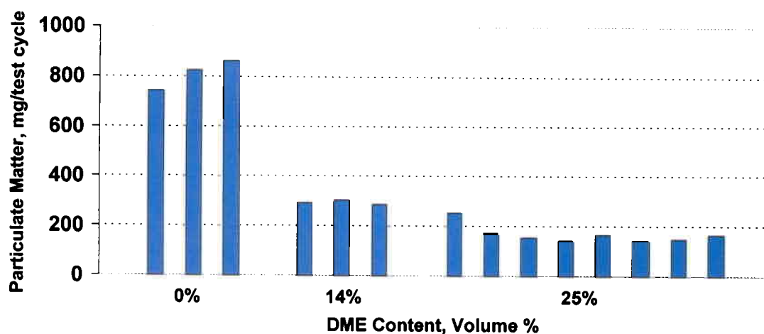
Figure 20. Particulate Matter Emissions During the Manhattan Cycle (cumulative mass emissions per test cycle) for 0, 14 and 25 vol.% DME in Diesel Fuel.
