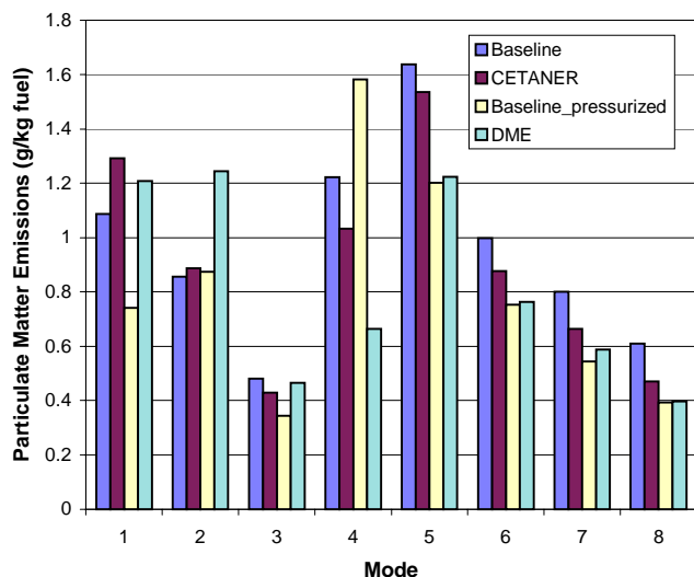
Figure 4. Particulate Matter Emissions, g/kg Fuel Basis.
