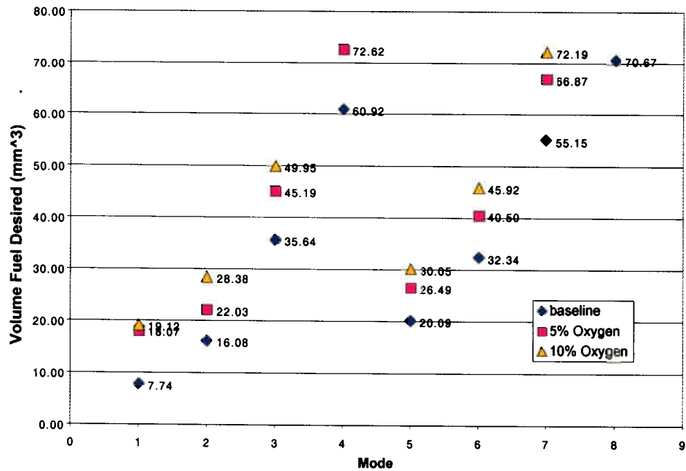
Figure 5. Engine control commanded fuel volume desired
