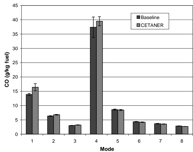
Figure 7. CO Emissions per Unit Fuel Consumed for CETANER™ Addition, g/kg Fuel Basis.
