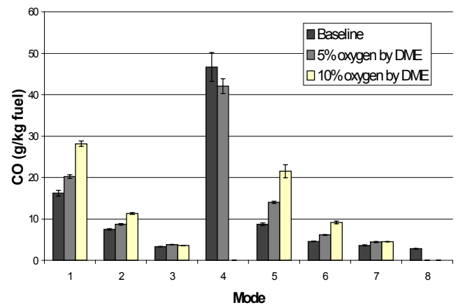
Figure 6. CO Emission Results per unit fuel consumed, g/ kg fuel
