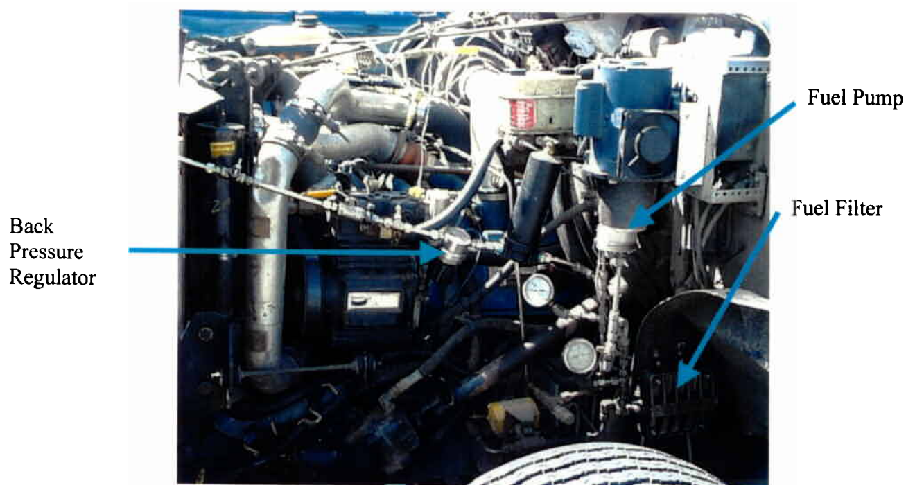
Figure 14. Photograph of the fuel handling system on the converted shuttle bus
