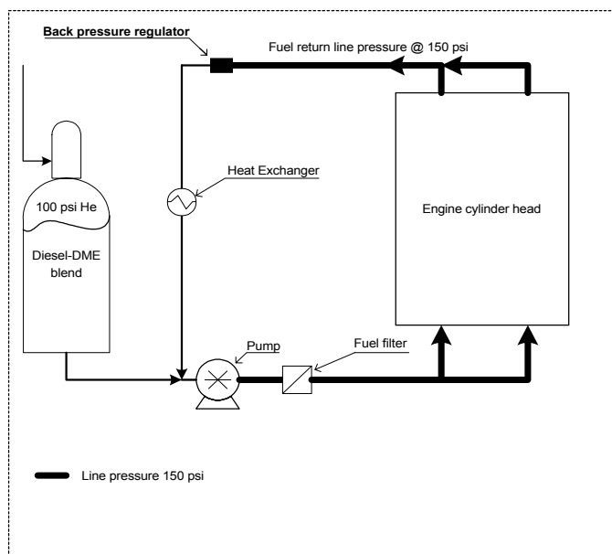
Figure 2. Diagram of Pressurized Fuel System
