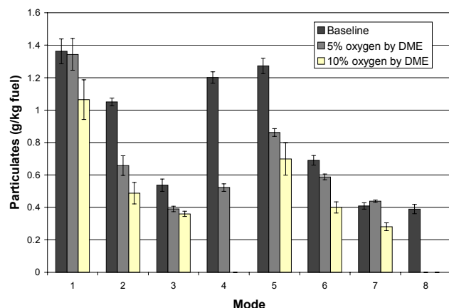
Figure 3. Particulate Matter Results per unit fuel consumed, g/kg fuel [5].
