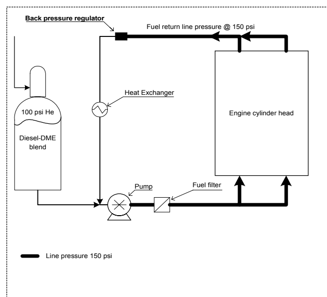
Figure 1. Pressurized Fueling System Developed in Laboratory Studies on DME-diesel Blends [46, 47]
