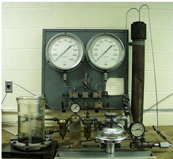
Figure 2. Supporting instrumentation for the high pressure viscometer.
