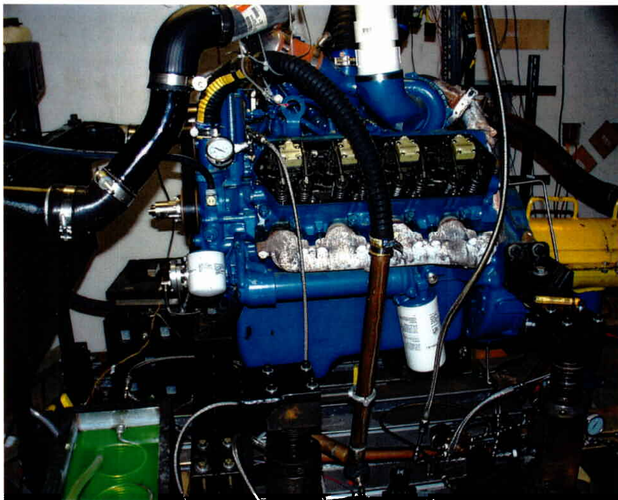
Figure 2. Navistar T444E showing conversion to DME-diesel operation.
