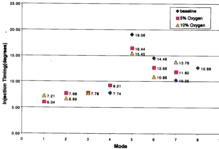
Figure 3. Engine Injection Timing
