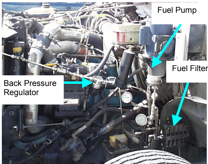
Figure 3. Photograph of the fuel handling system on the converted shuttle bus
