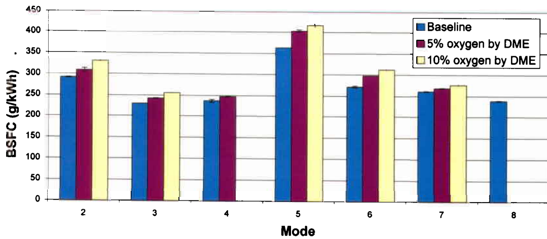
Figure 6. Fuel Consumption
