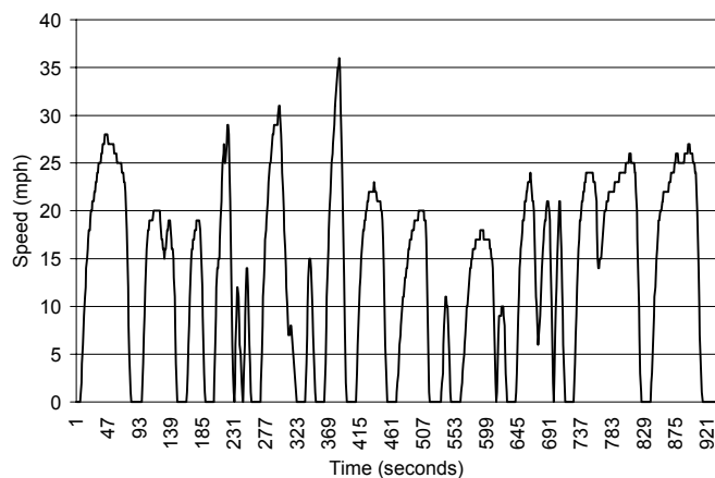
Figure 7. Part Two of the Orange County Cycle.
