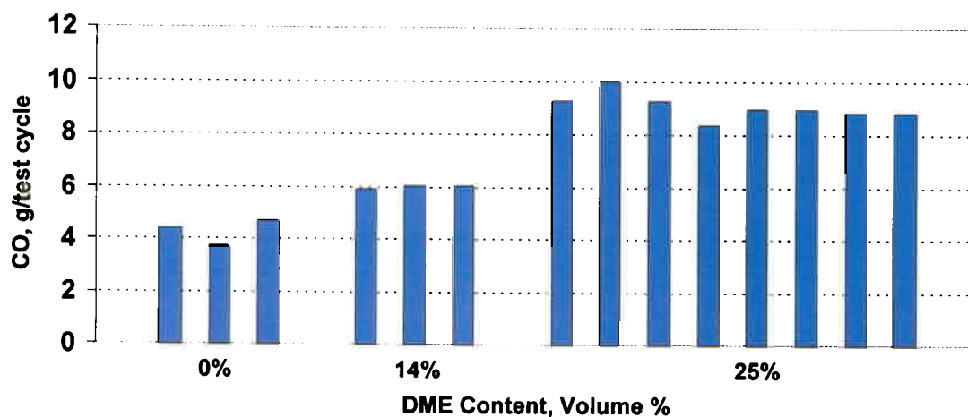
Figure 23. Carbon Monoxide Emissions During the Manhattan Cycle (cumulative mass emissions per test cycle) for 0, 14 and 25 vol.% DME in Diesel Fuel.
