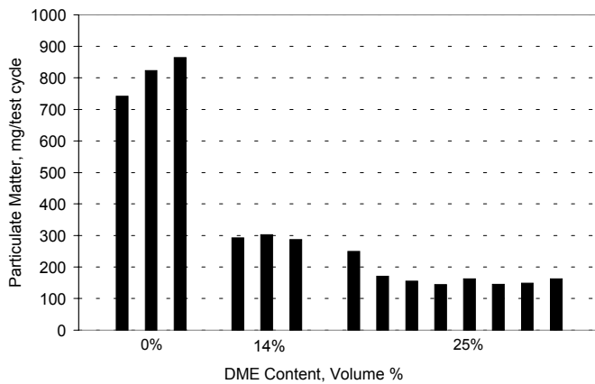
Figure 9. Particulate Matter Emissions During the Manhattan Cycle (cumulative mass emissions per test cycle) for 0, 14 and 25 vol.% DME in Diesel Fuel.
