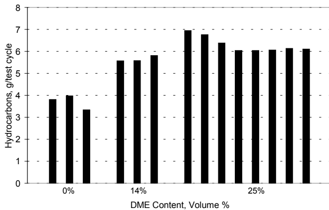
Figure 10. Hydrocarbon Emissions During the Manhattan Cycle (cumulative mass emissions per test cycle) for 0, 14 and 25 vol.% DME in Diesel Fuel.
