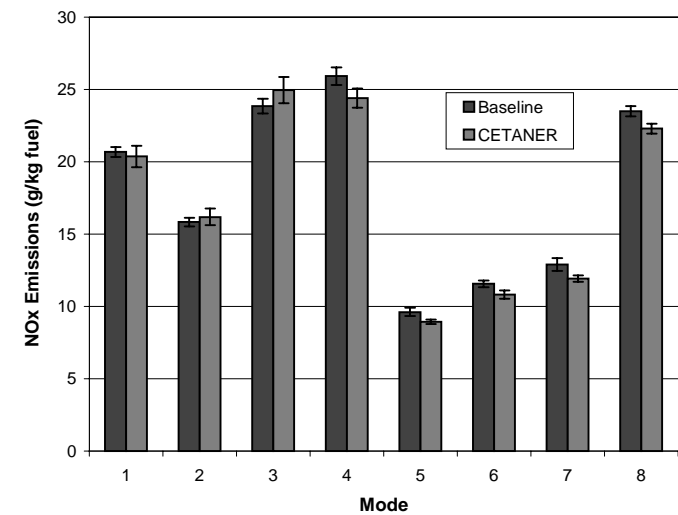
Figure 5. NOx Emissions per Unit Fuel Consumed for CETANER™ Addition, g/kg Fuel Basis.
