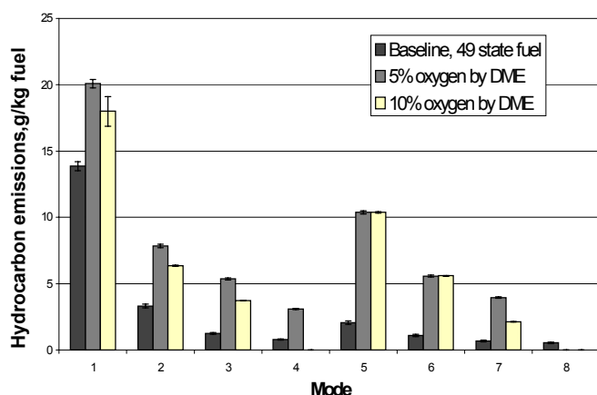
Figure 7. Hydrocarbon Emission Results per unit fuel consumed, g/ kg fuel
