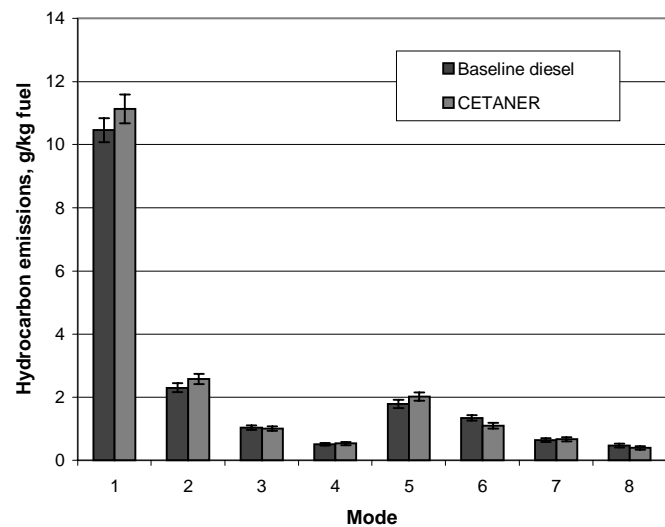
Figure 8. Total Hydrocarbon Emissions per Unit Fuel Consumed for CETANER™ Addition, g/kg fuel
