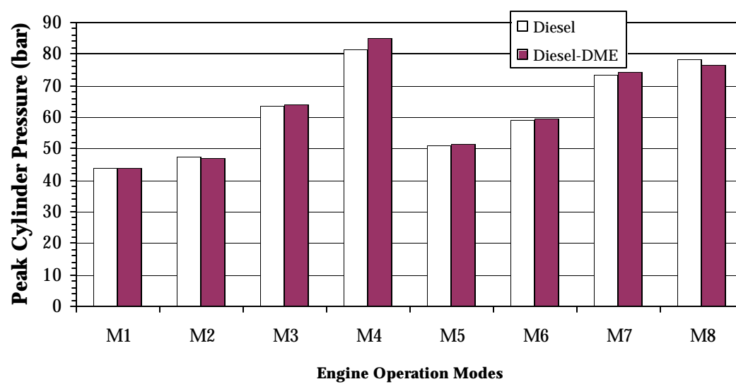
Figure 4-15: Peak Cylinder Pressure Comparison
