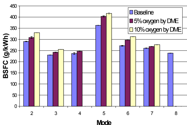
Figure 8. Brake Specific Fuel Consumption (BSFC)
