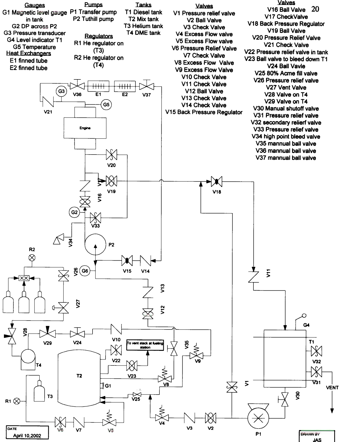
Figure 11. Schematic diagram of DME-diesel fueling system on the shuttle bus
