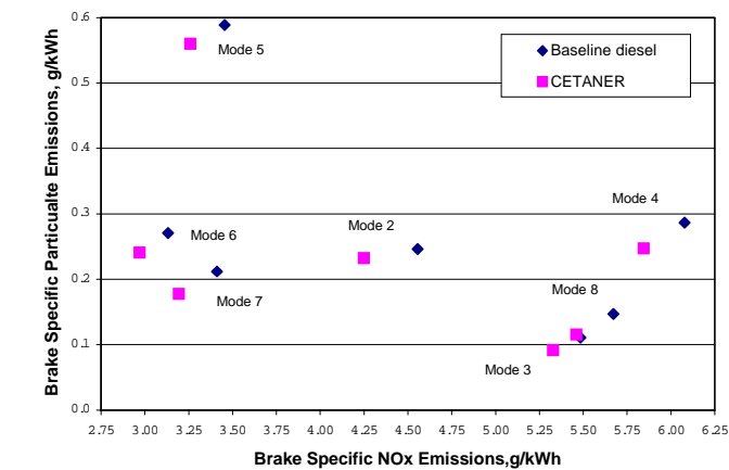
Figure 6. Brake-Specific Particulate Emission vs. NOx Emission Tradeoff.
