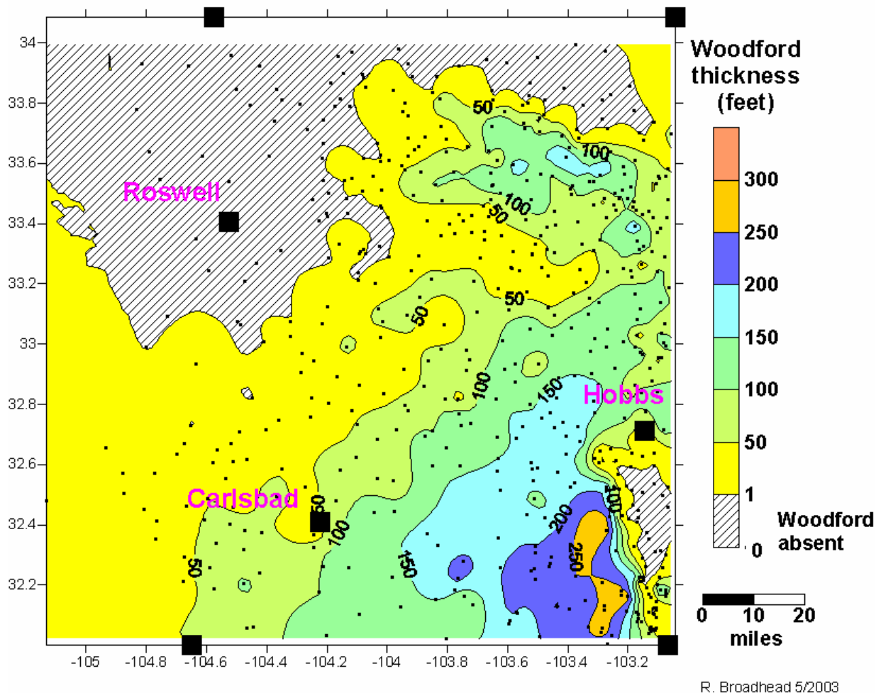
Fig. 70. Pseudo-corrected thickness map of Woodford Shale in southeastern New Mexico, constructed with same data used in Fig. 69 except that wells that encountered obvious steeply dipping Woodford were removed from database. This map more accurately portrays the true thickness of the Woodford than the map in Fig. 69.
