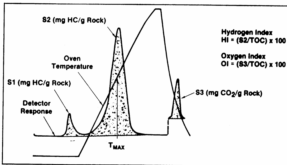
Fig. 75. Schematic of Rock-Eval pyrogram showing the evolution of organic compounds evolved from source rock during heating. Important parameters used for determination of thermal maturity are S_1 , S_2 , and T_{MAX} . From Peters (1986).
