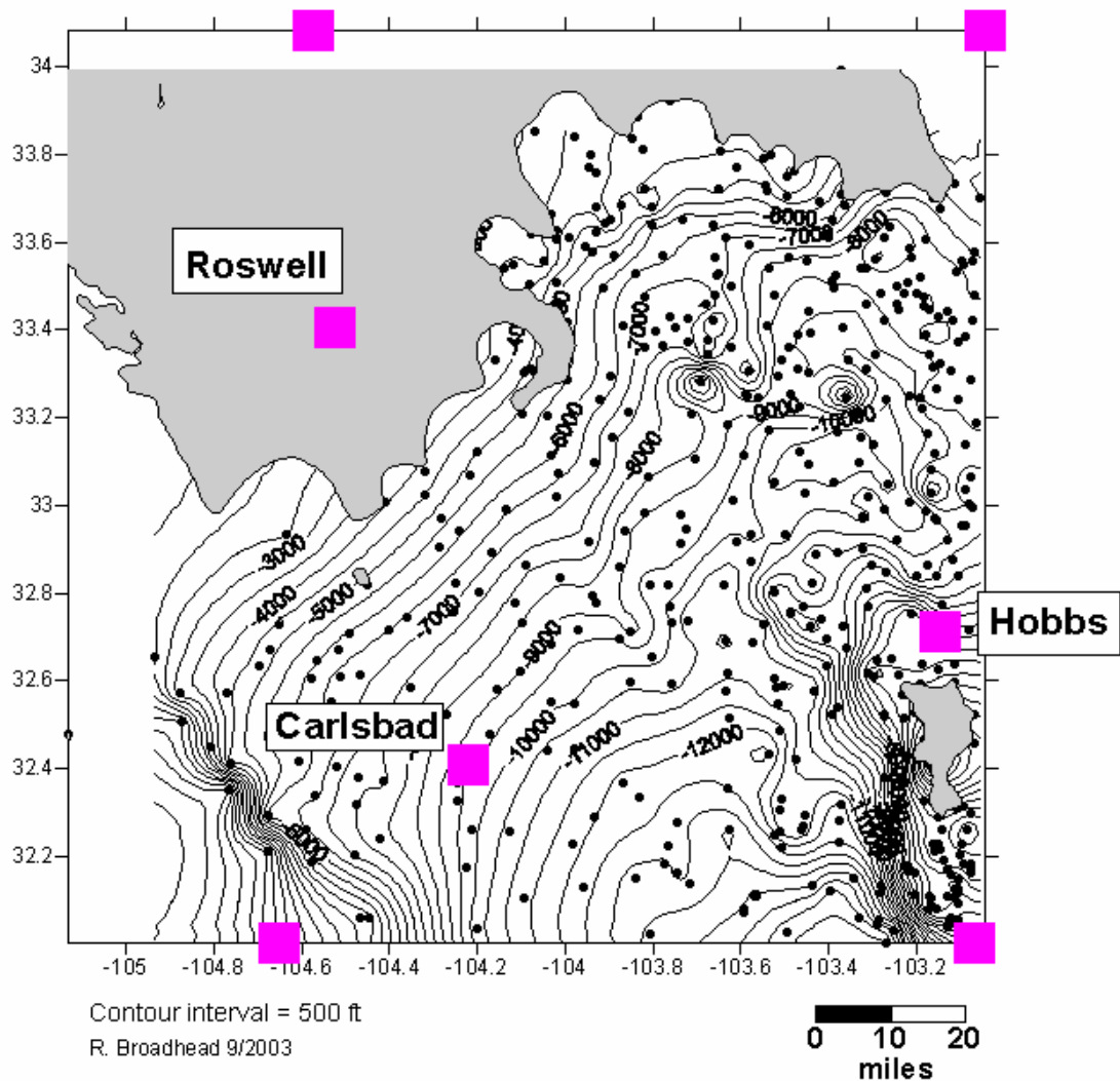
Fig. 64. Structure contour map of the top of the Siluro-Devonian carbonates in southeastern New Mexico. Dots are well control points developed in this project.
