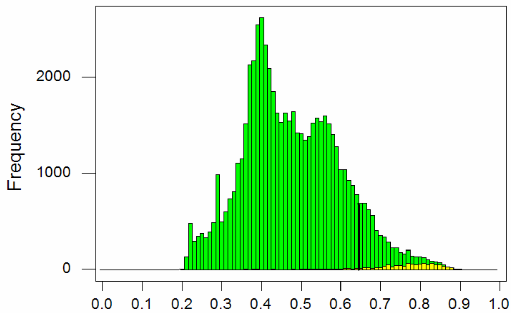
Fig. 54. Histogram of the estimates for the entire system (green) and the estimates for the successful wells (yellow).
