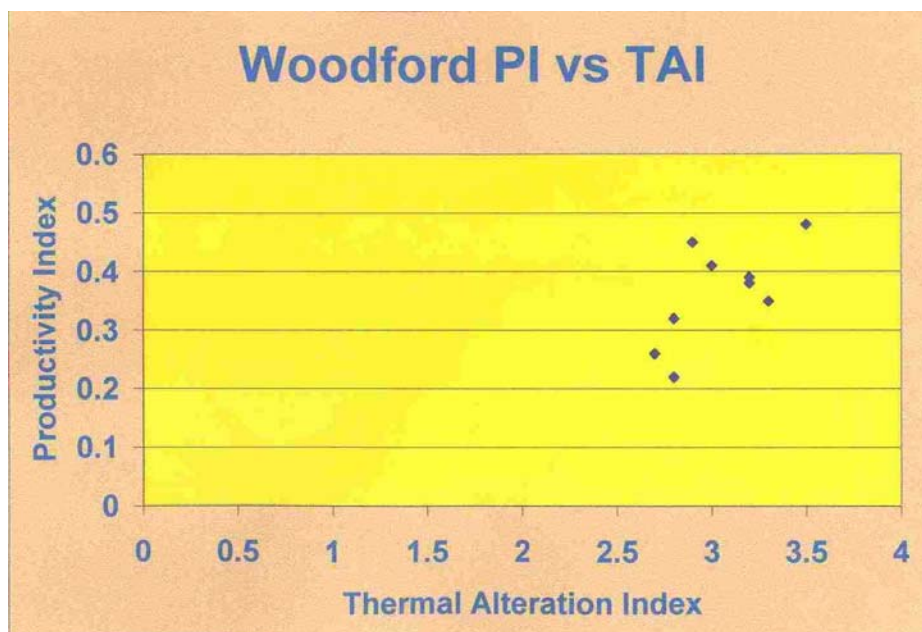
Fig. 78. Plot of Rock-Eval Productivity Index (PI) versus the Thermal Alteration Index (TAI) for samples of Woodford Shale in southeastern New Mexico. Note that as TAI increases, PI also increases, which is the trend expected because both parameters should increase as a function of thermal maturity.
