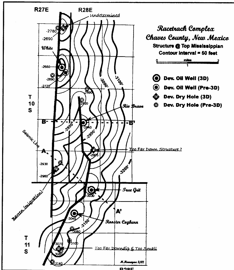
Fig. 62. Structure contours on top of the Mississippian limestones, Racetrack complex, Chaves County New Mexico. This structure is representative of productive structures that trap oil in Siluro-Devonian reservoirs.
