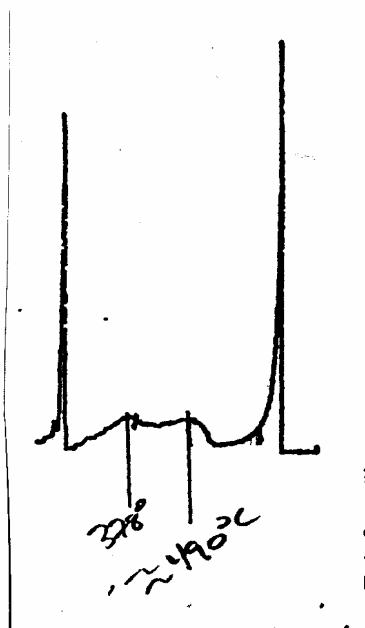
Fig. 79. Rock-Eval pyrogram for a sample of Woodford Shale, showing the bimodal S_2 peak which causes the instrument-derived TMAX values to be incorrect for the Woodford in this area.
