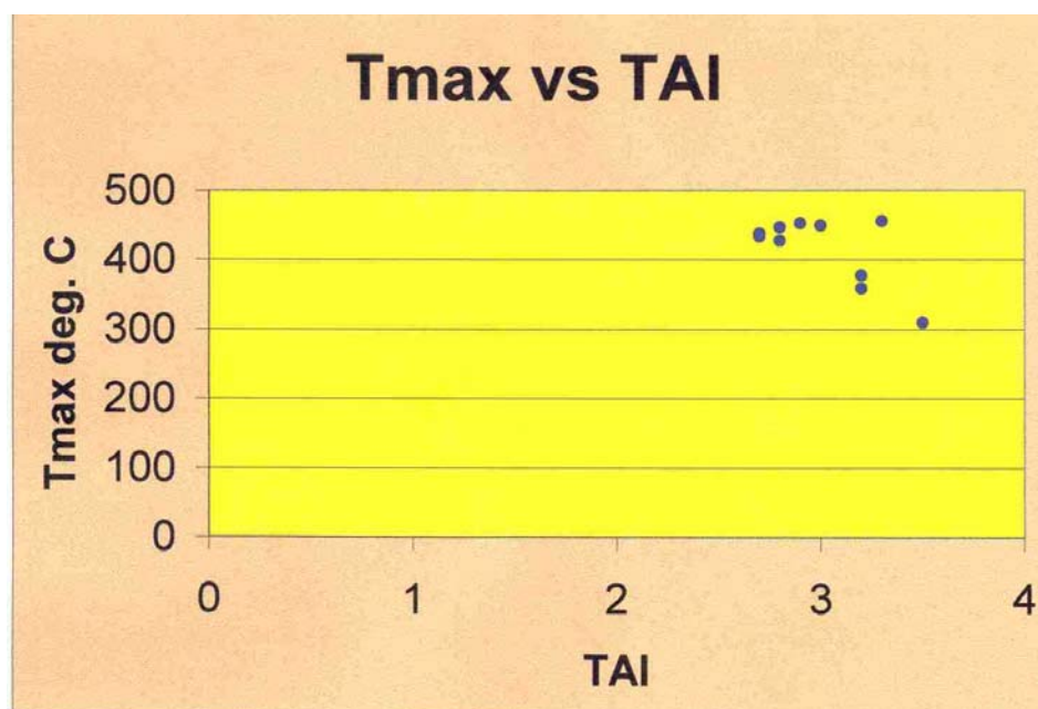
Fig. 77. Plot of Rock-Eval TMAX versus the Thermal Alteration Index (TAI) of kerogen for samples of the Woodford Shale in southeastern New Mexico. Note that as TAI increases, TMAX decreases, a trend opposite to what is expected as both parameters should increase as a function of increasing thermal maturity.
