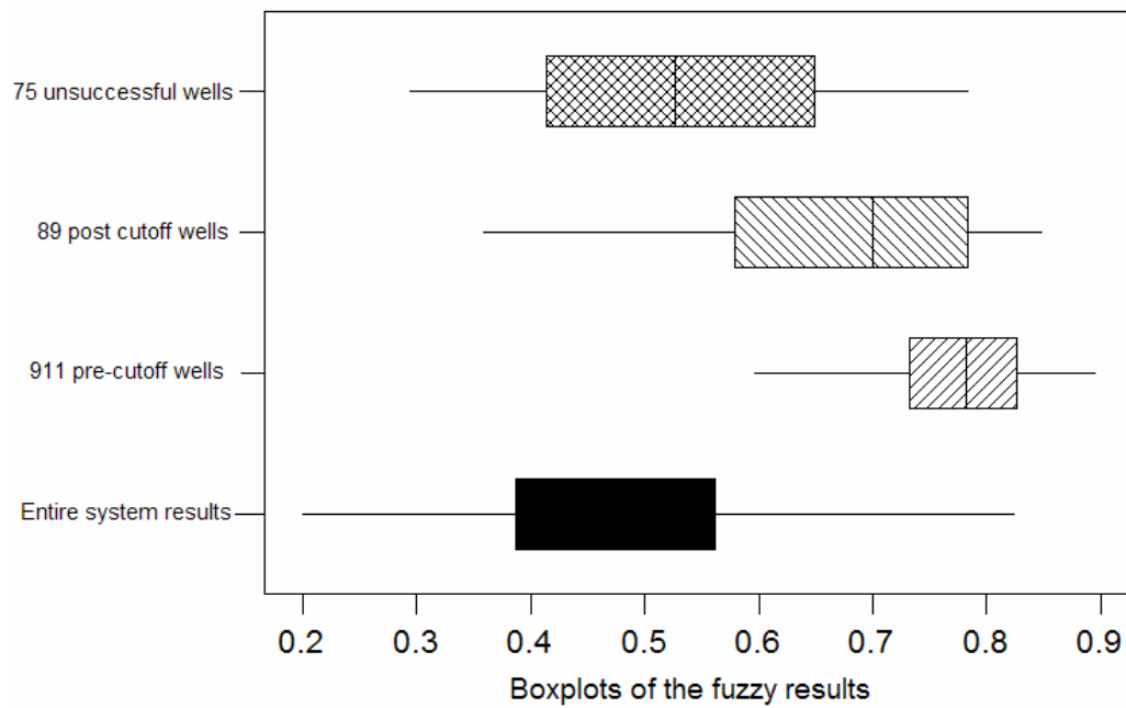
Fig. 53. Boxplots for the entire system and the three subsets.
