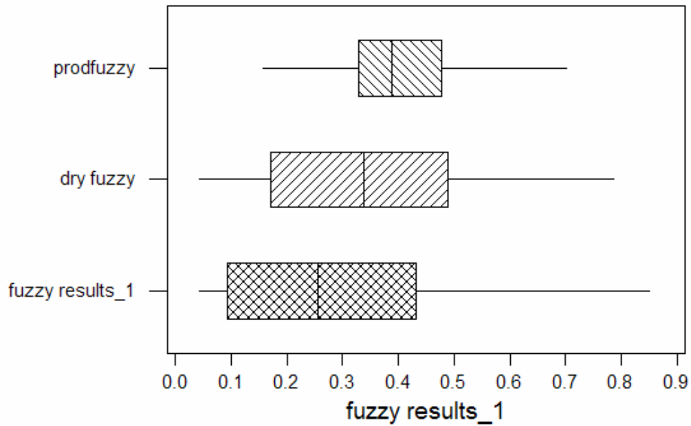
Fig. 58. Boxplot of the fuzzy results for prodfuzzy (set of producing wells), dry fuzzy (set of unsuccessful wells) and fuzzy results_1 (estimates for the entire system).
