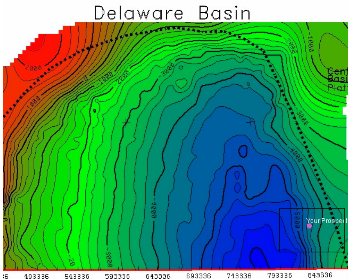
Fig. 28. Delaware Basin structure map.
