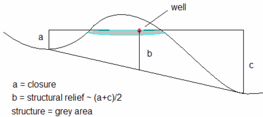
Fig. 55. Graphical representation of the variables: closure, structure and structural relief.
