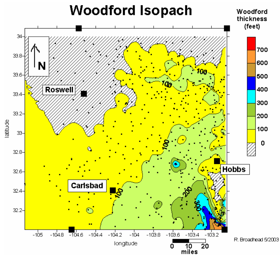
Fig. 69. Isopach map of Woodford Shale in southeastern New Mexico.
