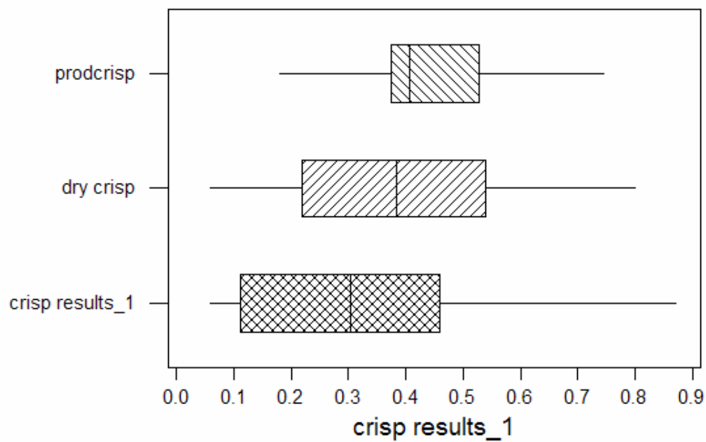
Fig. 57. Boxplot of the crisp results for prodcrisp (set of producing wells), dry crisp (set of unsuccessful wells) and crisp results_1 (estimates for the entire system).
