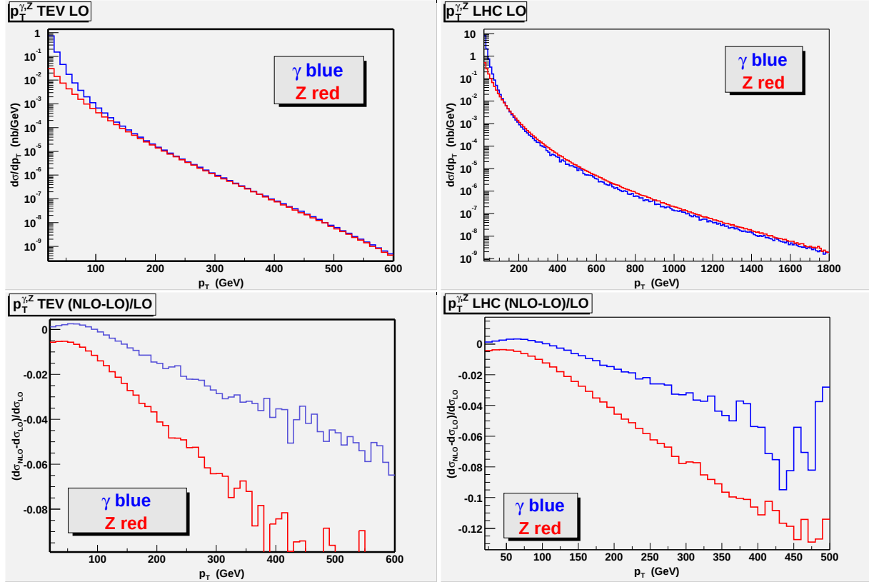
Fig. 55: The LO results through \mathcal{O}(\alpha_S \alpha_{EW}) for the \gamma - and Z -production cross sections at Tevatron and LHC, as a function of the transverse momentum (top) as well as the size of the NLO corrections through \mathcal{O}(\alpha_S \alpha_{EW}^2) relatively to the former.
