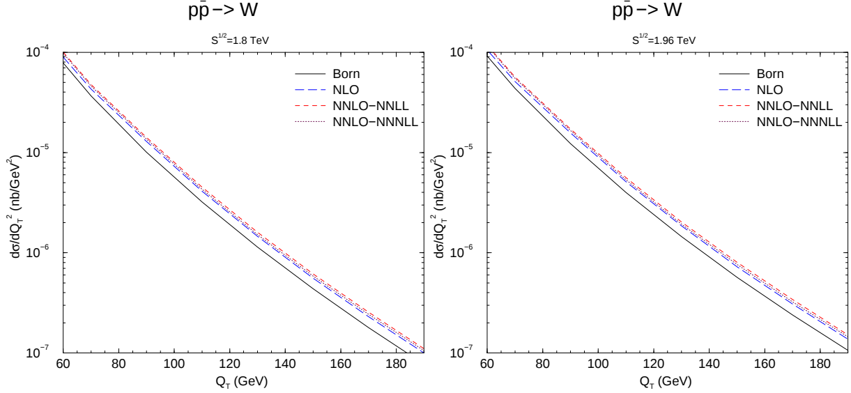
Fig. 27: The differential cross section, d\sigma/dQ_T^2 , for W hadroproduction in p\bar{p} collisions at the Tevatron at (left) \sqrt{S} = 1.8 TeV and (right) 1.96 TeV, with \mu_F = \mu_R = Q_T . Shown are the Born, NLO, NNLO-NNLL, and NNLO-NNNLL results.
