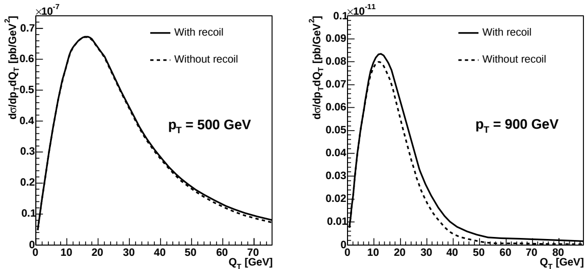
Fig. 32: The Q_T profile for two p_T values.
