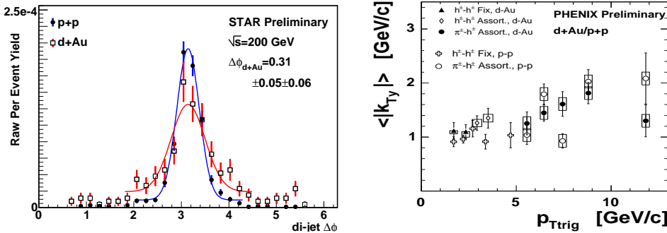
Figure 2. Left: Di-jet \Delta\phi distribution in p+p and d+Au collisions at \sqrt{s}=200 GeV from STAR [15]. Right: Variation of \langle |k_{Ty}| \rangle with p_{T,trigger} measured by PHENIX [16].
