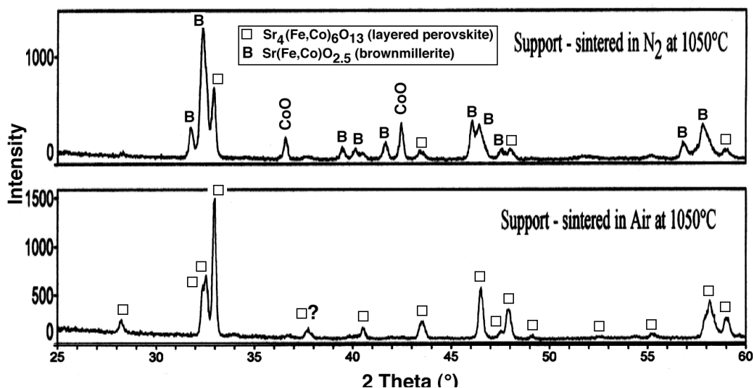
Fig. 4. X-ray diffraction data for \text{SrCo}_{0.5}\text{FeO}_x supports after sintering in air and nitrogen at 1050 °C.
