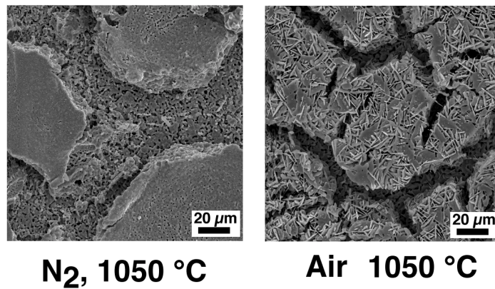
Fig. 11. Relatively low magnification scanning electron micrographs of \text{SrCo}_{0.5}\text{FeO}_x films sintered in \text{N}_2 and air at 1050 °C.
