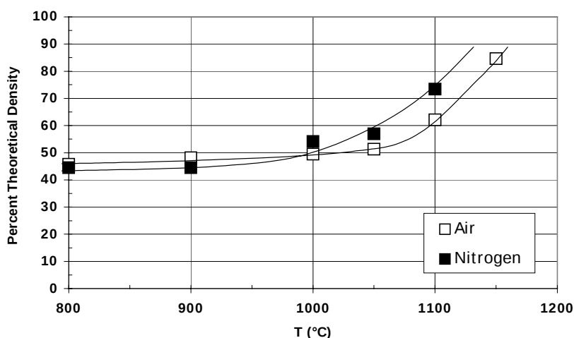
Fig. 2. Densification of \text{SrCo}_{0.5}\text{FeO}_x supports as a function of sintering temperature and atmosphere.
