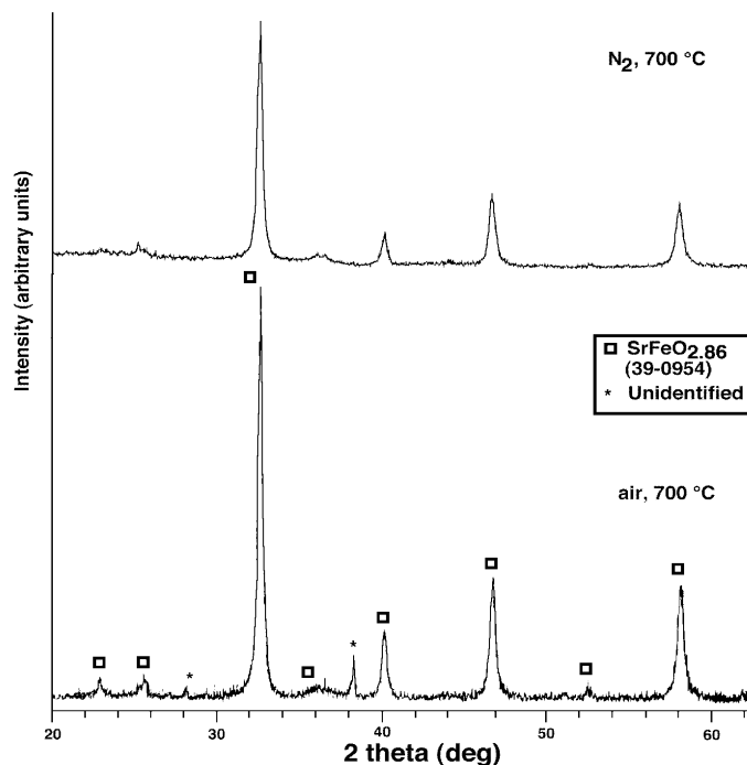
Fig. 7. X-Ray diffraction result for \text{SrCo}_{0.5}\text{FeO}_x powders made by aerosol pyrolysis using air and \text{N}_2 as carrier gas.
