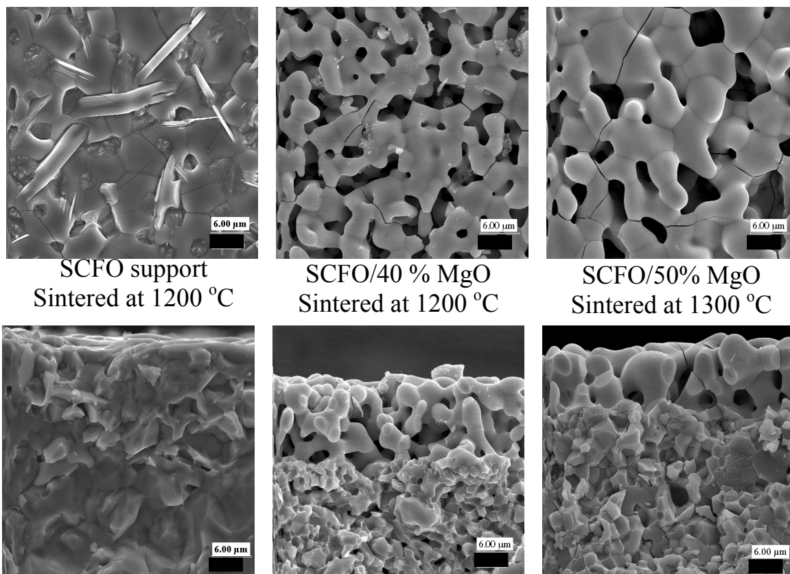
Fig. 5. Sintering of \text{SrCo}_{0.5}\text{FeO}_x films on composite MgO/SCFO supports compared to sintering on a pure SCFO support.
