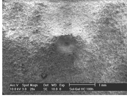
Fig.4 SEM image showing no cracks and spalling of YSZ in YSZ/ \text{Al}_2\text{O}_3 overlay( 2\ \mu\text{m} ) system after hot corrosion of 100 h.
