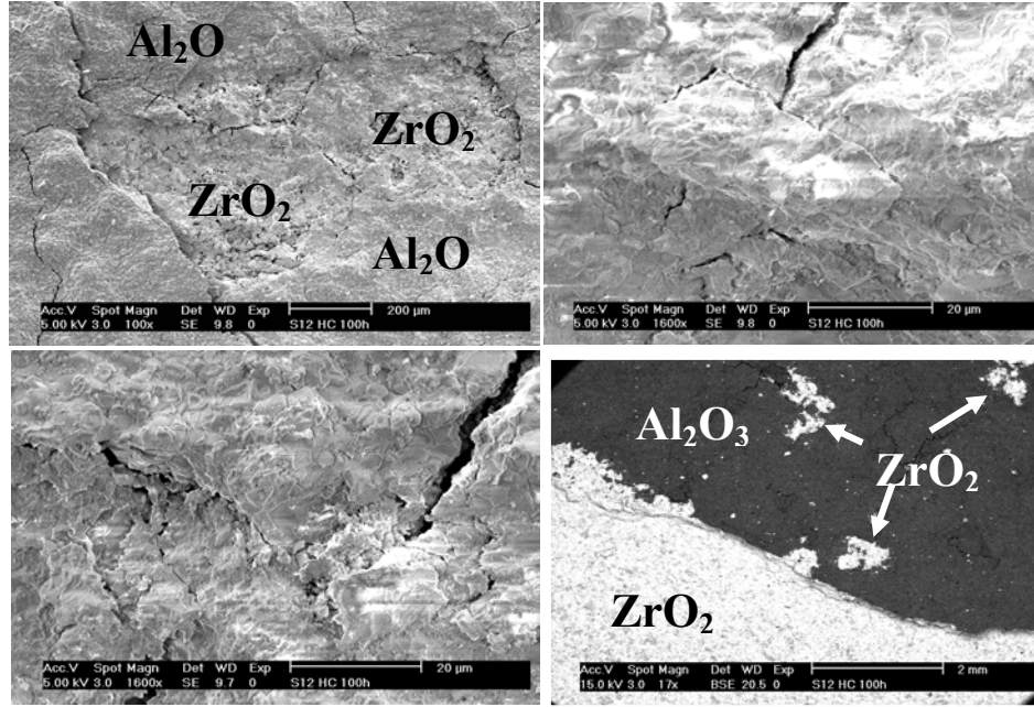
Fig.2 SEM images showing the formation of cracks and spalling of YSZ after hot corrosion for ~100 h in composite YSZ/ \text{Al}_2\text{O}_3 overlay ( 25\ \mu\text{m} ) system.
