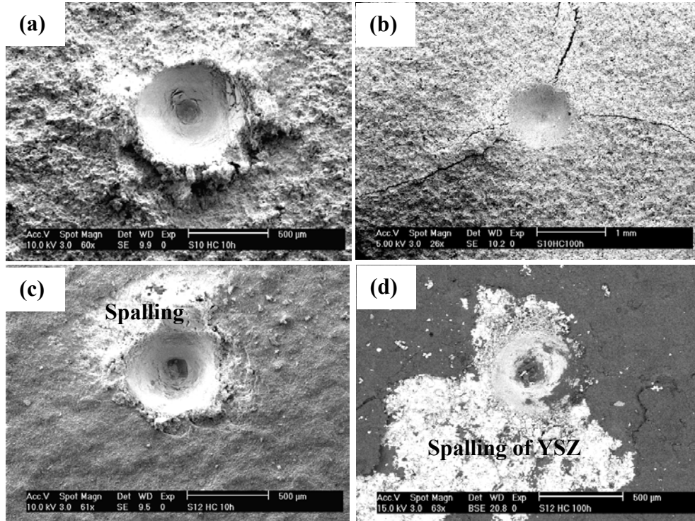
Fig.2 SEM images showing the formation of cracks and spalling of YSZ after hot corrosion for ~100 h in composite YSZ/ \text{Al}_2\text{O}_3 overlay ( 25\ \mu\text{m} ) system.
