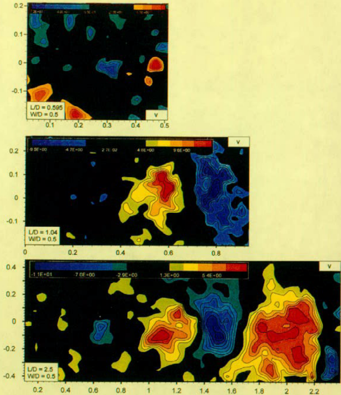
Figure 5c: Comparison of patterns of instantaneous transverse velocity v as a function of cavity length L at a constant value of cavity depth W , both of which are normalized by diameter D of the inflow pipe. For the top, middle, and bottom images, the minimum negative and positive levels of velocity are \bar{v}_{\min} = -0.9, -3.1, -2.9 m/sec and \bar{v}_{\max} = 4.2, 4.8, 1.3 m/sec and the incremental values are \Delta v = 1.1, 1.6 , and 1.4 m/sec.
