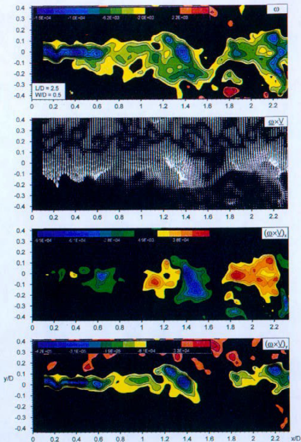
Figure 10c: Representations of the hydrodynamic contribution to the acoustic power integral for the case of a long cavity represented by a larger value of the cavity length L , normalized with respect to the diameter D of the inflow pipe. In the images, the minimum values of the contours are (\omega)_{\min} = -2000 \text{ sec}^{-1} ; [(\omega \times V)_x]_{\min} = -6100 \text{ m/sec}^2 ; [(\omega \times V)_x]_{\max} = 15900 \text{ m/sec}^2 ; [(\omega \times V)_y]_{\min} = -81000 \text{ m/sec}^2 ; and [(\omega \times V)_y]_{\max} = 33000 \text{ m/sec}^2 ; the corresponding incremental values are \Delta\omega = 1400 \text{ sec}^{-1} , \Delta(\omega \times V)_x = 11000 \text{ m/sec}^2 , and \Delta(\omega \times V)_y = 36333 \text{ m/sec}^2 .
