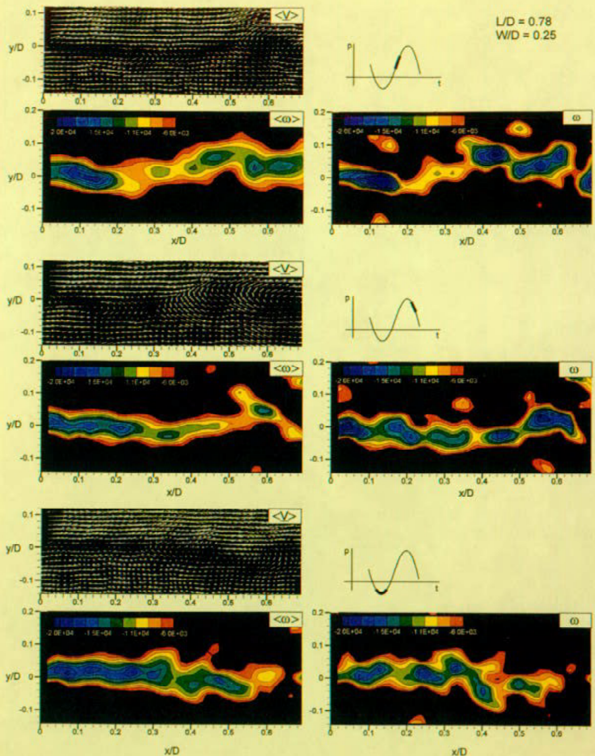
Figure 7: Patterns of phase-averaged velocity \langle V \rangle and vorticity \langle \omega \rangle , along with corresponding instantaneous representations of vorticity \omega for three different values of phase during the oscillation cycle. Dimensionless cavity length is L/D = 0.778 and cavity depth W/D = 0.25 , in which D is the diameter of the inflow pipe. For all images, the minimum contour level is \omega_{\min} = -6000 \text{ s}^{-1} , and the incremental value is \Delta\omega = 1333 \text{ s}^{-1} .
