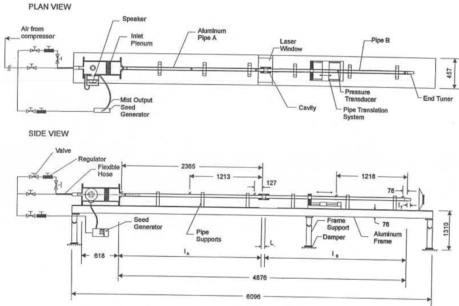
Figure 1: Overview of pipeline-cavity system. (From Rockwell et al. , 2002)
