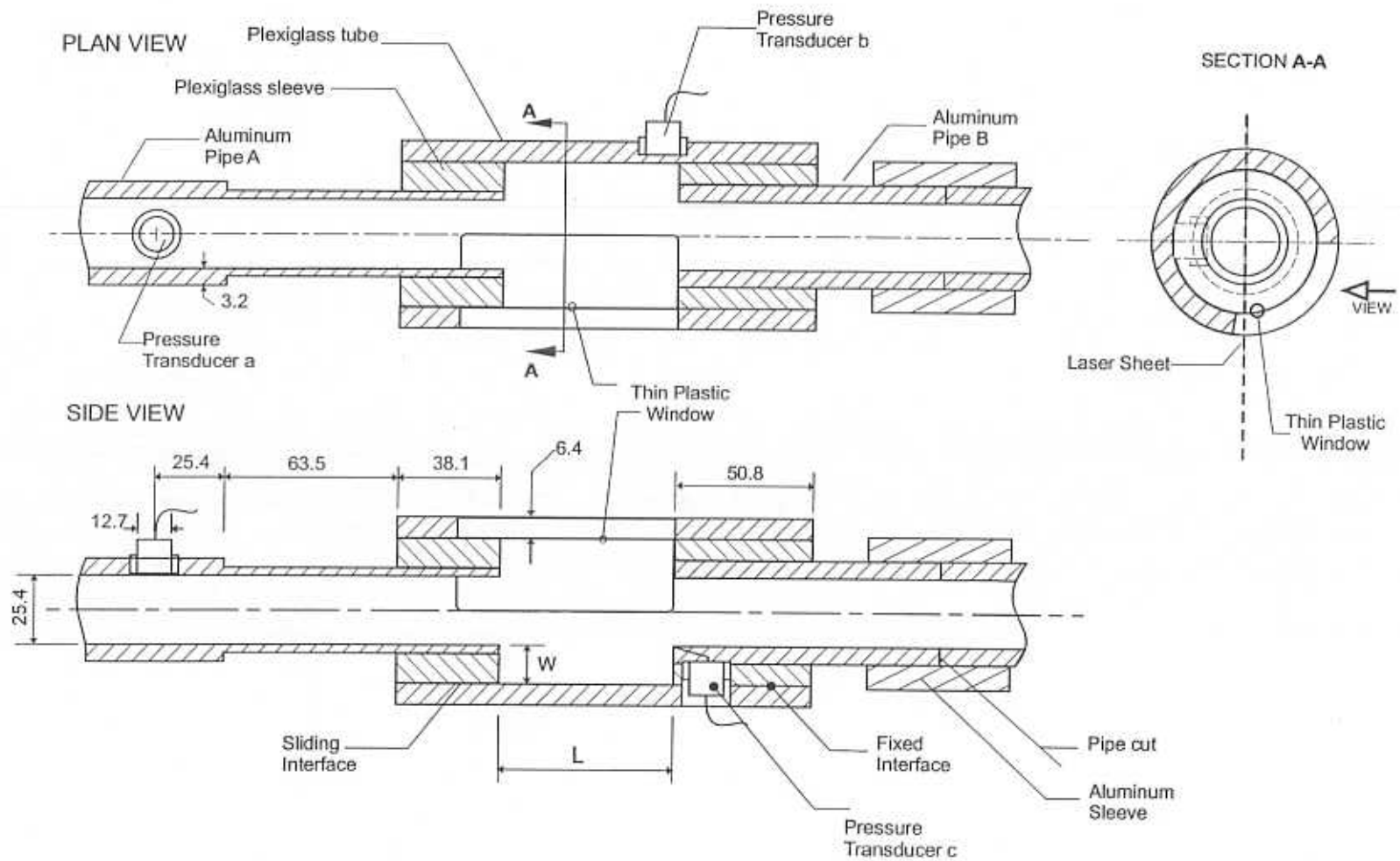
Figure 2: Cavity subsystem employed for PIV imaging. (From Geveci et al. , 2002)
