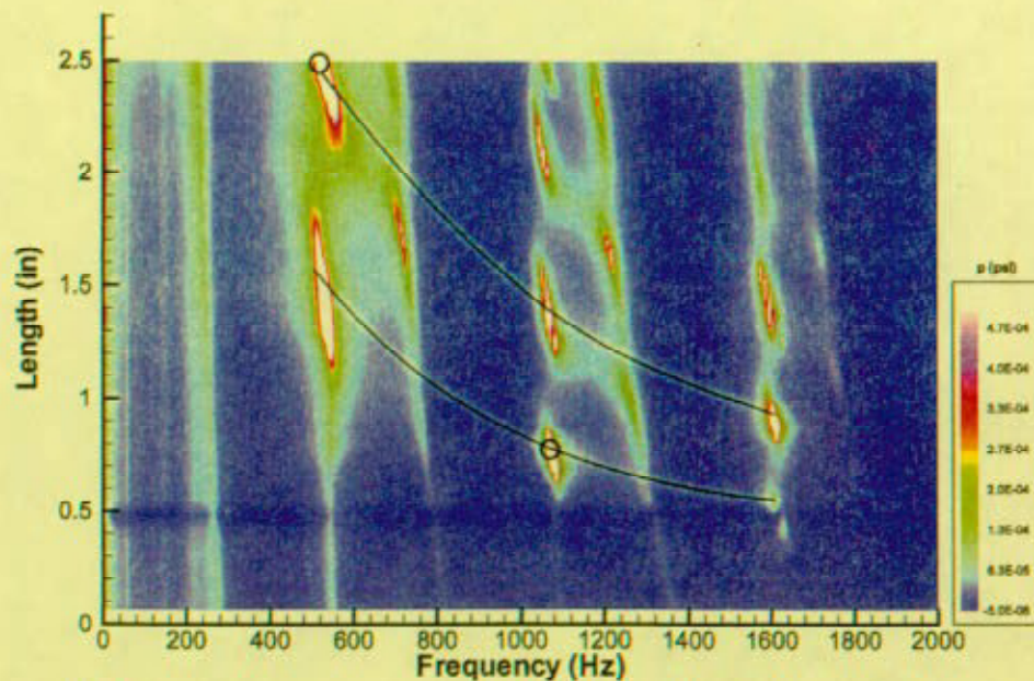
Figure 3b: Isometric view (top image) and plan view (bottom image) of pressure amplitude as a function of frequency and cavity length. Lines shown on plan view represent fits through peak values of pressure amplitude. (Based on plots of Oshkai, Rockwell, and Pollack, 2002.)
