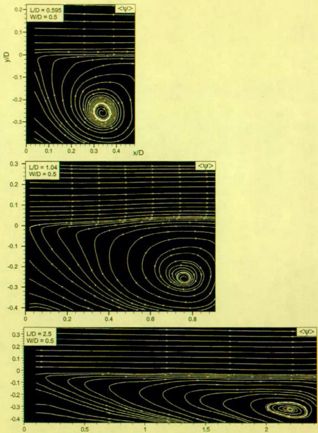
Figure 4a: Comparison of time-averaged streamline patterns as a function of cavity length L for a constant value of cavity depth W , both of which are normalized by the diameter D of the inflow pipe. Inflow velocity is U = 39.62 m/sec for top, middle and bottom images.
