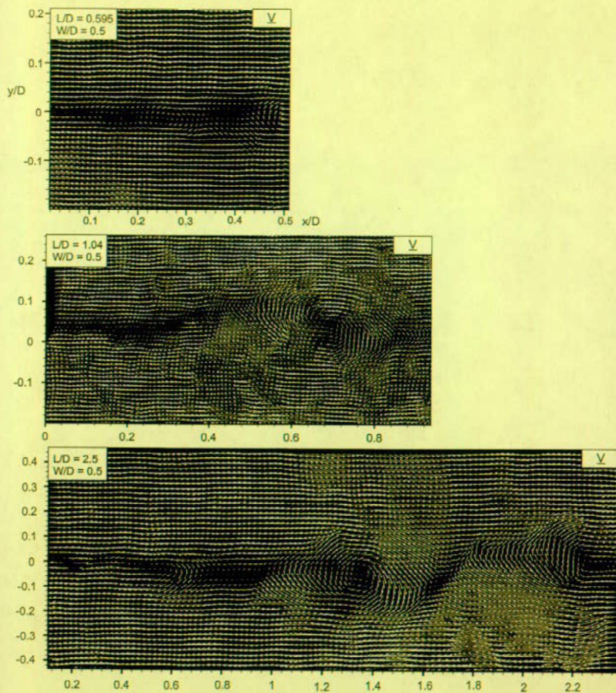
Figure 5b: Comparison of patterns of instantaneous velocity vectors \underline{V} as a function of cavity length L at a constant value of cavity depth W , both of which are normalized by diameter D of the inflow pipe.
