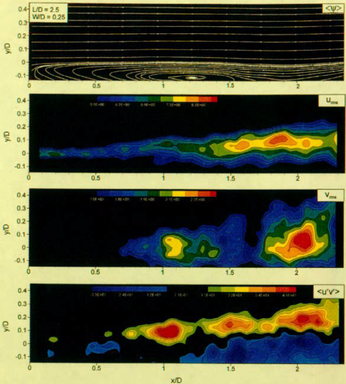
Figure 8a: Time-averaged representations of the unsteady shear layer along the cavity for a relatively long cavity of length L/D = 2.5 and shallow depth W/D = 0.25 . The minimum values of the contours in each of the images are: (u_{rms})_{min} = 5.5 m/sec; (v_{rms})_{min} = 1.6 m/sec; (\langle u'v' \rangle)_{min} = -9.6 m 2 /sec 2 ; and (\langle u'v' \rangle)_{max} = 11 m 2 /sec 2 . Corresponding incremental values of contours are \Delta u_{rms} = 0.35 m/sec, \Delta v_{rms} = 0.1 m/sec, and \Delta \langle u'v' \rangle = 6 m 2 /sec 2 .
