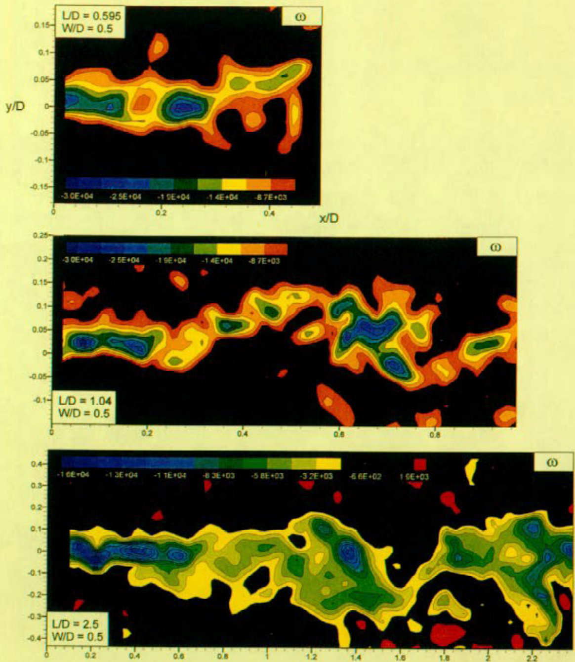
Figure 5a: Comparison of patterns of instantaneous vorticity as a function of cavity length L at a constant value of cavity depth W , both of which are normalized by diameter D of the inflow pipe. For the top, middle, and bottom images, the minimum levels of vorticity \omega_{\min} = -8700 , -8700 , and -1900 \text{ sec}^{-1} and the incremental values are 2650 , 2650 , and 1300 \text{ sec}^{-1} .
