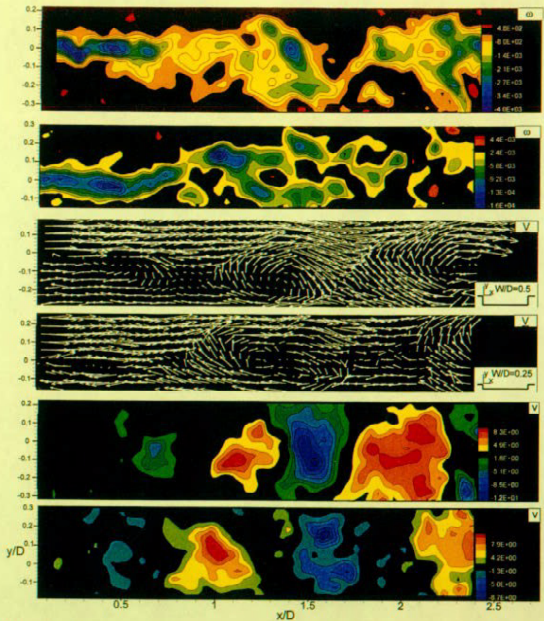
Figure 8b: Direct comparison of instantaneous flow structure along a relatively long cavity L/D = 2.5 for moderate depth W/D = 0.5 and shallow depth W/D = 0.25 . For the former case, the flow structure is predominantly locked-on, while for the latter, it exhibits substantial intermittency, and the selected images correspond to a locally sinusoidal oscillation. For the contours of constant vorticity \omega , the minimum levels are \omega_{\min} = -500 \text{ s}^{-1} and -2400 \text{ s}^{-1} for the top and bottom images respectively. The corresponding incremental values are \Delta\omega = 300 and 1700 \text{ s}^{-1} . For the bottom set of images, the minimum negative and positive contour levels are (v)_{\min}^- = -1.8 \text{ m/sec} , (v)_{\min}^+ = 3.1 \text{ m/sec} , and (v)_{\min}^- = -1.3 \text{ m/sec} , (v)_{\min}^+ = 2.3 \text{ m/sec} for the upper and lower images respectively, and the corresponding incremental values are \Delta v = 1.7 and 1.9 \text{ m/sec} respectively.
