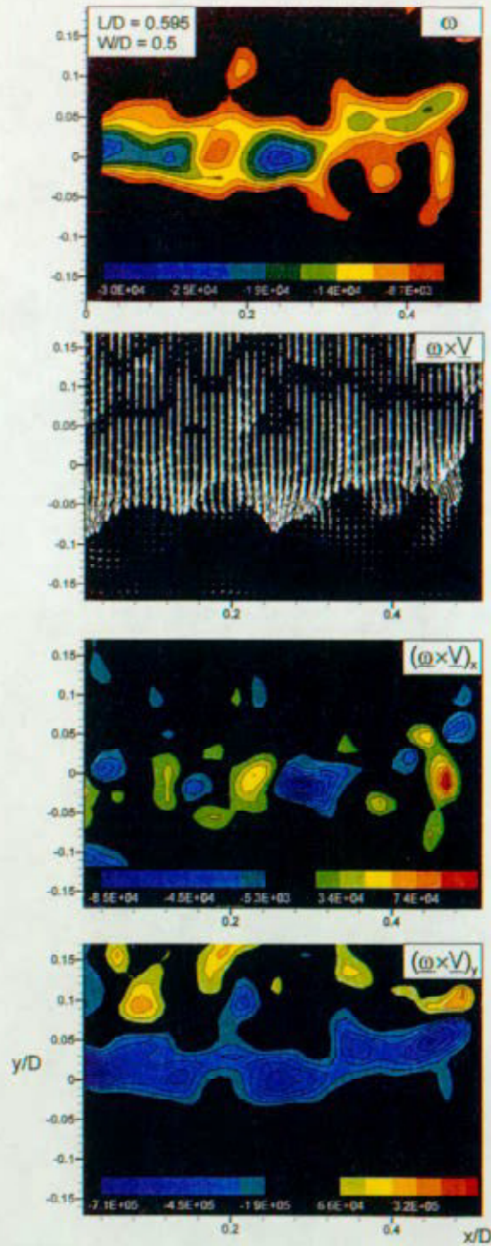
Figure 10a: Representations of the hydrodynamic contribution to the acoustic power integral for the case of a relatively short cavity represented by a relatively small value of L , normalized with respect to the diameter D of the inflow pipe. In the images, the minimum values of the contours are (\omega)_{\min} = -8700 \text{ sec}^{-1} ; [(\omega \times V)_x]_{\min} = -5300 \text{ m/sec}^2 ; [(\omega \times V)_y]_{\min} = 20667 \text{ m/sec}^2 ; [(\omega \times V)_z]_{\min} = -190000 \text{ m/sec}^2 ; and [(\omega \times V)_x]_{\min} = 66000 \text{ m/sec}^2 ; the corresponding incremental values are \Delta\omega = 2650 \text{ sec}^{-1} , \Delta(\omega \times V)_x = 13333 \text{ m/sec}^2 , and \Delta(\omega \times V)_y = 84667 \text{ m/sec}^2 .
