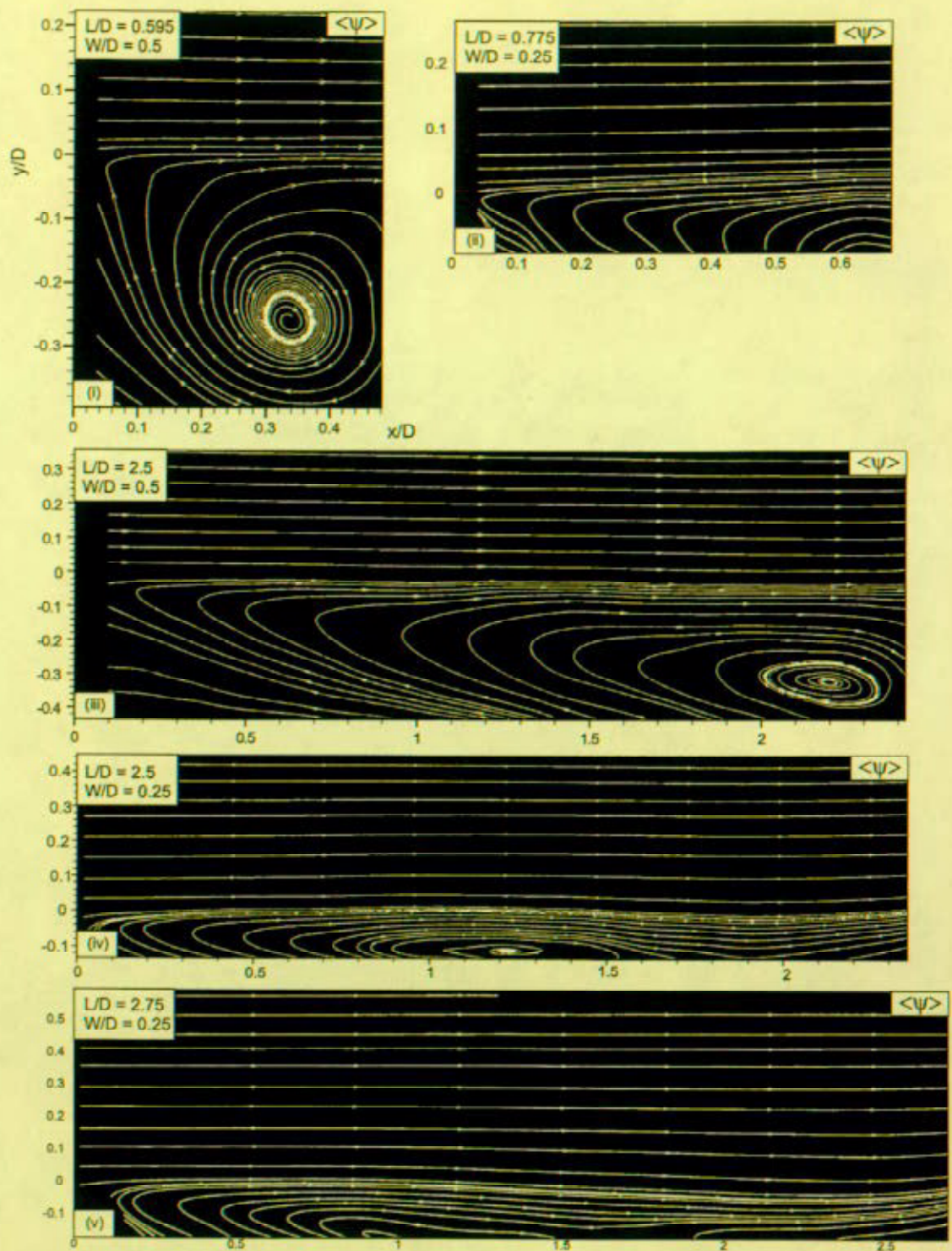
Figure 6: Comparison of time-averaged streamline patterns showing effect of cavity depth W for relatively short and long cavities, represented by small and large values of cavity length L . Length L and depth W are normalized with respect to the inflow pipe diameter D . For all images, the inflow velocity is in the range of 35.97 to 39.62 m/sec.
