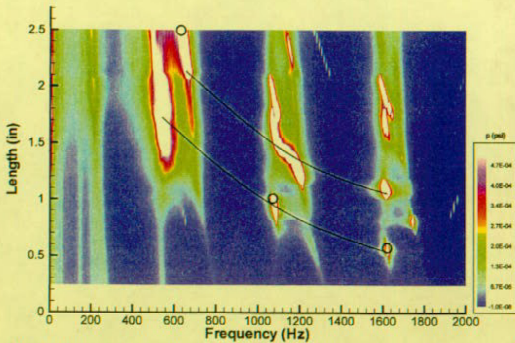
Figure 3a: Isometric view (top image) and plan view (bottom image) of pressure amplitude as a function of frequency and cavity length. Lines shown on plan view represent fits through peak values of pressure amplitude. (Based on plots of Oshkai, Rockwell, and Pollack, 2002.)
