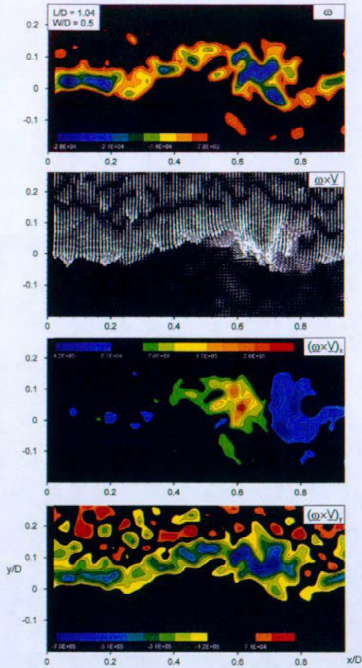
Figure 10b: Representations of the hydrodynamic contribution to the acoustic power integral for the case of an intermediate value of the cavity length L , normalized with respect to the diameter D of the inflow pipe. In the images, the minimum values of the contours are (\omega)_{\min} = -7000 \text{ sec}^{-1} ; [(\omega \times \underline{V})_x]_{\min} = -27000 \text{ m/sec}^2 ; [(\omega \times \underline{V})_y]_{\min} = 36667 \text{ m/sec}^2 ; [(\omega \times \underline{V})_z]_{\min} = -120000 \text{ m/sec}^2 ; and [(\omega \times \underline{V})_x]_{\min} = 71000 \text{ m/sec}^2 ; the corresponding incremental values are \Delta\omega = 2333 \text{ sec}^{-1} , \Delta[(\omega \times \underline{V})_x] = 33333 \text{ m/sec}^2 , and \Delta[(\omega \times \underline{V})_y] = 63333 \text{ m/sec}^2 .
