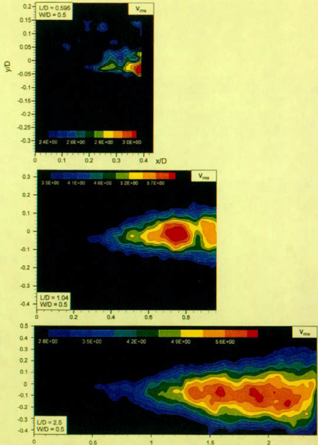
Figure 4b: Comparison of root-mean-square of the transverse velocity fluctuation v_{rms} as a function of cavity length L for a constant value of cavity depth W , both of which are normalized by the diameter D of the inflow pipe. Minimum contour levels are (v_{rms})_{min} = 2.4, 3.5 , and 2.8 m/s, and incremental contour levels are \Delta(v_{rms}) = 0.07, 0.25 , and 0.35 m/s for top, middle and bottom images.
