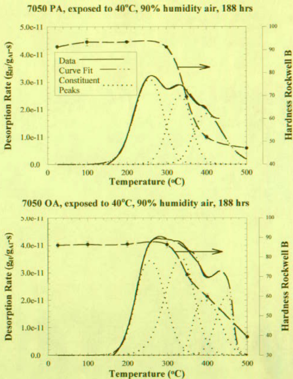
Figure 6. Thermal desorption spectra from peak aged (top) and overaged (bottom) AA 7050. The dashed lines show how the macroscopic hardness changes as the alloy is heated at a rate of 10°C/minute. These results illustrate the thermal instability of the microstructure during the TDS heating cycle.
