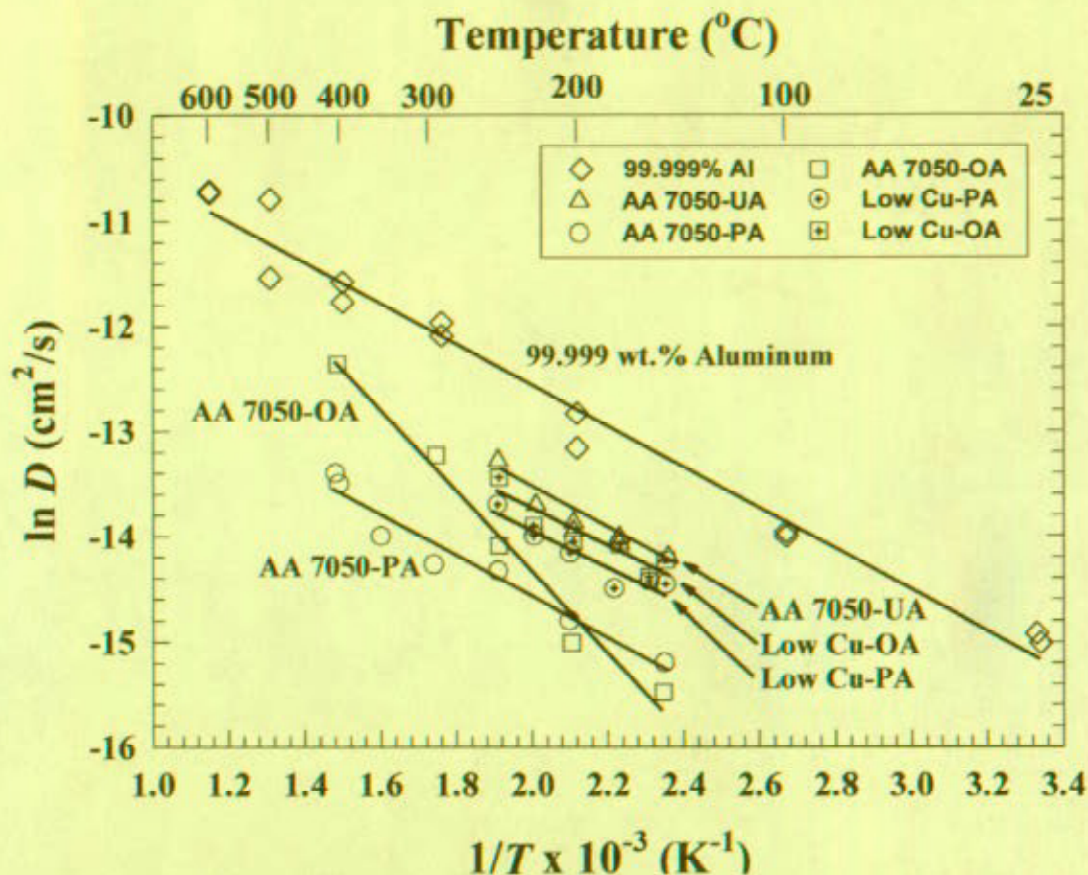
Figure 5. Summary of hydrogen diffusion data for AA 7050 and the low copper variant of the alloy.
