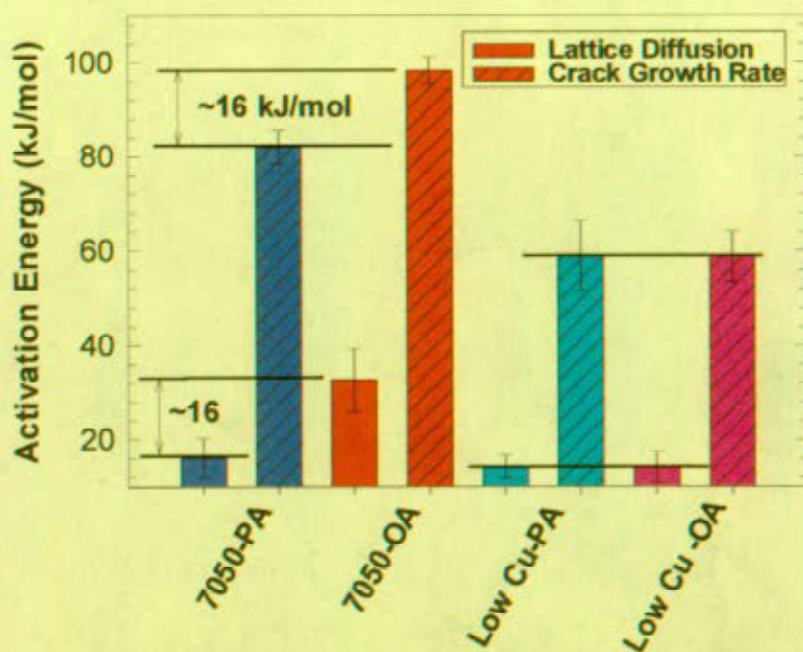
Figure 9. Comparison of the change in the apparent activation energy for stage II crack growth and for hydrogen diffusion. Note that the change for diffusion and crack growth is approximately equal (~16 kJ/mol) for the copper bearing AA 7050 while little change is observed for the low copper alloy.
