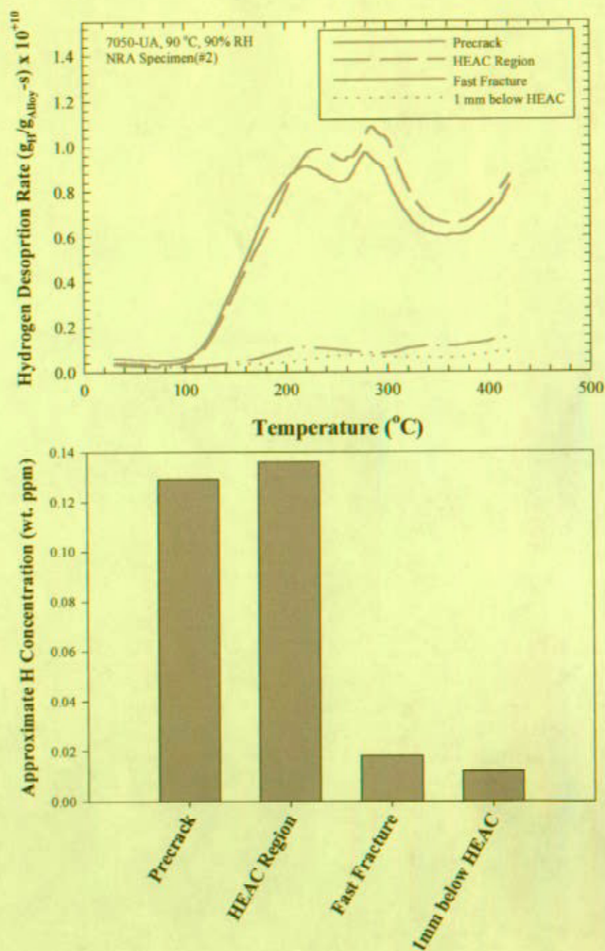
Figure 7. Thermal desorption spectra from crack wakes of AA 7050-UA. Note that the precrack and HEAC regions contain significantly higher hydrogen concentrations than the fast fracture region or a sample taken 1mm below the HEAC region.
