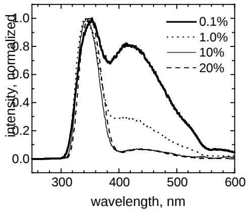
Fig. 3. Optical emission spectra for \text{LaCl}_3 samples with different Ce concentrations. Spectra were normalized with respect to 350 nm peak intensity.
