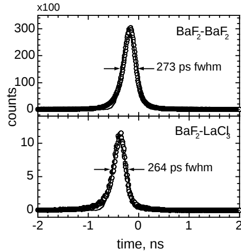
Fig. 6. Coincidence timing resolution results. Above coincidence timing resolution result for two \text{BaF}_2 -PMT detectors, one in start channel and one in stop channel. Below coincidence timing resolution result for a \text{LaCl}_3 -PMT detector in stop channel with a \text{BaF}_2 -PMT detector in start channel.
