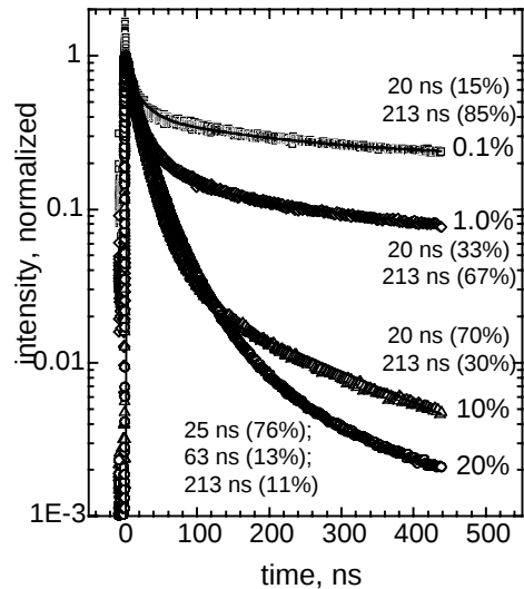
Fig. 4. Time profiles (points) measured for \text{LaCl}_3 crystals with 0.1, 1.0, 10, and 20% Ce concentrations, along with multi-exponential fits (lines). As seen in plots, the principal decay constant is fast ( \leq 25 ns) for samples with high (10-20%) Ce concentration.
