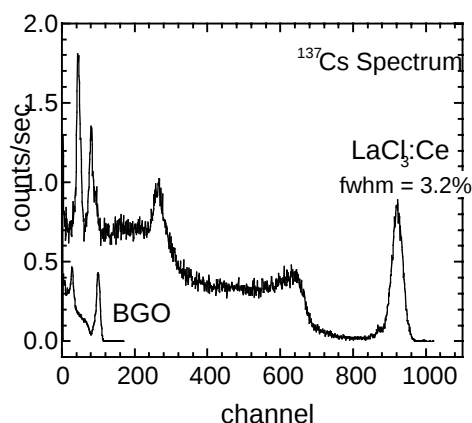
Fig. 1. ^{137}\text{Cs} spectra recorded with \text{LaCl}_3\text{:10%Ce} and BGO crystals coupled to PMT under identical operating conditions. Light output of \text{LaCl}_3\text{:10%Ce} was estimated to be \sim 50,000 photons/MeV from the calibration provided by BGO. The \text{LaCl}_3 spectrum shows resolution of 3.2% (FWHM) at room temperature.
