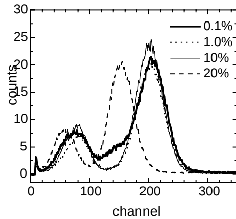
Fig. 2. ^{241}\text{Am} spectra (60 keV photons) recorded with \text{LaCl}_3:\text{Ce} crystals of different Ce concentrations. From the peak position light output was estimated for each crystal, see Table 1.
