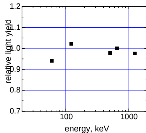
Fig. 5. Energy response (relative light yield, normalized to the value at 662 keV, as a function of energy) for \text{LaCl}_3:10\%\text{Ce} . The response of an ideal material would be independent of energy. Non-proportionality of measured sample is \sim 7\% which is much better than that in established scintillators.
