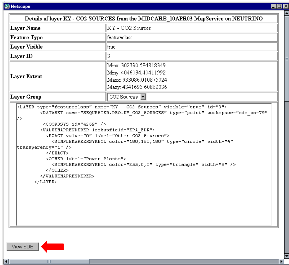
Figure 7 – A view of the ArcXML for the KY- CO2 Sources . ArcXML can be edited. Clicking on the SDE button (red arrow) provides the administrator a view of the coverage (Figure 8).
