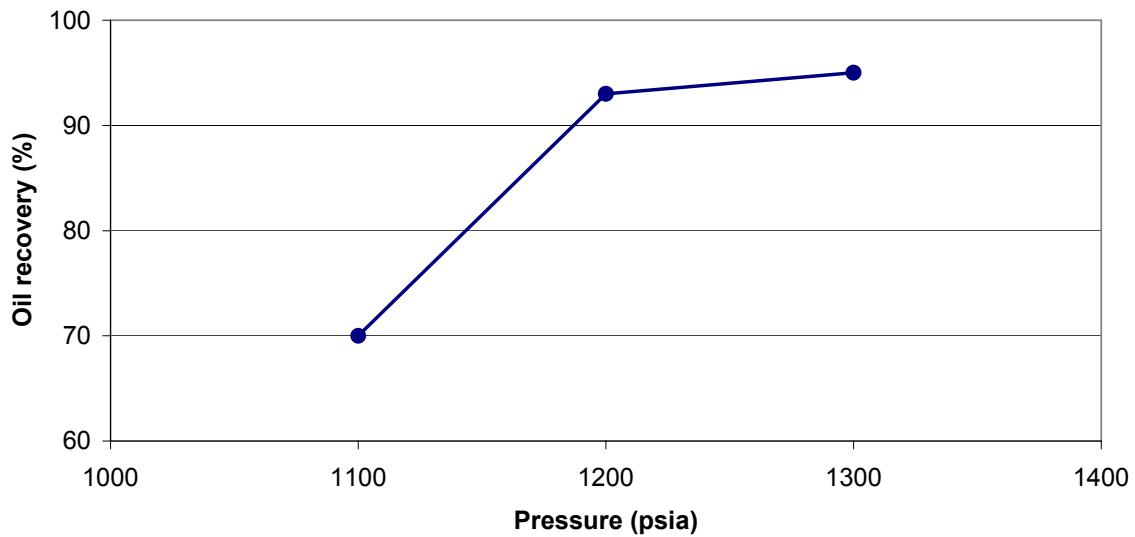
Figure A6 - Oil recovery (at 1.2 HCPV injection of CO 2 ) as a function of pressure for Illinois oil sample at 111 °F.
