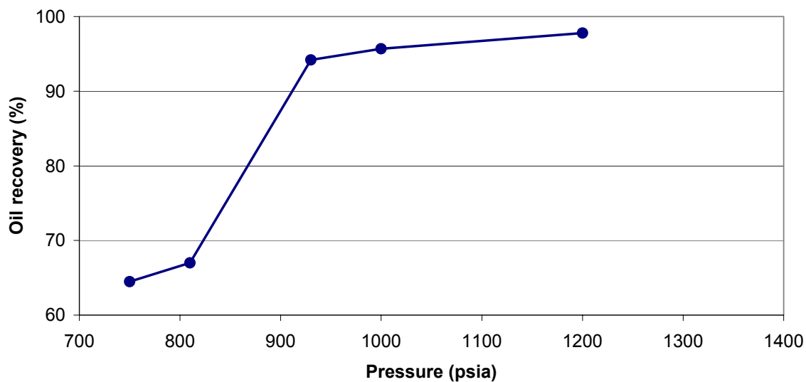
Figure A4 - Oil recovery (at 1.2 HCPV injection of CO 2 ) as a function of pressure for Kentucky oil sample #22 at 79 °F.
