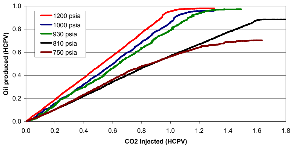
Figure A3 - Oil recovery results in slim-tube experiment with CO 2 displacing Kentucky oil sample #22 at 79 °F.
