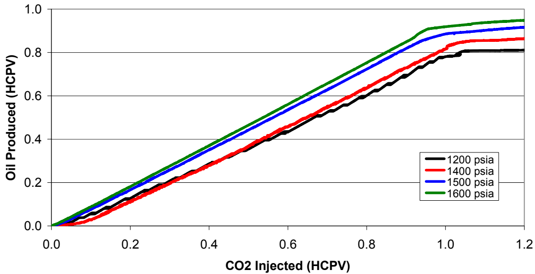
Figure A7 - Oil recovery results in slim-tube experiment with CO 2 displacing Ohio oil sample at 107 °F.
