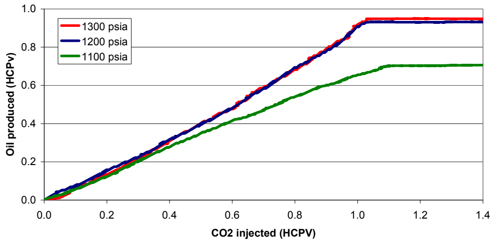
Figure A5 - Oil recovery results in slim-tube experiment with CO 2 displacing Illinois oil sample at 111 °F.
