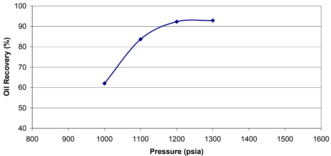
Figure A2 - Ultimate oil recovery as a function of pressure for Indiana oil sample at 101 °F.
