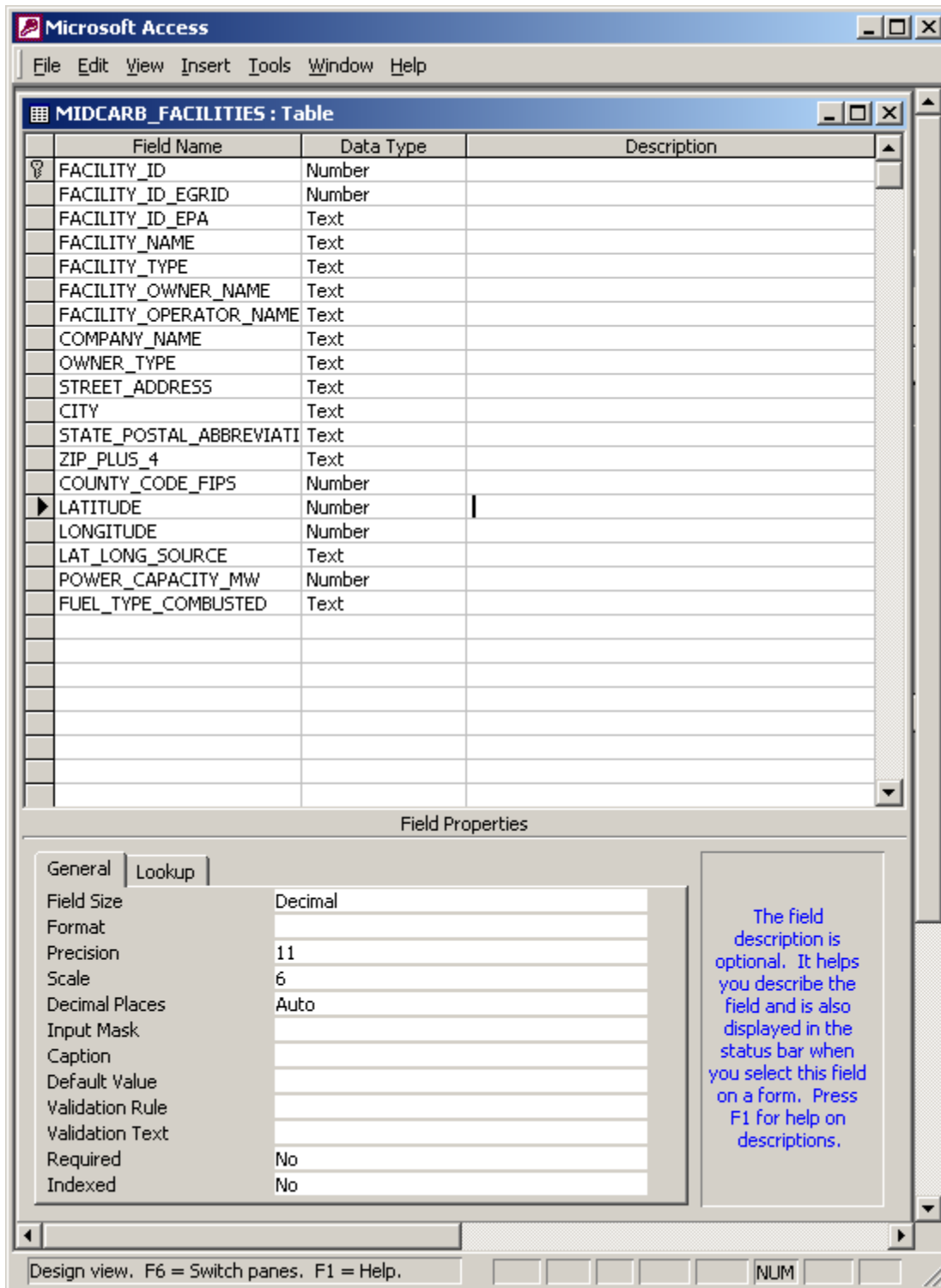
Figure 21 – View of selected data table containing facilities that are major sources of CO 2 emissions in Kansas. A listing of all data tables associated with the RDBMS covering CO 2 emissions in Kansas is provided in Table 2. Similar data tables exist in each of the five states of the MIDCARB Consortium and provide the data that is accessible across all states through the MIDCARB IMS browser and SDE layers.
