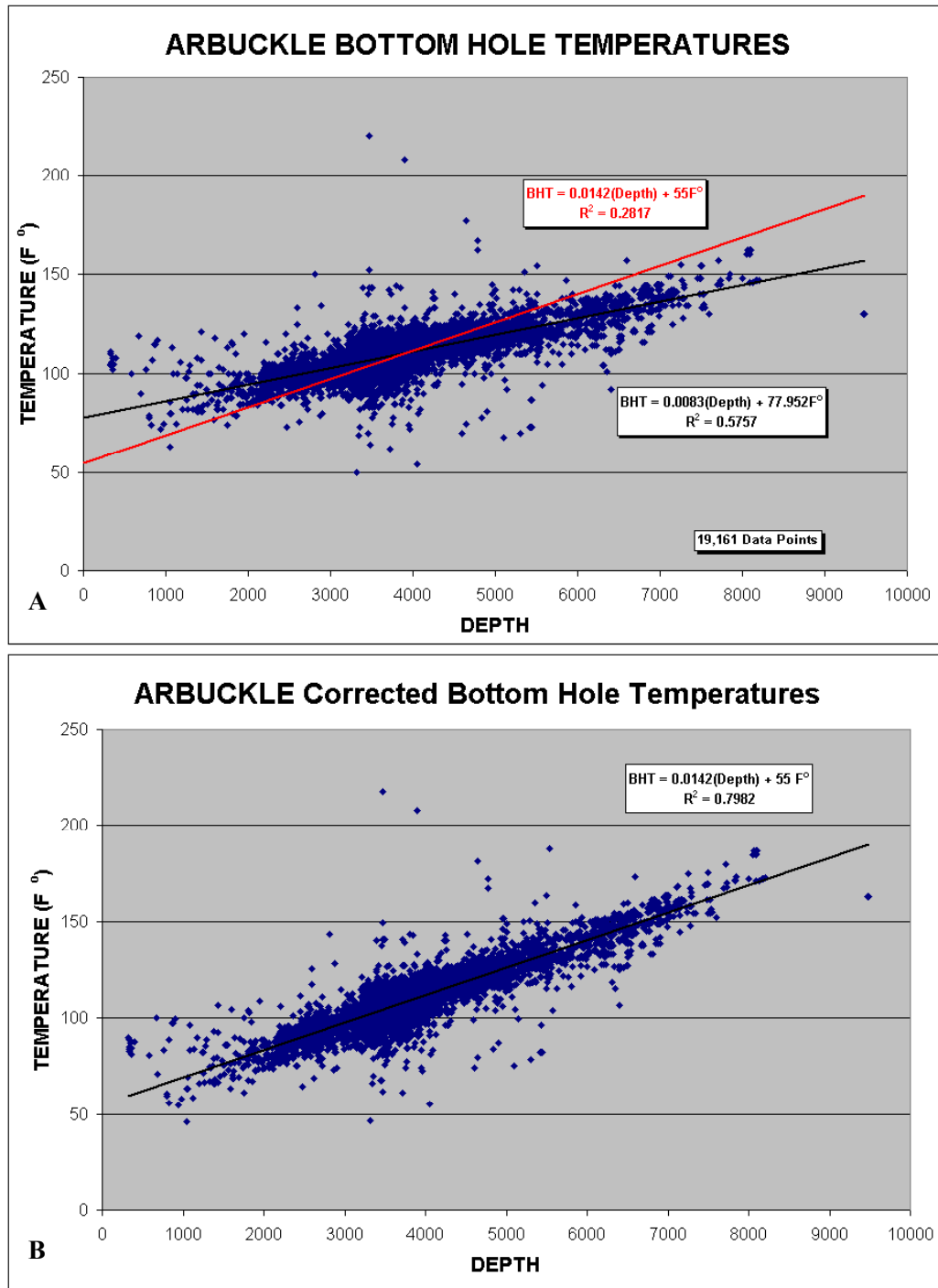
Figure 18 – A) Bottom-hole temperatures (BHTs), recorded from 19,161 wells, are not at equilibrium with formation temperature and require correction. The BHT correction factor adjusts the temperature recorded during logging to the “true” formation temperature. B) The corrected BHTs for the Arbuckle show the same relationship of temperature with depth and an improved fit ( R^2 = 0.8 ). The scattered outliers are obvious on the crossplots and are probably the result of tool malfunction, reading or recording errors at the time of logging, or data entry errors.
