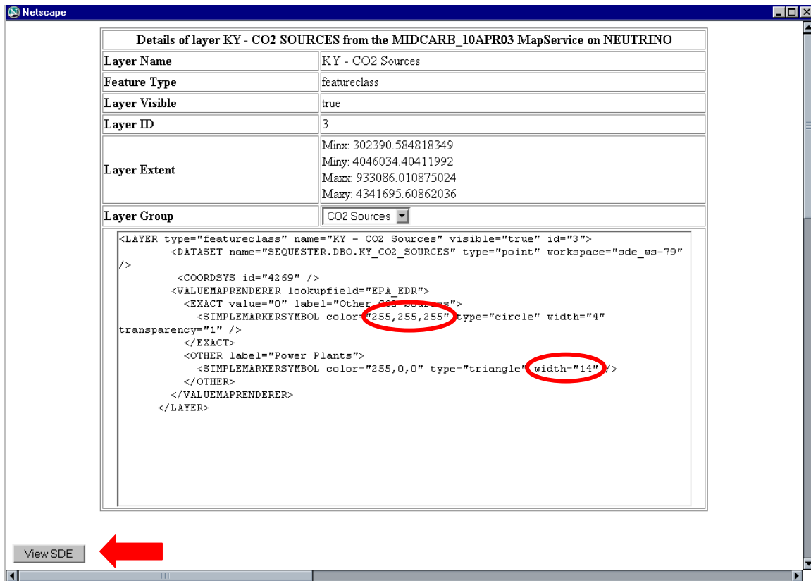
Figure 9 – For the coverage KY- CO2 Sources , the administrator changes the size of Kentucky electric generation sites and the color of the other Kentucky CO 2 sources (red ellipses - see Figure 7 for previous object characteristics). The result can be viewed by the administrator (red arrow) and if satisfied can be accepted (Figure 10). After acceptance, the result is available to all users on the MIDCARB system.
