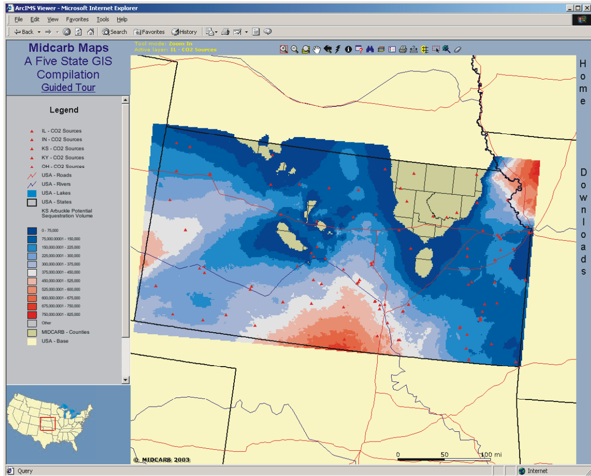
Figure 20 – Estimated CO 2 sequestration potential in the Arbuckle-Knox saline aquifer. SDE layer generated for each square mile of Kansas from aquifer temperature, pressure, salinity, porosity and thickness coverages. The entire Arbuckle Aquifer underlying Kansas has the potential to sequester a very large quantity of CO 2 - A number approaching 16,994 trillion cubic feet of CO 2 . (894 billion metric tonnes). Assumes solubility in brine. If displacement is more significant the volumes will be significantly greater.
