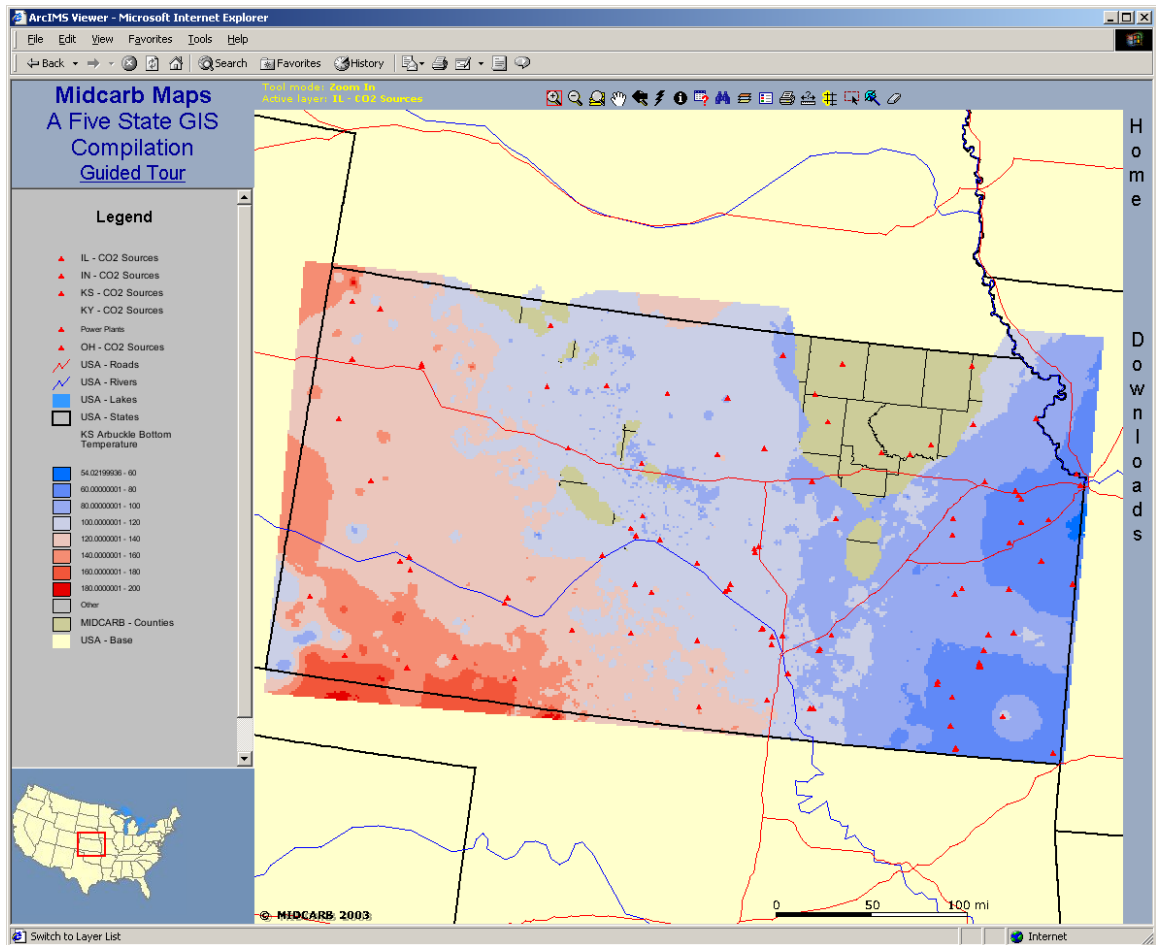
Figure 19 – View of KS-Arbuckle-Knox Aquifer Temperature SDE layer using corrected bottom hole temperatures from 19,161 wells across Kansas (Figure 17).
