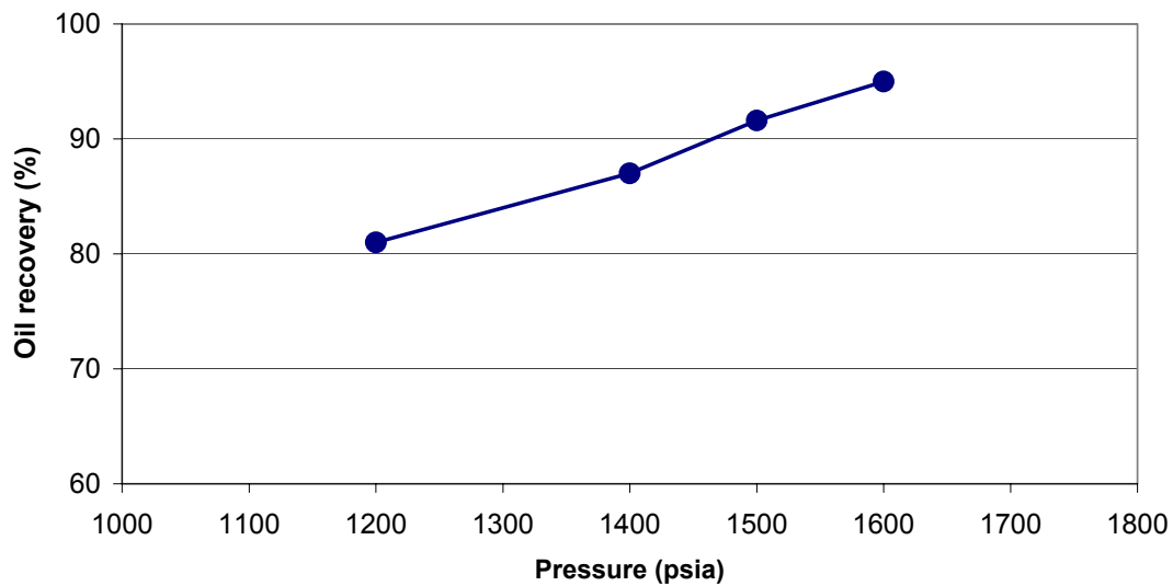
Figure A8 - Oil recovery (at 1.2 HCPV injection of CO 2 ) as a function of pressure for Ohio oil sample at 107 °F.
