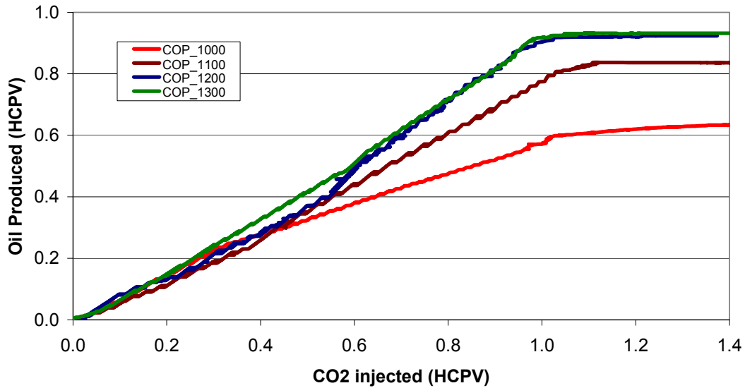
Figure A1 - Oil recovery results in slim-tube experiment with CO 2 displacing Indiana oil sample at 101 °F.
