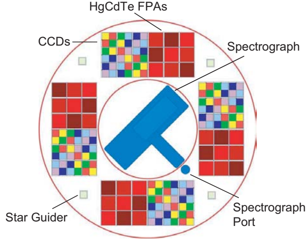
Figure 5. The SNAP near infrared imager concept: The imager contains optical and IR sensors integrated on a common focal plane. A total of thirty-six, 2k \times 2k , 18 \mu m detectors will be used to cover the 900 nm to 1700 nm range.
