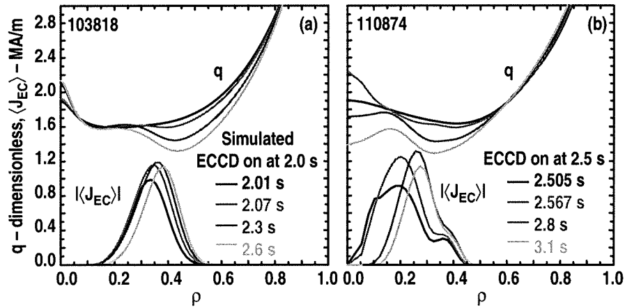
FIG. 2. Shown are: (a) Theory-based design of q -profile control experiment, showing time dependent Corsica simulations of the effect of 2.5 MW of co-ECCD at \rho=0.35 , with fixed \chi , n_e and Z_{\text{eff}} as determined from QDB discharge 103818. (b) Time dependent Corsica analysis of corresponding ECCD experiment, discharge 110874, with \sim 2 MW of co-ECCD injected at \rho \sim 0.2-0.3 , using experimental time dependent profiles as input.
