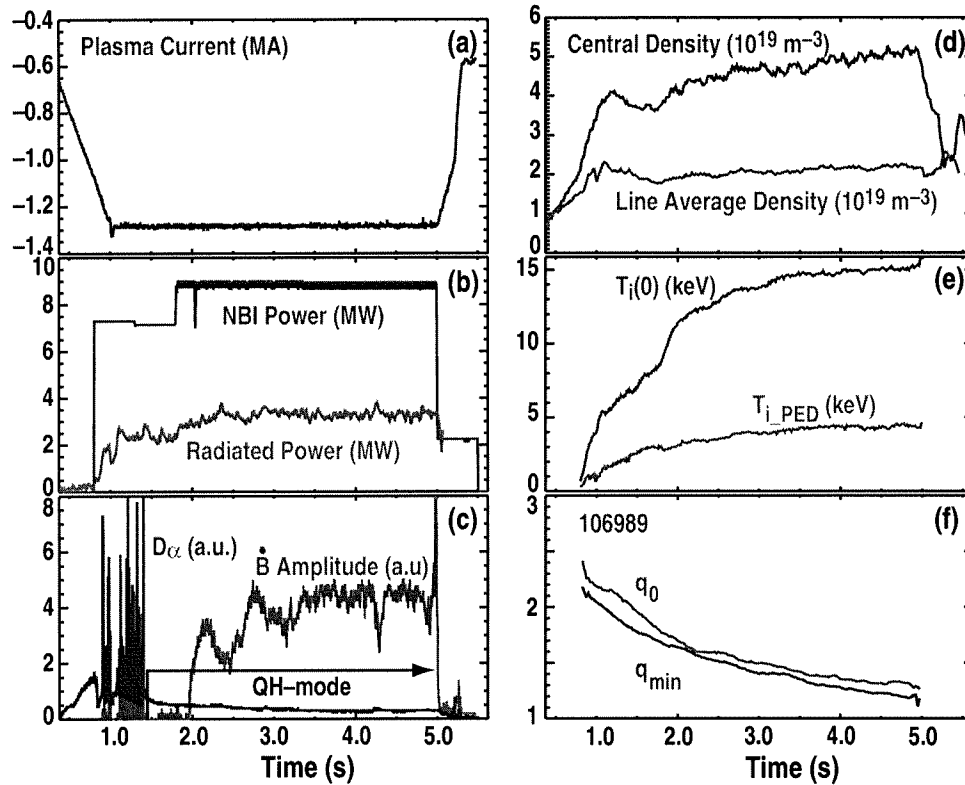
FIG. 1. Time history of a long-pulse QDB plasma (106989), showing: (a) plasma current I_p , (b) PNBI and P_{rad} , (c) divertor D_\alpha emission and magnetic probe signal amplitude, (d) central and line average density, (e) central and edge pedestal T_i and, (f) q_0 and q_{min} . This discharge maintains a quiescent edge for 3.8 s, or \sim 26 \tau_E .
