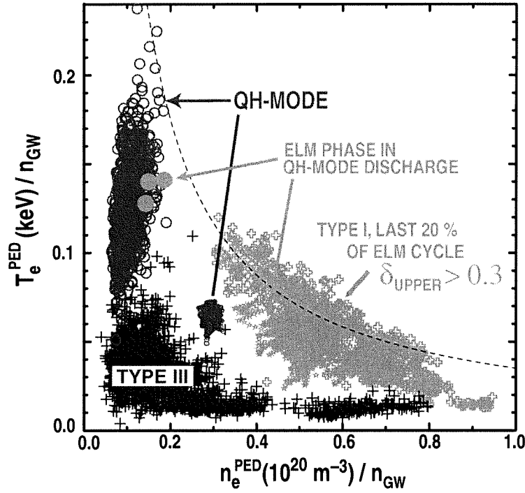
FIG. 6. Comparison of edge pedestal conditions in QH-mode and Type I and III ELMy regimes. The temperature at the top of the pedestal, T_e^{\text{PED}} is plotted versus n_e^{\text{PED}} , both quantities being determined from Thomson scattering data. Both axes are normalized by the Greenwald density, n_{\text{GW}} . The dashed curve illustrates a surface of constant pressure.
