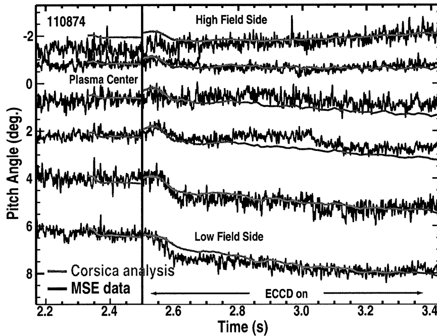
FIG. 3. Comparison of internal magnetic field pitch angles as determined from Corsica analysis with raw MSE data as a function of radius and time for discharge 110874. Channels on the high field side of the device are at the top of the plot while the low field side is at the bottom. In this discharge, ECCD is applied at 2.5 s. The rapid and large changes in pitch angle with ECCD directly indicate q -profile modification, while the data from the central channels indicate an initial transient rise in q_0 .
