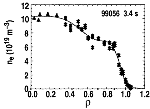
FIG. 7. Density profile for a 2 MA QH-mode discharge (99056), with n_e^{\text{PED}} = 6.5 \times 10^{19} \text{ m}^{-3} and a line average density of 7.6 \times 10^{19} \text{ m}^{-3} , corresponding to \bar{n}_e/n_{\text{GW}} = 0.43 .
