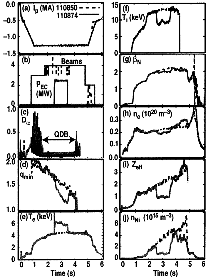
Fig. 1. QDB parameters for no ECCD reference 110850 and shot 110874 with 2 MW EC power with co-ECCD aiming at \rho = 0.2 .
