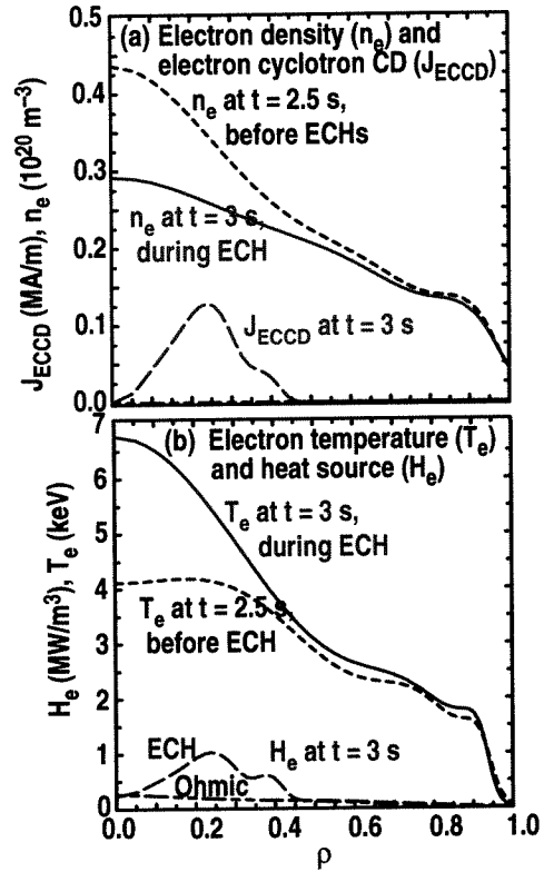
Fig. 2. Density and temperature profile response to EC power inside barrier.
