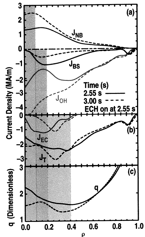
Fig. 3. Current and q profile response to EC injected inside the ITB for shot 110874 with 2 MW EC for co-ECCD at \rho = 0.2 .
