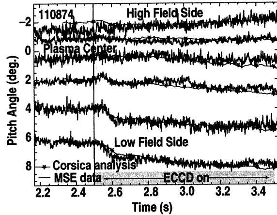
Fig. 4. Comparison of MSE data and calculated synthetic MSE data from evolution of current profiles and equilibrium.
