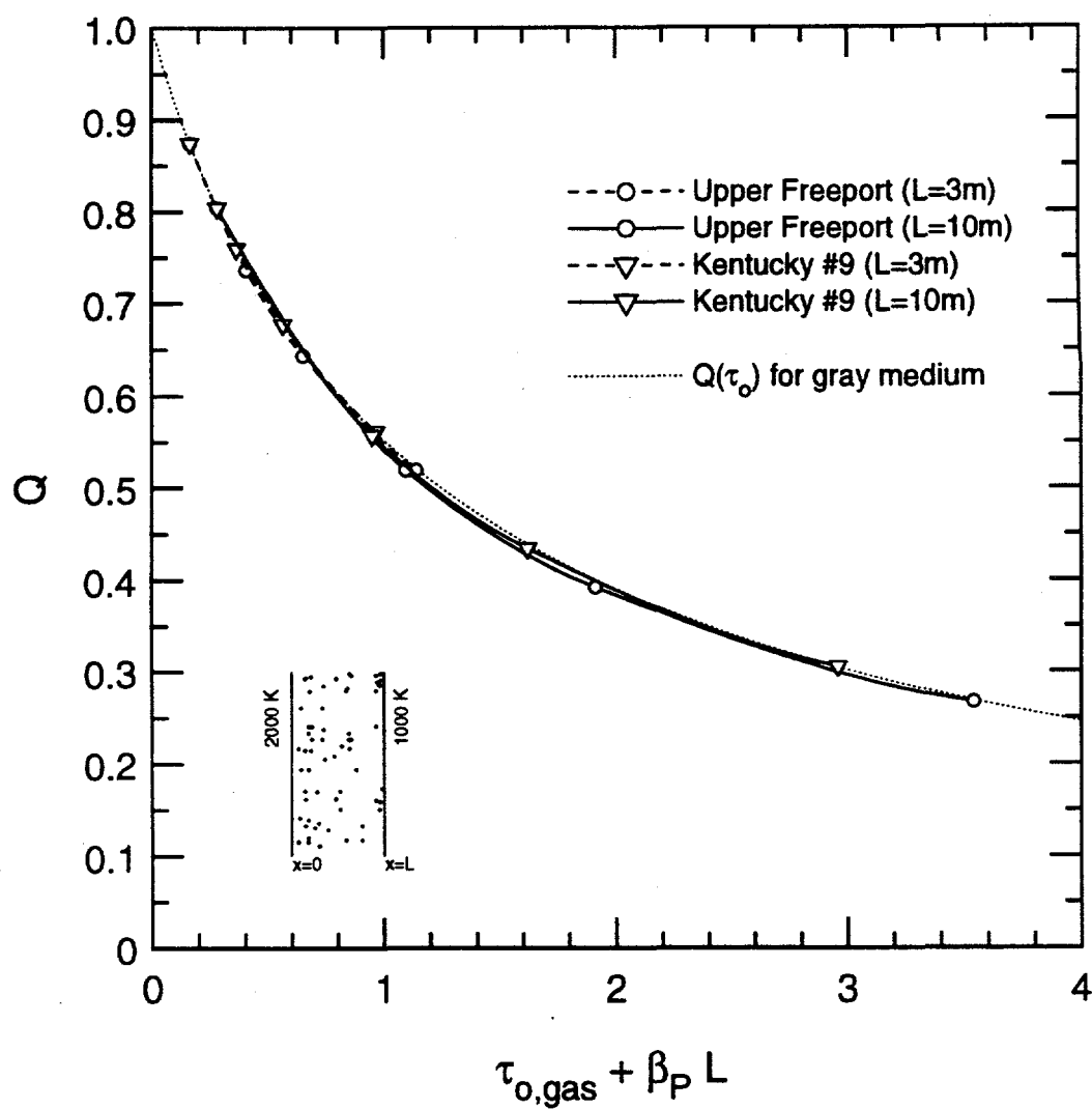
Figure VI.13: Effect of ash loading on the total radiative heat flux through a planar layer of ash plus CO_2 and H_2O versus the approximate optical depth of the layer.
