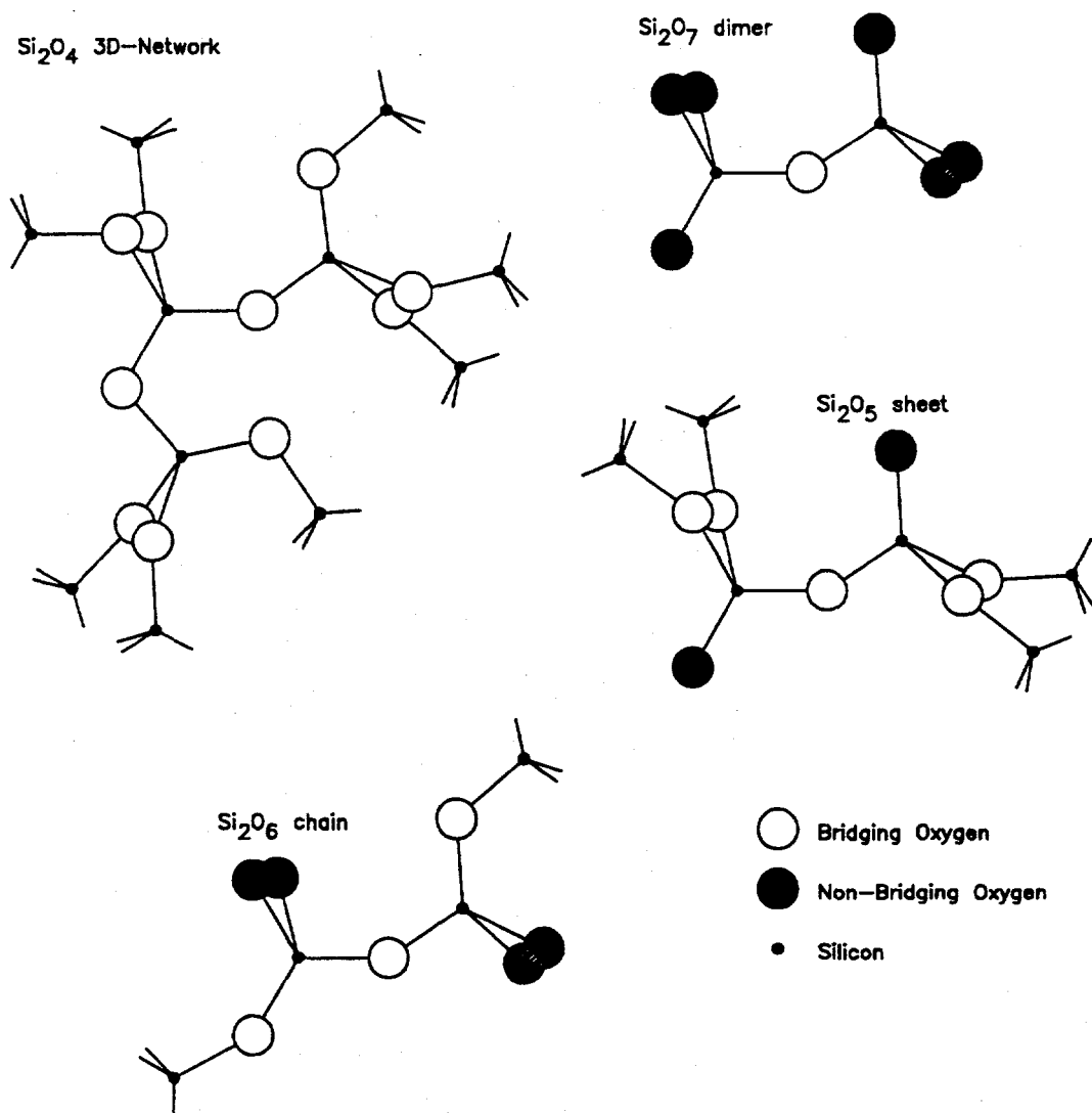
Figure F.2: Examples of silica random network model structures for glasses.
