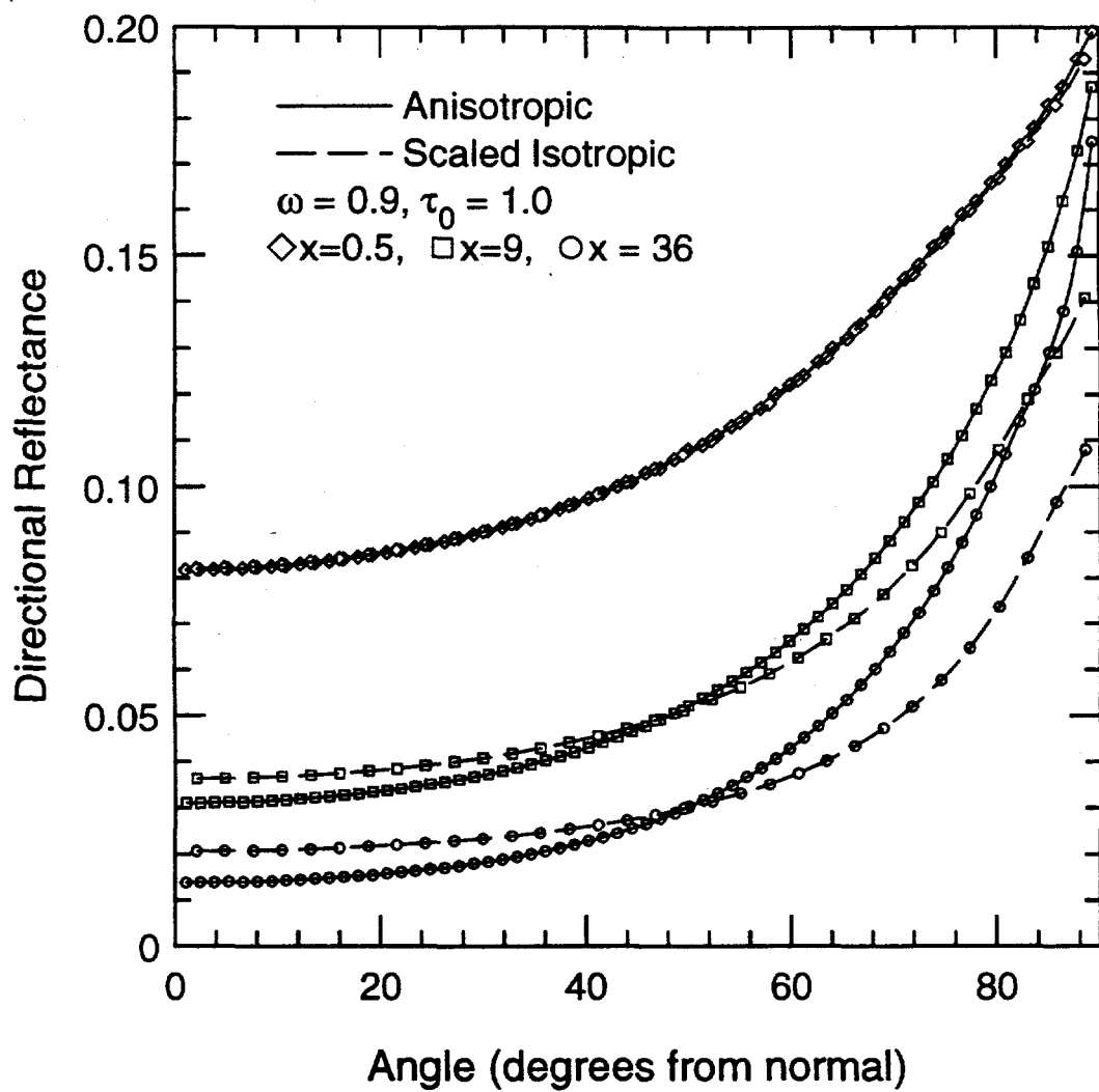
Figure E.6: The directional reflectance for \omega = 0.9 , \tau_0 = 1 , and x = 0.5, 9 , and 36
