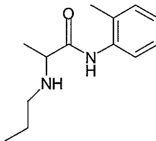
Prilocaine
