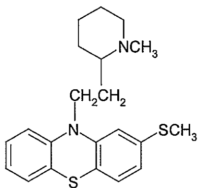
Thioridazine
