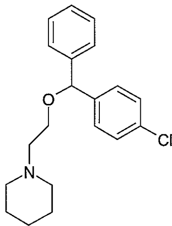
Cloperastine
