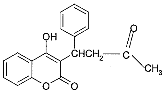
Warfarin
