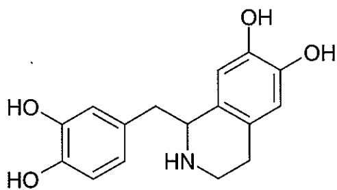
Tetrahydropaveroline
