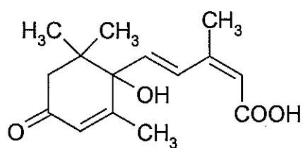
Absciscic acid
