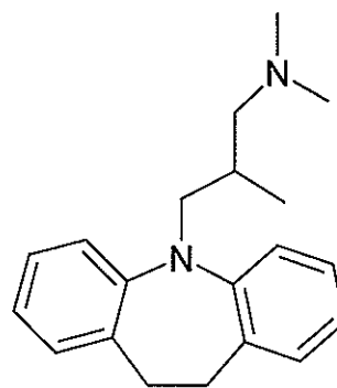
Trimipramine
