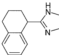
Tetrahydrozoline
