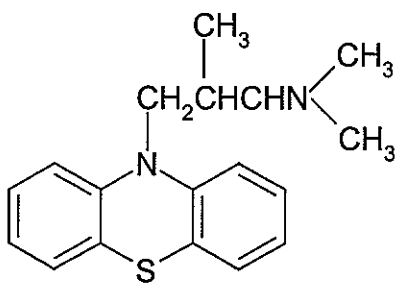
Trimiprazine
