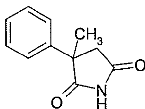
Methylphenylsuccinimide
