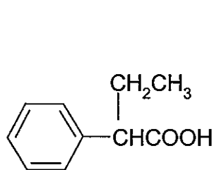
Phenylbutyric acid
