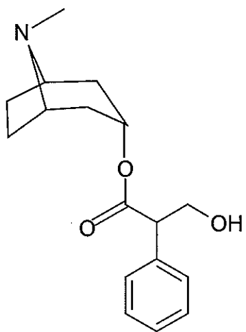
Atropine
