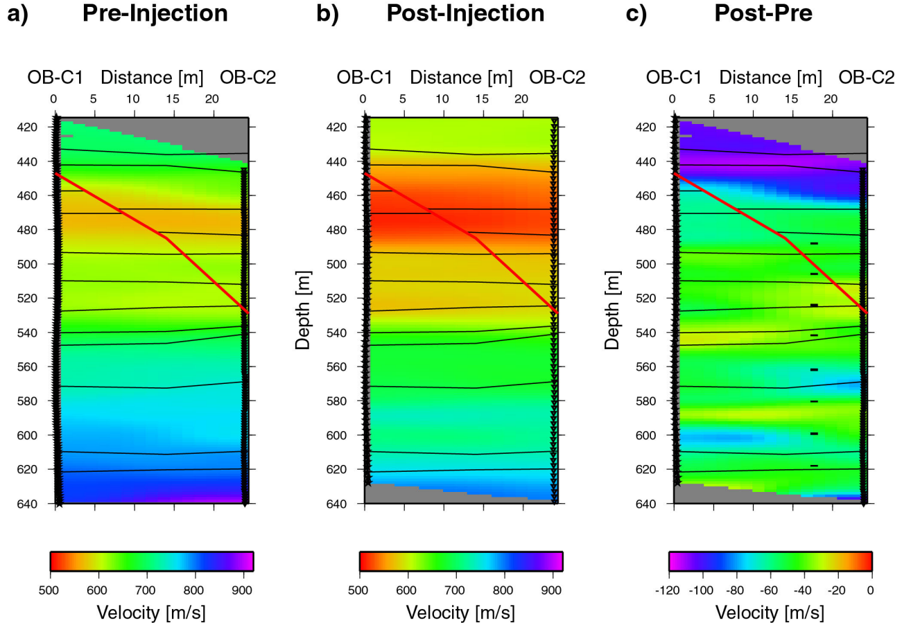
Figure 5: S-wave velocity estimates based on travel time data. a) Pre-injection estimates. b) Post-injection estimates. c) Result of differencing the Pre-Post injection estimates. The black dashes represent the projection of the CO 2 injection intervals onto the imaging plane.
