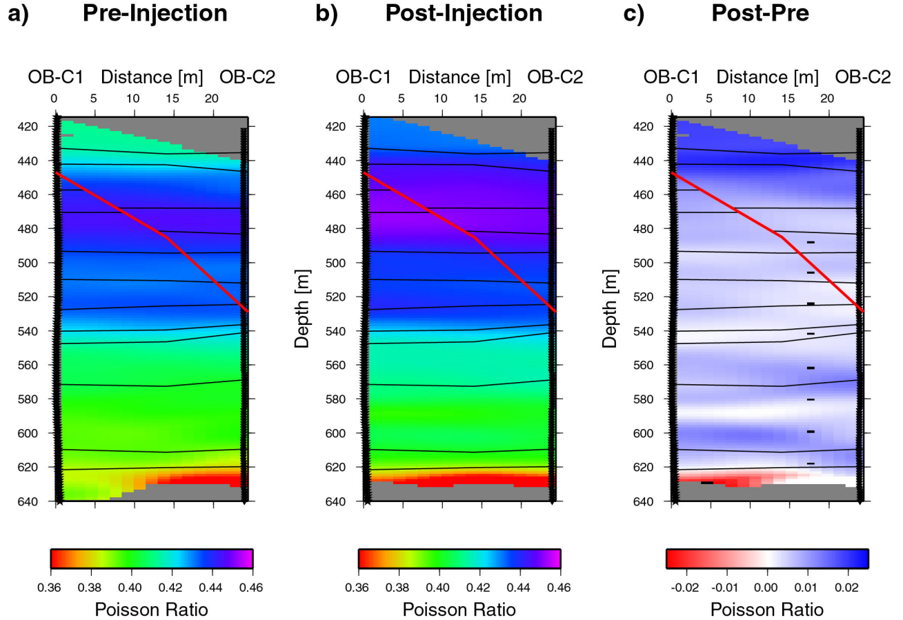
Figure 6: Poisson ratio based on the P- and S-wave velocity estimates in Figures 4 and 5. a) Pre-injection ratio. b) Post-injection ratio. c) Result of differencing the Pre-Post injection ratios. The black dashes represent the projection of the CO 2 injection intervals onto the imaging plane.
