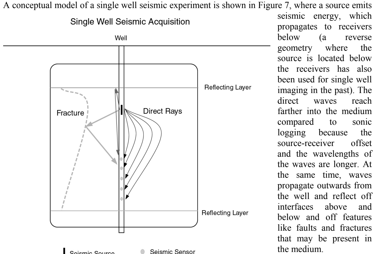
Figure 7: Wave propagation in single well seismic data acquisition. The sketch displays the principle of wave propagation from the source to the receivers along direct or reflected ray paths.
