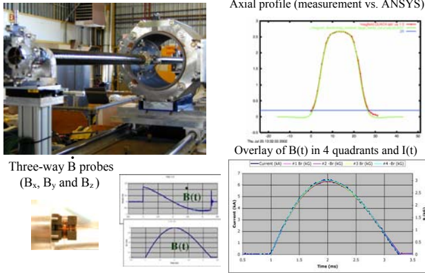
Figure 4: Magnetic field measurement.
