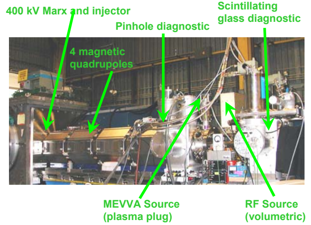
Figure 1: Neutralized Transport Experiment (NTX).
