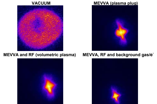
Figure 6: Spot size dependence on neutralization mechanism. Image box size is 4cm \times 4cm squares.
