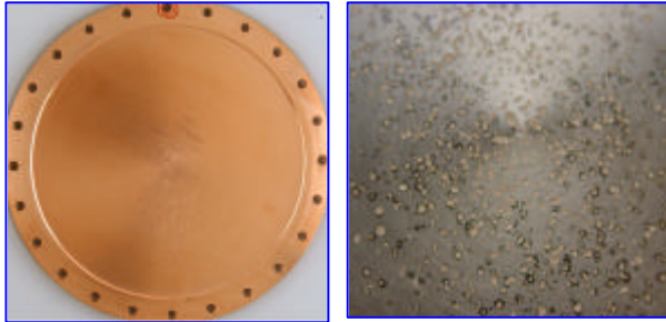
Figure 2: Cu window after RF conditioning with the external 2.5 T magnetic field in solenoidal mode. Surface damage (pitting) can be seen clearly on the photo (right), which is a close-up view of the center region of the same window.
