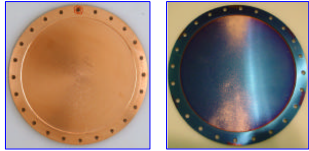
Figure 3: Cu window (left) and Be window (right) after RF conditioning with magnetic field. Deposited Cu particles on the Be window can be seen clearly.
