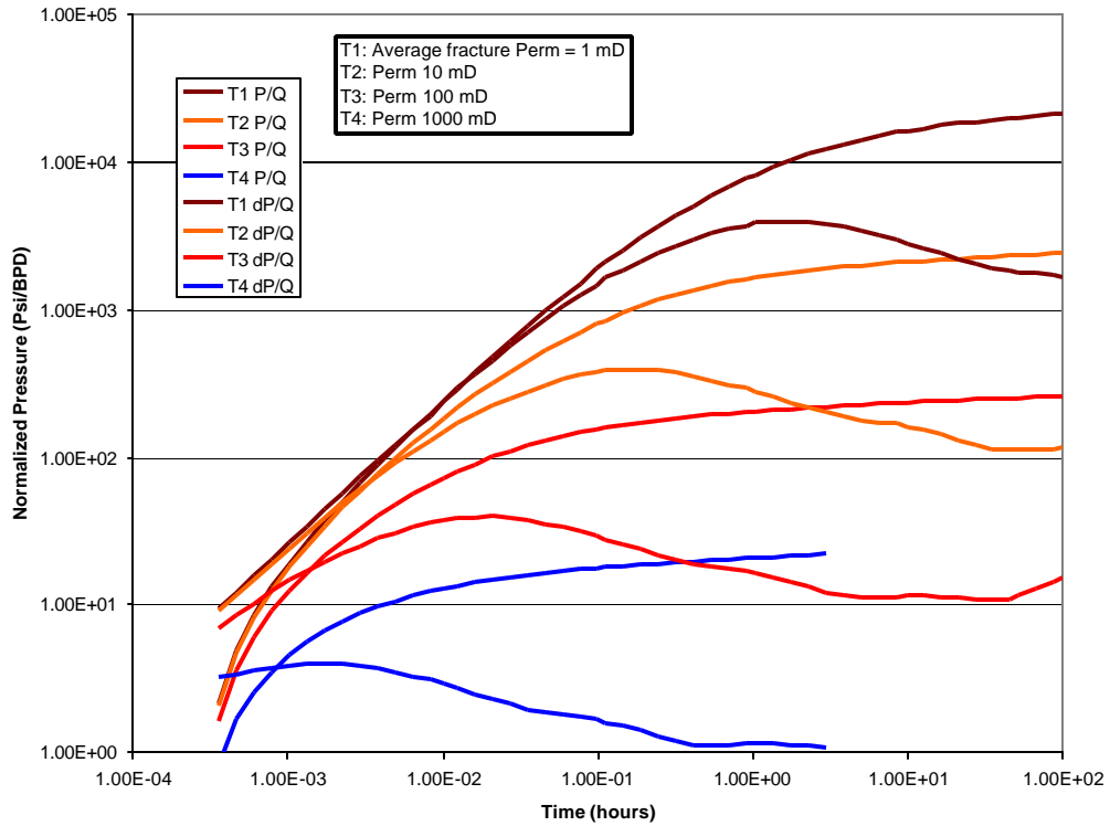
Figure 3-82. Build up test simulations for average fracture permeabilities of 1 to 1000 mD
