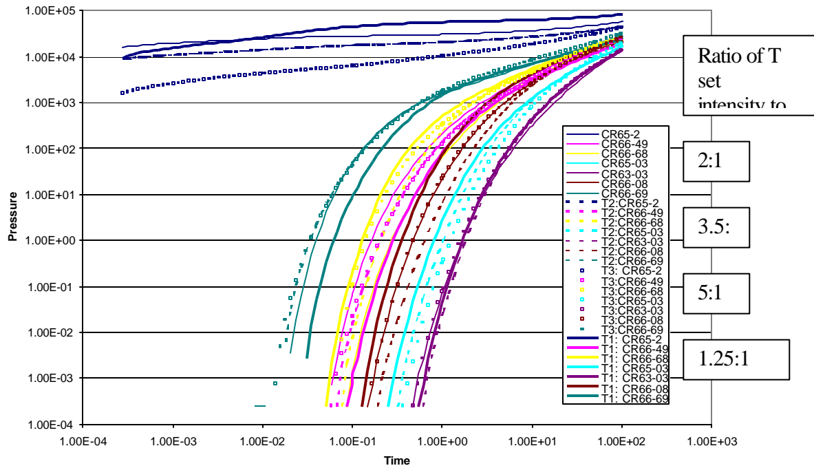
Figure 3-92. Breakthrough curves for all wells for varying the ratio of the fracture intensities between the T and L sets.
