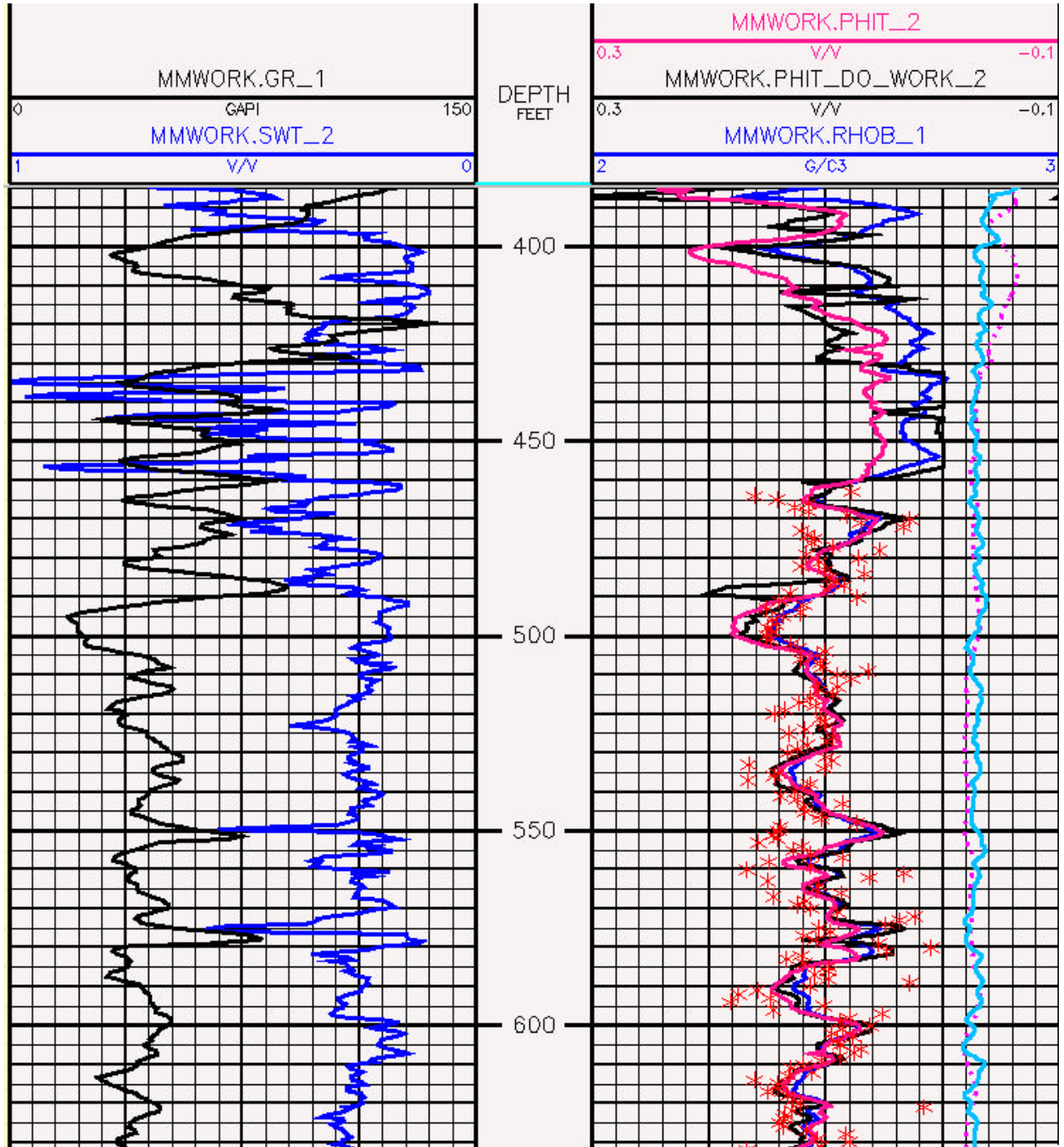
Figure 2-12. Porosity determination from density log, Shoshone 66-49, Tensleep Formation.
