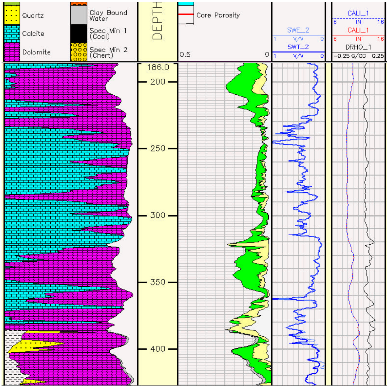
Figure 2-1. Phosphoria MULTIMIN display
