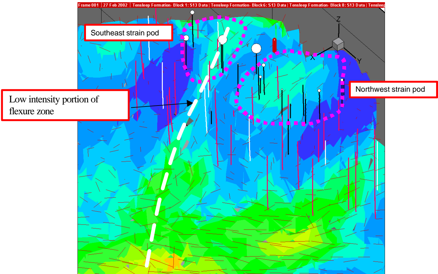
Figure 3-72. Delineation of strain pods. Most of the responding wells are in one of two strain “pods”. Non-responding wells are typically not in these pods. They tend to be in low strain zones or in pods separated from the pods connected to the injector pods by areas of low strain. White dashed line indicates a dip-parallel flexure zone.
