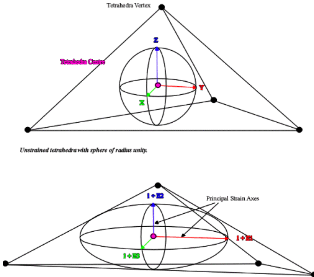
Figure 2-46 Strained tetrahedron with strain ellipsoid. The XYZ axes are eigenvectors of the strain field, and are the principal strain axes.
