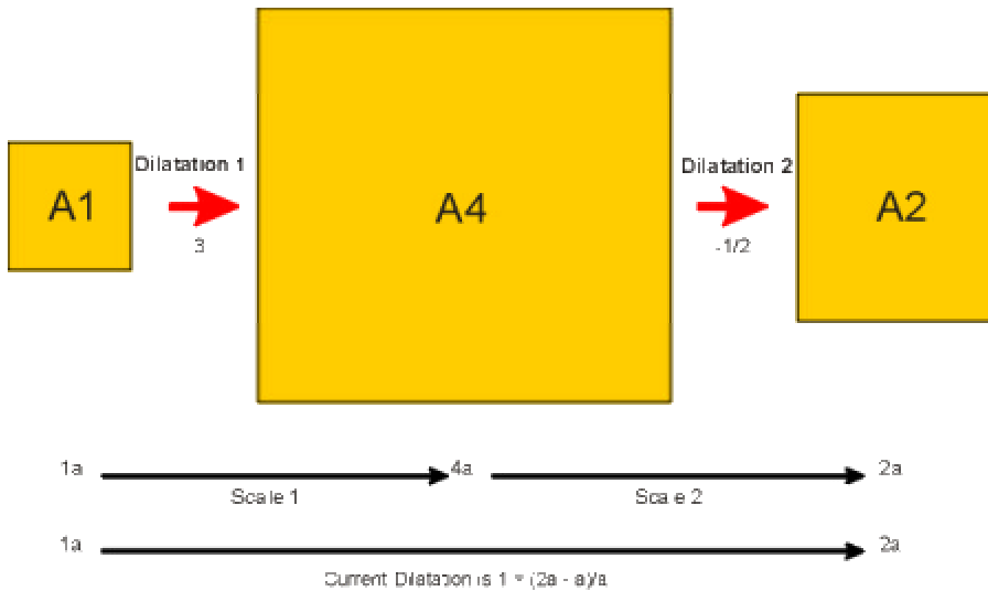
Figure 2-47 Example of the calculation of current dilatation (from Midland Valley, 2000)
