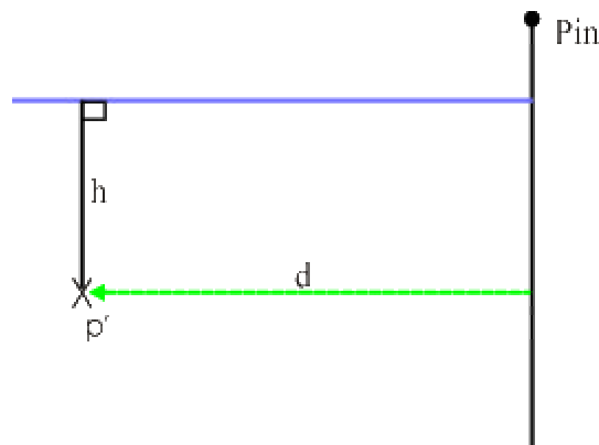
Figure 2-45 Flexurally unfolded template and passive horizons (from Midland Valley, 2000)
