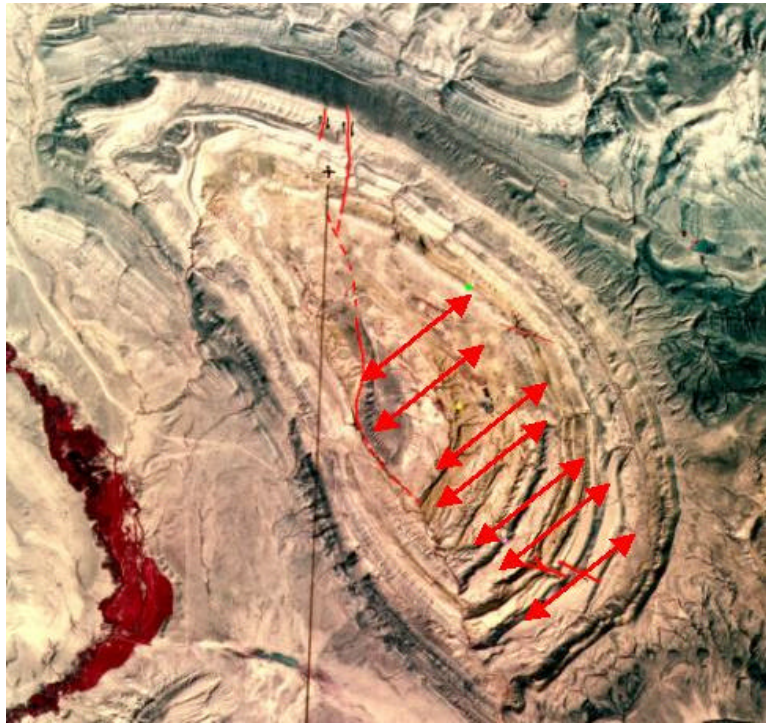
Figure 4-5. Satellite image of Field with perceived regional northeasterly striking fracture set superimposed on photo.
