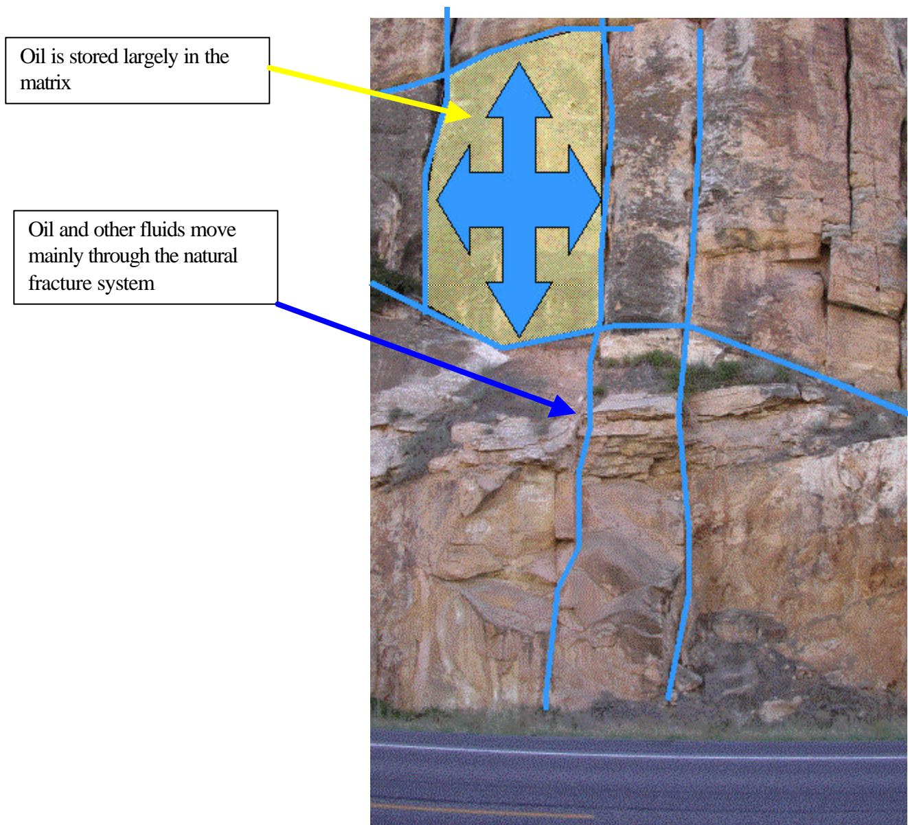
Figure 1-3. Outcrop of Tensleep Formation, Wind River Canyon, Wyoming, illustrating roles of matrix as storage and natural fractures as permeability.
