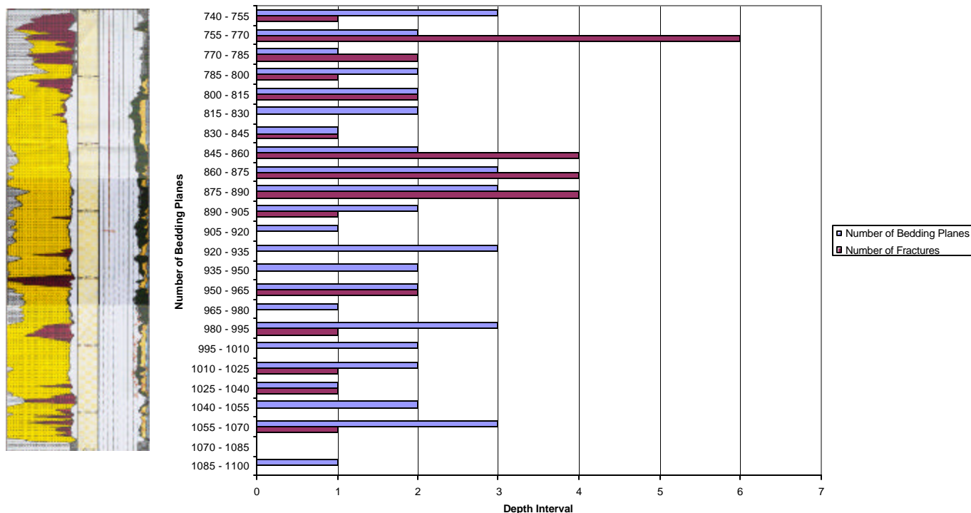
Figure 3-76. Correspondence of bedding intensity and fracture intensity. Intensity is calculated over 15 ft (4.572 m) non-overlapping windows.
