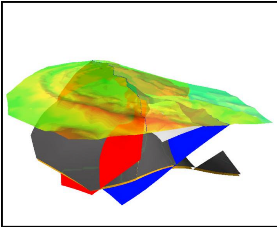
Figure 4-2. 3D visualization of the faults as reconstructed in this project.
