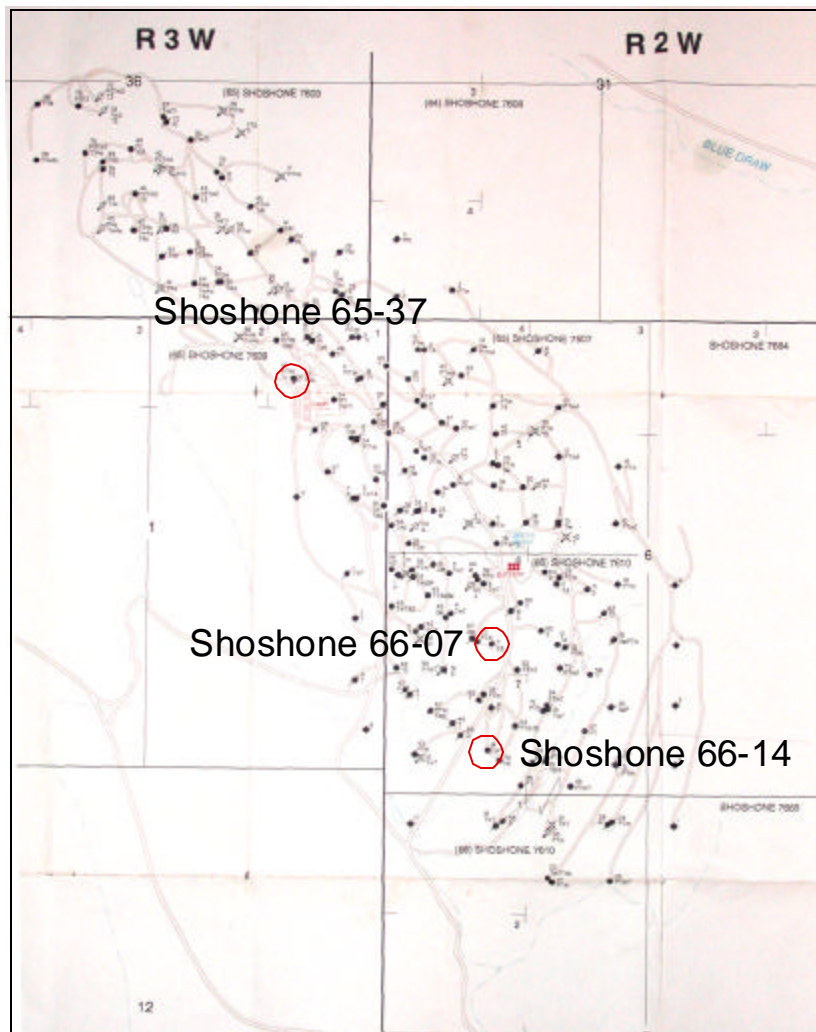
Figure 2-50. Location of wells in which fracture image log and spinner survey data was collected for the project. Shoshone 66-07 and Shoshone 66-14 are in the Overthrust block
