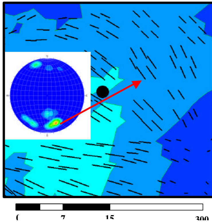
Figure 3-53. Comparison of fracture orientations in Shoshone 65-37 with direction of maximum extension.
