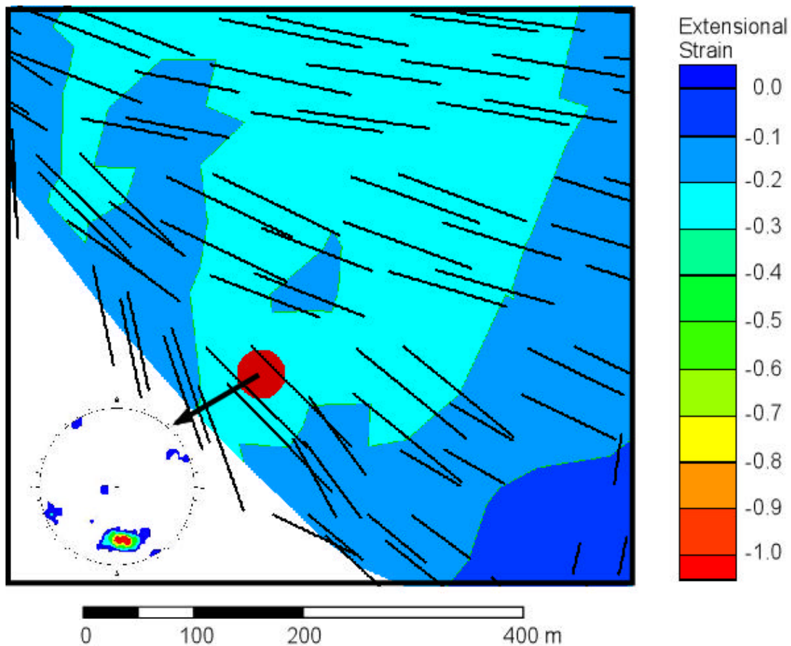
Figure 3-45. Orientation of joints and principal extensional strain for Scanline 10 (Red Peak). The direction of strain is perpendicular to the dominant northeasterly-striking joint set. Black lines indicate trend of principal extension. Lines lengths are proportional to the magnitude of extension.
