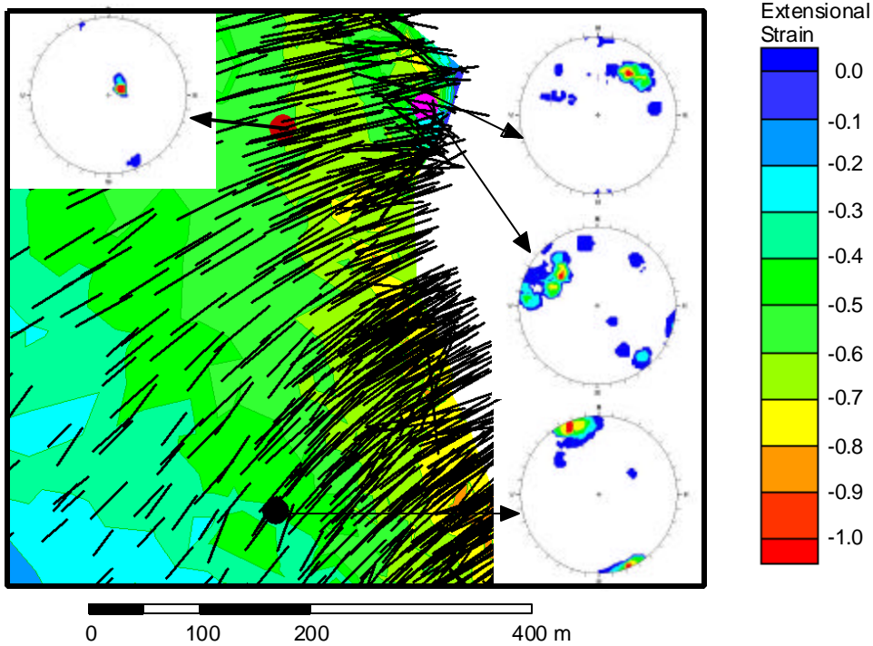
Figure 3-49. Orientation of joints and principal extensional strain for Scanlines 1 and 2 (pink circle), Scanline 3 (red circle) and Scanline 4 (black circle). Black lines indicate trend of principal extension. Lines lengths are proportional to the magnitude of extension.
