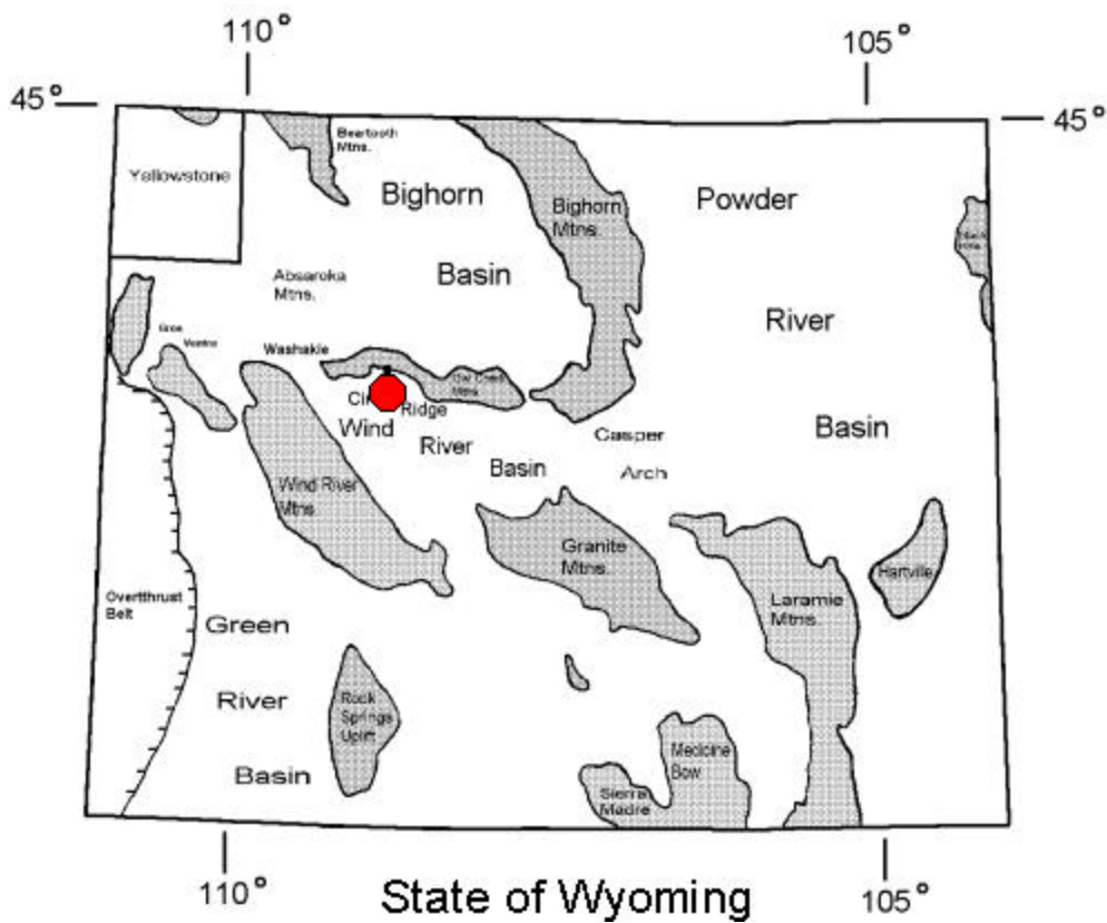
Figure 1-5. Index map showing the Circle Ridge Field and surrounding positive and negative structural elements that define the primary basin and uplift pattern in Wyoming.
