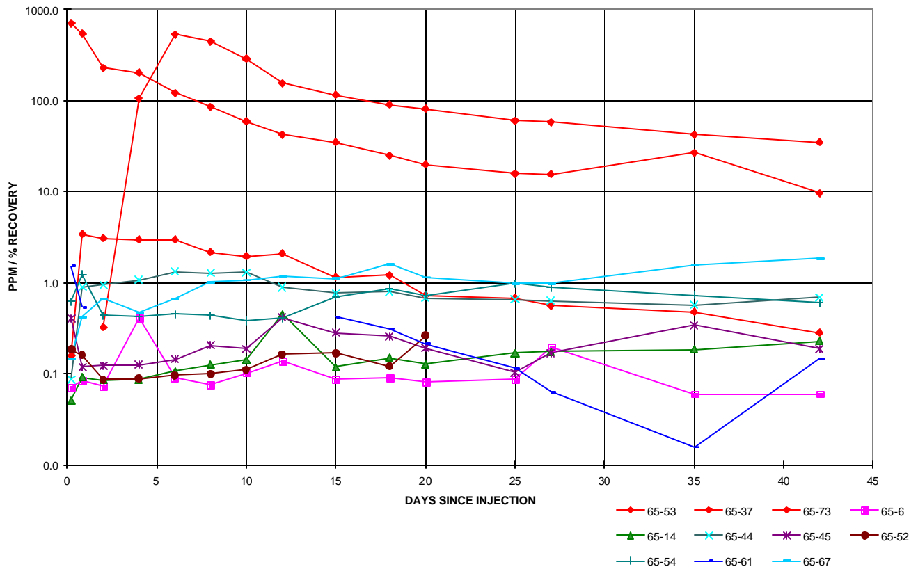
Figure 3-63. Time vs. bromide concentration for the bromide tracer test monitoring wells.
