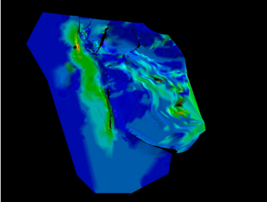
Figure 3-27 Vertical Shear Unfolding of the unfaulted Amsden formation (top view). The color map shows the accumulated strain, with blue colors showing the lowest recorded strains and the red colors the highest.
