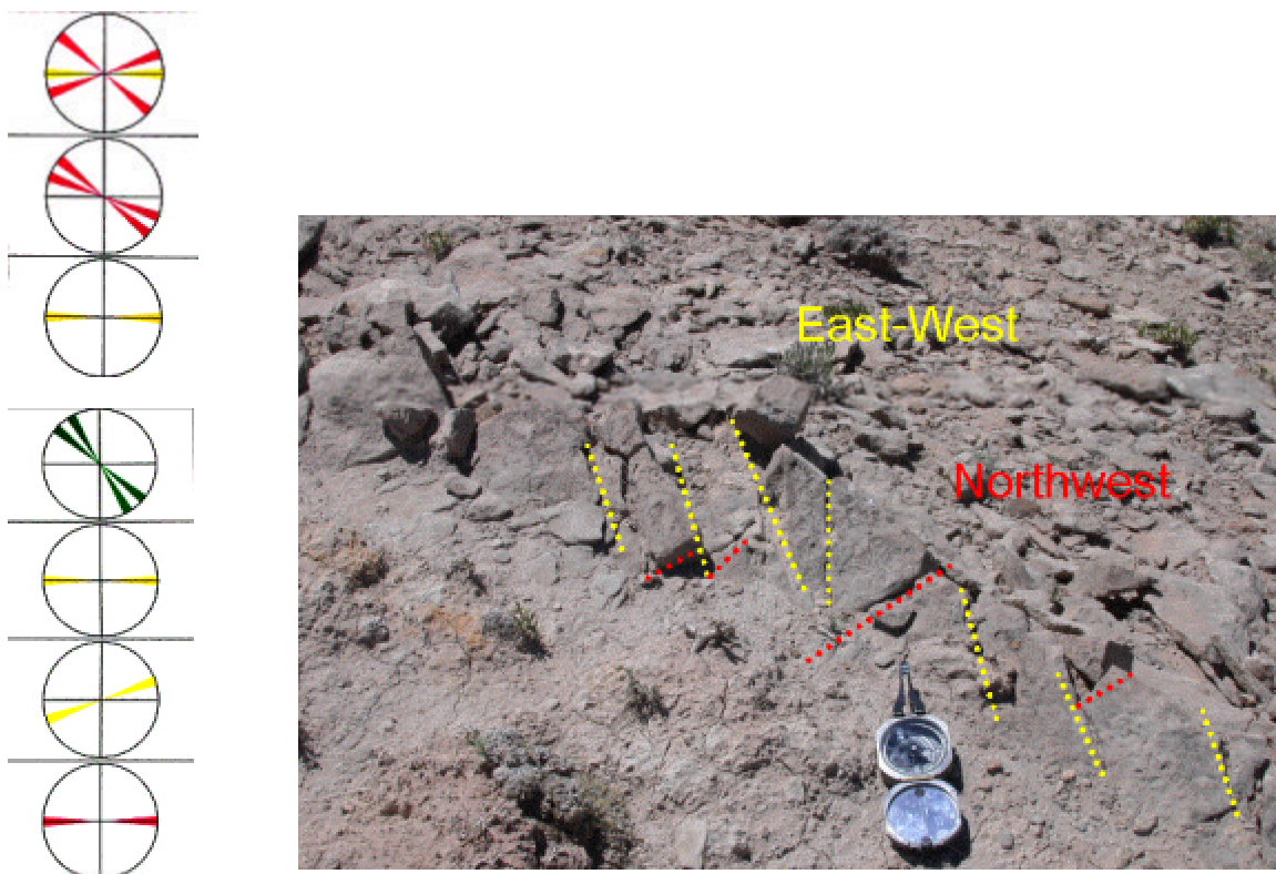
Figure 3-51. Comparison of fracture orientations in outcrop and in the subsurface for Shoshone 66-14.
