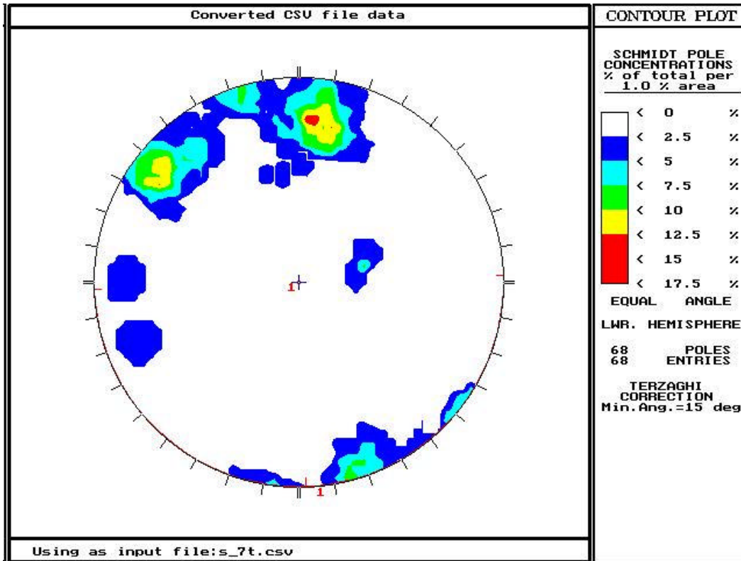
Figure 3-34. Stereoplot for Scanline 7, rotated relative to bedding plane.
