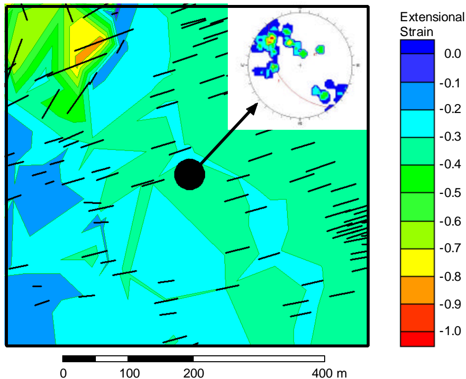
Figure 3-47. Orientation of joints and principal extensional strain for Scanline 11 (Red Peak). The direction of strain is perpendicular to the dominant northeasterly-striking joint set. Black lines indicate trend of principal extension. Lines lengths are proportional to the magnitude of extension.
