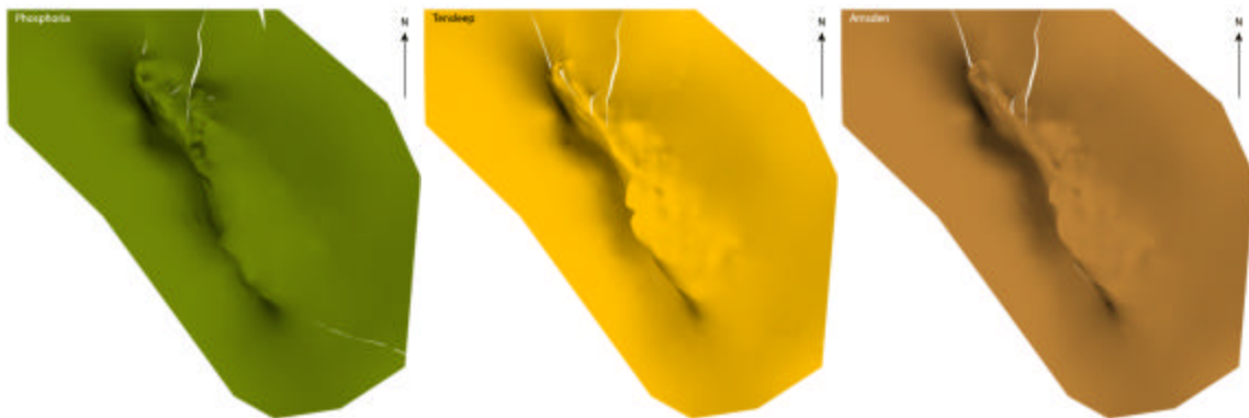
Figure 3-20 The Phosphoria, Tensleep and Amsden formation top surfaces
