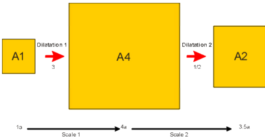
Figure 2-48 Example of absolute and RMS dilatation calculations (from Midland Valley, 2000)
