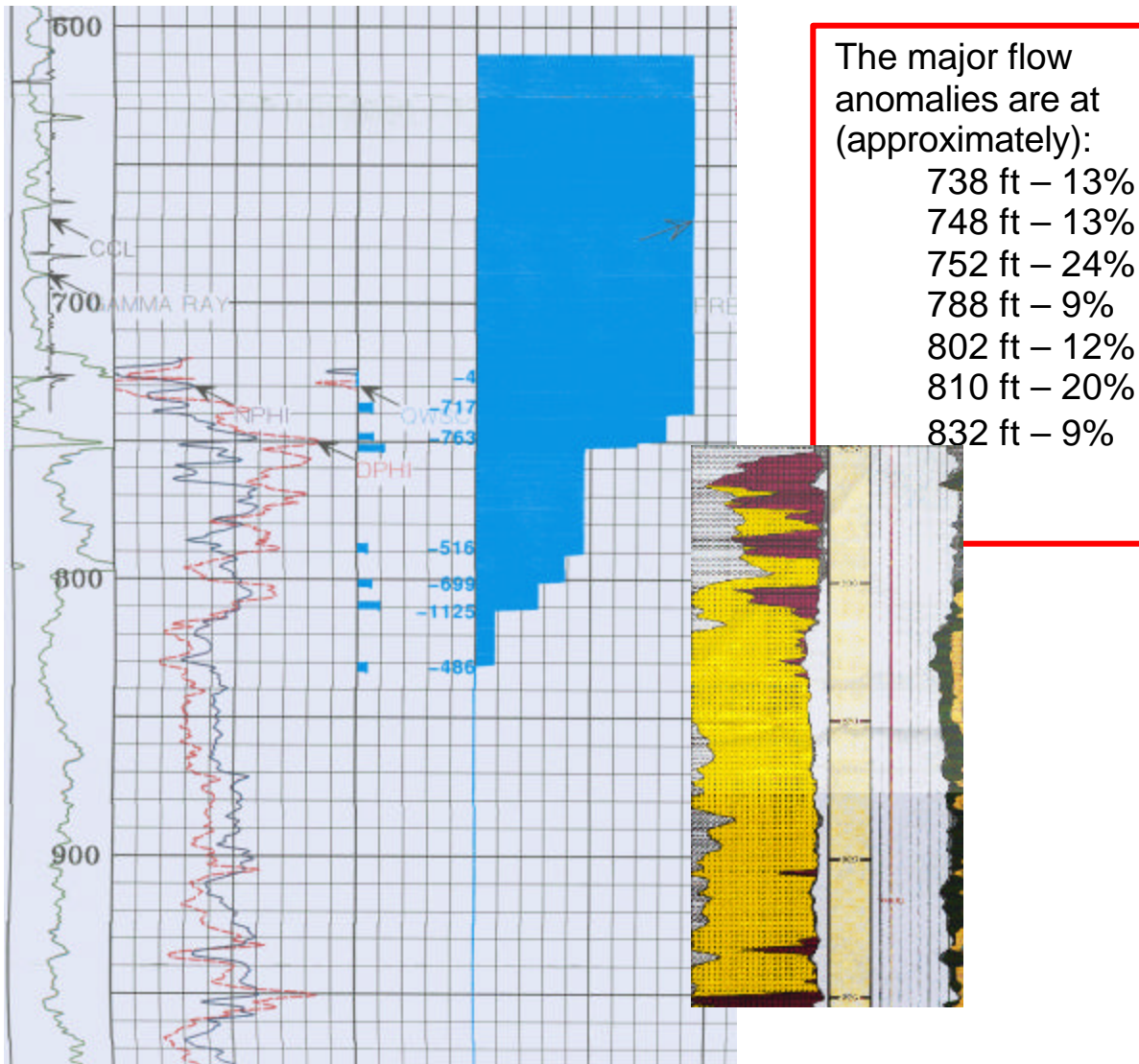
Figure 3-77. Cumulative production profile for Shoshone 66-14.
