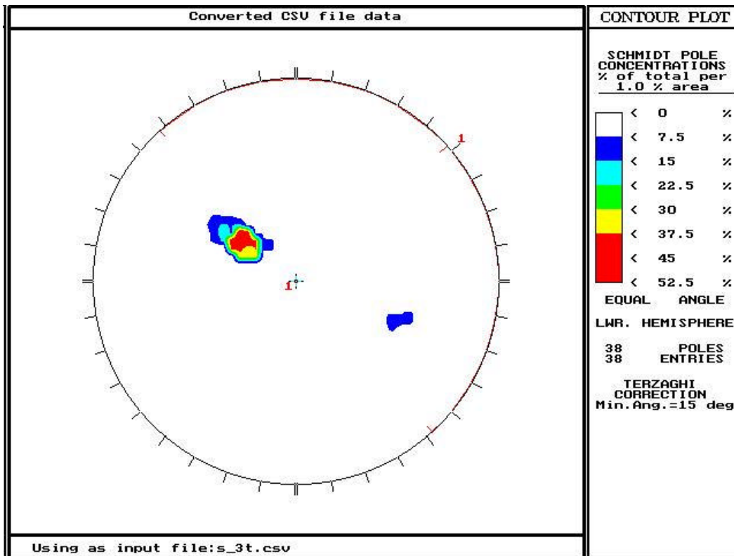
Figure 3-30. Stereoplot for Scanline 3, rotated relative to bedding plane.
