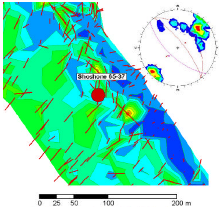
Figure 3-53. Comparison of fracture orientations in Shoshone 65-37 with direction of maximum extension.
