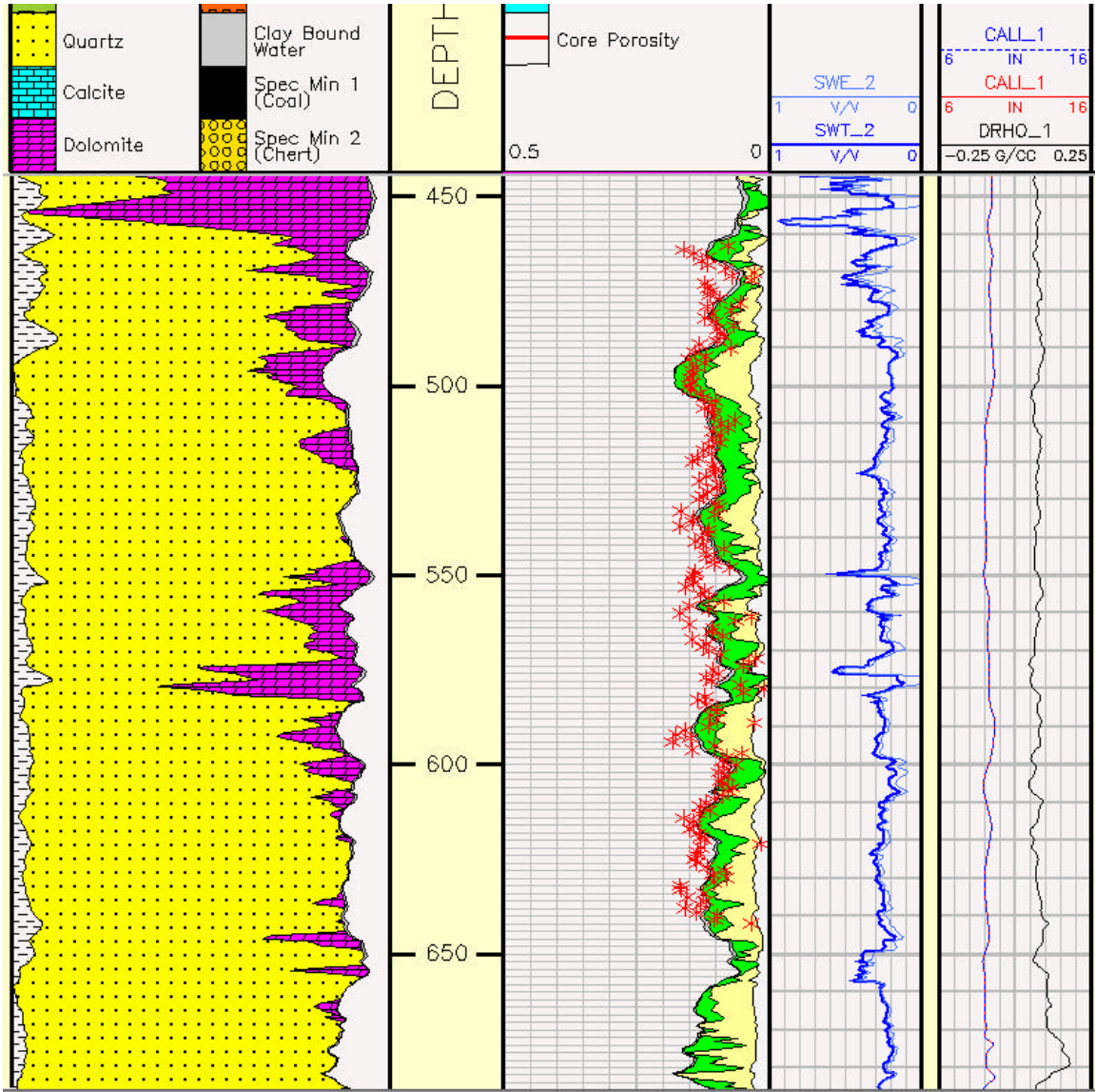
Figure 2-4. Tensleep MULTIMIN display
