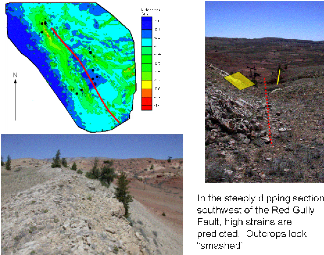
Figure 3-57. Comparison of strain magnitude and fracture intensity in outcrop near the northwest nose of the anticline.
