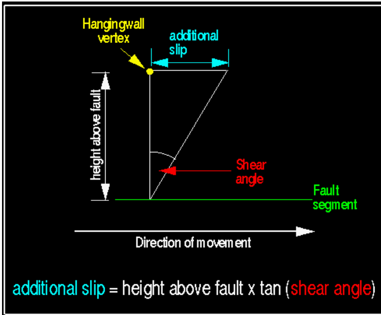
Figure 2-35 Shear calculation using fault parallel flow (from Midland Valley, 2000)
