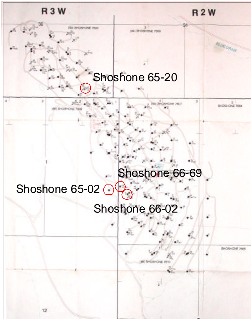
Figure 2-51. Location of wells in which single-well buildup or fall-off test data was obtained for the project.
