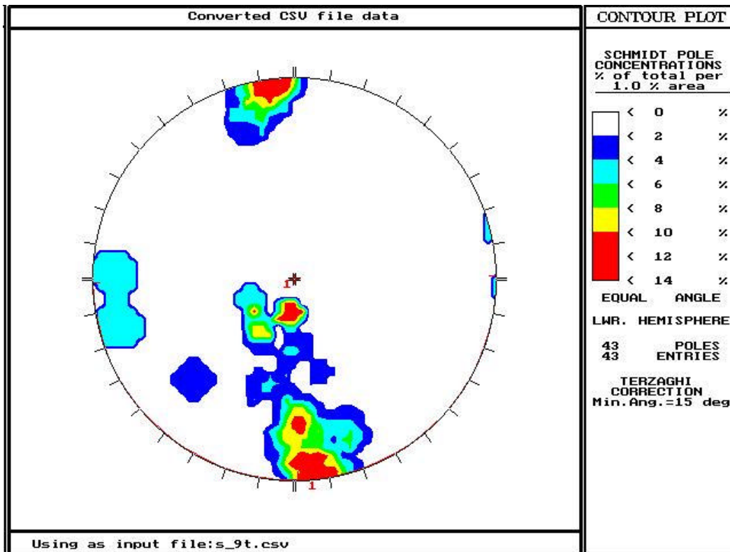
Figure 3-36. Stereoplot for Scanline 9, rotated relative to bedding plane.
