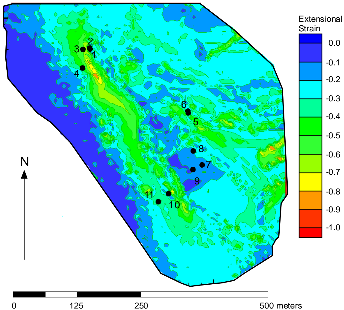
Figure 3-40. Map of principal extensional strain magnitude produced by folding. The contour map shows the approximate horizontal limits of the fault blocks used in the reconstruction. The location of the eleven scanline sites are shown on the map. The strains shown have been mapped on the present-day structural configuration of the Circle Ridge Field, and represent deformation in the Tensleep Formation.
