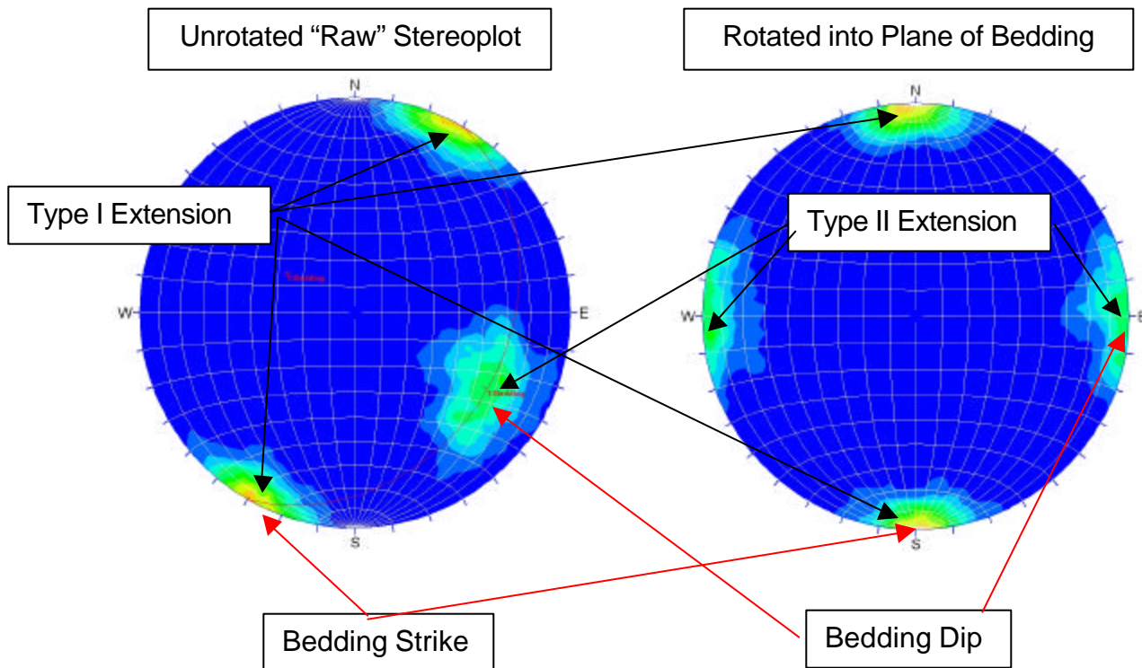
Figure 1-13. Stereoplots illustrating the characteristic relations of the Type I and Type II extension joint sets with respect to bedding.
