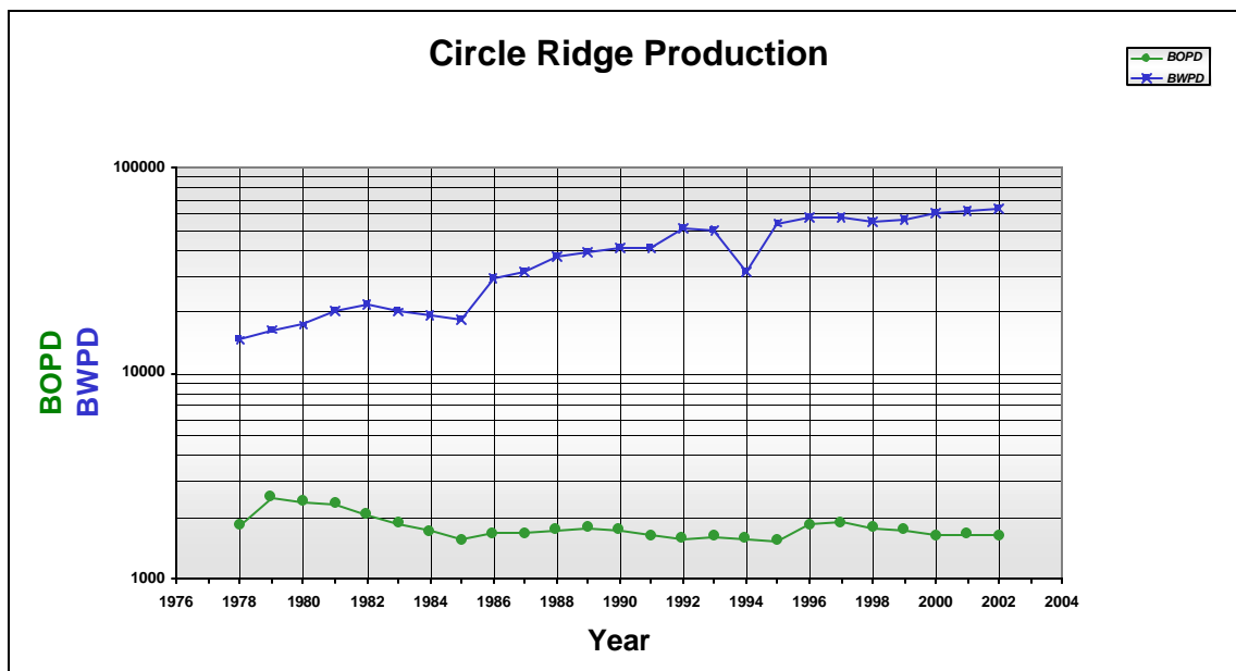
Figure 4-8. Water and oil rates for the Circle Ridge Field, 1978 – present.
