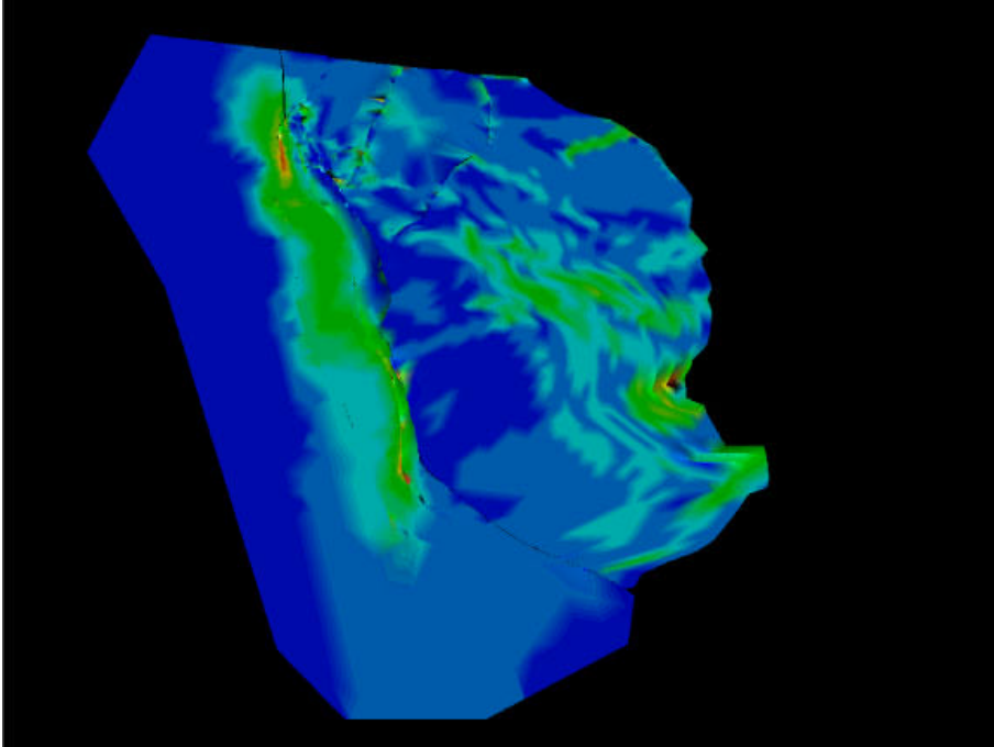
Figure 3-25 Vertical Shear Unfolding of the unfaulted Tensleep formation (top view). The color map shows the accumulated strain, with blue colors showing the lowest recorded strains and the red colors the highest.
