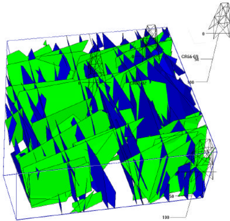
Figure 3-80. Local scale DFN model for Shoshone 65-02.
