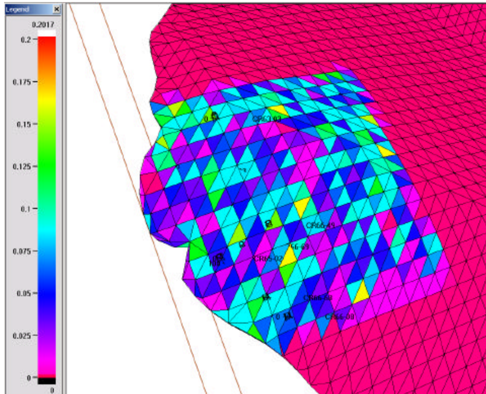
Figure 3-86. Fracture intensity values ( P_{32} ) resulting from an average P_{32} value of 0.08
