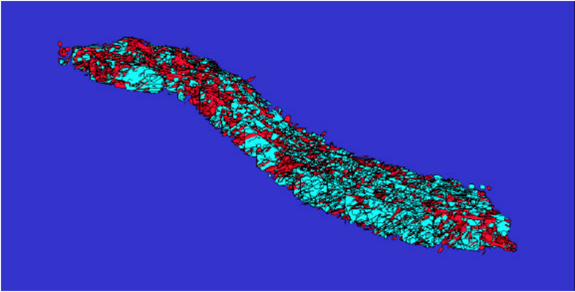
Figure 2-62. Final DFN model for Tensleep Formation, Block 6, including both major fracture sets clipped against the upper and lower boundaries of the Tensleep Formation.
