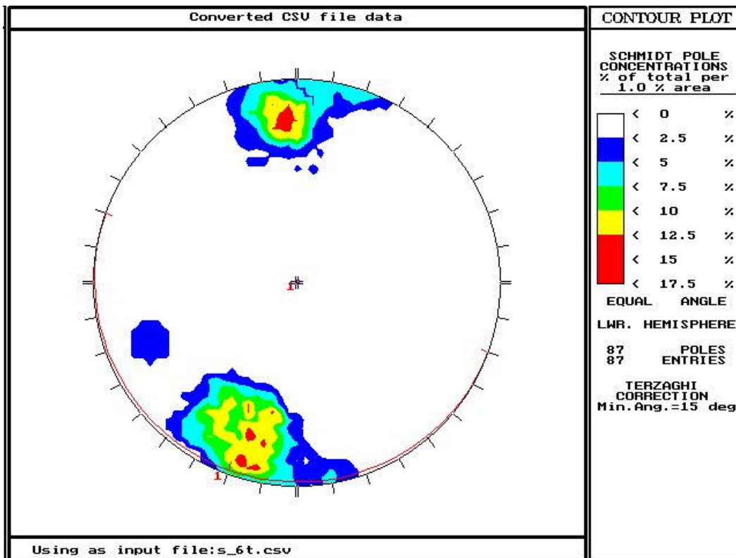
Figure 3-33. Stereoplot for Scanline 6, rotated relative to bedding plane.
