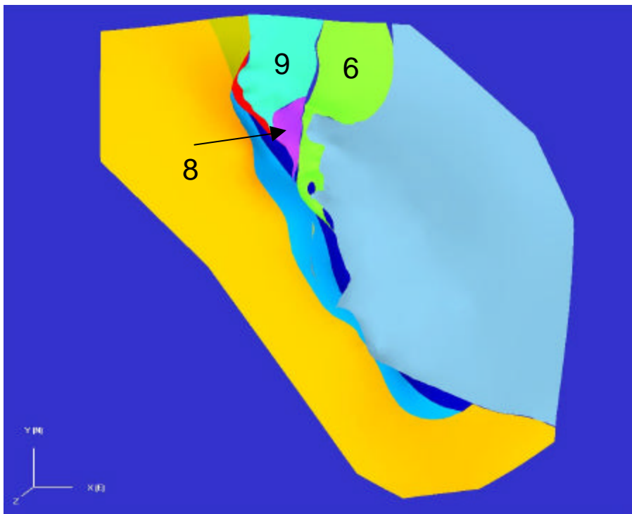
Figure 3-62. Structural blocks involved in the Bromide Tracer experiment in the Phosphoria Formation. Blocks 6, 8 and 9 are the uppermost imbricate fault blocks.
