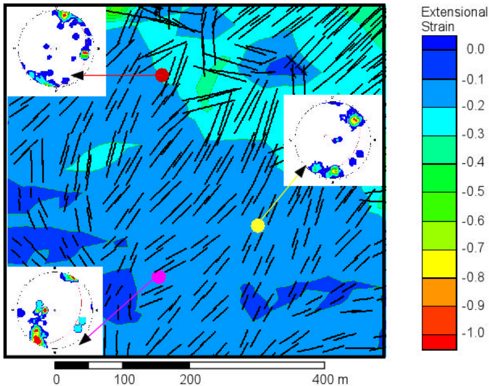
Figure 3-43. Comparison of extensional strain and fracture orientations measured at scanlines 7 (yellow circle), 8 (red circle) and 9 (violet circle). Black lines indicate trend of principal extension. Lines lengths are proportional to the magnitude of extension.
