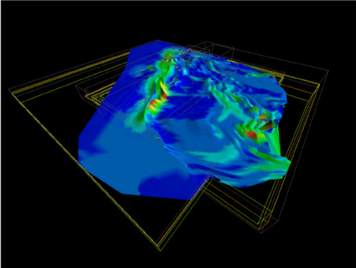
Figure 3-24 Completely restored Tensleep formation using Flexural Slip Unfolding. The color map reflect the amount of accumulated strain throughout the restoration process where blue colors are lowest recorded strains and the red are the highest.
