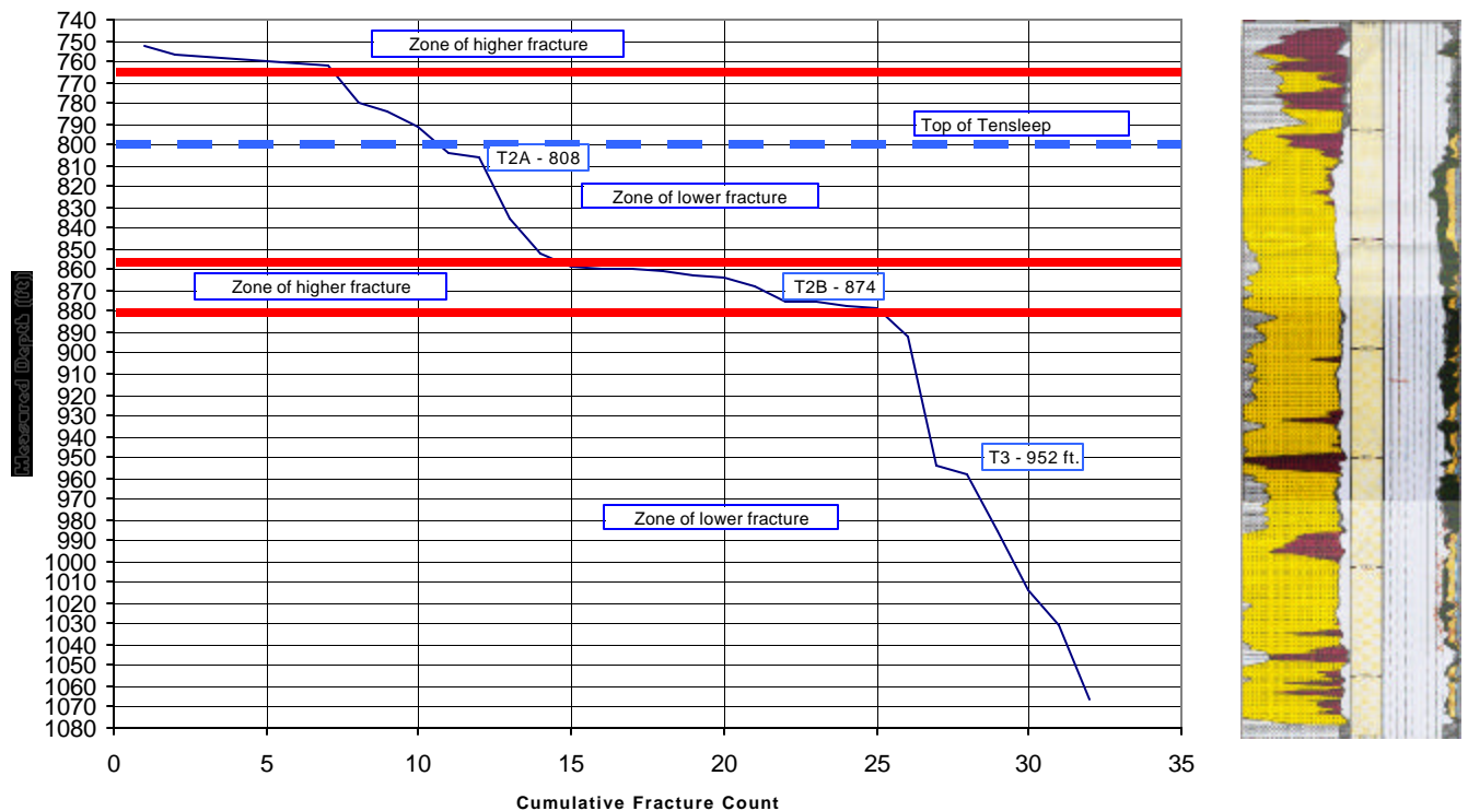
Figure 3-75. Cumulative fracture count for Shoshone 66-14 for fractures interpreted from image log. Red solid lines indicate alternating zones of higher and lower fracture intensity. Dashed blue line indicates the approximate top of the Tensleep Formation.
