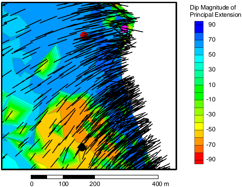
Figure 3-50. Plunge of principal direction of extension (contours) and trend of maximum extension direction around Scanlines 1, 2 (pink circle) 3 (red circle) and 4 (black circle). The contours show the amount of plunge of the principal direction of extension. Dark blue and orange/red shading indicates steep plunges. Black lines indicate trend of principal extension. Lines lengths are proportional to the magnitude of extension.
