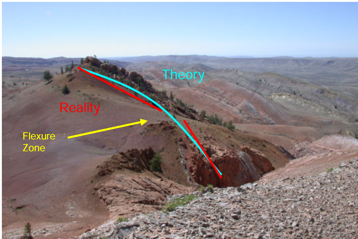
Figure 3-60. Example of a horizontal flexure zone. Most rock does not deform in a continuous curve (cyan-colored line), but rather as panels with more or less constant curvature that deform in zones of higher intensity fracturing or faulting between panels (red lines). The more highly fractured nature of these hinge zones typically leads to greater erosion on the surface.
