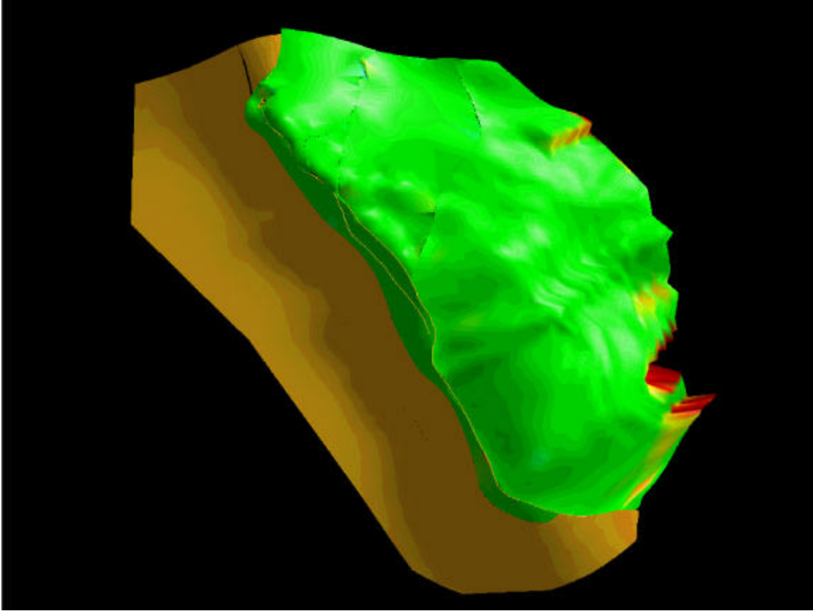
Figure 3-23 Illustration of the unfaulted Tensleep formation showing fault blocks 1, 6, 8, 9, 11 and 14 in green color as part of the overthrust and the top of the anticline.
