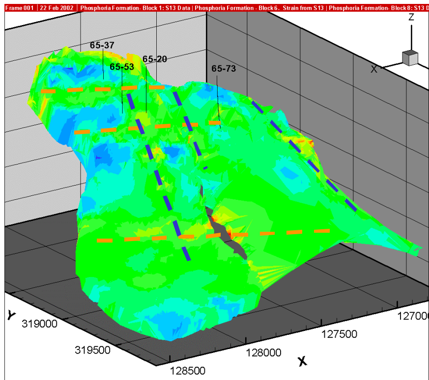
Figure 3-58. 3D view of imbricate blocks 6, 8 and 9 from the north looking south. The orange and blue dashed lines correspond to high strain corridors that separate the rock into panels that have more or less constant dip
