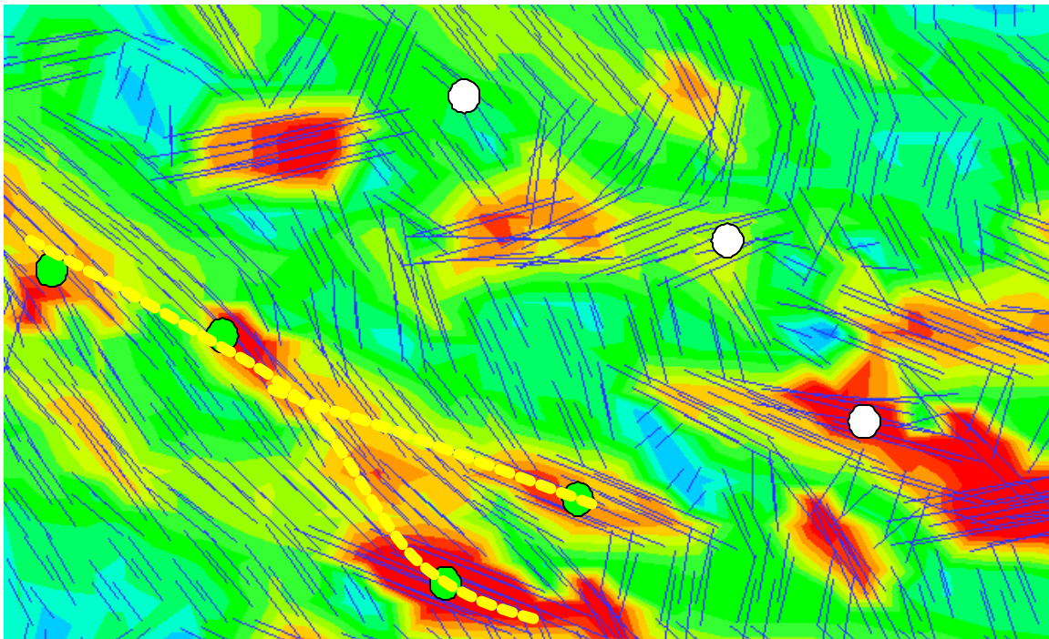
Figure 2-57. Hypothetical example of how strain maps and subsurface tracer data can be related to understand compartmentalization and tributary drainage. Green circle represent wells that appear to have strong pressure or flow connection in a tracer test, while white-shaded circle represent wells that appear disconnected. The contour colors denote the magnitude of strain, while the blue arrows indicate the trend of the dominant extensional fracture set predicted from the strain tensor.
