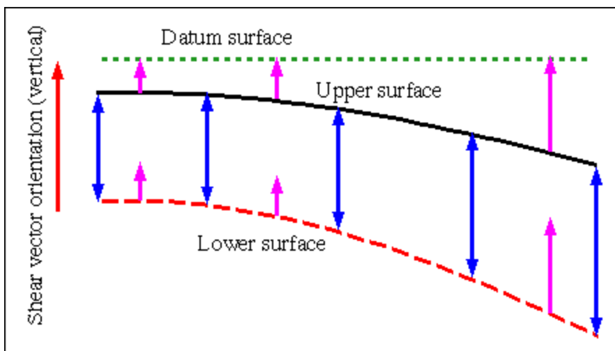
Figure 2-38 Cross-section through a hanging wall fold (from Midland Valley, 2000)
