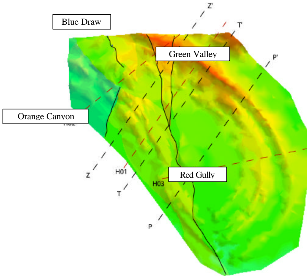
Figure 2-18. Picture showing the topography of Circle Ridge. The spectrum corresponds to elevation where red is the highest and green represents the lower parts. The fault traces of the Red Gully and Green Valley faults cross cut the whole field. Orange Canyon and Blue Draw are also shown in the NW part of the field. The cross-sections are shown as hatched lines. The P, T and Z sections were produced by Anderson and O'Connell (1993) and H01, H02 and H03 are the new cross-sections from the June field campaign.
