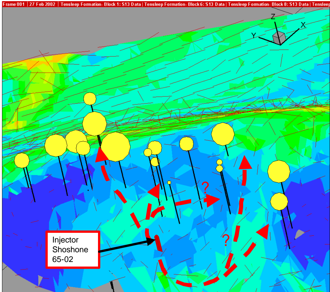
Figure 3-71. Time to breakthrough for only the wells in which a breakthrough response was observed. Radius of circle is proportional to time of breakthrough, so large circle indicate a longer time to breakthrough than small circles. Note that the responding wells tend to be in the high strain regions around the injector, and that the time to breakthrough is relatively short for the 5 wells in the center of the diagram nearest the injector, and increases along the red-dashed fracture corridors as indicated in the figure.
