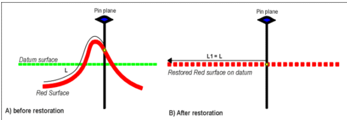
Figure 2-43 Maintaining sinuous line length with a vertical pin (from Midland Valley, 2000)
