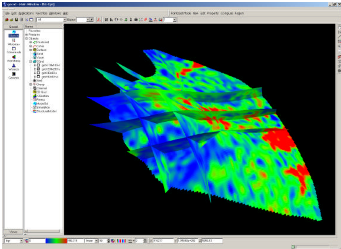
Figure 3-101. Distribution of fracture intensity in the Overthrust Block.
