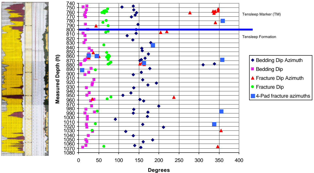
Figure 3-74. Orientation of fractures and bedding in Shoshone 66-14 interpreted from image logs. The top of the Tensleep Formation is shown by the solid blue line.
