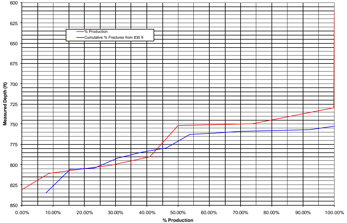
Figure 3-78. Comparison of cumulative fracture intensity and cumulative production from Shoshone 66-14. The red line is the % production from the spinner survey data. The blue line is the cumulative percent of fractures starting at a depth of 835 ft. (there were not enough 4-pad fractures to plot this component separately).
