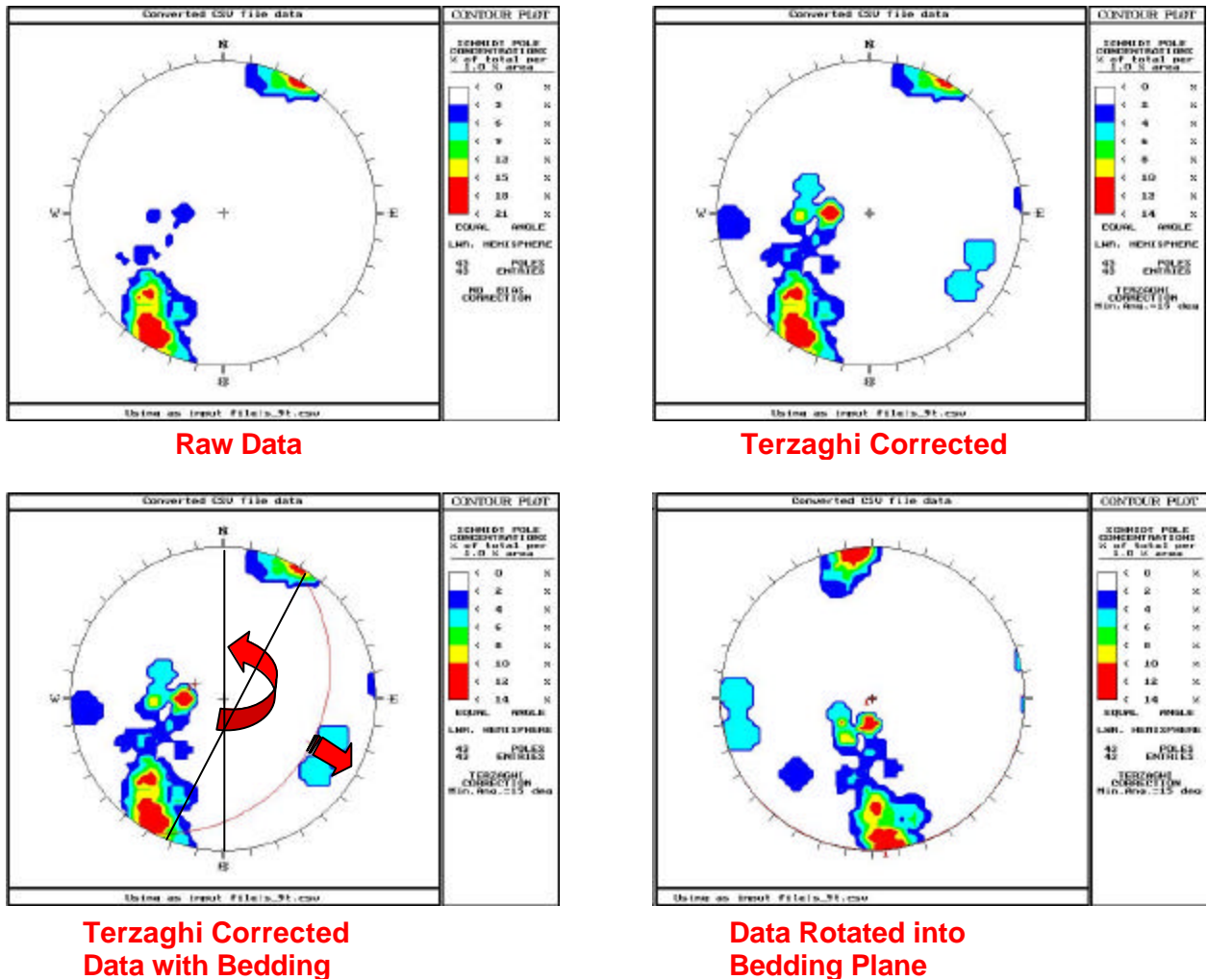
Figure 2-22. Analysis of fracture orientations, including rotation into bedding plane.
