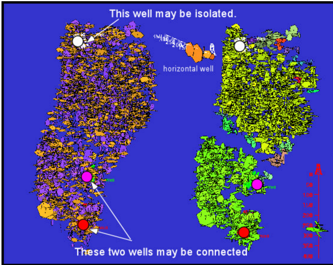
Figure 2-56. DFN model for subthrust block 6, showing fracture compartments formed due to variation in intensity related to folding. The diagram on the left shows all fractures and three vertical well locations. The diagram on the right shows the fracture compartments.
