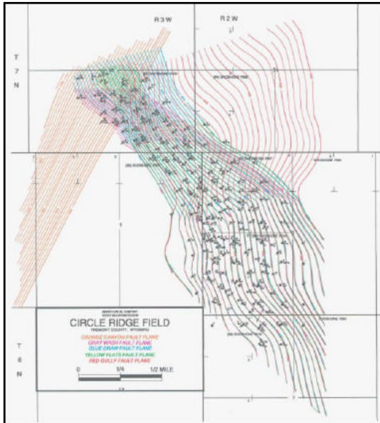
Figure 4-3. Visualization of fault surfaces prior to this project.
