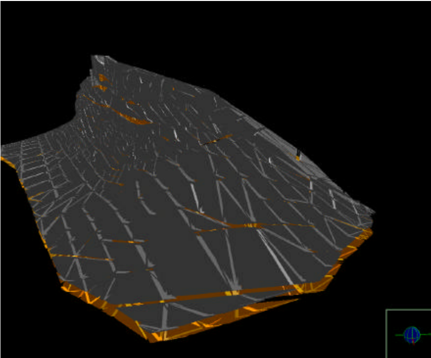
Figure 3-22 Phosphoria and Tensleep volume elements
