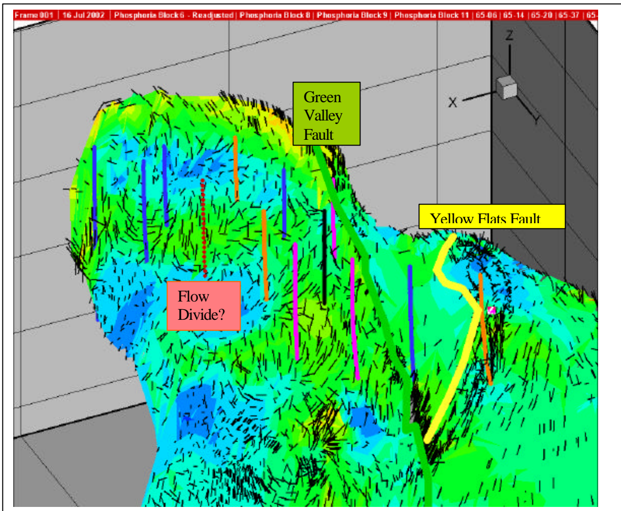
Figure 3-66. Fracture strikes inferred from strain field. Black lines indicate strike of dominant extensional fracture set, while length of line and color of contour indicates the magnitude of extensional strain. Wells are color-coded according to result and completion interval: black = injector; purple = Tensleep but no Phosphoria completion; blue = Phosphoria completion but no response; orange = Phosphoria completion and breakthrough observed.
