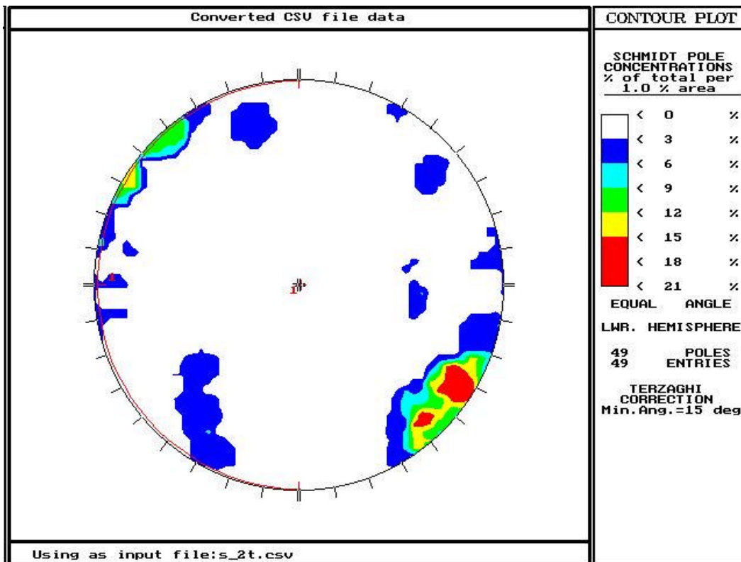
Figure 3-29. Stereoplot for Scanline 2, rotated relative to bedding plane.
