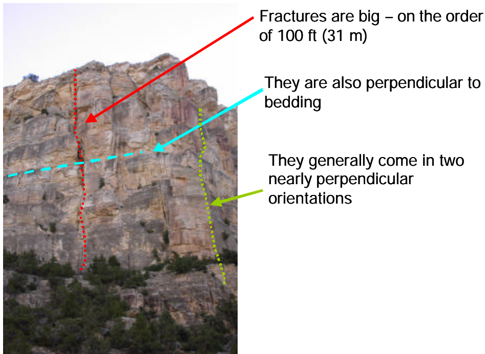
Figure 3-96. Outcrop of Tensleep Sandstone in the Wind River Canyon.
