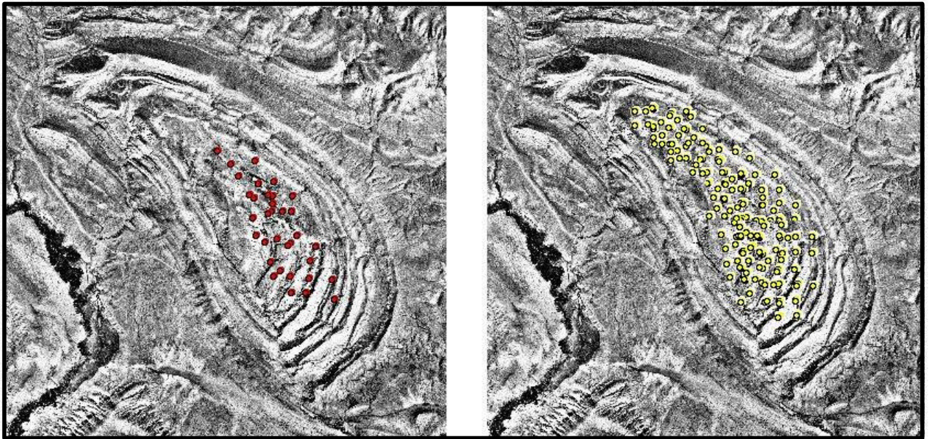
Figure 3-1. Expansion of matrix property data through re-calibration of older logs. Photograph on left shows wells (red circles) where modern logs had previously made it possible to calculate matrix porosity and oil saturation. Photograph on right shows wells (yellow circles) in which re-calibrated logs were used to estimate matrix properties.
