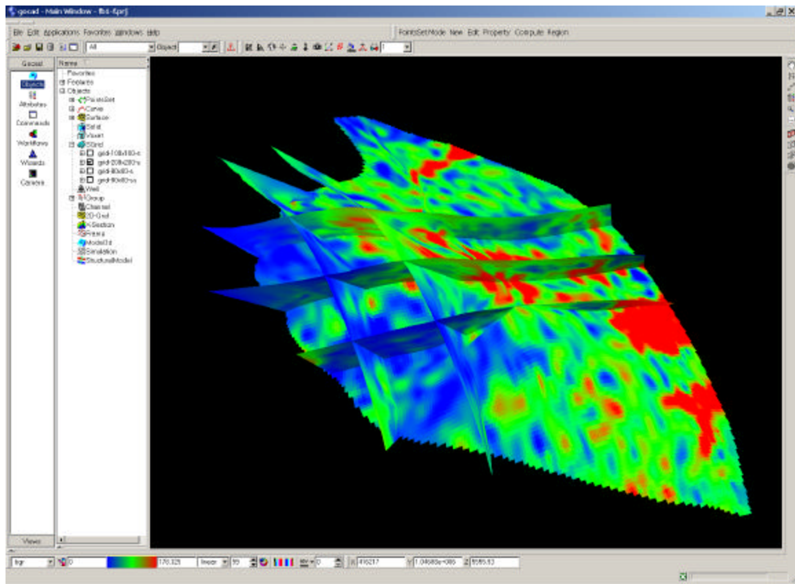
Figure 3-100. Distribution of fracture porosity in the Overthrust Block.
