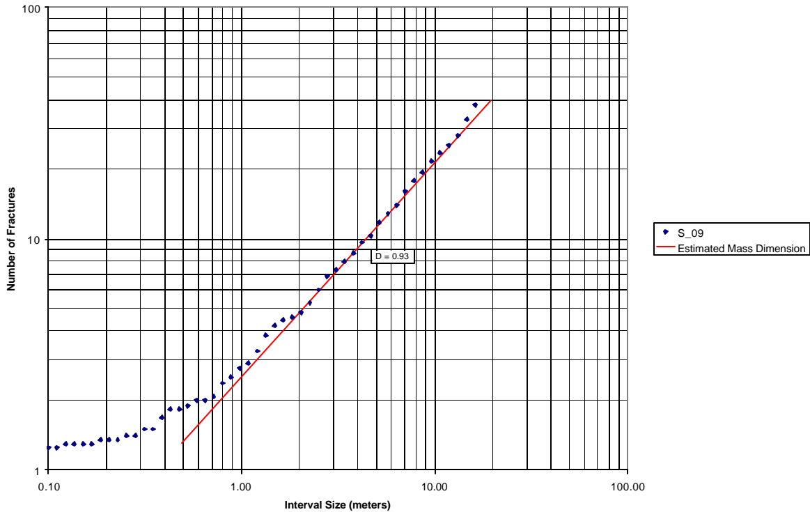
Figure 2-25. Example of a plot to determine the intensity scaling characteristics of fracture data collected along a scanline.
