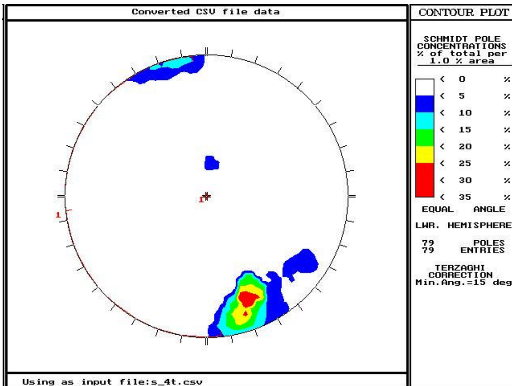
Figure 3-31. Stereoplot for Scanline 4, rotated relative to bedding plane.
