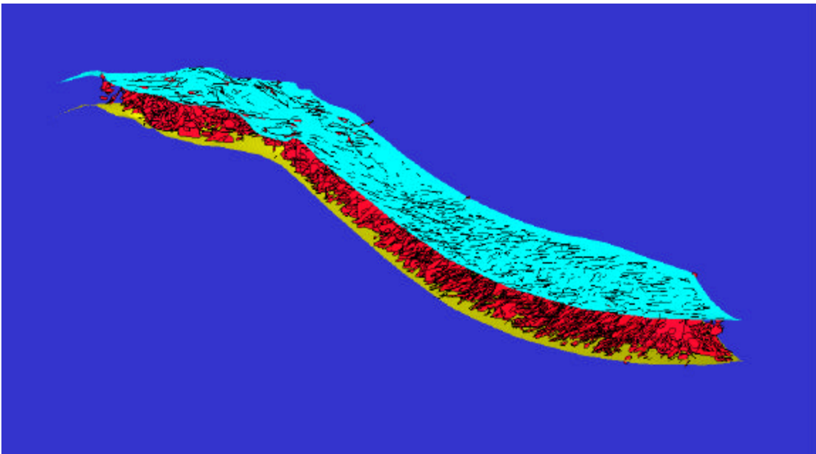
Figure 2-61. Example of fracture set clipped against upper and lower boundaries of Tensleep Formation, Block 6.
