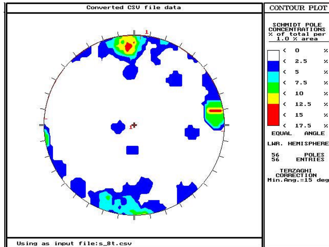
Figure 3-35. Stereoplot for Scanline 5, rotated relative to bedding plane.
