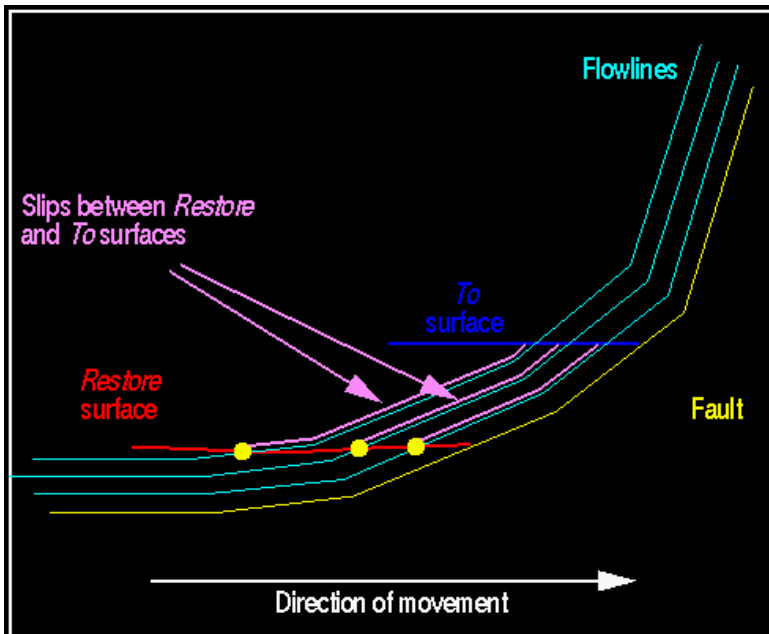
Figure 2-37 Implications of the Restore-to-Surface movement method (from Midland Valley, 2000)
