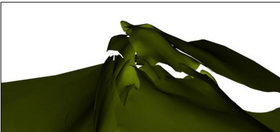
Figure 3-10 Illustration of the undulating extension of the top of the Phosphoria formation. The undulation of the surface is controlled by well top information from the Anderson and O’Connell database.
