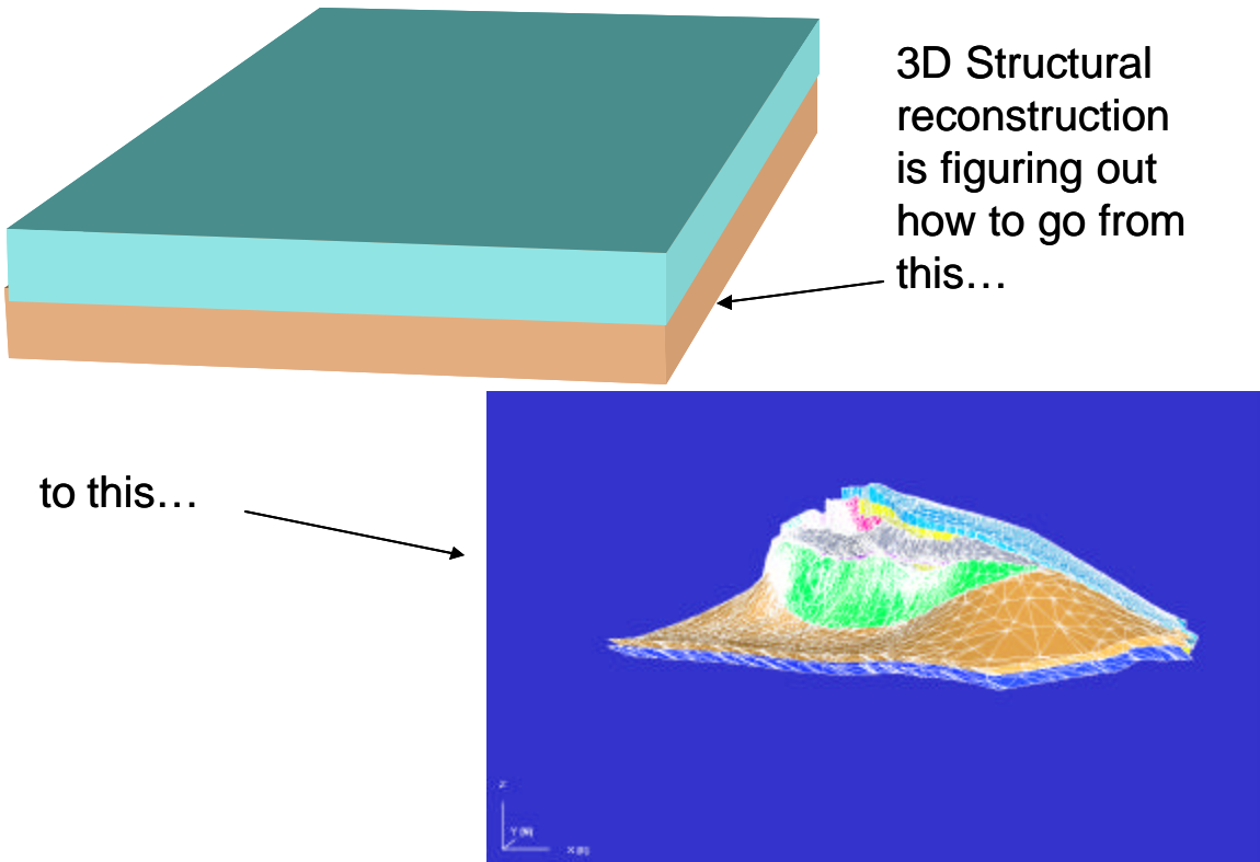
Figure 2-26. Illustration of the structural restoration process.
