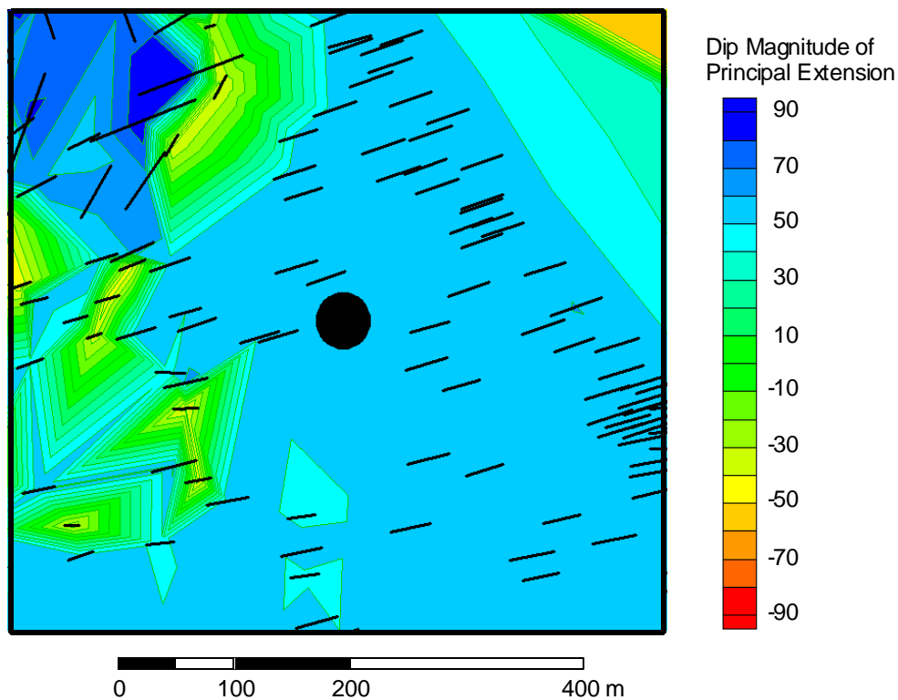
Figure 3-48. Plunge of principal direction of extension (contours) and trend of maximum extension direction around Scanline 11. The contours show the amount of plunge of the principal direction of extension. Light blue shading indicates shallow plunges. Black lines indicate trend of principal extension. Lines lengths are proportional to the magnitude of extension.
