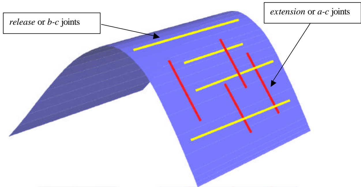
Figure 1-11. Illustration of release (b-c) and extension (a-c) joints in relation to fold geometry.
