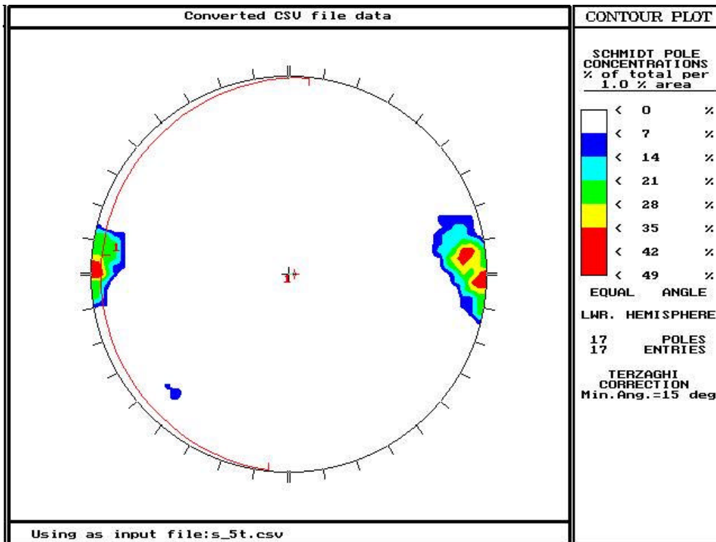
Figure 3-32. Stereoplot for Scanline 5, rotated relative to bedding plane.
