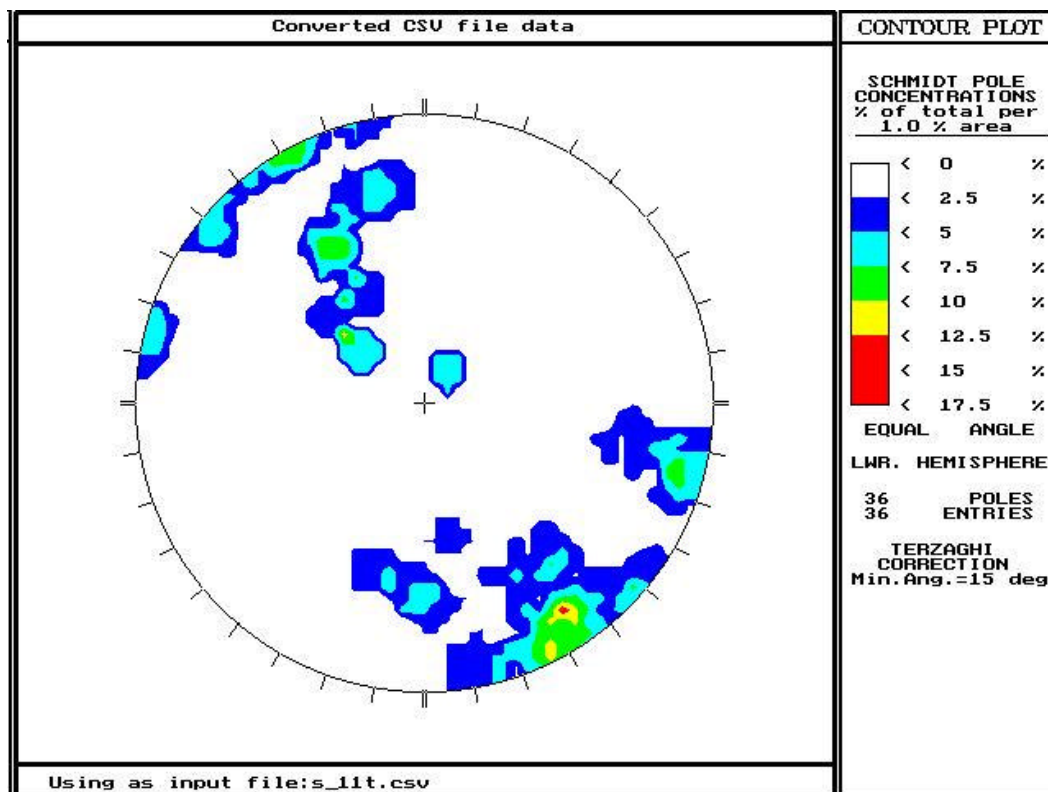
Figure 3-37. Stereoplot for Scanline 11, rotated relative to bedding plane.
