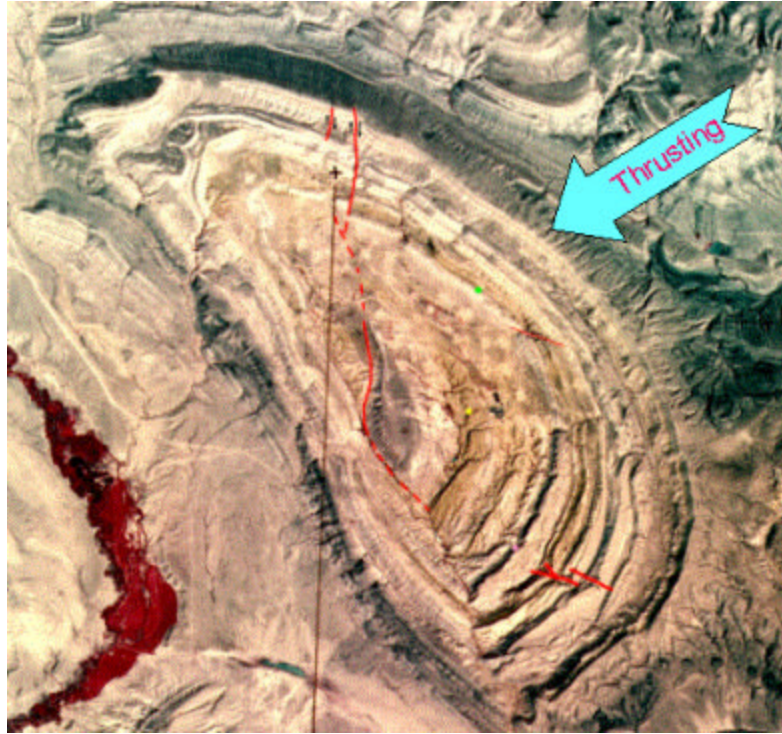
Figure 1-7. False-color satellite photo of the Circle Ridge Field. The Field formed due to compression and thrusting from the northeast. Note the increased shortening in the northwestern end of the Field. The increased shortening was accommodated through tighter folding and imbricate faulting.
