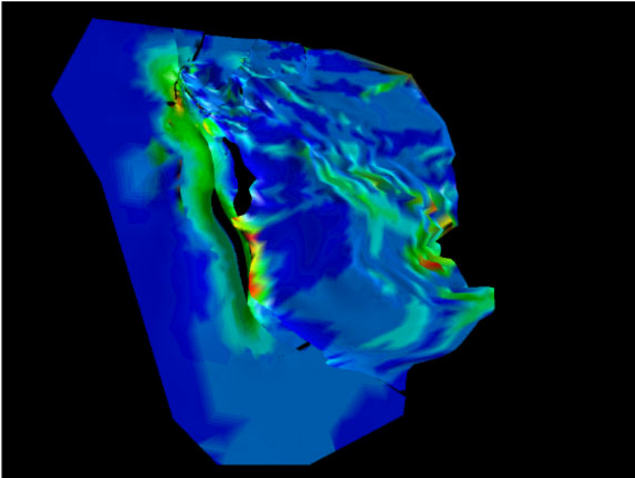
Figure 3-26 Vertical Shear Unfolding of the unfaulted Phosphoria formation (top view). The color map shows the accumulated strain, with blue colors showing the lowest recorded strains and the red colors the highest.
