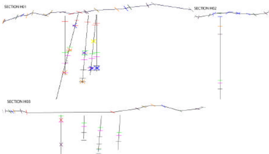
Figure 2-28. Cross-sections H01, H02 and H03 performed by the project team during the June 2000 field campaign.
