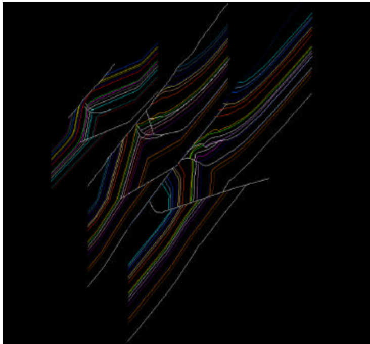
Figure 2-27. Perspective view of the Anderson and O’Connell (1993) P, T and Z sections as they appear in the 3D model.
