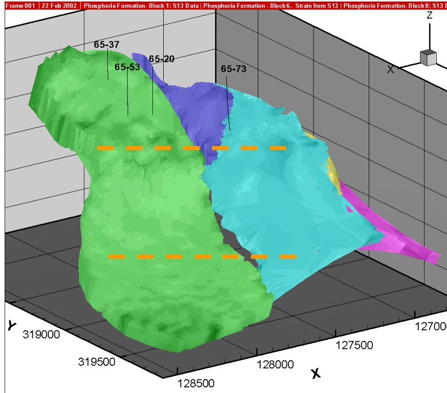
Figure 3-59. 3D view of imbricate blocks and illustration of two horizontal “hinges” or flexure zones (orange dashed lines) formed during the initial folding of the field.
