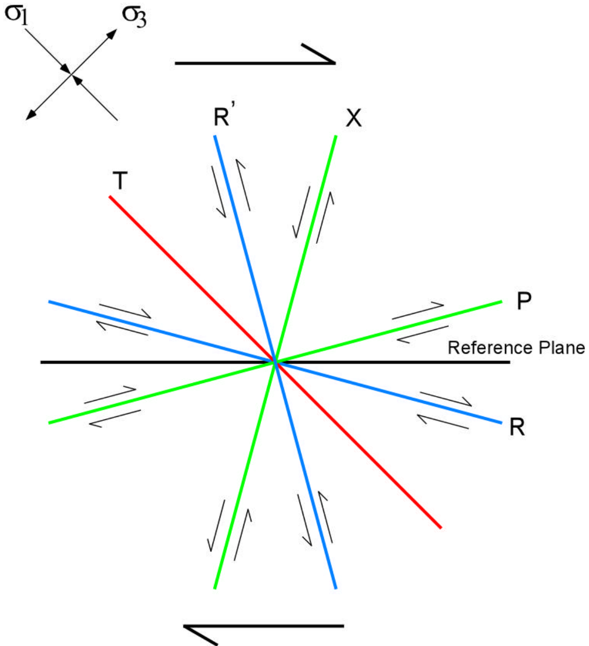
Figure 1-10. Relation between principal stress directions and resultant fracture orientations (Riedel, 1929). \sigma_1 and \sigma_3 are the maximum and minimum principal stresses, respectively. “T” is the extension (Mode I) joint set. “R” and “R'” are the primary and secondary Riedel shears, which are active in compression, typically when the deformation occurs deep in the crust, pore pressures are low and the angle between \sigma_1 and the reference fault plane is large. At shallow depths, low confining pressures, high pore pressures or when the master fault subparallels \sigma_1 , the “P”, “X” and “T” sets are favored.
