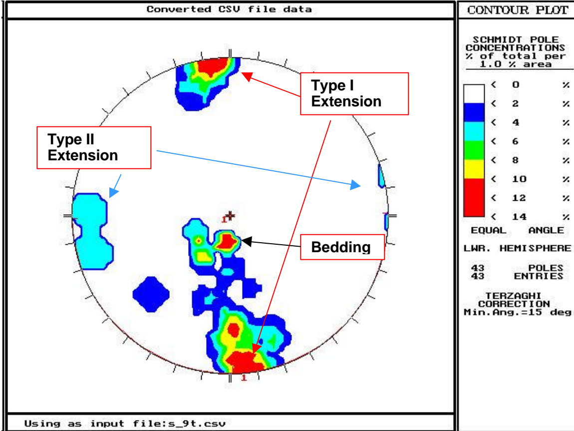
Figure 2-23. Example of possible interpretation of fracture orientations relative to bedding orientation.
