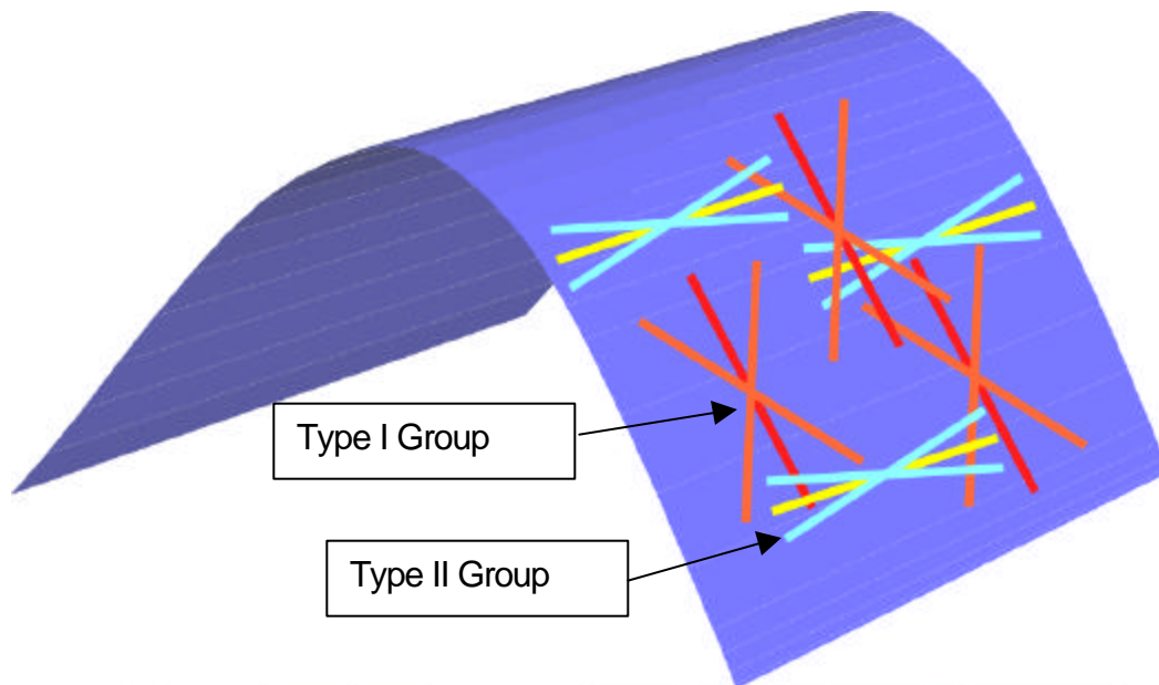
Figure 1-12. Schematic diagram of Stearns model of fracture orientations related to folding. The red line in the Type I fracture group is a joint or extension fracture, while the orange lines show the orientations of Type I conjugate “shear” fractures. The yellow line shows the orientation of the Type II joint or extension fracture, while the cyan lines show the orientations of the Type II conjugate “shear” fractures. The complete Stearns model contains other fractures not shown in the schematic above.
