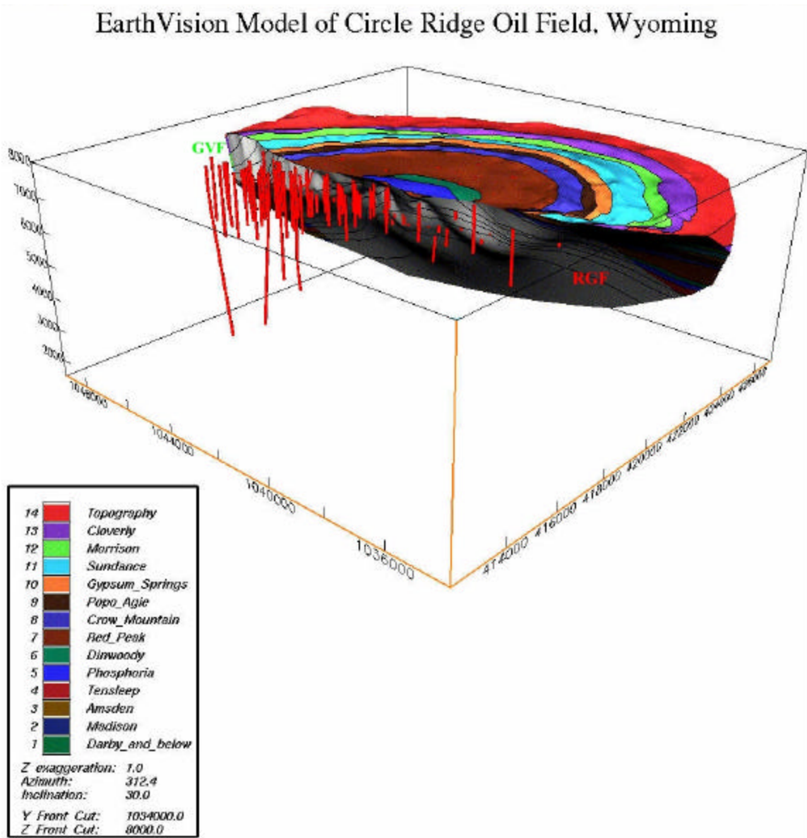
Figure 2-31 Overthrust block at Circle Ridge after Smith (2000).
