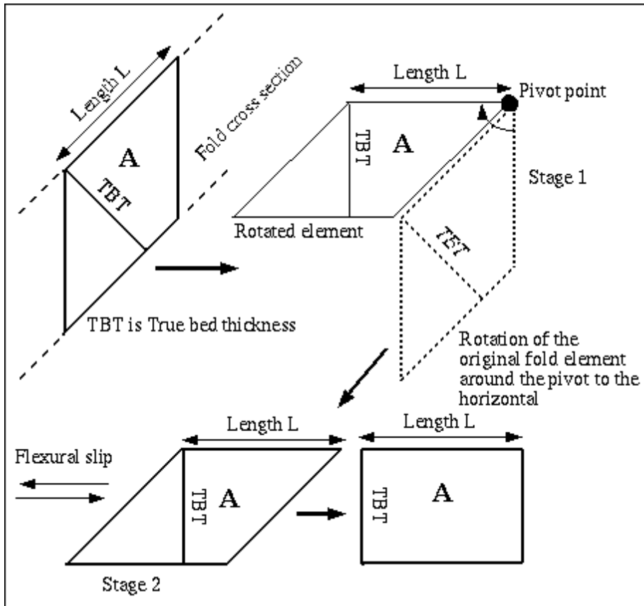
Figure 2-41 Illustration of the flexural slip unfolding algorithm (from Midland Valley, 2000)
