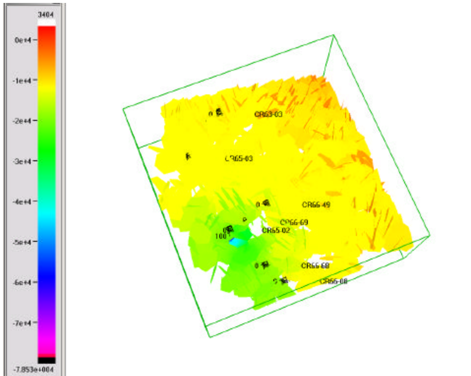
Figure 3-87. Pressure snapshot of injection in regional model with permeability ratio Set1:S
