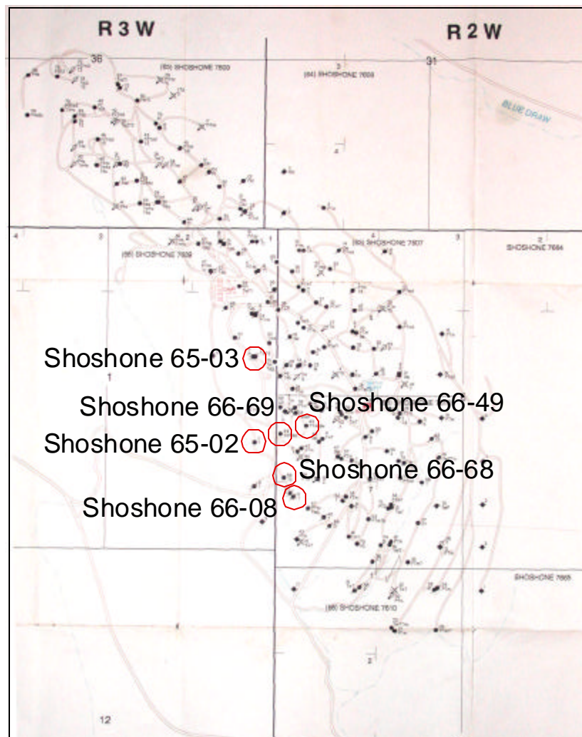
Figure 2-53. Location of wells in which Bottom Hole Pressures (BHP) were monitored during the Nitrogen Injection experiment. Shoshone 65-02 was the injector.
