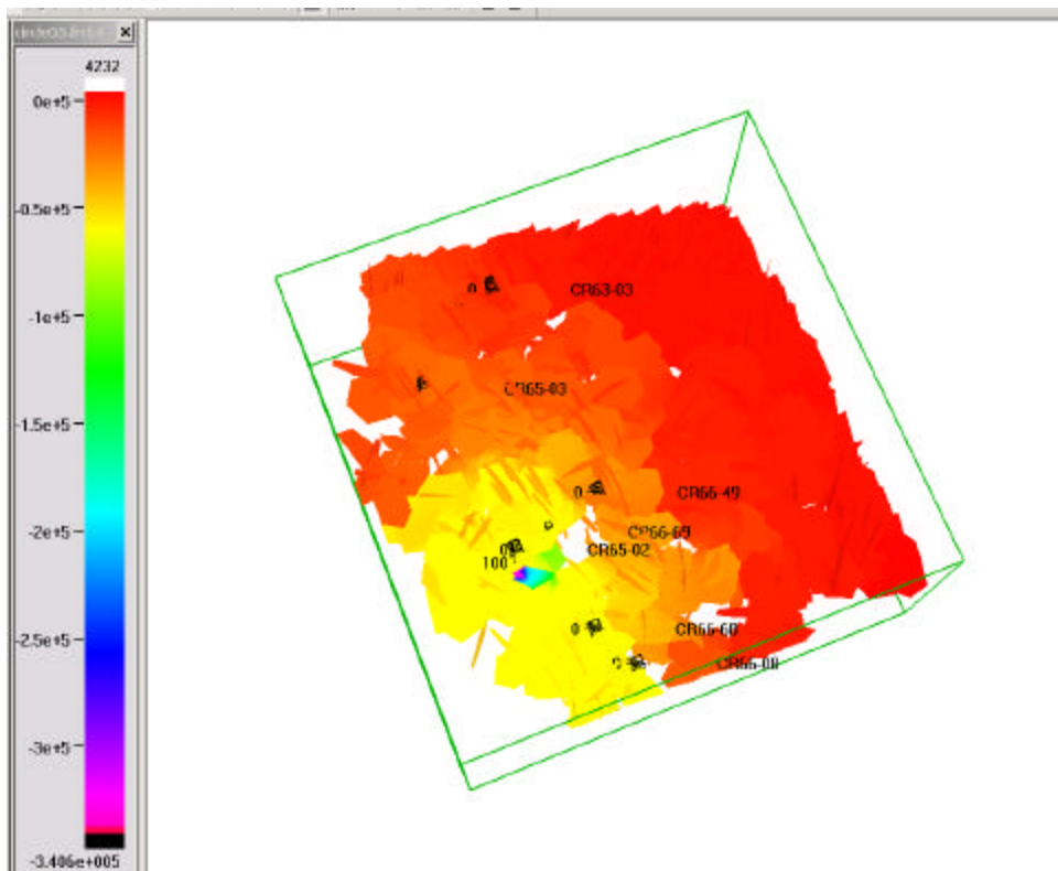
Figure 3-88. Pressure snapshot of injection in regional model permeability ratio Set1:Set2 = 10. This simulation shows earlier pressure breakthrough to the north-west and south-east rather than to the north-east set2 = 1
