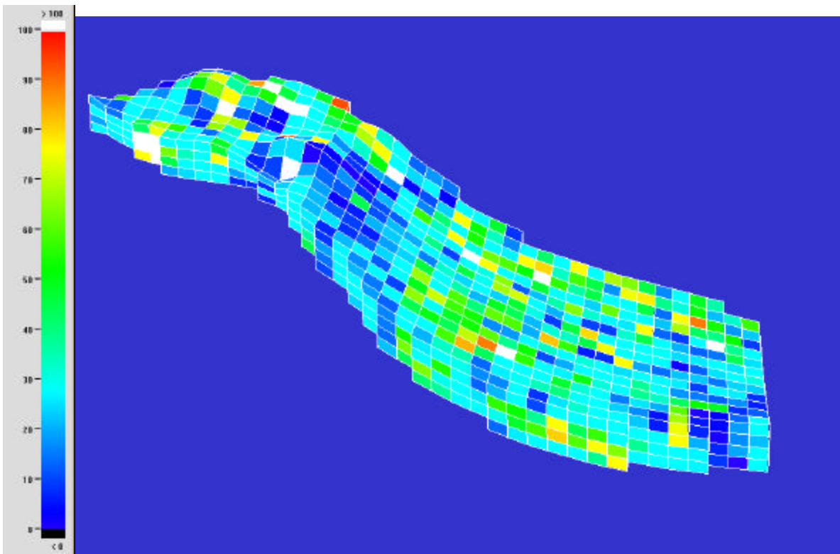
Figure 2-65. Values of vertical permeability calculated for grid shown in Figure 2-64. Values are in mD.
