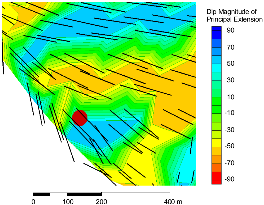
Figure 3-46. Plunge of principal direction of extension (contours) and trend of maximum extension direction. The contours show the amount of plunge of the principal direction of extension. Green shading indicates very shallow plunges. Black lines indicate trend of principal extension. Lines lengths are proportional to the magnitude of extension.
