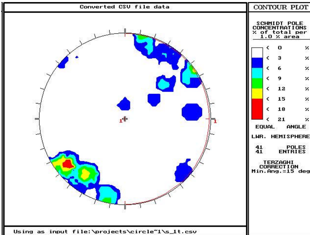
Figure 3-28. Stereoplot for Scanline 1, rotated relative to bedding plane.
