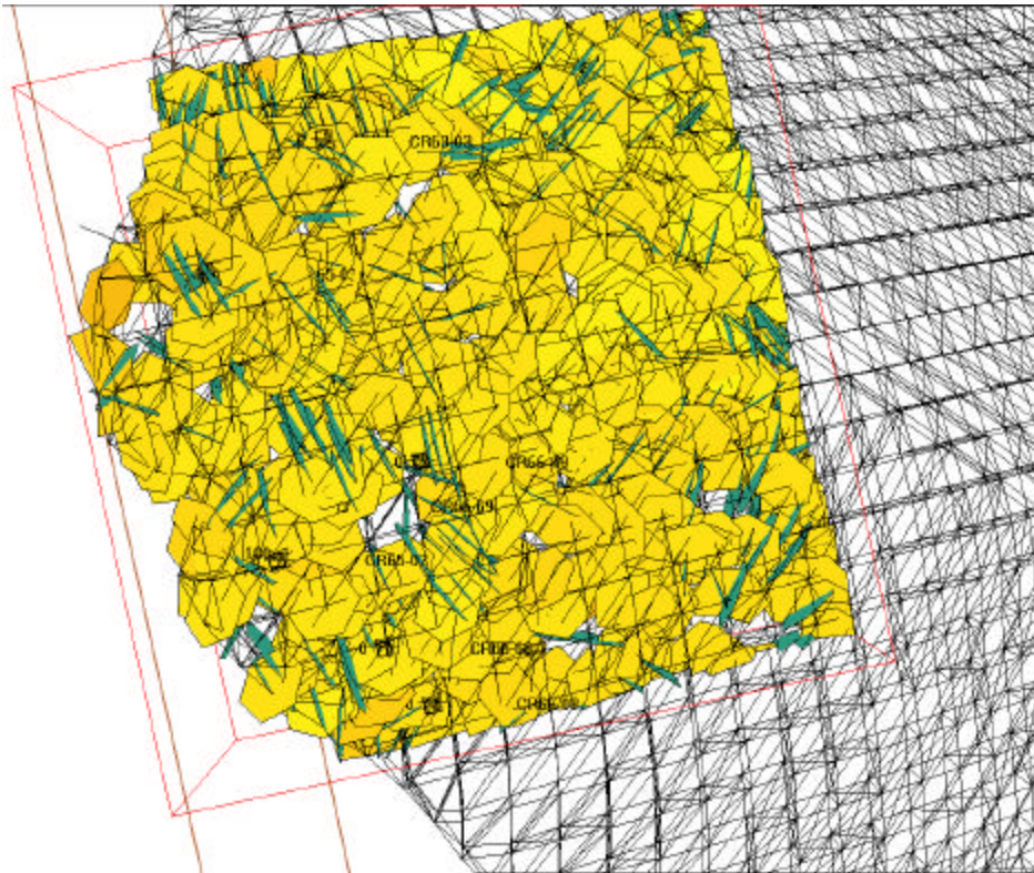
Figure 3-85. Regional scale DFN model populated by strain perpendicular and strain parallel fracture sets.
