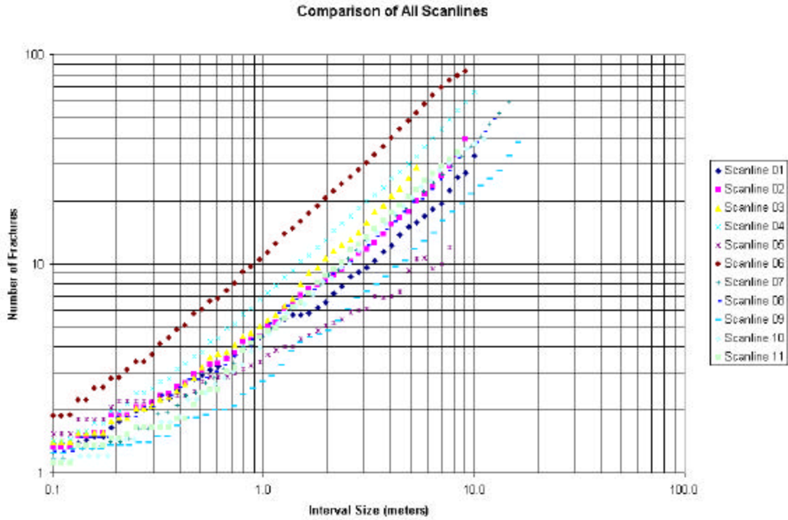
Figure 3-39. Composite plot of mass dimension calculations for all 11 scanlines.
