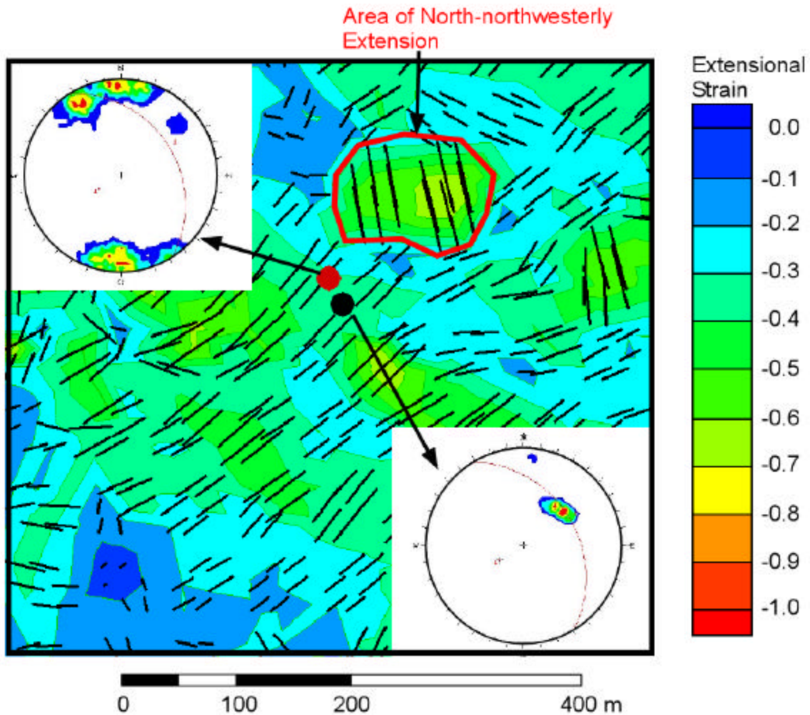
Figure 3-41. Fracture orientations measured at scanlines 6 (red circle) and 5 (black circle). Black lines indicate trend of principal extension. Lines lengths are proportional to the magnitude of extension.
