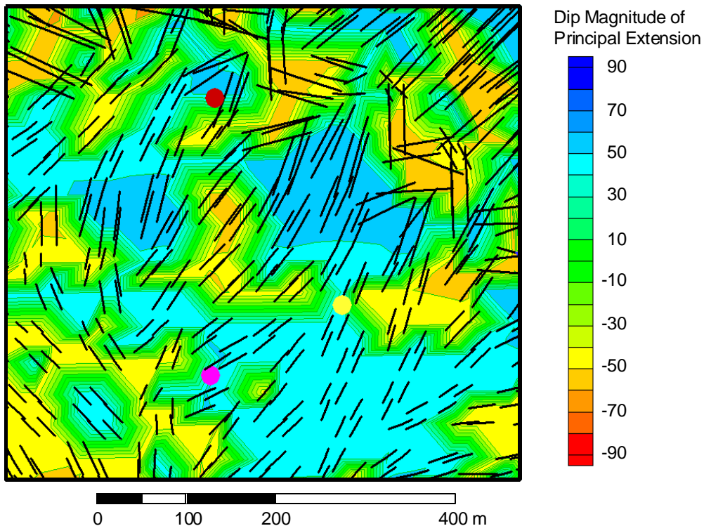
Figure 3-44. Plunge of principal direction of extension (contours) and trend of maximum extension direction. Green shading indicates very shallow plunges. The three scanlines generally are in the vicinity of very shallow plunges, varying from -30^{\circ} to +30^{\circ} . This is consistent with the steep dips shown by all of the major joint sets in Scanlines 7, 8 and 9. Black lines indicate trend of principal extension. Lines lengths are proportional to the magnitude of extension.
