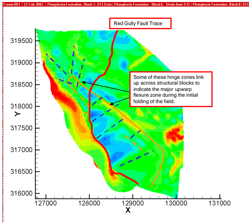
Figure 3-73. Strain pattern and the development of dip-parallel and strike parallel hinge zones.
