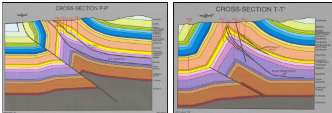
Figure 4-1. Two of three structural cross-sections prepared by Anderson and O'Connell for the Circle Ridge Field.
