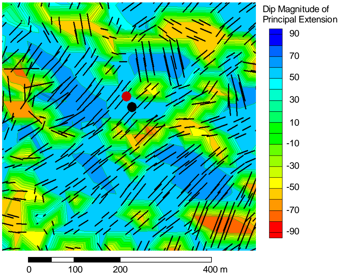
Figure 3-42. Plunge of principal direction of extension (contours) and trend of maximum extension direction. Plunge at Scanline 6 (red circle) is about 50° to the northeast. Plunge at Scanline 5 (black circle) is similar. Black lines indicate trend of principal extension. Lines lengths are proportional to the magnitude of extension.
