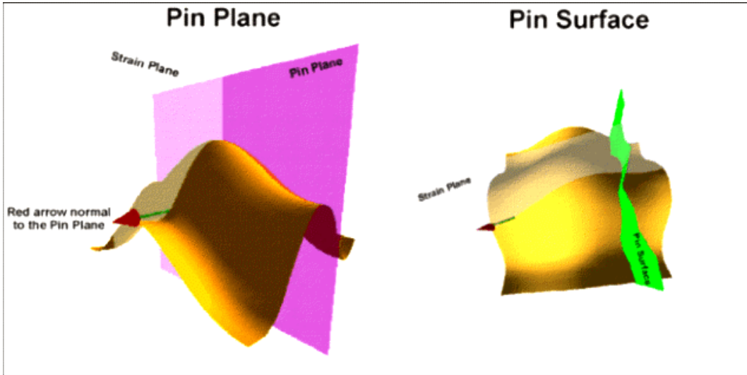
Figure 2-42 Orientation of the pin plane/surface and strain plane. Red arrow indicates the unfolding direction (from Midland Valley, 2000)
