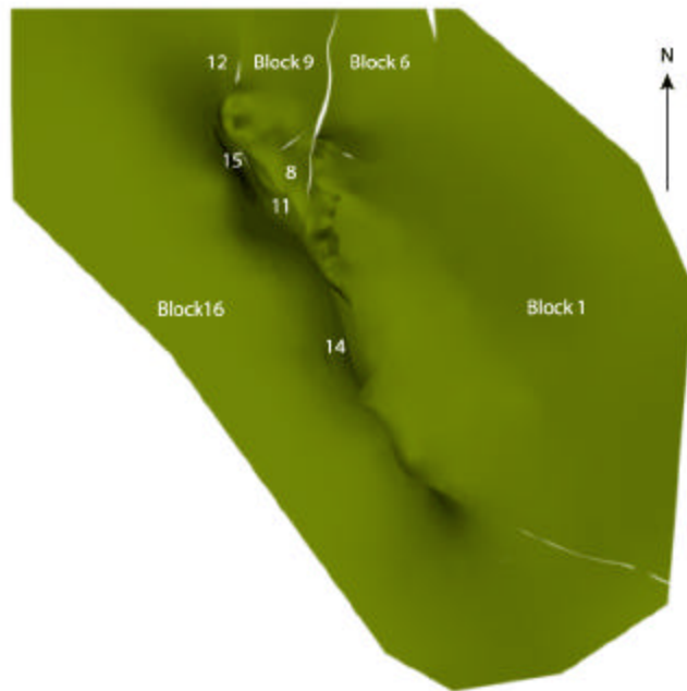
Figure 3-9 Top view of the location of major fault blocks in the Phosphoria formation.
