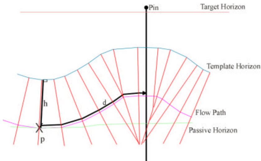
Figure 2-44 Illustration of the bed linkage and the slip system for each vertex in the deformed formation (from Midland Valley, 2000)
