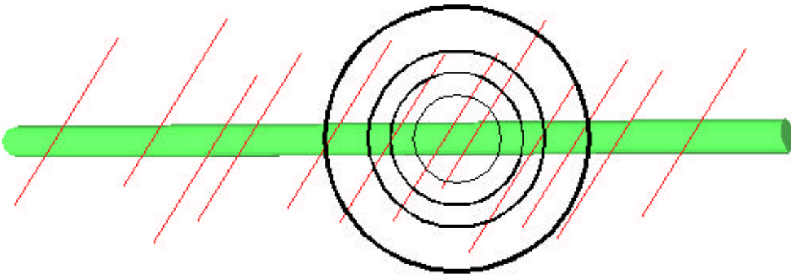
Figure 2-24. Methodology for calculating intensity scaling parameters.
