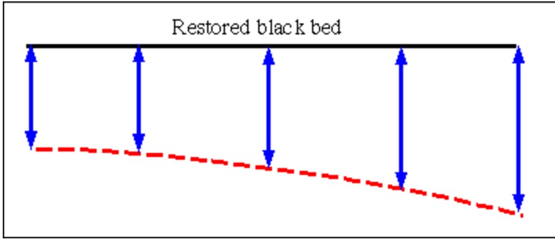
Figure 2-39 Cross-section through the restored hanging wall fold (from Midland Valley, 2000)
