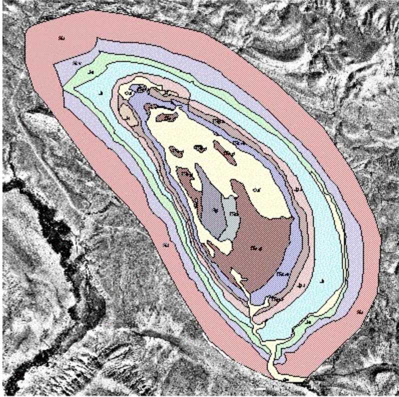
Figure 1-9. Geologic map (from Smith, 2000). Geological symbols used in map are referenced in Figure 1-8.
