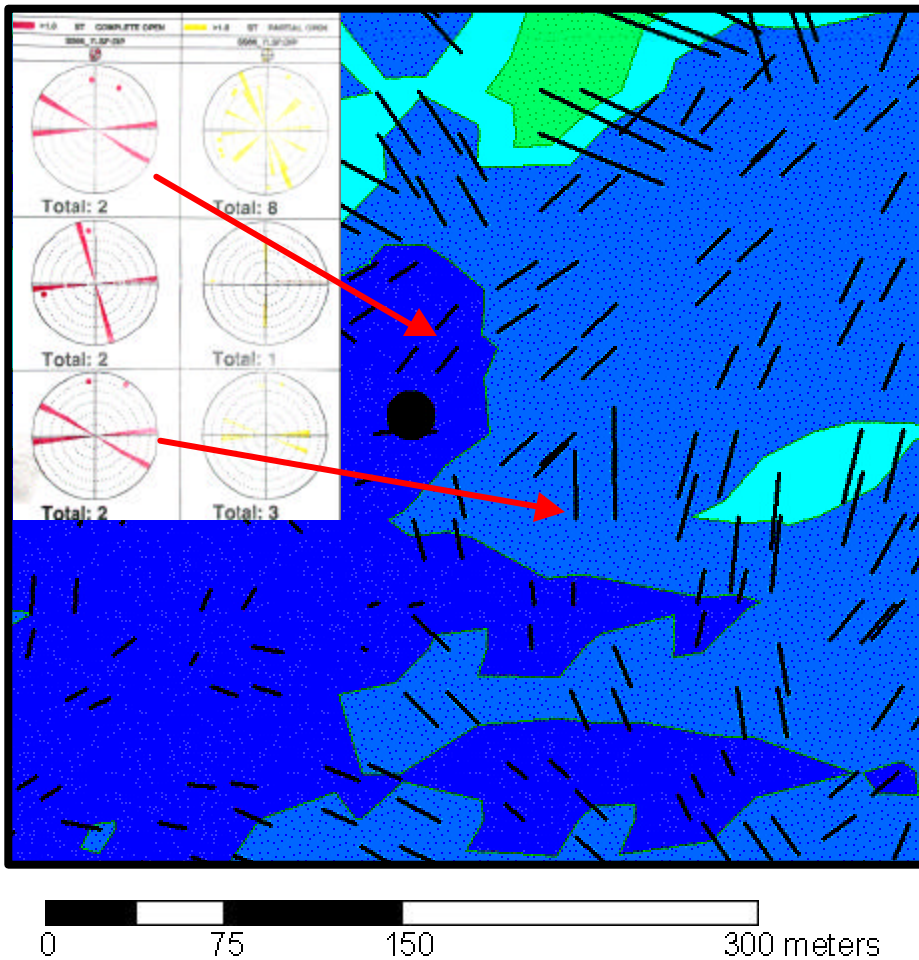
Figure 3-55. Comparison of fracture orientations in Shoshone 66-07 with direction of maximum extension.
