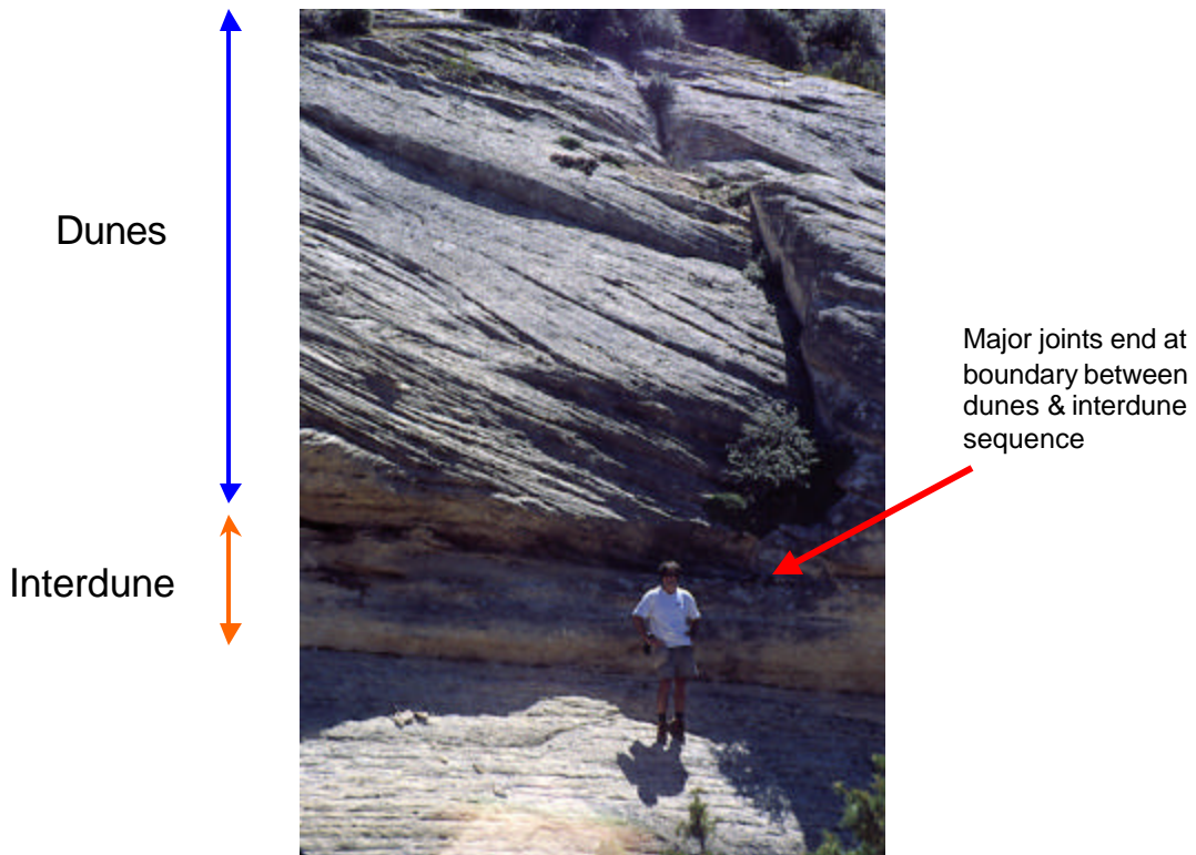
Figure 3-65. Large-scale fracturing in the upper Tensleep Formation at Zeisman dome. Upper photo shows large joints that extend from the top of the dune sequence to the bottom of the dune sequence, but consistently terminate at the boundaries of the dune sequence (lower photo).
