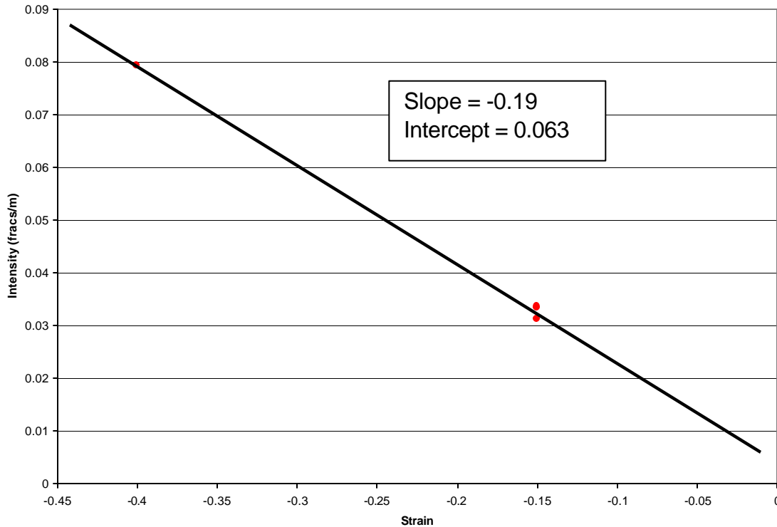
Figure 3-56. Graph of fracture intensity vs. extensional strain magnitude.
