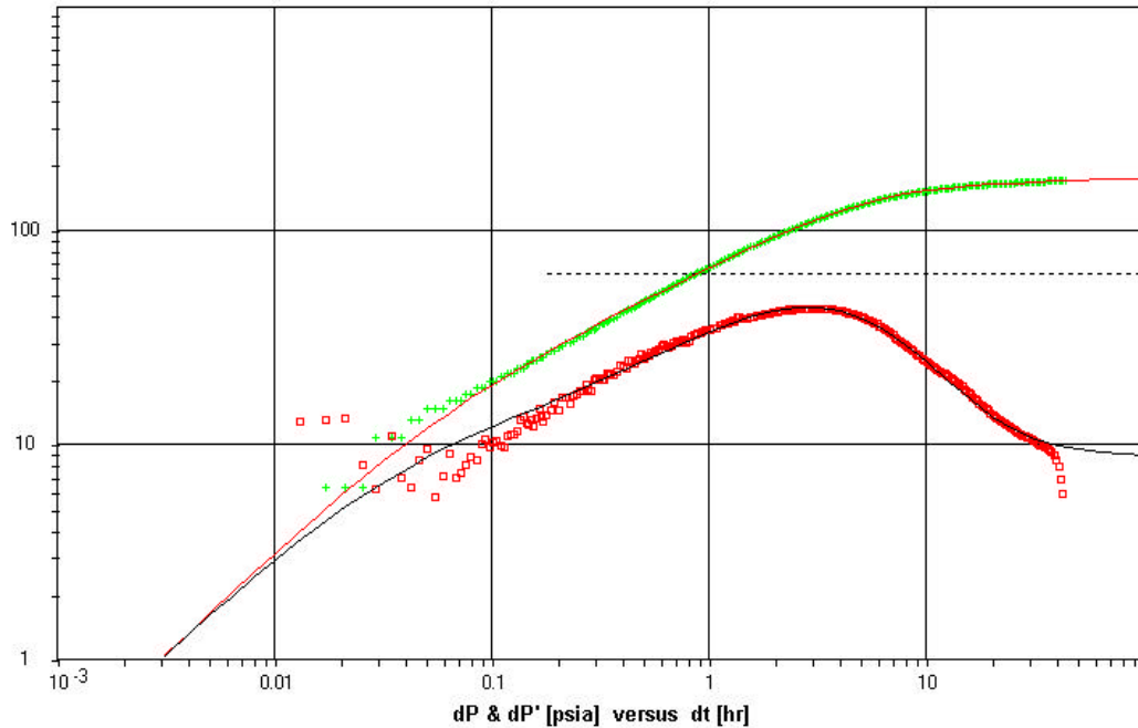
Figure 3-95. Fall-off curve for Shoshone 65-20.
