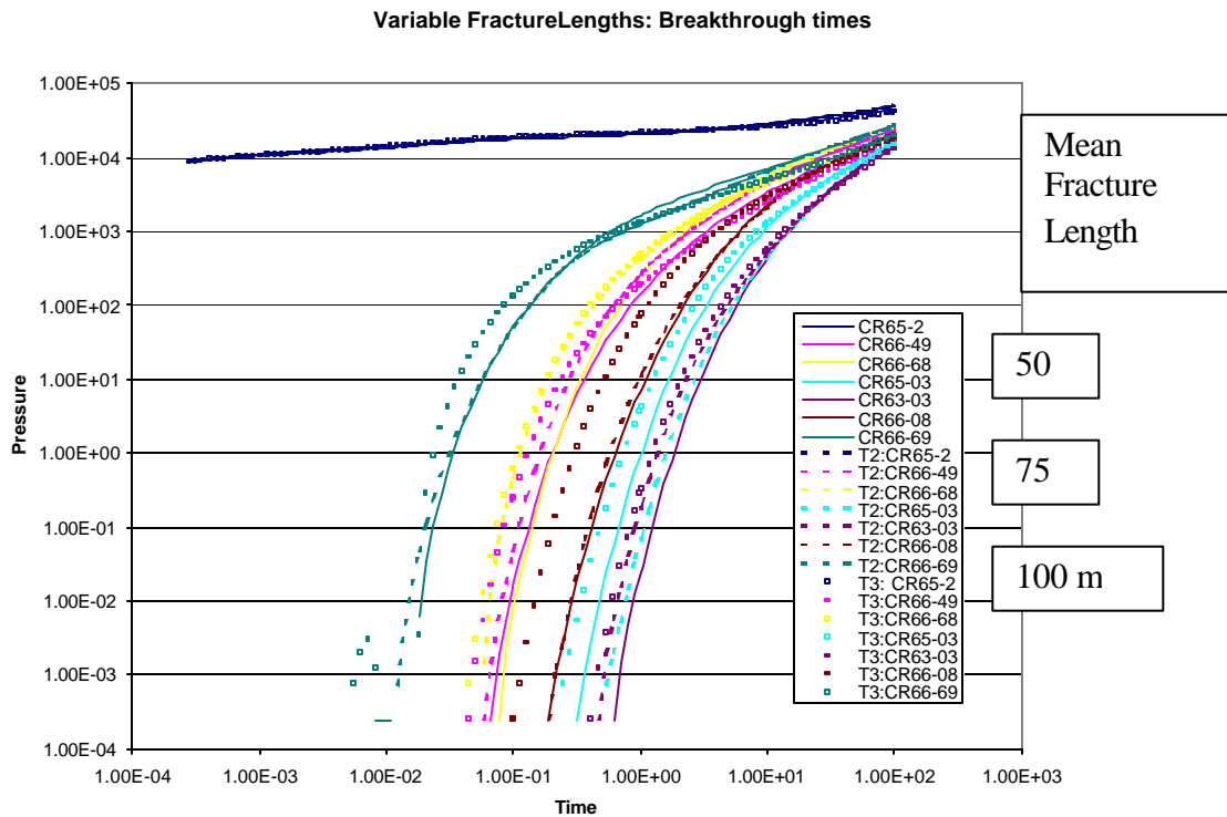
Figure 3-93. Relative breakthrough curves as a function of fracture length.
