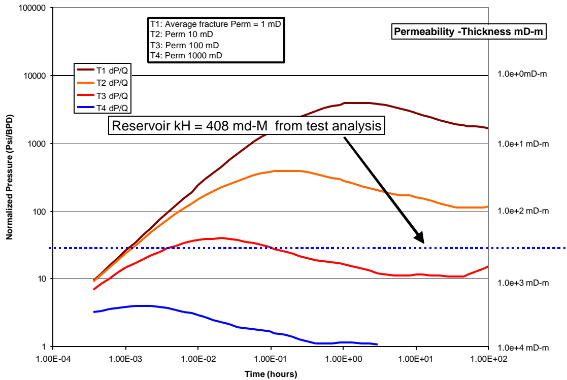
Figure 3-83. Permeability thickness values based on late-time derivative curves
