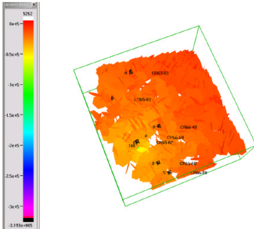
Figure 3-89. Permeability ratio Set1:Set2 = 0.1.
