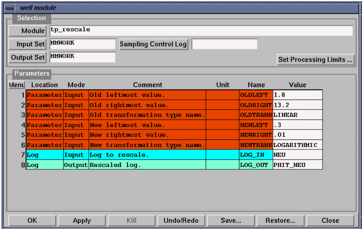
Figure 2-17. Rescale module with representative settings for the GRN count rate (NEU) to porosity (PHIT_NEU), Shoshone 66-34.
