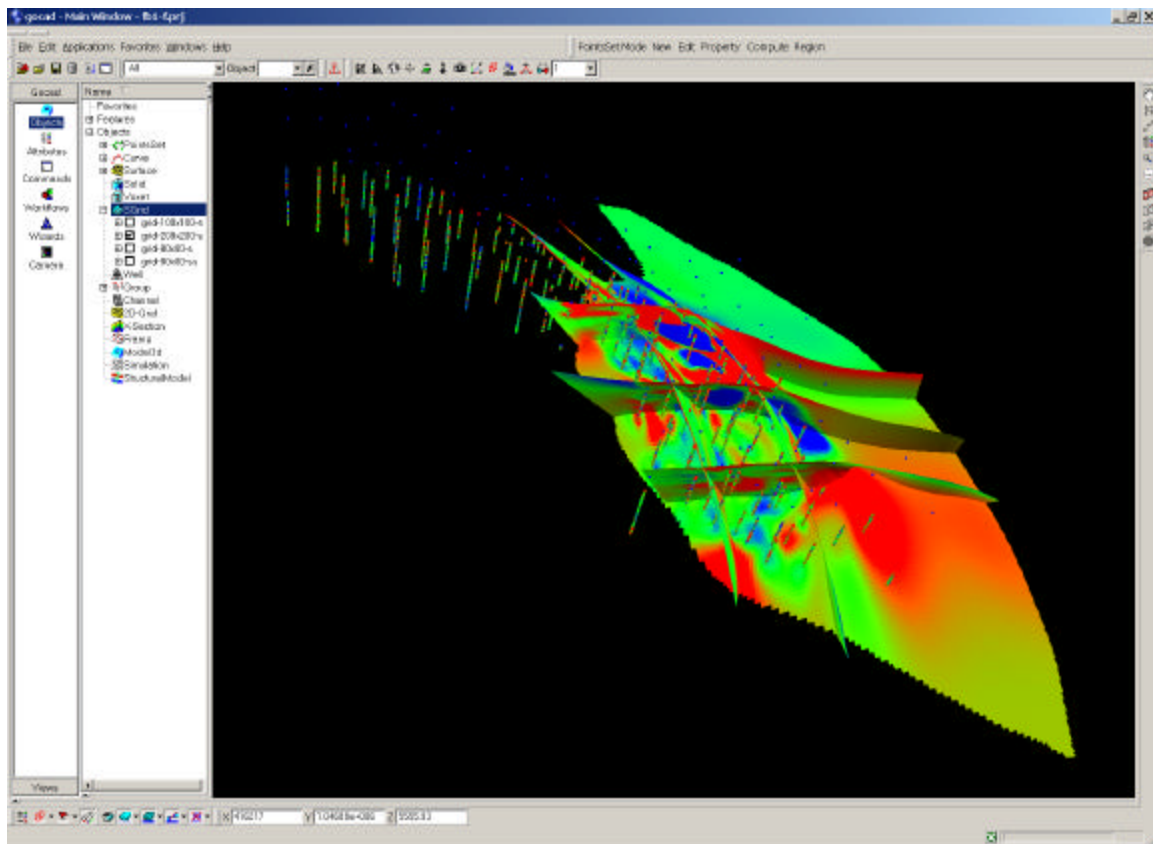
Figure 3-99. Matrix porosity distributed from well data in the Overthrust Block. The colors represent the value of the porosity. The wells used to create the model are also shown, and the colors in these wells indicate the value of matrix porosity calculated from the wireline log suite. The subvertical surfaces shown are not faults, but rather fence displays of the matrix porosity to help visualize the three-dimensional distribution of the data.
