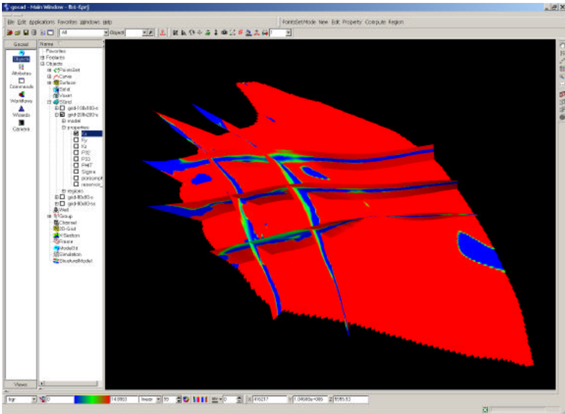
Figure 3-102. Distribution of effective fracture K_{xx} values in the Overthrust Block
