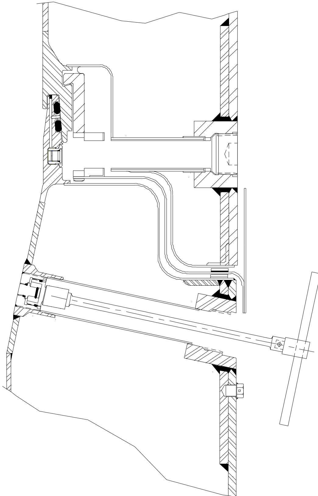
Figure 1.2 - ICV / OCV Vent Port Cover Removal Tool (2077-092-A1)
