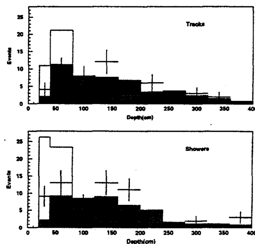
Fig. 1: The depth distributions for tracks (top) and showers (bottom)
