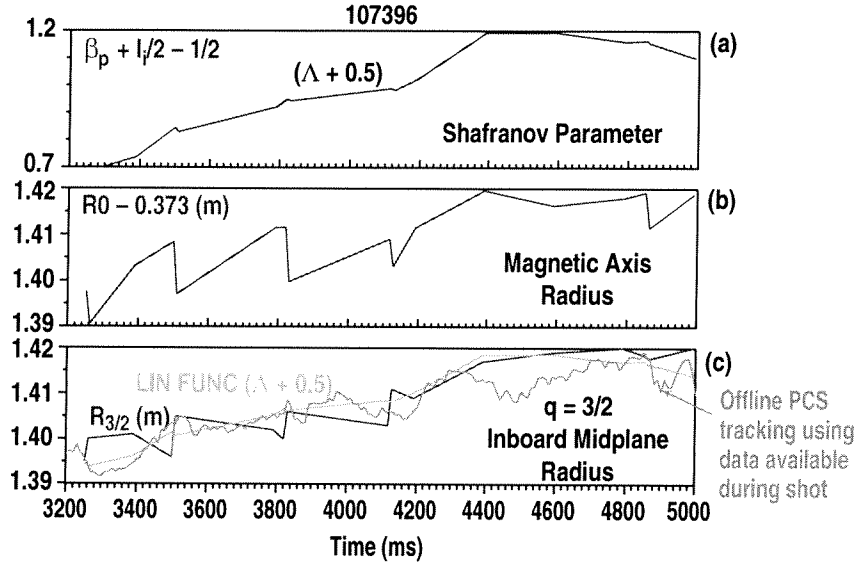
Fig. 4. For the discharge 107396 of Fig. 3 during the period in which beta is raised, (a) the Shafranov parameter \Lambda + 0.5 increases, (b) the plasma magnetic axis R_0 increases as a result (the plasma separatrix boundary is held fixed) and (c) the inboard midplane major radius R_{3/2} of q=3/2 also shifts outward. Also shown in (c) is a simple linear fit to \Lambda + 0.5 as well as the subsequently developed PCS tracking of the change in the q=3/2 location ready to be used in future work.
