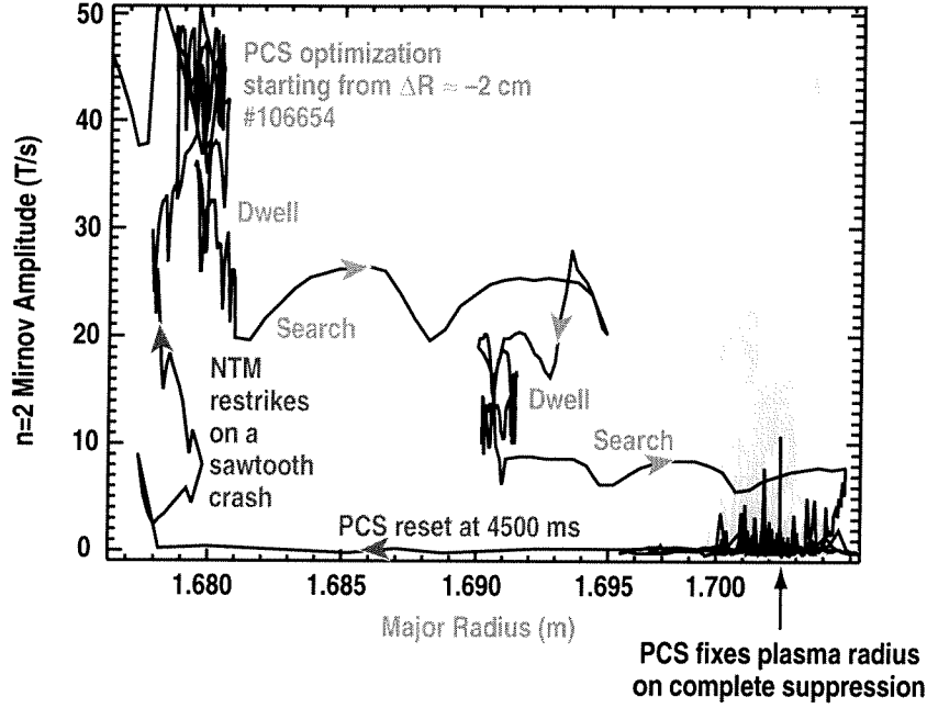
Fig. 2. Trajectory of n=2 Mirnov amplitude versus plasma major radius with (#106654) and without (#106642) real-time control of the plasma position for ECCD suppression ( m/n=3/2 NTM, three gyrotrons for 1.5 MW injected from 3000 to 4800 ms).
